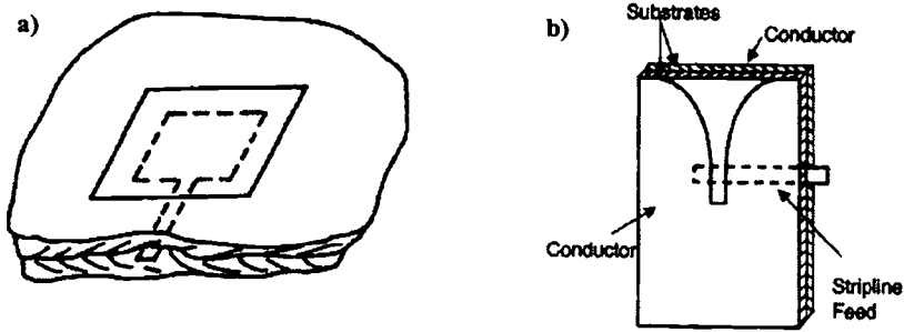
Figure 17.18. Microstrip Patch and Flared Notch Elements: a) proximity coupled microstrip patch (ground screen beneath lower substrate); b) Strip-line fed Flared Notch Element.
