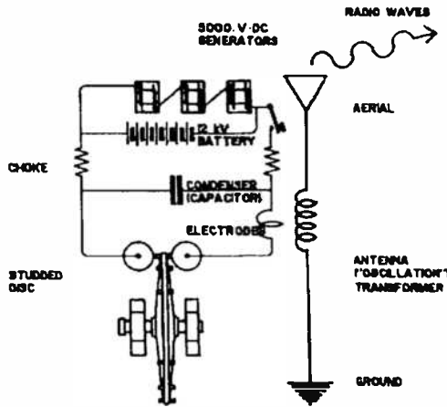
Figure 12.31. Schematic circuitry of Marconi's Glace Bay, NS high power spark transmitter
