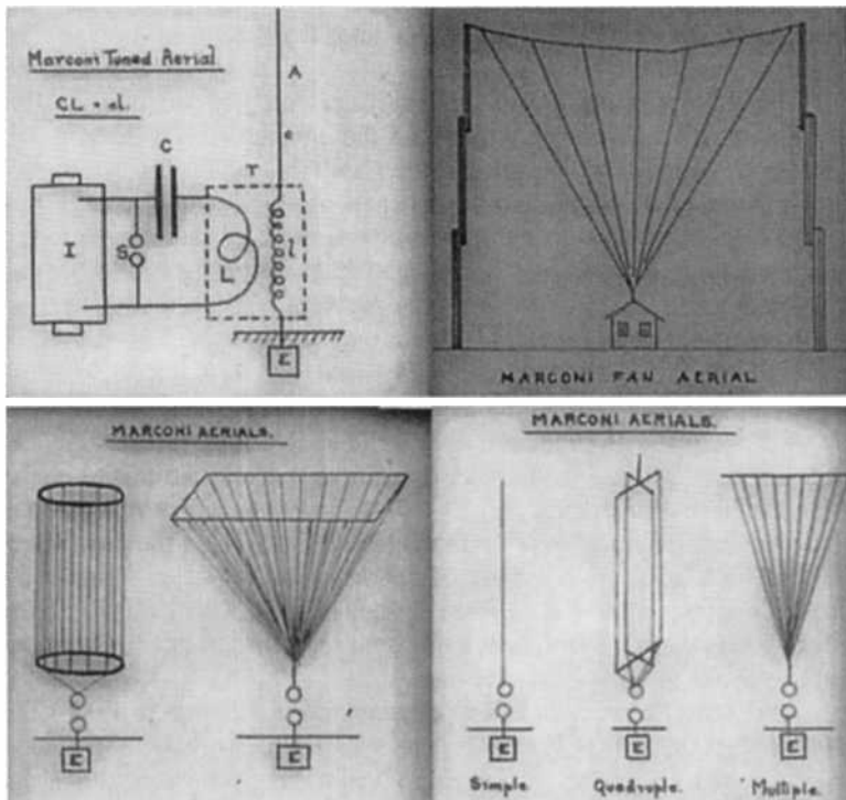
Figure 10.4. Examples of Marconi's designs for wireless aerials.
