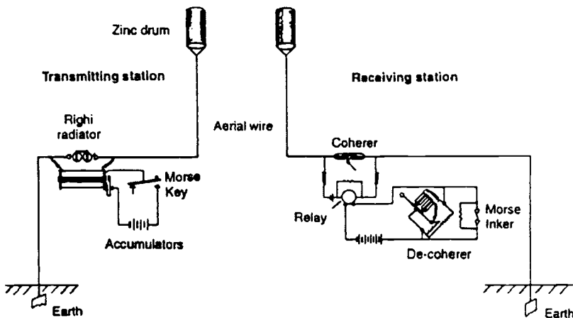
Figure 12.3. Circuit diagram of the plain aerial transmitter-receiver system used during Marconi’s Lavernock Point trials in May 1897 (after Lemme and Menicucci [27]).
