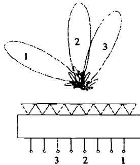
Figure 17.12. Multiple Beam Array.
