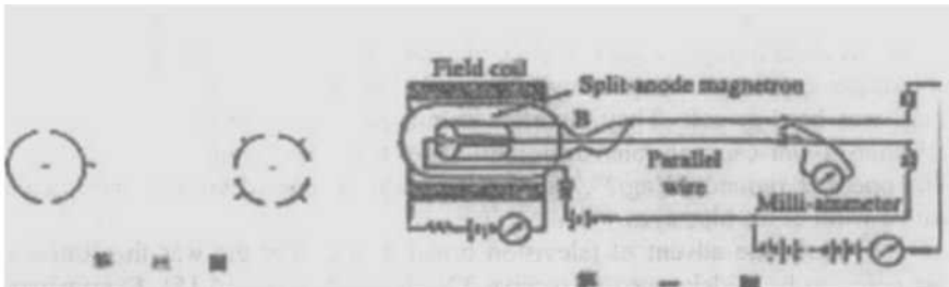
Figure 14.11. Split-anode magnetron, 2 and 4-segment type, 2-segment type magnetron with the oscillation circuit (K.Okabe, JIEE, march 1928).
