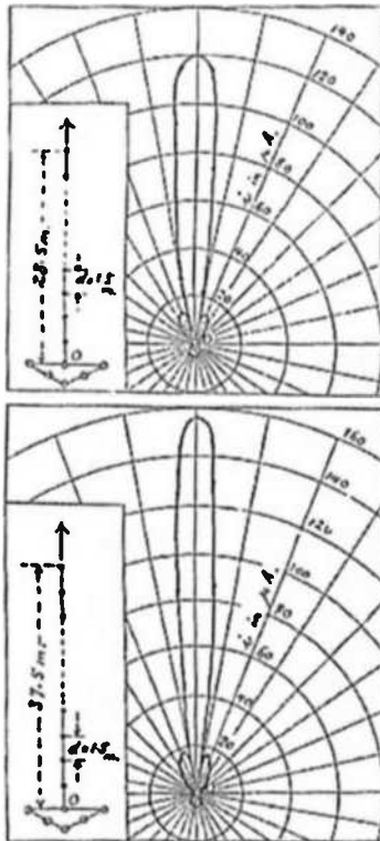
Figure 14.8. Characteristics of Yagi-Uda antennas. (H.Yagi and S. Uda, Proc. Imperial Academy, Feb. 1926) (S. Uda, JIEE, June 1927).
