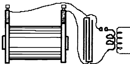
Figure 8.1. First drawing of the Tesla Coil driven by Ruhmkorff coil presented in his 1891 lecture.
