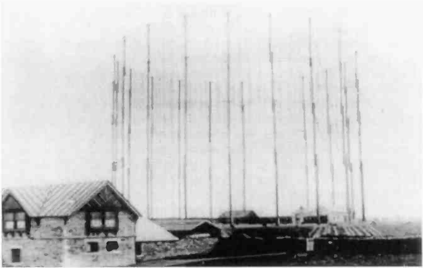
Figure 12.22a. Poldhu aerial systems: first inverted-cone aerial.
