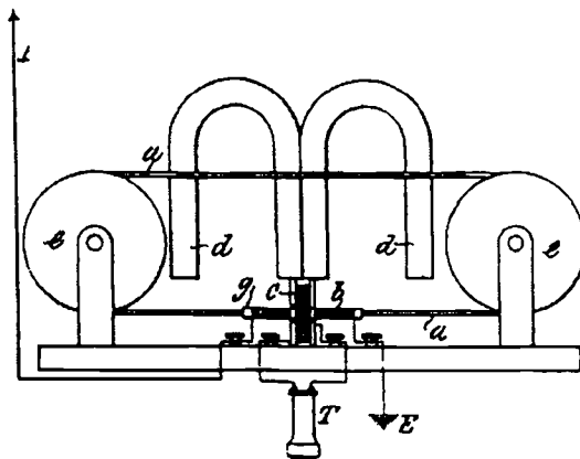
Figure 12.11a. Diagram from Marconi's Patent No. 10,245 of 1902 showing the magnetic detector.
