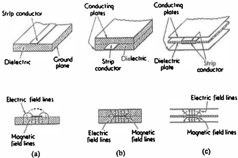
Figure 16.4. Typical commercial microwave printed systems; (a) Microstrip, Federal Telecommunication Laboratories, ITT. (b) Tri-Plate, Sanders Associates. (c) Stripline, AIL. (From [45], p. 985, Fig. 4.)
