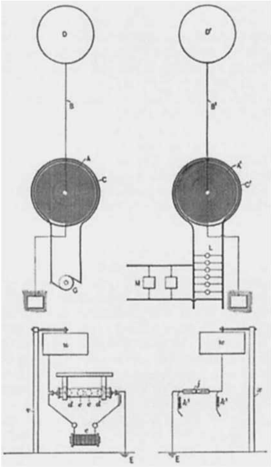
Figure 8.5. Tesla's system of four tuned circuits (US Patents [10,11]) and Marconi's system as shown in his US patent 11,913 June 4,1901. Applications to all these patents are filed in 1897.
