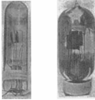
Figure 14.12. Split-anode magnetron. (H.Yagi, Proc. IRE, June 1928), (left) 2-segment type, (right) 4-segment type.
