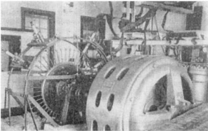
Figure 12.7. Fessenden's synchronous spark transmitter.
