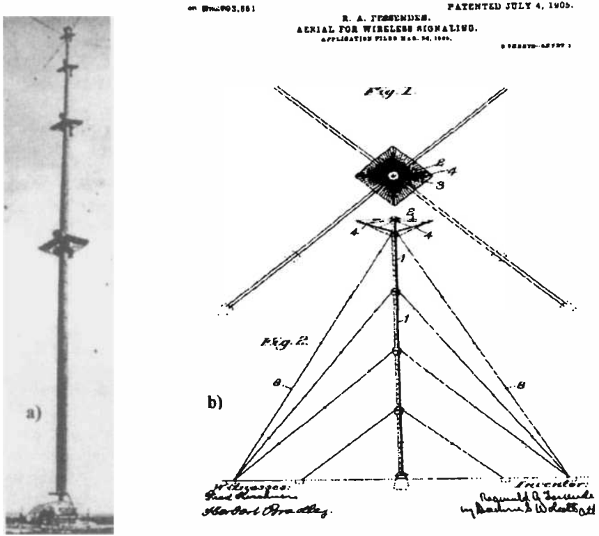
Figure 12.24. a) (left) Fessenden’s Brant Rock, MA mast aerial used for his transatlantic experiments in 1906. b) (right) A sketch copied from Fessenden’s 1905 patent.
