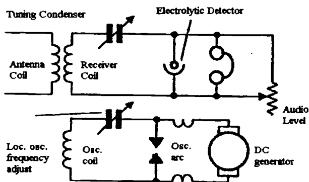
Figure 12.13. Sketch of Fessenden's advanced heterodyne receiver system.
