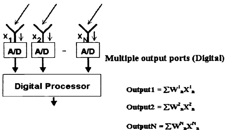
Figure 17.7. Digital Beamformer In Receive Mode.
