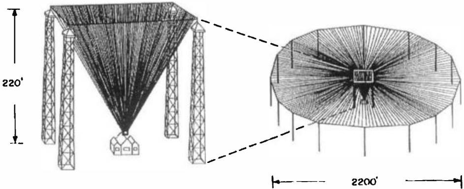
Figure 12.23. Marconi's antenna systems used at Table Head, Glace Bay, NS (on the left); and (on the right) at Marconi Towers, Glace Bay, NS.
