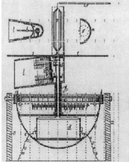
Figure 11.8. Schematic of Hülsmeyer's quasi-monostatic RADAR system. Quasi-monostatic system with single frequency operation, tunable PRF, 1m wavelength, a: Support structure, b: Cardian Join azimuth, c: Cardian joint elevation, d: Induction coil, h: spark gap, t: Large metallic disc to reduce coupling between transmit and receive. Transmitting Aerial: m: Concave Mirror, l: Projection Case, Receiving Aerial 'o': n: Cage Arrangement Reflector.
