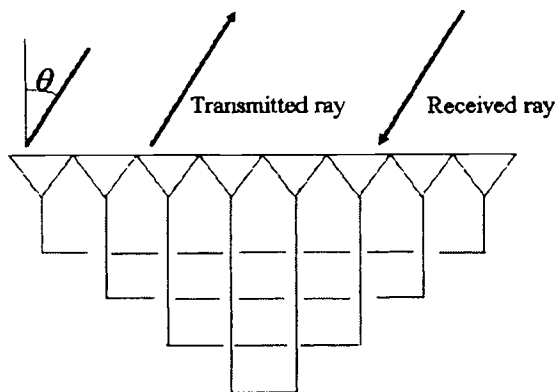
Figure 17.11. Van Atta Retrodirective Array.
