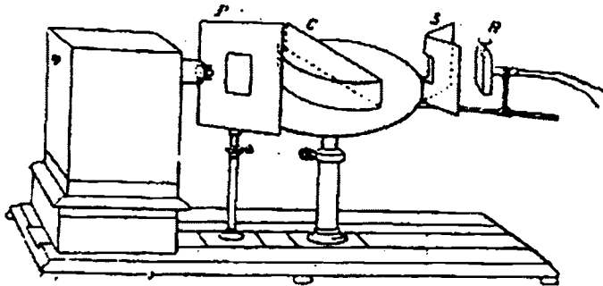
Figure 9.5. The electric refractometer developed by Bose [4]. P – the plate with a diaphragm; C – semi-cylinder of glass; S – the shield (only one shown in the diagram); R – the receiver.
