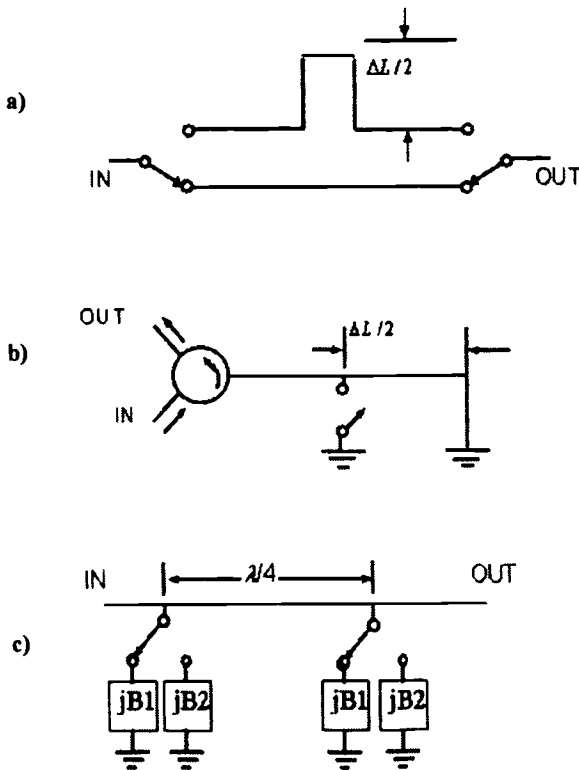
Figure 17.6. Electronic Phase Shifter Circuits a) switched line phase shifter b) reflection phase shifter c) loaded line phase shifter.
