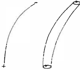
Figure 3.8. Faraday's magnetic line of force connecting positive and negative magnetic charges can be interpreted in terms of a rotating tube connecting equivalent current loops.
