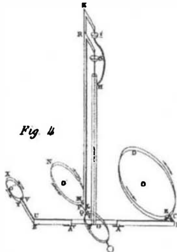
Figure 3.4. Ampère's null-force experiment. The forces by the loops on each side of the movable loop cancel one another when the sizes and distances of the two loops are in the same ratio and the current in all loops is the same. This leads to the 1/r^2 force law.
