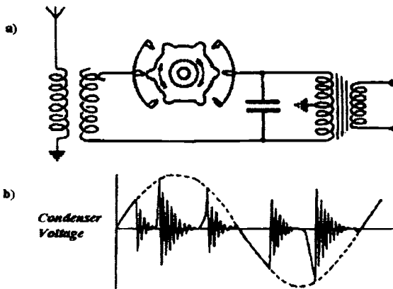
Figure 12.6. a) A synchronous rotary gap arranged to generate sparks on, b) both positive and negative excursions of the AC voltage.
