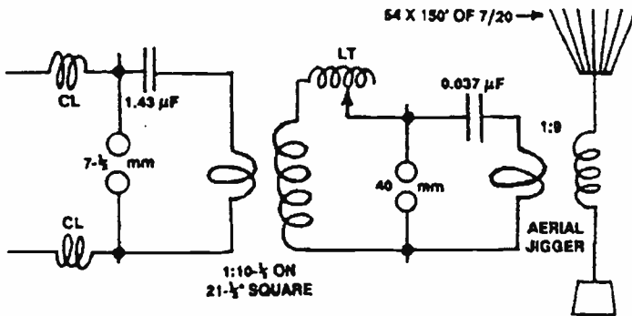
Figure 12.27b. Schematic (redrawn) showing component values, note the additional components CL (extra coils), and LT (a long adjustable tuning inductance of forty turns using 40 feet of wire), after Thackeray [52].
