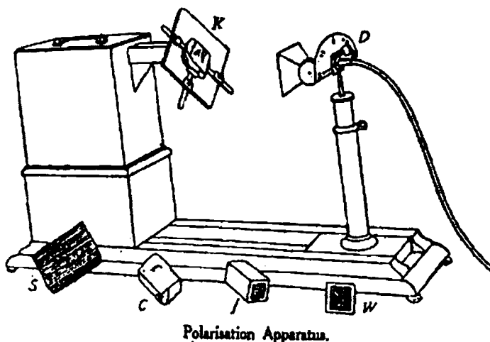
Figure 9.6. The polarization apparatus developed by Bose [4]. K- Crystal Holder; S – a piece of stratified rock; C – a crystal; J – jute polarizer; W – wire grating polarizer; D – vertical graduated disc by which rotation is measured.
