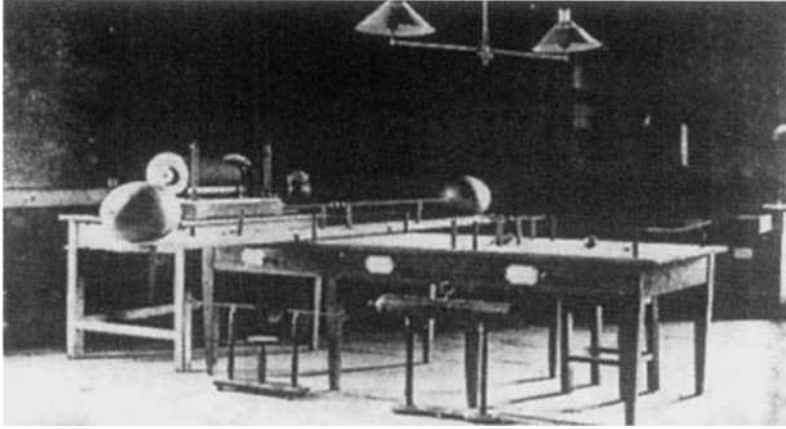
Figure 11.4. Original Hertzian oscillator at Institute of Physics of Polytechnical University of Karlsruhe (1886-1888).
