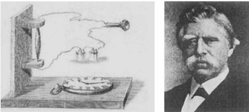
Figure 7.12. The microphone by Hughes was based on a loose contact of a pointed carbon bar which made it sensitive to catch the faintest vibrations. It also served as a nonlinear detector in his wireless experiments.
