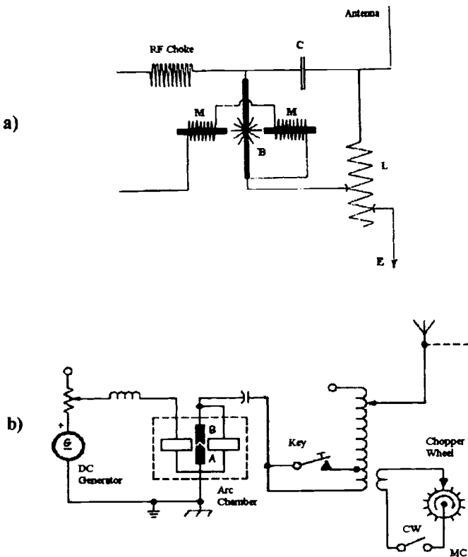
Figure 12.14. a) Poulsen Arc Oscillator with Magnetic Blast; b) a practical arc transmitter, for purposes of discussion (after Schrader[47]).
