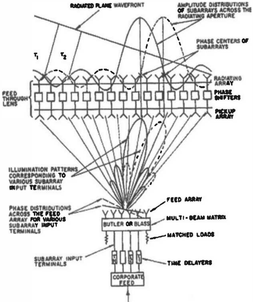
Figure 17.17. Completely Overlapped Subarray Antenna System (after Tang [104]).
