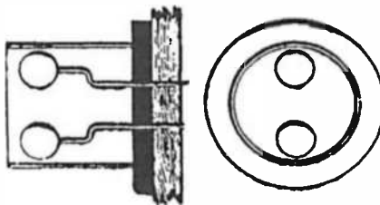
Figure 15.7. Lodge’s waveguide radiator having the form of a section of a copper tube with circular cross-section used in 1894 (reproduced from [36]).
