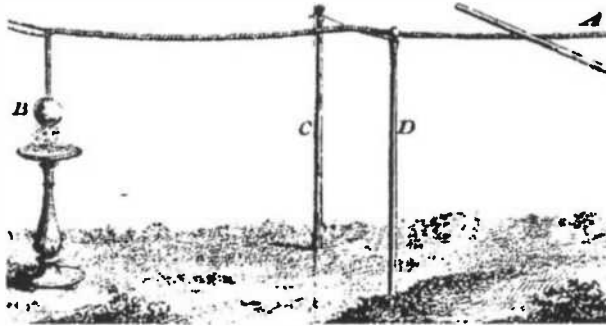
Figure 7.1. The first transmission line by Gray conveyed the electrostatic force from a rubbed glass tube to an ivory ball over common packthread hanging on isolating strings.
