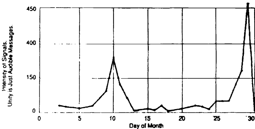
Figure 12.41. Curve showing variation of the intensity of transatlantic signals (path Machrihanish-Brant Rock, frequency about 80 kHz) for the month of January 1906.
