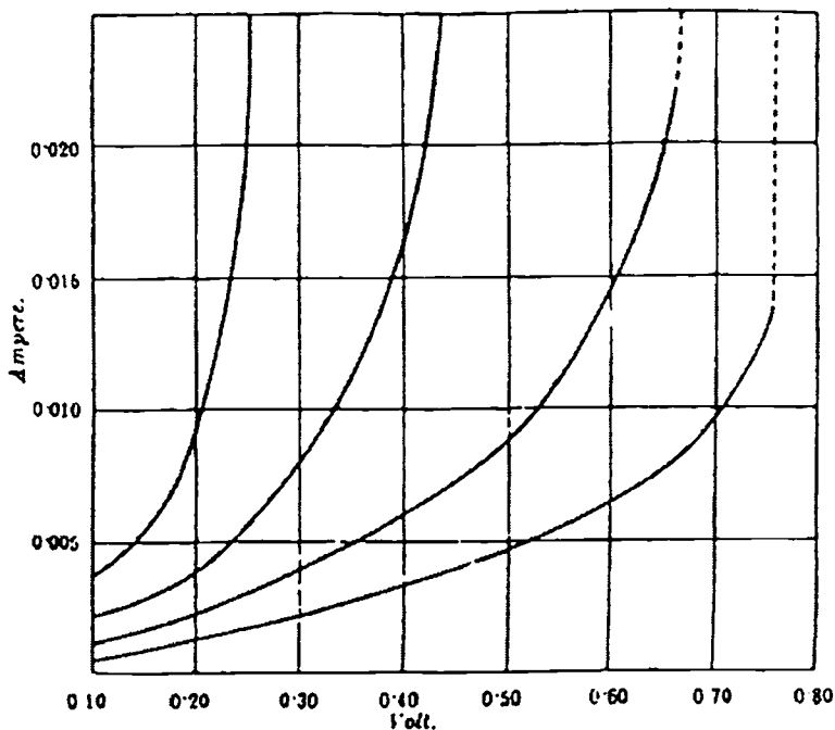
Figure 9.9. V-I characteristics of a point contact device [4].
