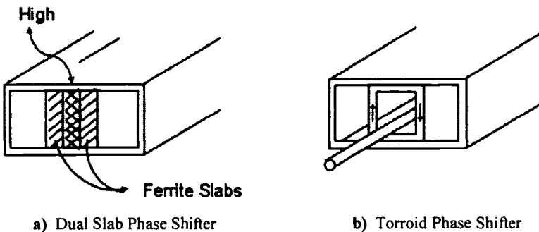
Figure 17.5 Ferrite Phase Shifter Configurations.
