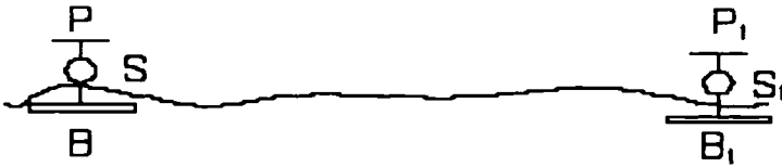
Figure 8.3. Tesla's proposition from 1893: S – high frequency generator: B-ground plate; P-elevated plate (antenna). Receiver is tuned to the transmitter frequency.
