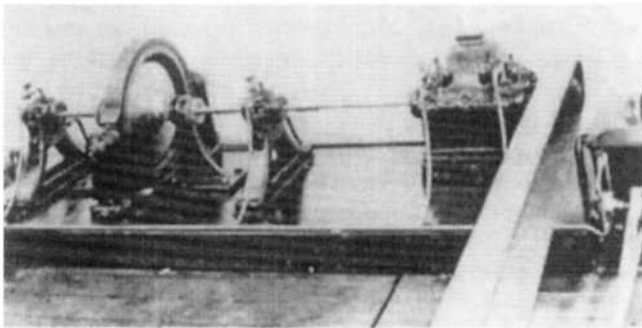
Figure 12.15. Photograph of Fessenden's first HF alternator.
