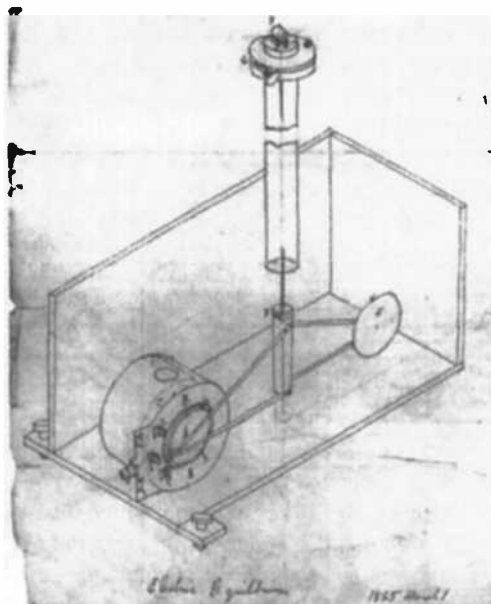
Figure 4.8. Maxwell's drawing (1865) of the torsion balance for the determination of the ratio of electrostatic and electromagnetic units of electricity.
