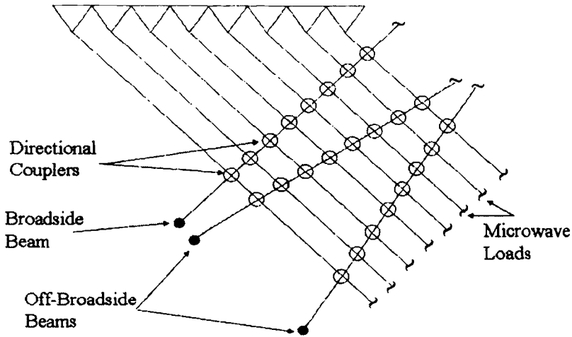
Figure 17.15. Time Delayed Version of Blass Matrix.
