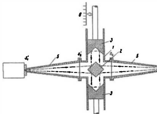
Figure 15.26. Circuit of the Michelson interferometer used in 1968 based on rectangular OSW with cross-section of 23 by 10 mm working with the H_{10} mode at \lambda = 1-4 \text{ mm} designed at IAP RAS (reproduced from [117]).
