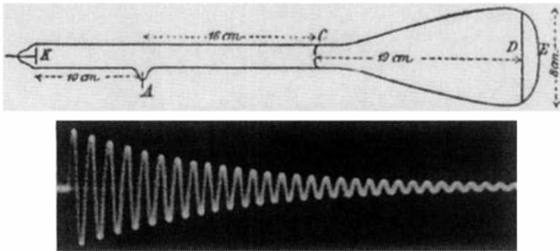
Figure 11.5. Braun's cathode ray tube.
