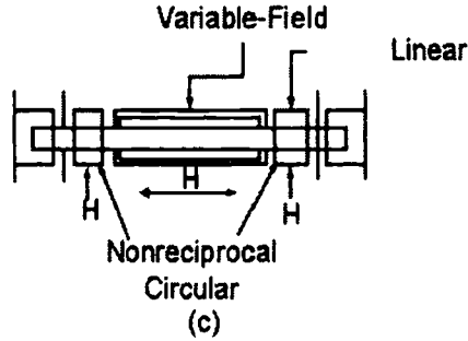
Figure 17.5c. Ferrite Phase Shifter Configuration: Dual Mode Reciprocal Phase Shifter.
