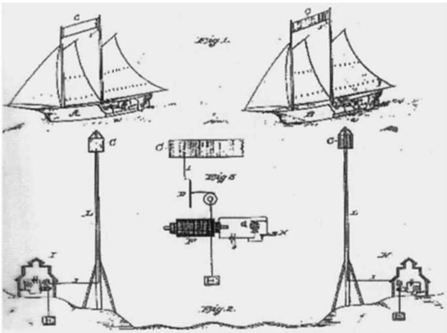
Figure 7.7. Edison's patent for wireless telegraphy between ships and ground stations used chopped current and telephone receivers. The antennas relied on quasi-static capacitive coupling.
