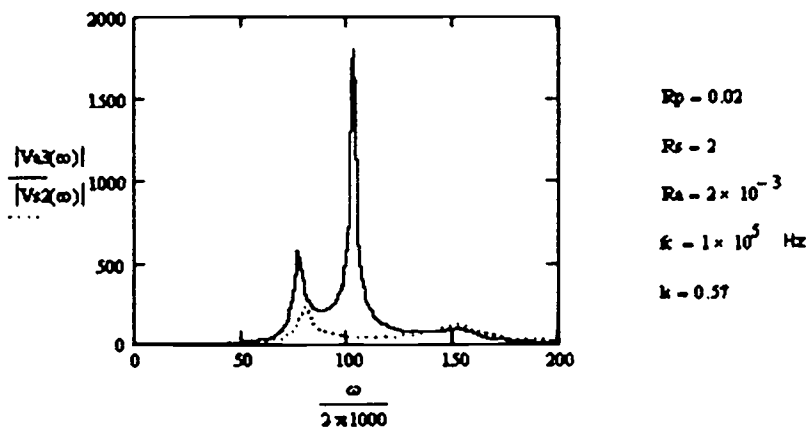
Figure 8.9. Relative voltages across output terminal of three coupled circuits (full line) and two coupled circuits (dashed line): primary circuit ( L_p C_p ), secondary circuit ( L_s C_s ) and circuit with extra coil ( L_{ex} C_a ).
