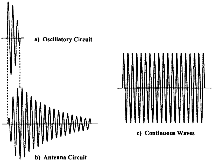
Figure 12.4. Idealized waveforms in the oscillation circuit a) ; and the antenna circuit b) . The spark generated damped waves are much more noisy and broadband compared with c) undamped or continuous waves.
