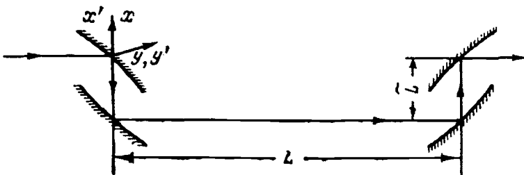
Figure 15.34. Periscopic reflector beam waveguide of 1965 (reproduced from [149]).
