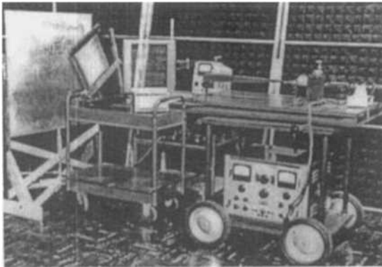
Figure 15.17. Open type antenna duplexer for operation in a circularly polarized mode at \lambda = 8.5 \text{ mm} used in 1962 (reproduced from [76]).
