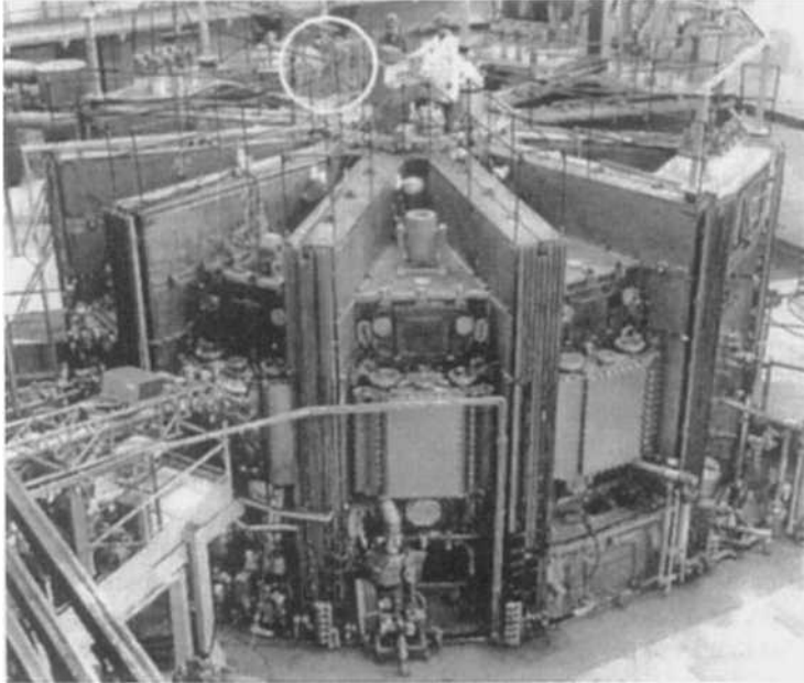
Figure 15.42. General view of the nuclear fusion machine Tokamak T-15 at IAE; with a circle marking the placement of the QO interferometer (photo provided by V. Kiseliiov, 1985).
