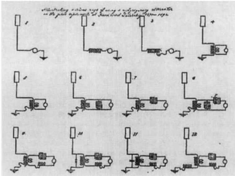
Figure 8.2. Various connections of high frequency transformers used by Tesla in 1891–1892 (Tesla's own slide, now at the Nikola Tesla Museum, Belgrade).
