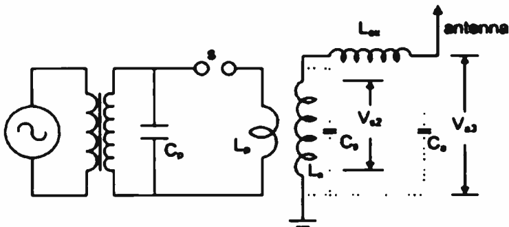
Figure 8.8. Lumped elements three-circuit Tesla coil.
