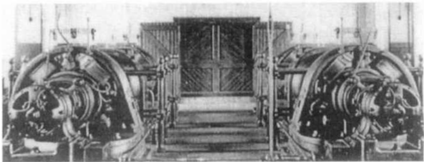
Figure 12.32. DC power source for the Glace Bay, NS station, four 5000 volt DC generators (one is a spare).
