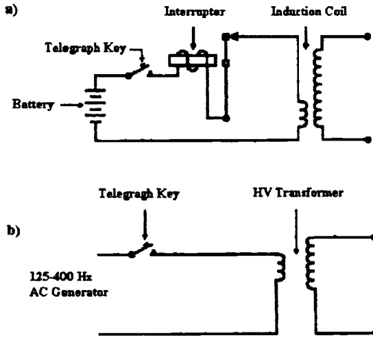
Figure 12.5. Power sources for spark transmitters.
