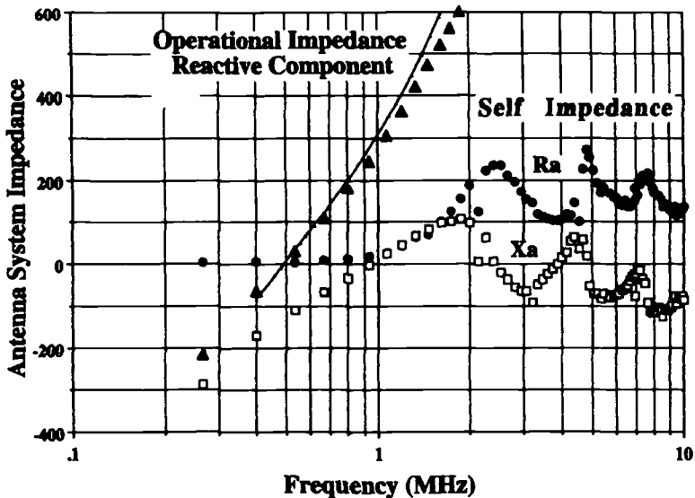
Figure 12.28. Impedance vs. frequency for Marconi's temporary fan monopole December 1901 (experiment and simulation)
