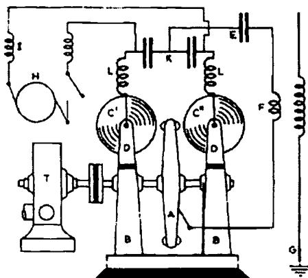
Figure 12.36. Final version of Marconi's rotating disc charger (1908), which was intended to simulate a CW like signal.
