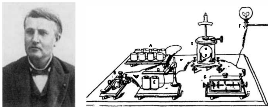
Figure 7.11. Edison's setup for studying the etheric force. Current from battery A is chopped by key B whence the inductance C gives a spark D. Galvanometer E does not react but there is a visible spark in the spark gap G grounded in the gas mains F.
