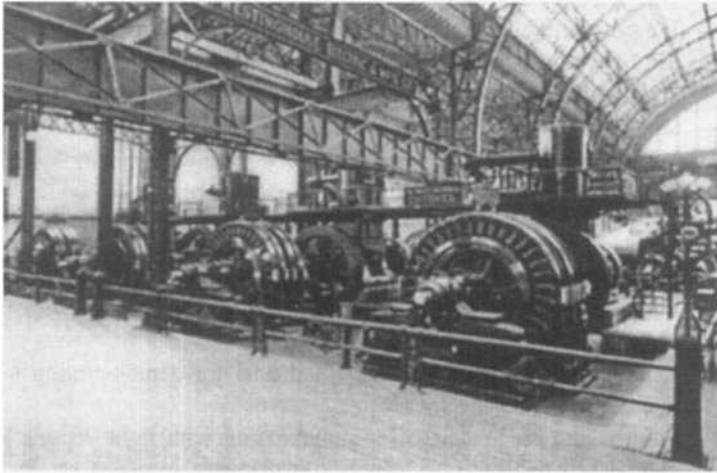
Figure 2.26. Tesla's AC power plant at World's Fair (Columbian Exposition), Chicago, 1893 showing four of the twelve 1000 horse power two-phase generators.
