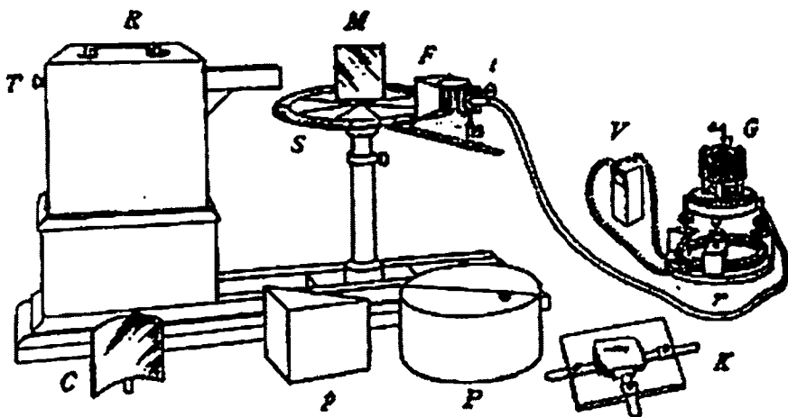
Figure 9.2. Electromagnetic Horn receiving antenna on microwave spectrometer used for quasi-optical demonstrations by Bose (1896). [Scanned from Longman's and Green Co].
