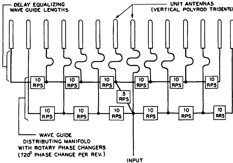
Figure 17.2b. Phase Control for a Polyrod Array.
