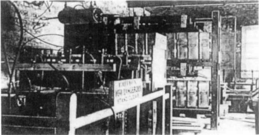
Figure 12.27a. The two-stage spark transmitter system used for this experiment
