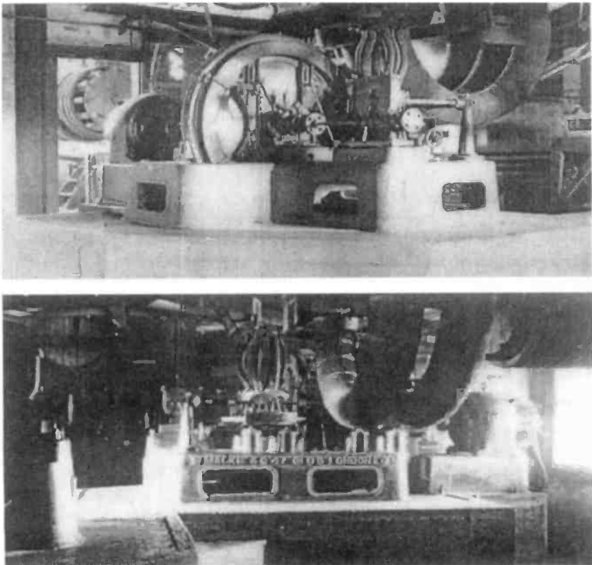
Figure 12.35. Photographs of Table Head, Glace Bay, NS spark transmitter (credit Canadian Marconi Company).
