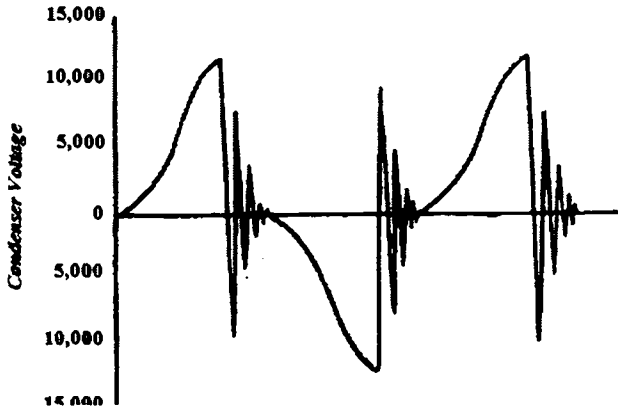
Figure 12.8. Synchronous spark transmitter 2-sparks/cycle precisely at voltage peaks of the AC waveform.
