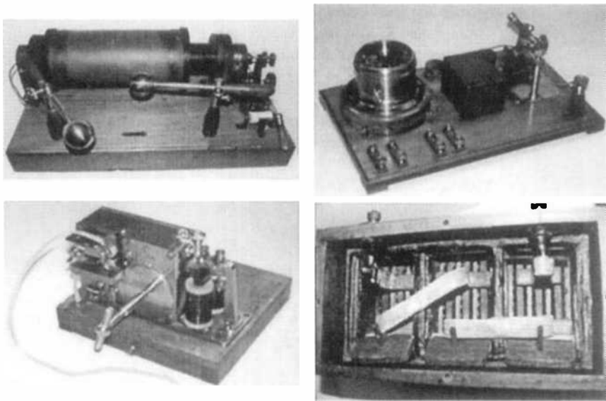
Figure 13.16. Wireless telegraphy equipment ( upper left ) Refurbished Marconi Wireless Telegraph Co. Ltd. London Ruhmkorff coil (No. 31705) used for transmitting wireless telegraph signals during the South African War of 1899-1902. ( upper right ) Refurbished receiver consisting of a Siemens and Halske AG telegraphic relay (No. 23959) with coherer used to receive wireless telegraphy signals. This is believed to be one of only two original receivers used during the South African War of 1899-1902 still in existence. ( lower left ) Morse code inker (Farbenschreiber) (No. 50478) used to print Morse code signals on a paper strip for reading by wireless telegraphy operators. ( lower right ) Battery used as power source for the Ruhmkorff coil transmitter. (All photos by courtesy of the Museum of the Boer Republics, Bloemfontein, South Africa).
