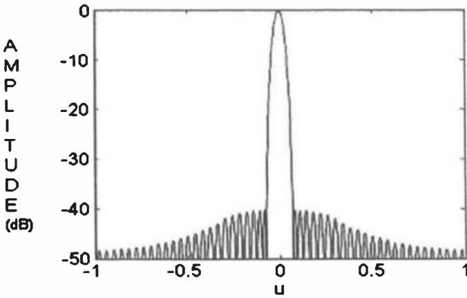
Figure 17. 9a. Low Sidelobe Taylor [73] Radiation Pattern ( n = 8 ) .
