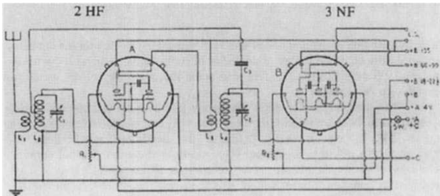
Figure 11.13. Circuit diagram of the “five-in-two”-receiver, note that the two tubes are coupled through the tuned-radio-frequency transformer composed of coils L_3 and L_4 and the condenser C_2 . The first stage of RF amplification is resistance-coupled.
