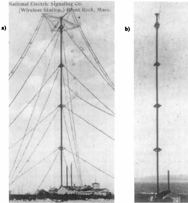
Figure 12.37 a) General view of Brant Rock, MA station, date not known but probably after 1906, showing the shore in the forefront. Notice the tall smoke stacks by the steam engine to power the station. The Brant Rock tower might be standing today if it was not cut down during WW1, since the United States did not want this landmark visible to enemy ships at sea. For comparison b) shows the station at Machrihanish, Scotland
