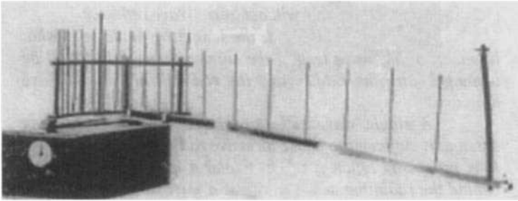
Figure 14.9. One of the original apparatus of Yagi-Uda antenna made in 1929.
