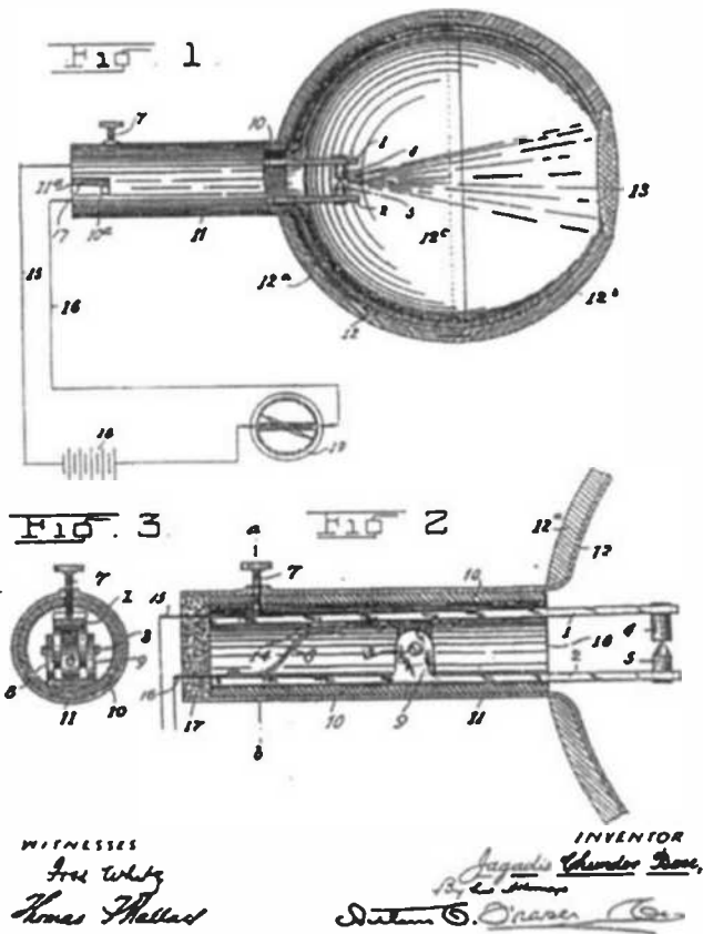
Figure 2.34. Bose's drawings for patent "Point contact diode using galena".
