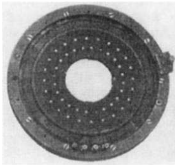
Figure 12.17. One half of the completed armature [after Zennick, 52].
