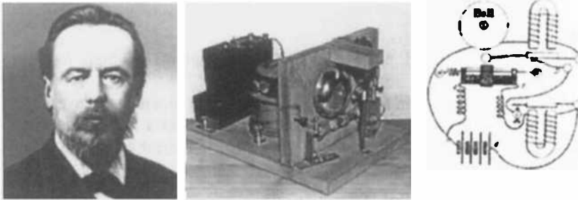
Figure 2.27. From left to right, Alexander Stepanovich Popoff (1859–1906), Popoff's radio receiver, and its electrical scheme.
