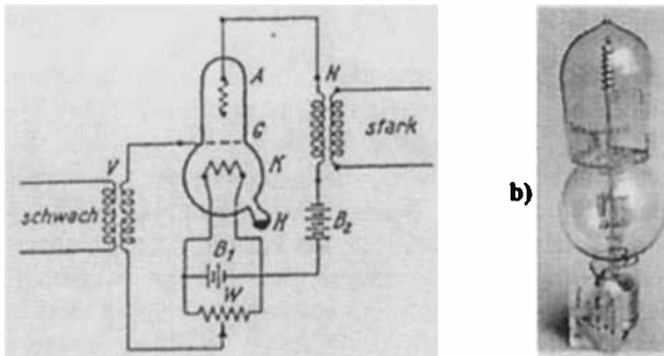
Figure 11.10. a) Circuitry for the Lieben tube, b) The big Lieben tube (height: 315 mm).
