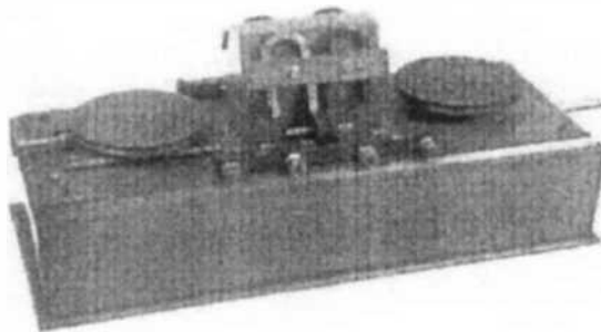
Figure 12.11b. Photograph of a commercial version of Marconi's magnetic detector device.
