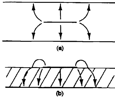
Figure 16.3. Cross-sections of (a) stripline and (b) microstrip line, showing the basic electric field lines (from [8], p. 1033, Figure 5).
