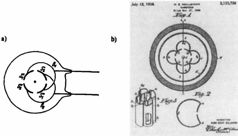
Figure 11.16. Pictured above are schematics of a) Habann's split-anode magnetron, and b) Hollmann's multi-cavity magnetron.
