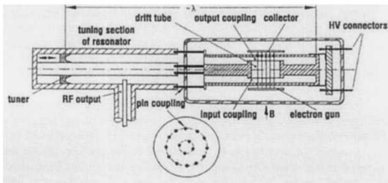
Figure 11.19. The Heil Generator (coaxial-line oscillator) [17], (bottom) Cross-section of Heil Generator RD12La (C. Lorenz AG) \lambda = 21.5 - 24 cm, PRF = 15 W, U_0 = 500 V, I_0 = 200 mA, B = 0.15 T.
