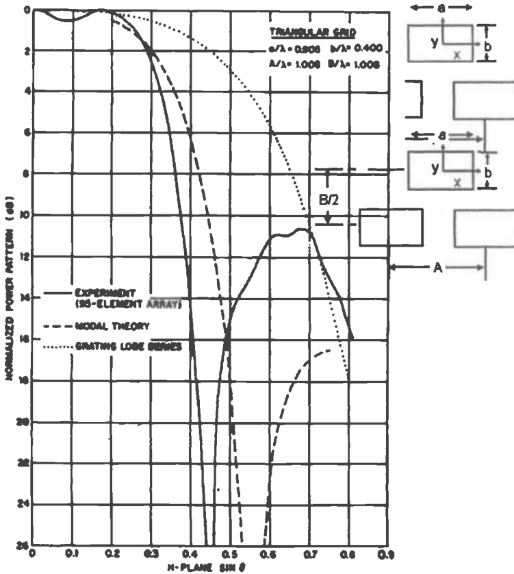
Figure 17. 10. Array Element Pattern Illustrating "Blindness," after Farrell and Kuhn [83,84].
