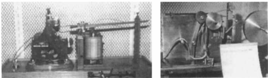
Figure 2.13. Left, photograph of Morse's embosser utilized in 1844 as recording device. In 1845 Bain's chemical recorder, shown in the right photograph, substituted it.
