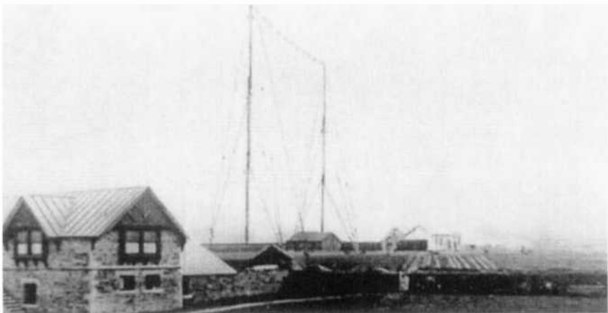
Figure 12.22c. Poldhu aerial systems: a temporary fan aerial (credit BAE Systems Marconi Research Centre, Chelmsford, Essex).
