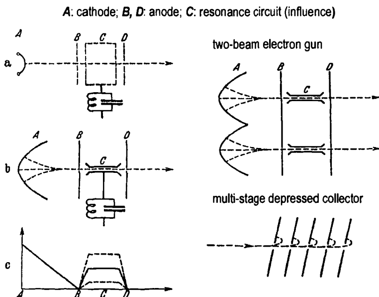
Figure 11.18. Original drawings from the Heils' publication, figures 1 (left), 9 (upper right), and 10 (lower right).
