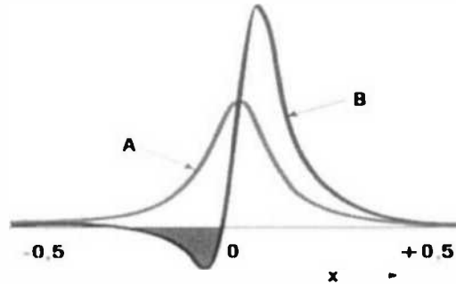
Figure 11.23. Cyclotron resonance absorption of electrons ( x = (\omega_{\pi+1} - \omega_{RF}) \tau ), non-relativistic (A), relativistic (B).
