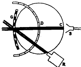
Figure 9.7. Sketch of experimental setup to measure wavelength [23].
