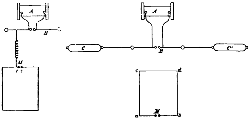
Figure 11.3. Experimental set-ups of Heinrich Hertz (A) Inductorium, (B) Spark gap in transmitter circuit, (C) Metal spheres at both ends of transmitting antenna, (M) Spark gap in receiver circuit (“Nebenfunkeln”).
