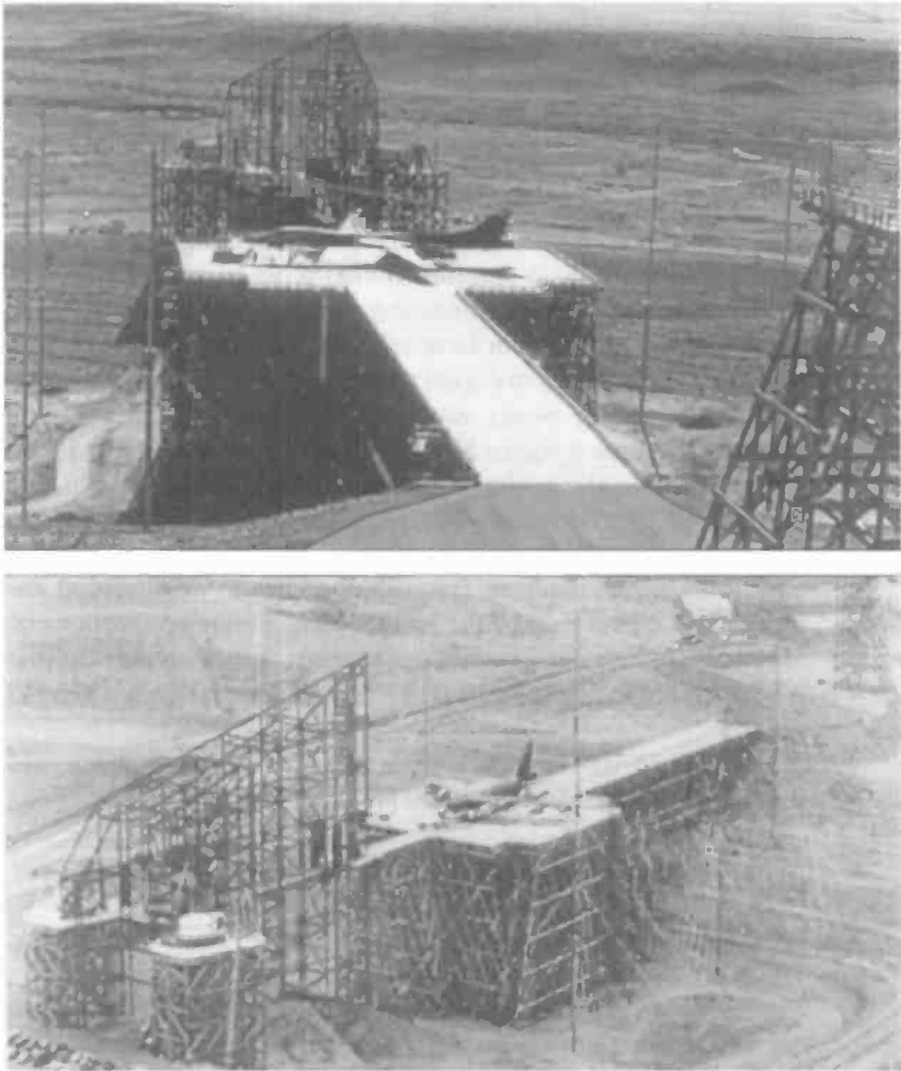
Figure 2.50. The ATLAS I EMP Simulator with a full scale B1B (upper photograph) and a C130 (lower photograph) undergoing test (photos provided by Carl E. Baum, AFRL).
