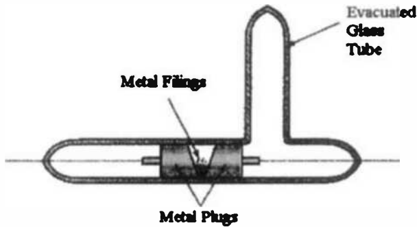
Figure 12.9a. Diagram of a coherer.
