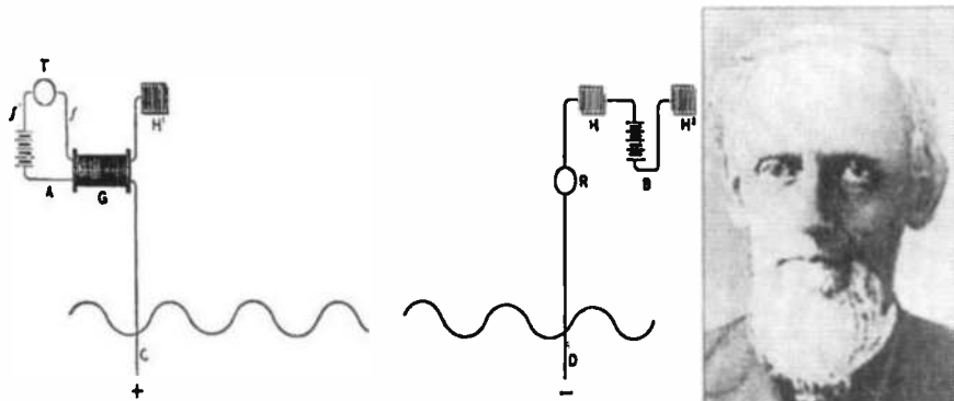
Figure 7.6. Dolbear's wireless telegraph resembles that of Marconi with antennas and ground electrodes. However the frequency of operation in the first experiments was too small for the electromagnetic waves. Dolbear interpreted the operation through currents in the ground.
