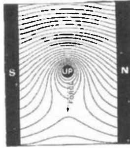
Figure 3.7. Faraday viewed the magnetic lines like rubber bands connecting opposite magnetic charges. The lines make tubes which expel each other laterally. Here the current flowing in a wire between the magnetic poles experiences a force due to the field lines.
