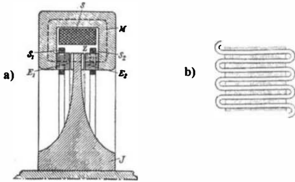
Figure 12.16. The Fessenden-Alexanderson HF alternator: a) diagrammatic cross-section of one of these alternators; and b) the armature winding in which the EMF was induced [after Zennick, 52].
