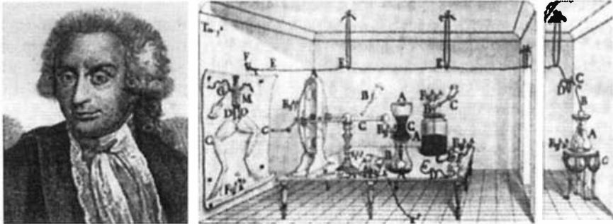
Figure 7.10. Continued experiments with his observation on the effect of electric sparks on frog legs could have made Galvani an early inventor of the electromagnetic wireless.
