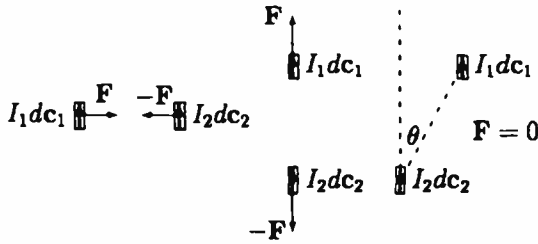
Figure 3.3. Ampère's law for two parallel current elements predicts both attractive and repulsive forces. At a certain angle the force disappears.
