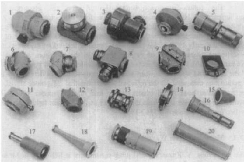
Figure 15.39. Quasi-optical LEGO-like kit for a sub-mm wave engineer. HDB-based components used for building wideband ( \lambda = 0.5-1.7 mm) measuring circuits developed in IRE NASU: 1- polarization attenuator, 2- polarization phase shifter, 3- tunable attenuator-power divider, 4- polarization plane rotator, 5- wave meter, 6- polarization converter, 7- tunable phase shifter, 8- matching tuner, 9- beam splitter, 10- cassette of polarization discriminator, 11- linear polarizer, 12- right-angled corner, 13- movable two-facet reflector, 14- rotating joint, 15- terminating load, 16- movable reflector, 17,18- two waveguide-to-beamguide transitions, 19- telescopic section, 20- HDB straight section (photo provided by V. Kiseliiov, 1971).
