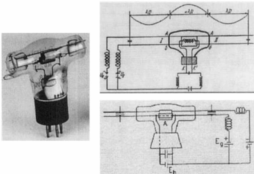
Figure 11.12. (left) Retarding-field tube RS296 and its circuit, (upper right) Hollmann 1930 and (lower right) Kühle 1932 at Telefunken, “Hammer Tube” [8,11].
