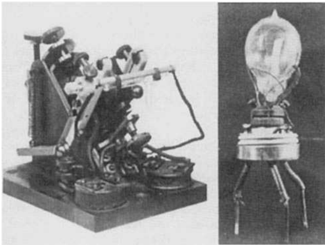
Figure 10.8. Fleming's first wireless valve (right) compared with Marconi's coherer (left); which it replaced. Photos reproduced by courtesy of the Director of the Science Museum, South Kensington.
