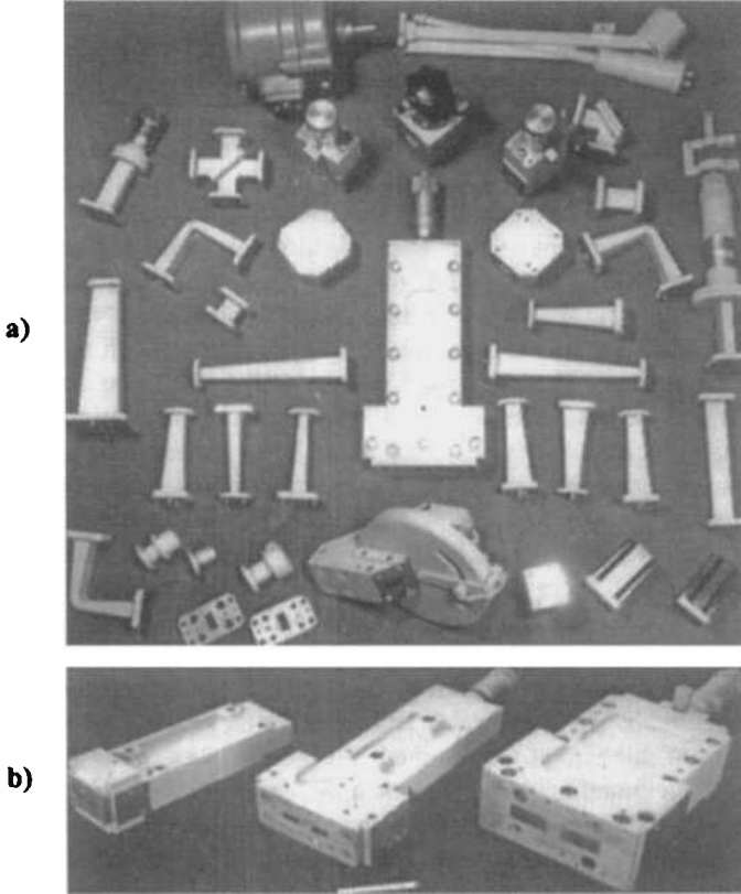
Figure 15.27. The components of 1970 a) and superheterodyne radiometers b) based on the rectangular OSW with the H_{10} mode developed at IAP RAS (photo provided by I. I. Fedoseyev).
