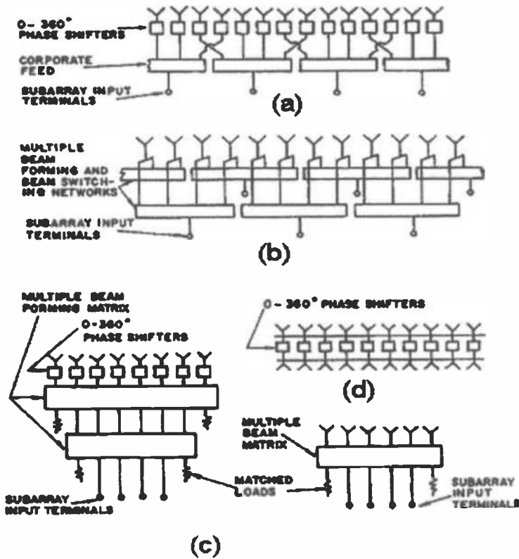
Figure 17.16. Subarray schemes for minimizing gain reduction and grating lobe level. (after Tang [104]).
