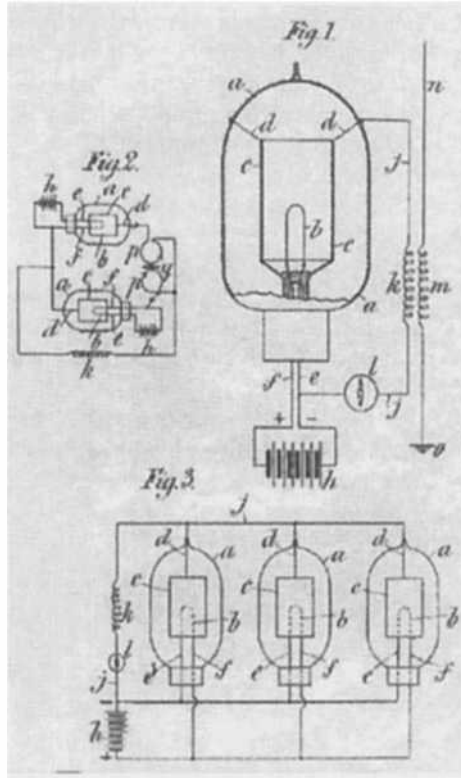
Figure 10.7. Valve Circuit from GB Patent No 24,850, 16 November 1904.
