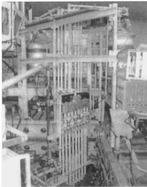
Figure 15.43. The second QO nine-channel HDB-based interferometer ( \lambda=0.337 mm) with an HCN-laser source for hot plasma diagnostics of Tokamak T-15 at IAE (photo provided by V. Kiseliiov, 1985).
