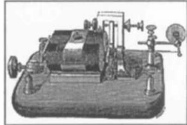
Figure 2.10. Upper part: Contemporary drawing of Morse's first telegraph equipment, 1837. Lower row: left, Morse's sounder widely use on telegraph lines after 1855; right, Morse's receiving magnet.
