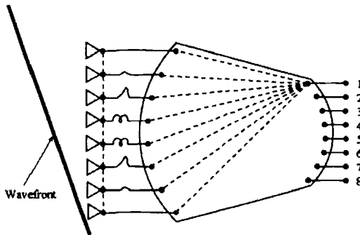
Figure 17.14. Rotman Lens, ray traces, and radiating wavefront.
