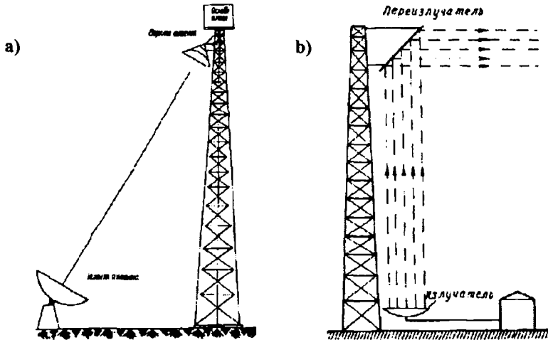
Figure 15.16. a) A microwave wireless power transmission line made of two focused reflector antennas, and b) a line of the periscopic type (reproduced from [68, 69]). Circa 1965.
