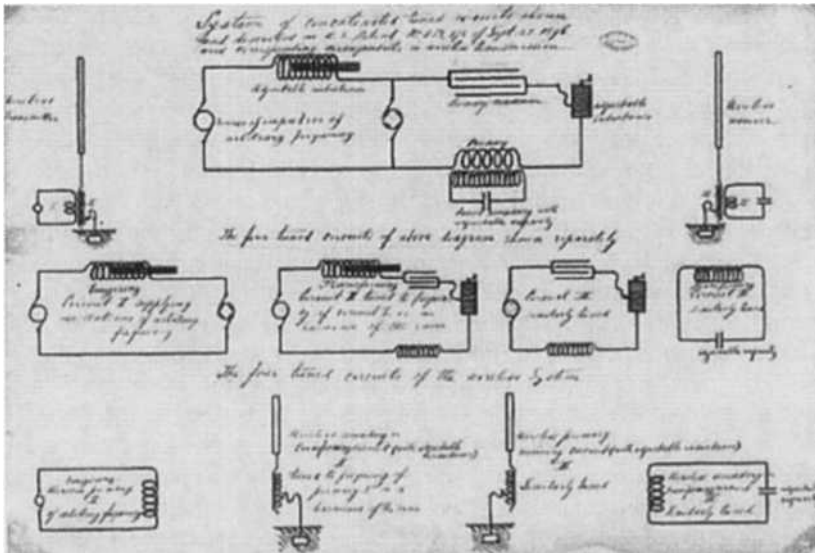
Figure 8.6. Tesla's drawing of four tuned circuits. The diagrams in Tesla's patents are as shown in upper part of Figure 8.5. (copyright Nikola Tesla Museum, Belgrade).
