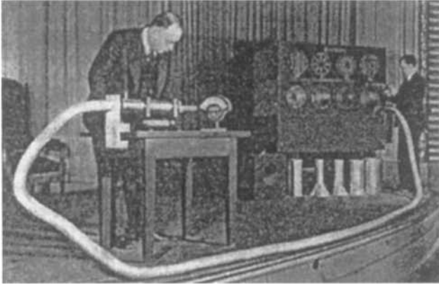
Figure 16.1. Photograph of George C. Southworth (foreground) demonstrating different waveguide modes of transmission and their cutoff frequencies on February 2, 1938. This was the first demonstration of waveguides before the Institute of Radio Engineers in New York (from [10], courtesy Gordon and Breach).
