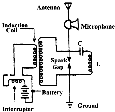
Figure 12.40. An early version of a transmitter for amplitude modulation shown with Fessenden's spark gap telephony transmitter, with a carbon microphone in series with the antenna lead
