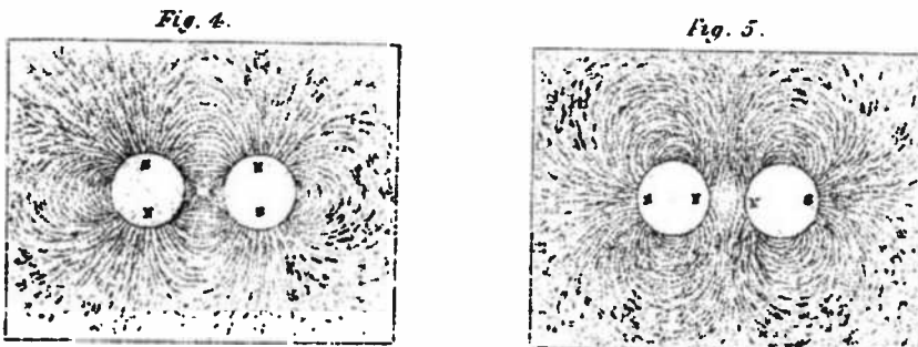
Figure 3.6. Faraday's concept of magnetic lines of force were suggested by figures made by iron filings in the vicinity of magnetized bodies. Because iron particles act like small magnets, there appears to be an attractive force along the magnetic line.
