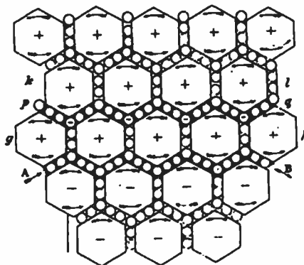
Figure 3.9. Maxwell's drawing depicting his mechanical model of electromagnetic fields. Direction of rotation of the vortex tubes with hexagonal cross section is shown by arrows. The line of balls A - B moving to the right represents an electric current. Because of the rigidity of the structure, the motion of all vortices is synchronous.
