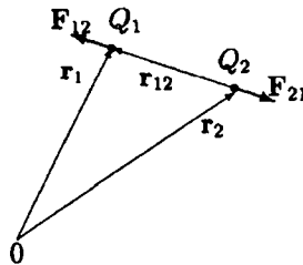
Figure 3.1. Coulomb's force between two static charges.
