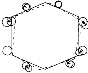
Figure 3.10. Assuming vortex tubes elastic so that fixed balls could be displaced by electric force made Maxwell's model elastic and capable of carrying mechanical waves. Displacement of electricity corresponds to current creating a magnetic field.
