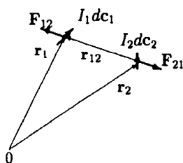
Figure 3.2. Ampère’s force law for two current elements.
