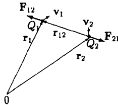
Figure 3.5. Weber's force law for two moving charges depends on the distance r_{12} and its time derivatives.
