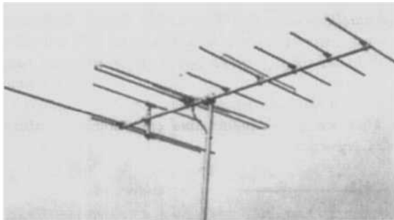
Figure 14.15. Yagi-Uda antenna for TV reception.
