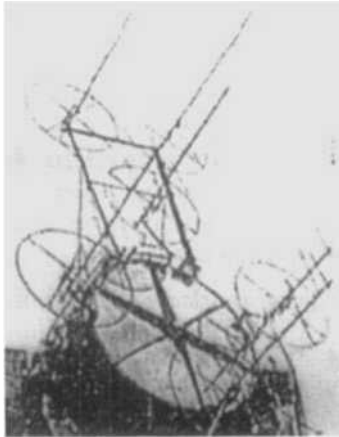
Figure 14.14. Yagi-Uda antenna employed in British radar for "Searchlight" (A Japanese translation of the book Radar written by Piere David, translated by Yukio Nakamura).
