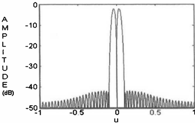
Figure 17. 9b. Asymmetrical Bayliss [74] Radiation Pattern ( n = 8 ) .
