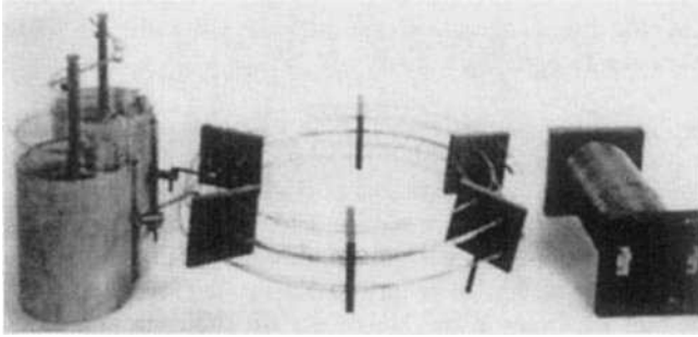
Figure 11.6. Braun's transmitter with two Leyden jars and two coupled resonance circuits.
