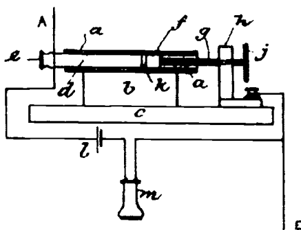
Figure 12.10. The Italian Navy Coherer as patented by Marconi in September 1901, British Patent No. 18,105 (after Phillips [35]); d = carbon plug, f = adjustable iron plug, k = drop of mercury, A = antenna, E = earth.
