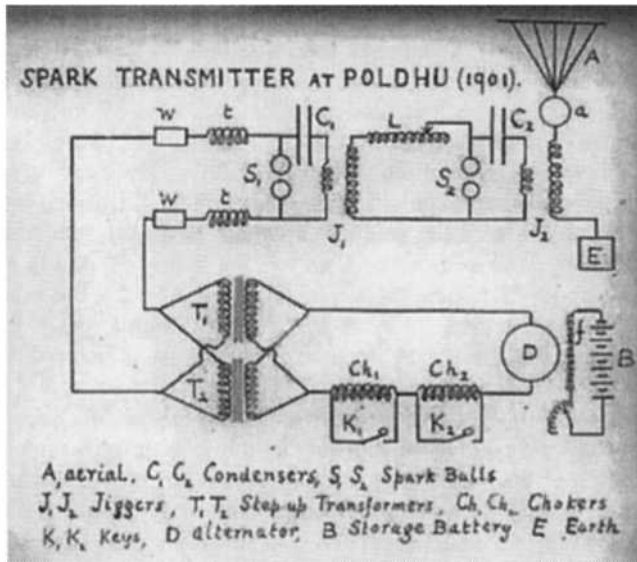
Figure 10.3. Circuitry used in Poldhu, 1901.
