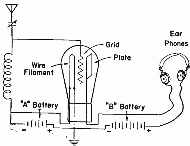
A TUBE USED TO AMPLIFY RADIO SIGNALS
