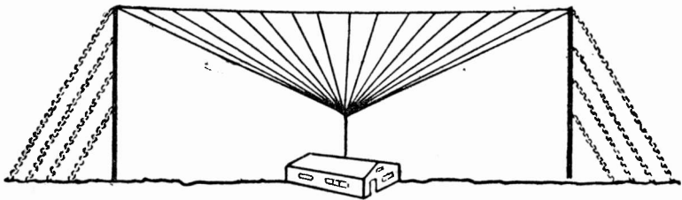
SUBSTITUTE AERIAL AT POLDHU
