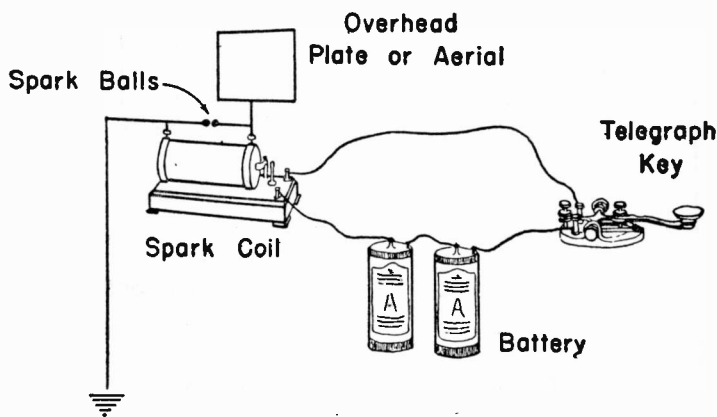
MARCONI'S EARLY TRANSMITTER
