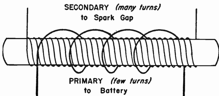
INDUCTION COIL
