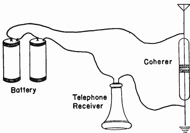
CIRCUIT USED TO DETECT THE HISTORIC "S" AT NEWFOUNDLAND
