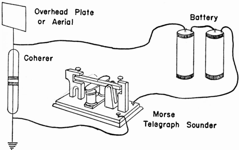
MARCONI'S EARLY RECEIVER
