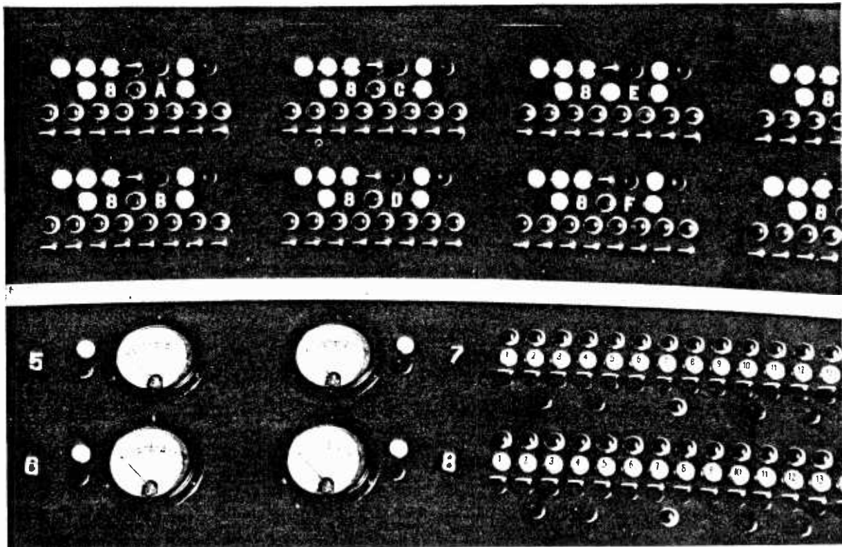
Figure 28. A closeup view of part of the left end of the master control desk. The two rows of 14 keys at the lower right are switchbanks 7 and 8 for selecting channels 1 to 14. Volume indicator meters for these switchbanks are immediately to the left. The groups of 8 keys above are switchbank selectors allowing any one of the switchbanks to be assigned to any studio.
