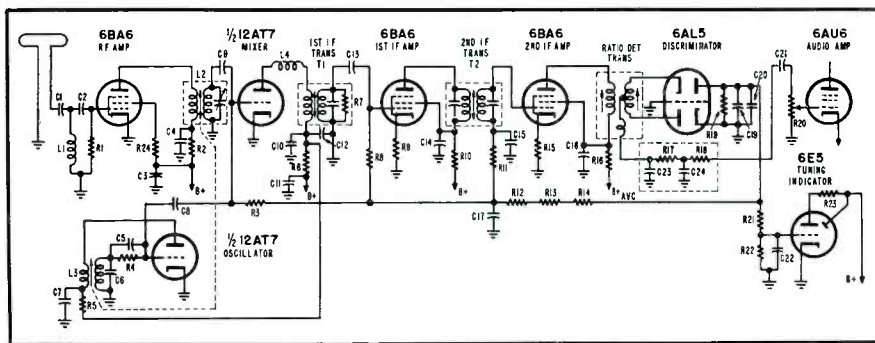
FIG. 1: CIRCUIT of FM section of AM-FM tuner used in Westinghouse chassis.
