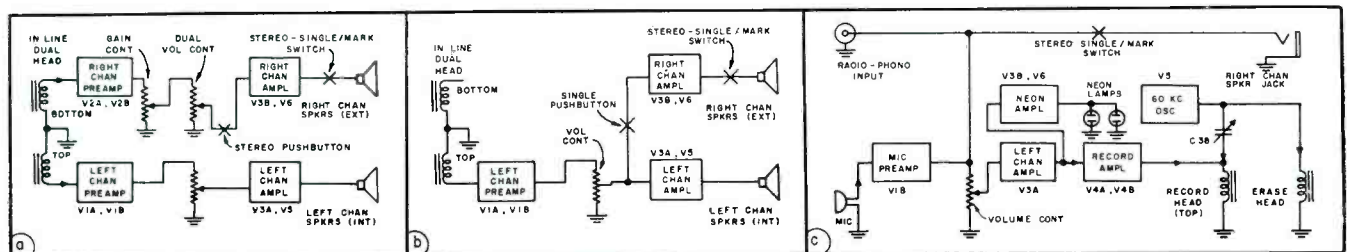
FIGS. 3, 4 and 5: BLOCK DIAGRAMS of stereo playback and monaural record-playback systems used in RCA STR-6/8 tape machines.
