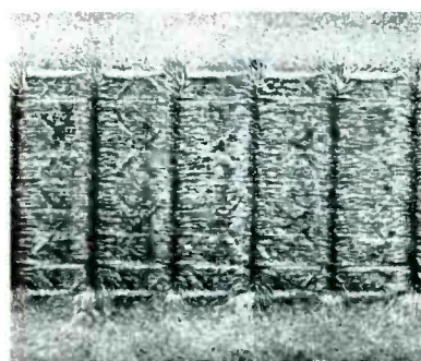
PHOTOMICROGRAPH showing lineup of iron-oxide particles in magnetic field. This is an actual section of magnetic recording tape with a signal on it made visible by a special process.
