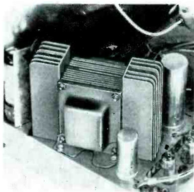
FIG. 3: PRESENT MOUNTING on a horizontal chassis where short brackets are used and the fins protrude through holes in the chassis to take advantage of the cooler air available from openings in the cabinet bottom.
