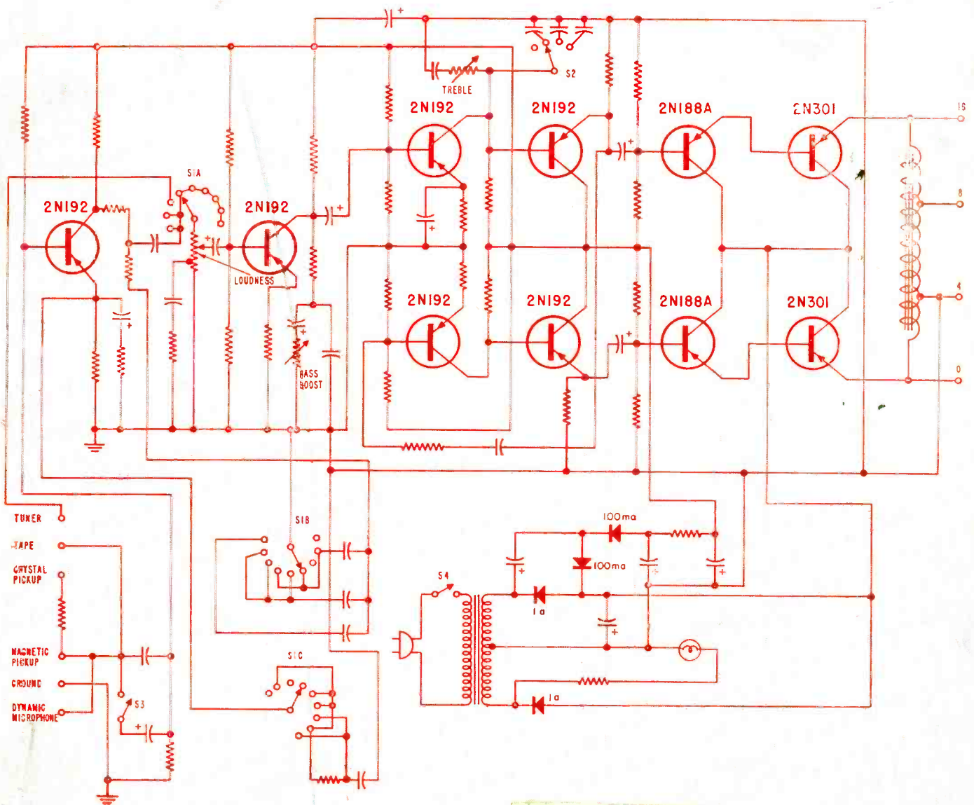
Ten-transistor audio amplifier with inputs for tuner, tape, magnetic or crystal pickups and dynamic microphone, which can deliver 20 watts to speaker load.
