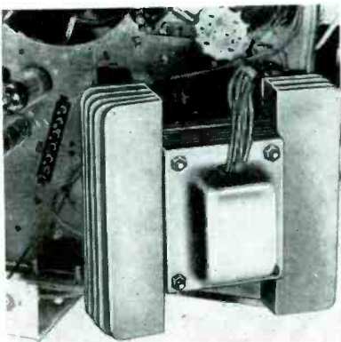
FIG. 1: VERTICAL CHASSIS mounting of recently-designed fin-cooled power transformer which simplifies chassis layout and removes heat problems.
