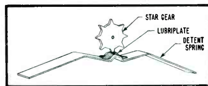
FIG. 2: POINT of lubrication in tuner detent spring. Both sides of the point of contact on the detent spring, as well as the point of contact, should be well lubricated.
