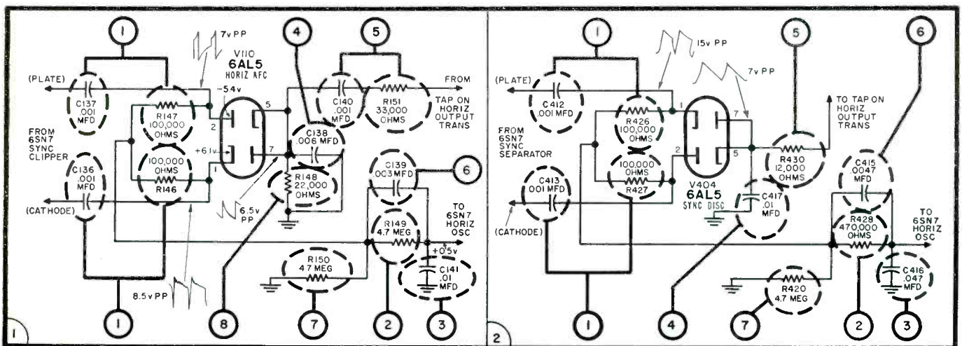
FIGS. 1-2: The Fig. 1 diagram is the horizontal-sync circuit used in the Crosley 393-394. Fig. 2 is the horizontal-sync circuit used in the Admiral 22E2 chassis.
