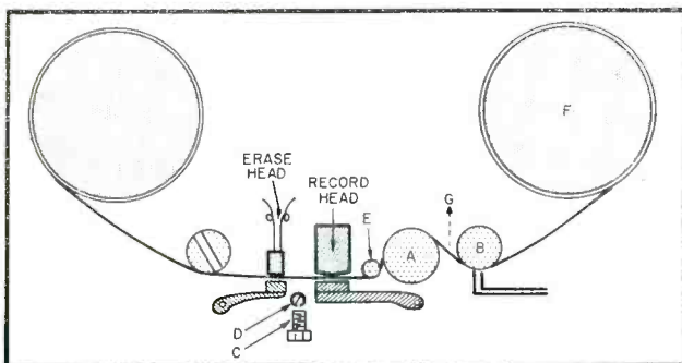
TAPE COMPONENTS in Ampro equipment which require adjustments to cure pinch rollersqueek: A—pinch roller, B—guide, C—set screw, D—adjusting cam screw, E—capstan, and F—takeup reel. G represents direction tape should be pushed.
