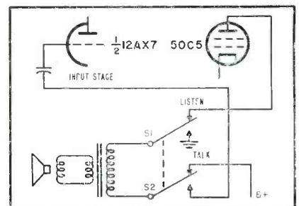
FIG. 3: SWITCHING system in an intercom where speaker functions as a listening and transmitting device.
