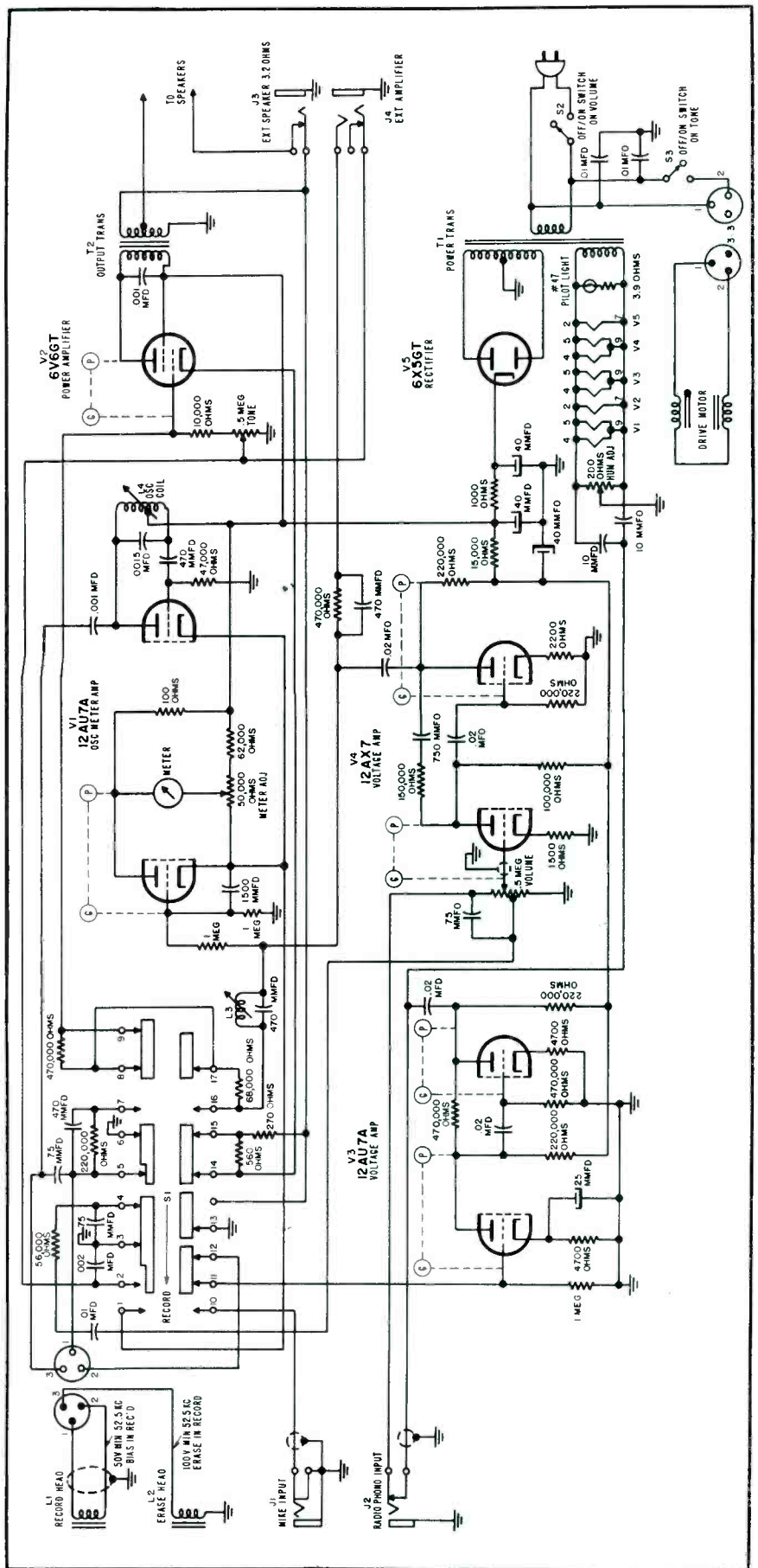
SCHEMATIC of amplifier used in Crescent tape recorder models TR-773, 773A, 773B, 774, 774A and B.
