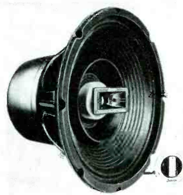
COAXIAL THREE-ELEMENT speaker available in both 12" and 15" sizes. In these units, a dual diaphragm affords lf and mid-range performance, while a compression driver supertweeter covers the higher frequency range.—Type CX; Jensen Mfg. Co., 6601 S. Laramie Ave., Chicago 38, Ill. [SERVICE].
