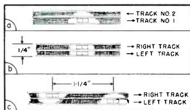
STEREOPHONIC SOUND showing the difference in head arrangement of (a) dual track monaural recording, (b) stereo or binaural recording (in-line heads), (c) stereo or binaural recording (staggered heads).
