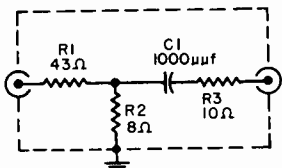
FIG. 4 I-F INJECTION NETWORK
