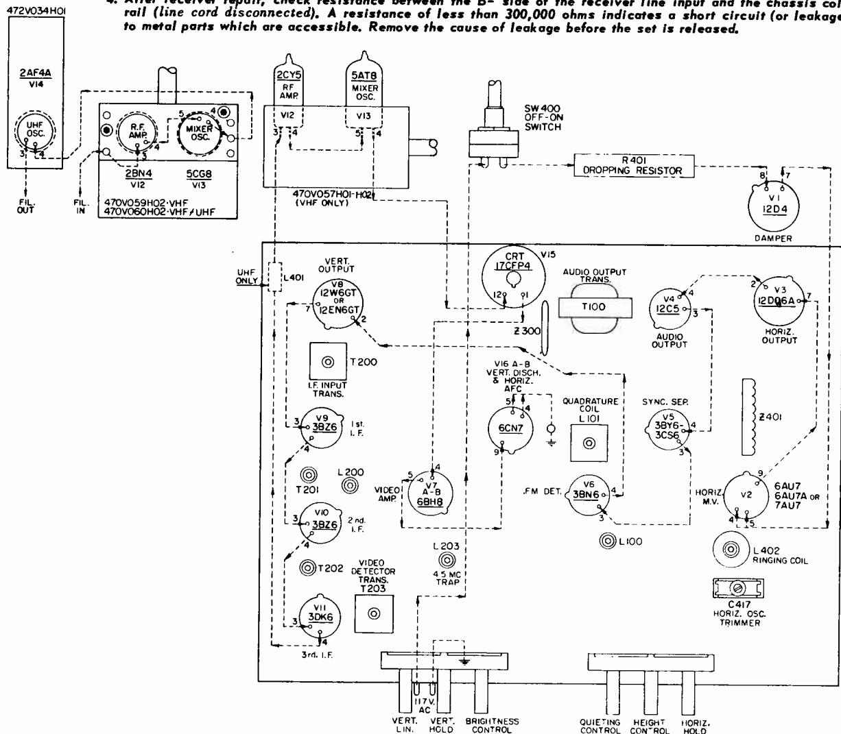
Figure 4. Top view of chassis. Tube location, heater string, and adjustments.
