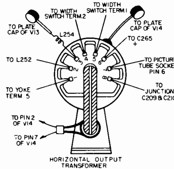
HIGH VOLTAGE TRANSFORMER WIRING
