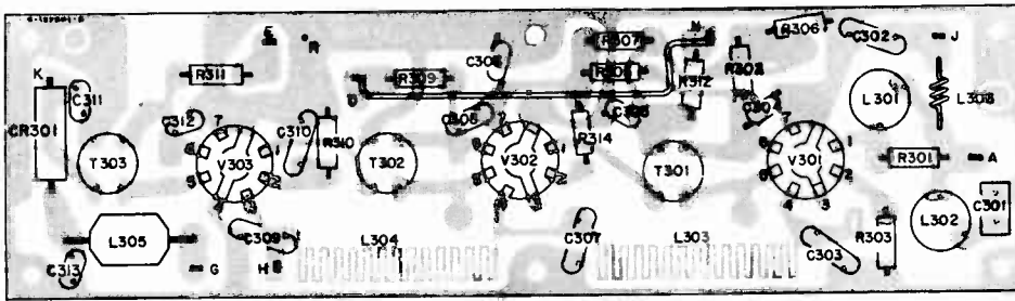
Figure 24—PW300 Picture I-F Circuit Layout
