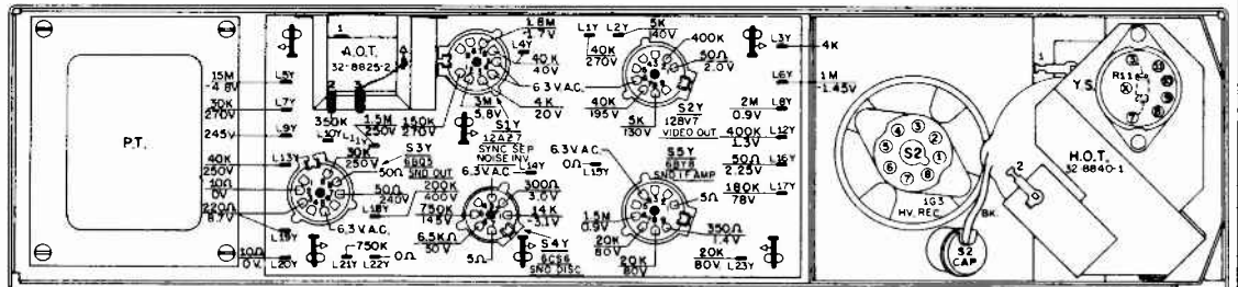
Chassis Layout Showing Voltage and Resistance Readings
