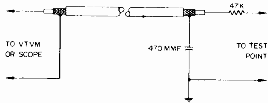
Figure 11. Decoupling network.
