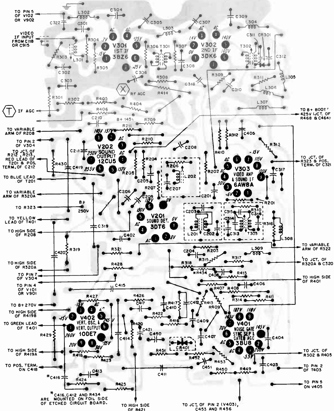
Figure 17. View of Wiring Side of Etched Circuit Board A7265-1. Gray Area Represents Etched Wiring; Black Symbols and Lines Represent Components and Connections on Opposite Side.
