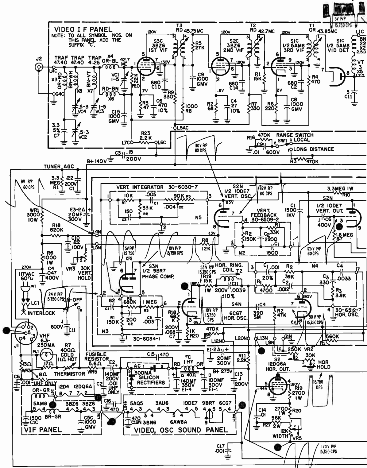
Schematic Diagram for Chassis 9L38 and 9L38U, Run 3
