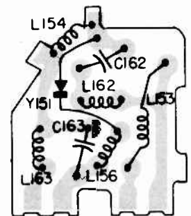
VIDEO DETECTOR BD. COMPONENT LOCATION AS VIEWED FROM COMPONENT SIDE.
