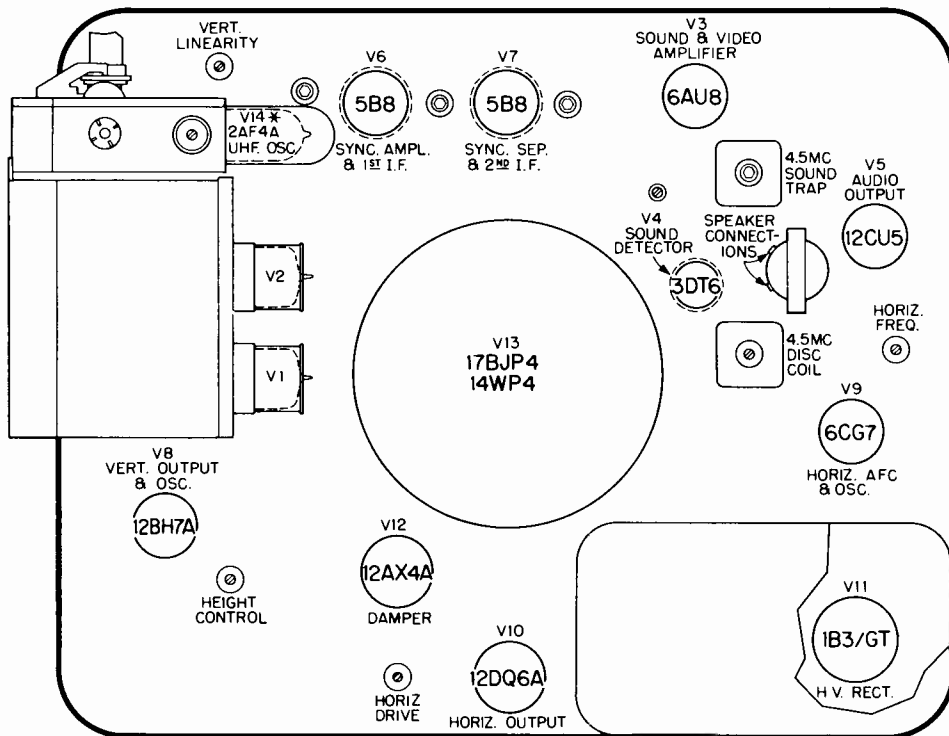
TUBE LAYOUT
