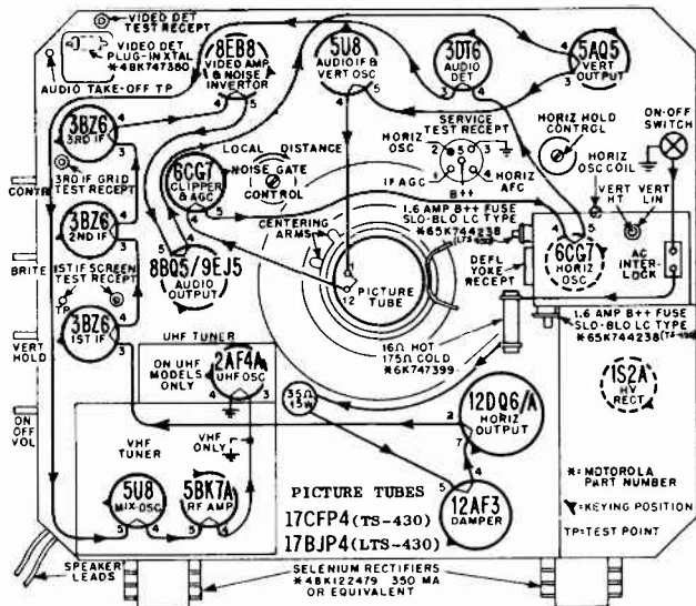
FIGURE 1. TUBE LOCATIONS & FILAMENT WIRING
