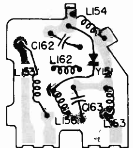
VIDEO DETECTOR BD. COMPONENT LOCATION AS VIEWED FROM CONDUCTOR SIDE.
