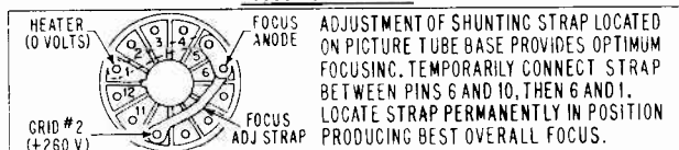
FIGURE 2. FOCUS STRAP ILLUSTRATION
