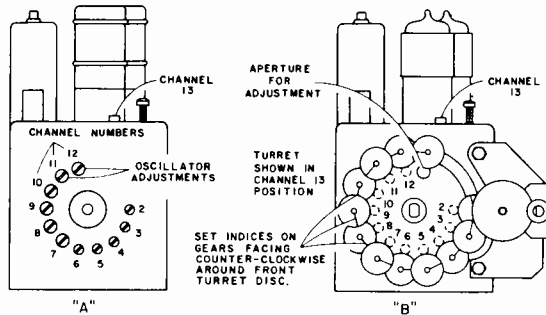
Figure 4—VHF Oscillator Adjustments
