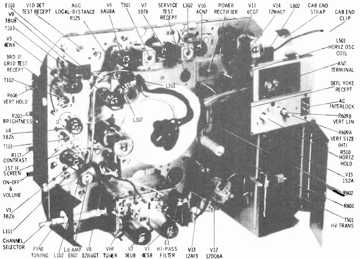
FIGURE 9. PARTS LOCATIONS
