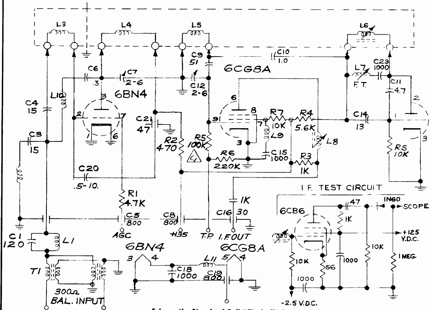
Schematic, Standard Coil "Fireball" Tuner
