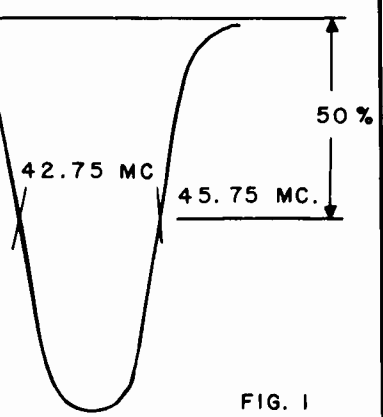
OVERALL I.F. RESPONSE CURVE
