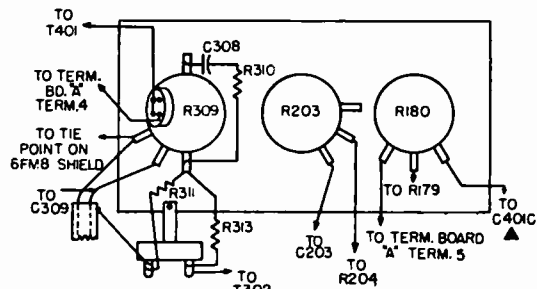
REAR VIEW 21" CONTROL PANEL WIRING
