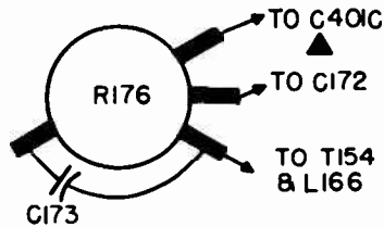
21" CONTRAST CONTROL WIRING - REAR VIEW
