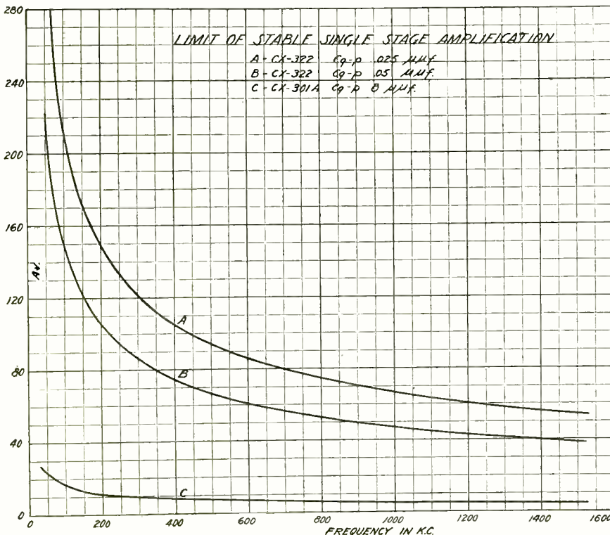
Fig. 3. Limits of Stable Amplification with Single Stage
