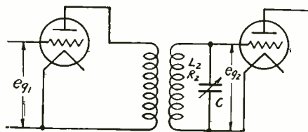
Fig. 1. Transformer-Coupled R.F. Amplifier Circuit
