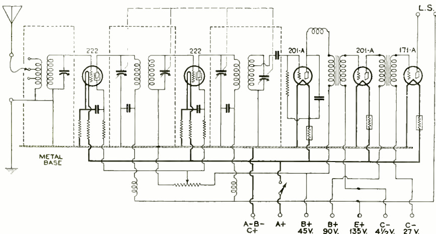
Circuit Diagram of Hammarlund-Roberts "Hi-Q 29"
