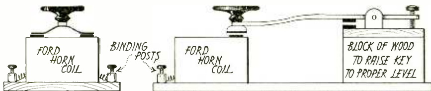
Fig. 1. Constructional Details of the Ford Horn Relay
