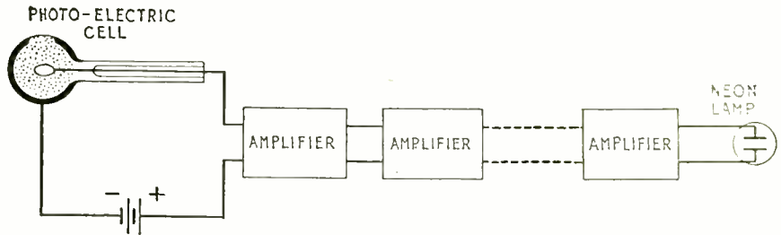
Fig. 3. Position of Amplifiers in Television Circuit
