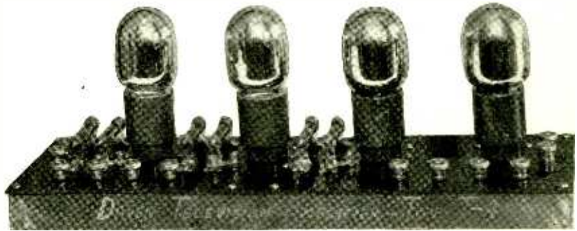
Fig. 4. Commercial Four-Stage Resistance-Coupled Amplifier of Received Television Signals
