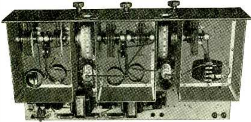
Top View of Hammarlund-Roberts "Hi-Q 29"
