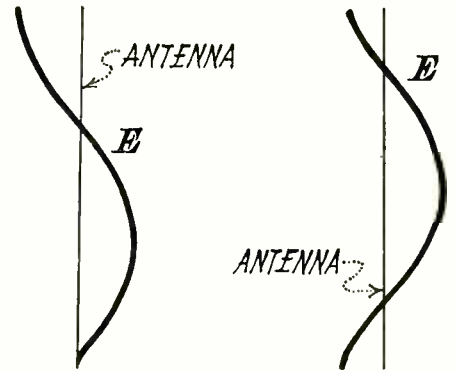
Fig. 2. Distribution in \frac{3}{4} Wavelength Antenna
