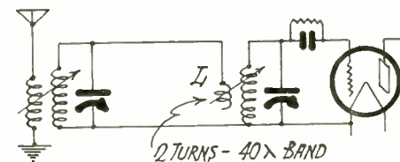
Fig. 5. More Selective Antenna-Coupling Circuit
