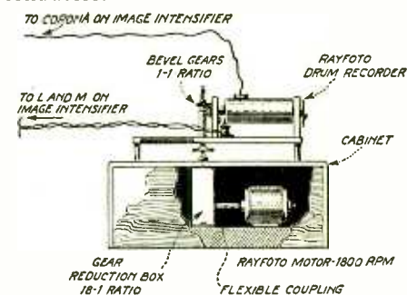
Fig. 3. Mechanical Printer Unit
