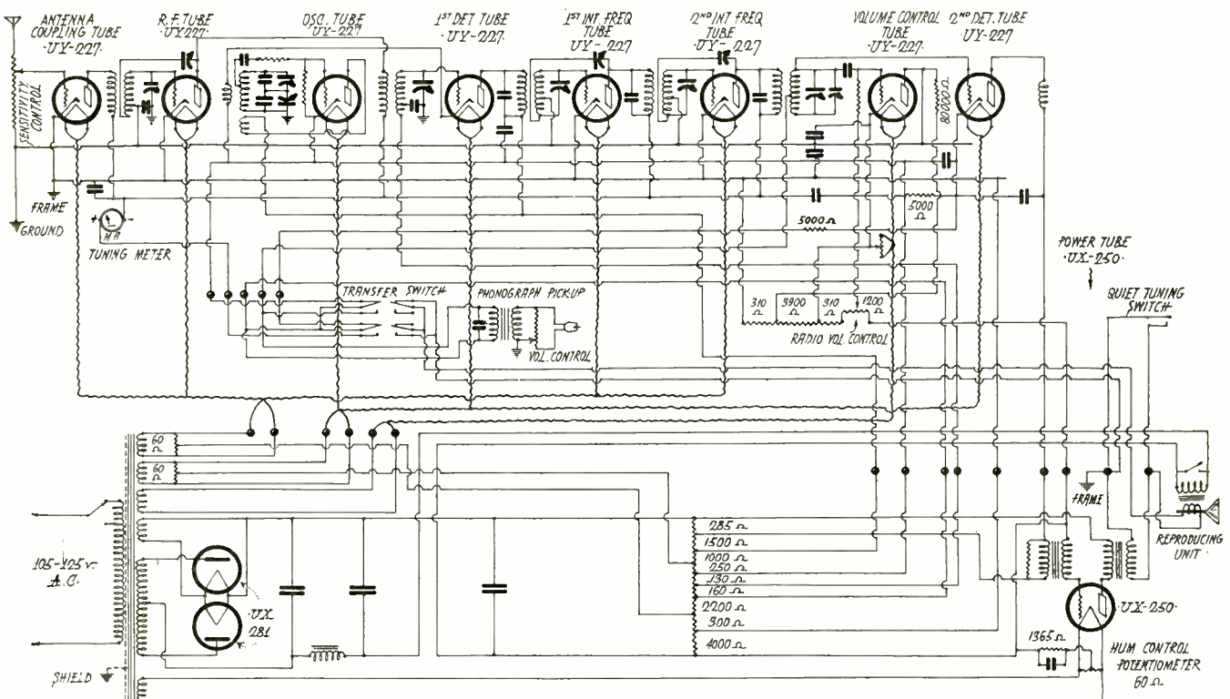
Fig. 2. Circuit Diagram of Radiola 64
