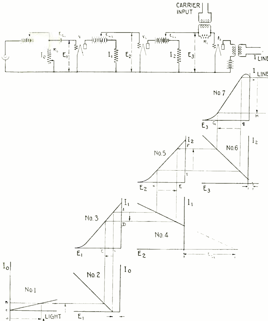
Fig. 1. Circuit Diagram and Characteristics of Amplifier-Modulator for Still-Picture Transmission
