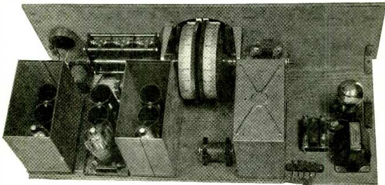
Rear View of Five-Tube A.C. Screen-Grid Receiver
