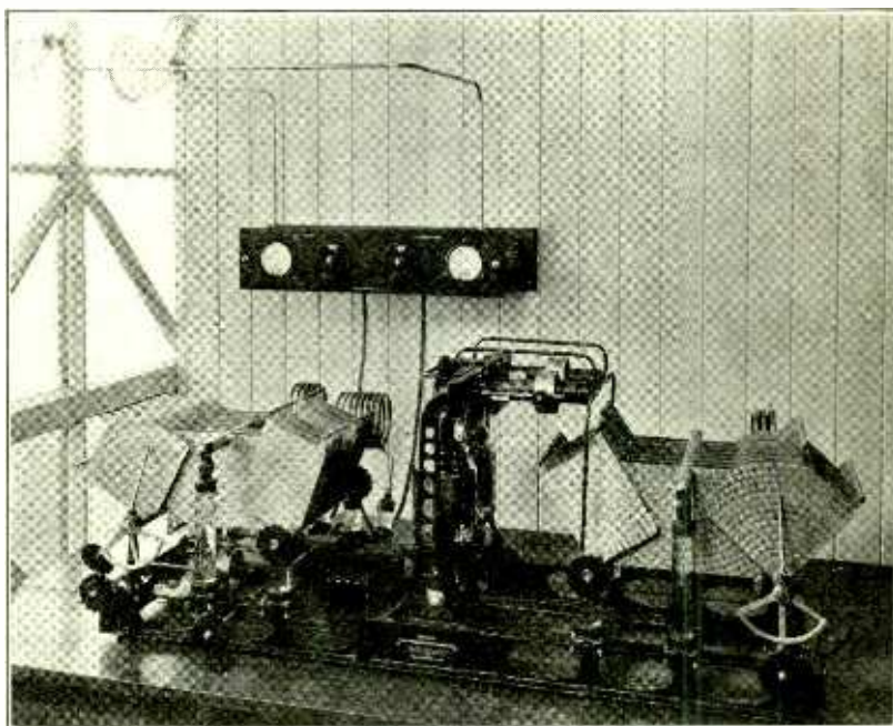
500-Watt, 32.4 Meter Transmitter at Control Station KRG
