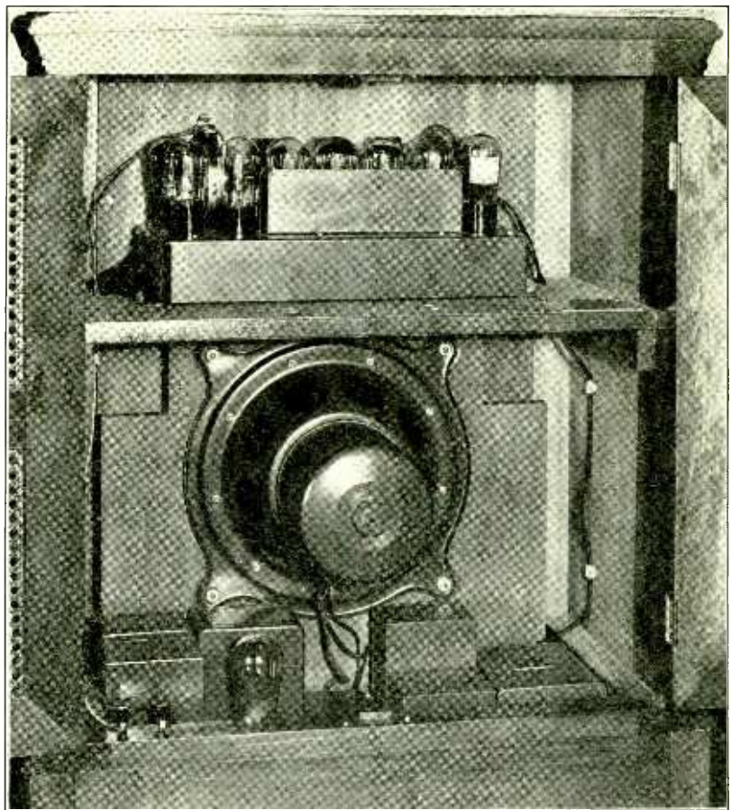
Rear View of Radiola 62
