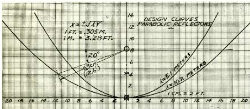
Fig. 1. Design Curves for Parabolic Reflectors
