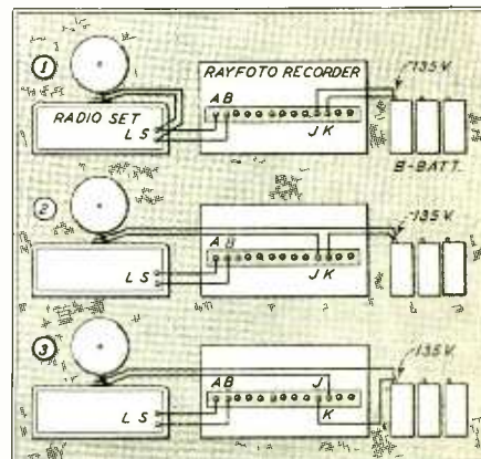
Fig. 4. Test Connections
