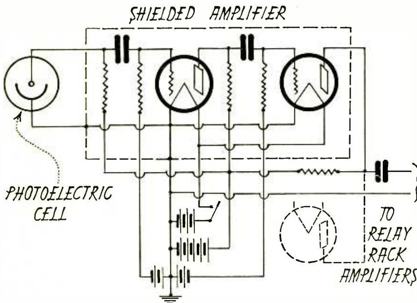
Fig. 2. Preliminary Stages of Television Amplifier Circuit
