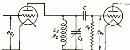
Fig. 2. Impedance-Coupled R.F. Amplifier Circuit
