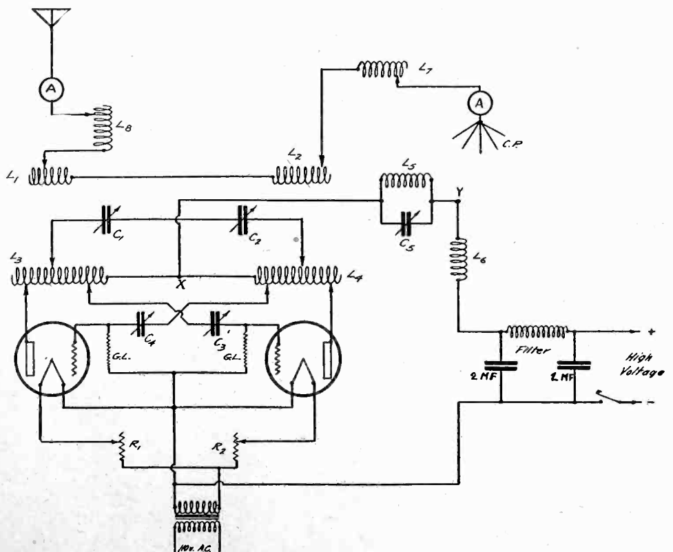
Fig. 1. Schematic Diagram of Push-Pull Radio Frequency Oscillator.
