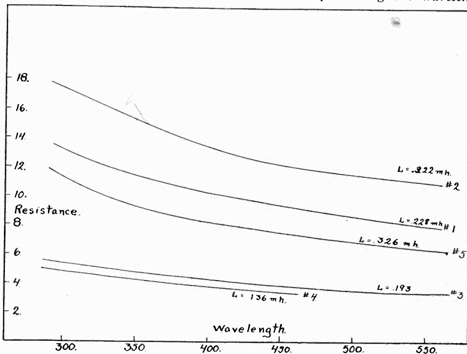
Fig. 1. Variation of Radio Frequency Resistance with Wavelength for Five Coils.
