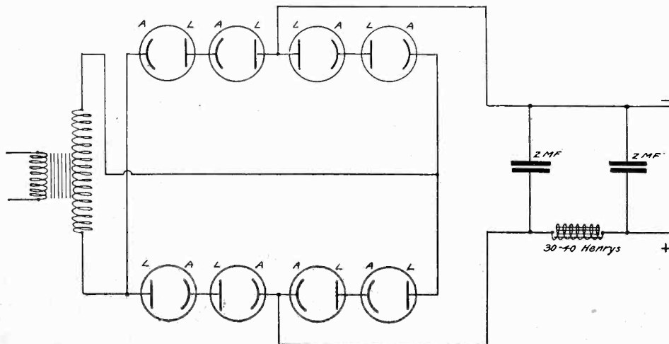
Fig. 1. Bridge Method of Connecting Rectifier Jars.
