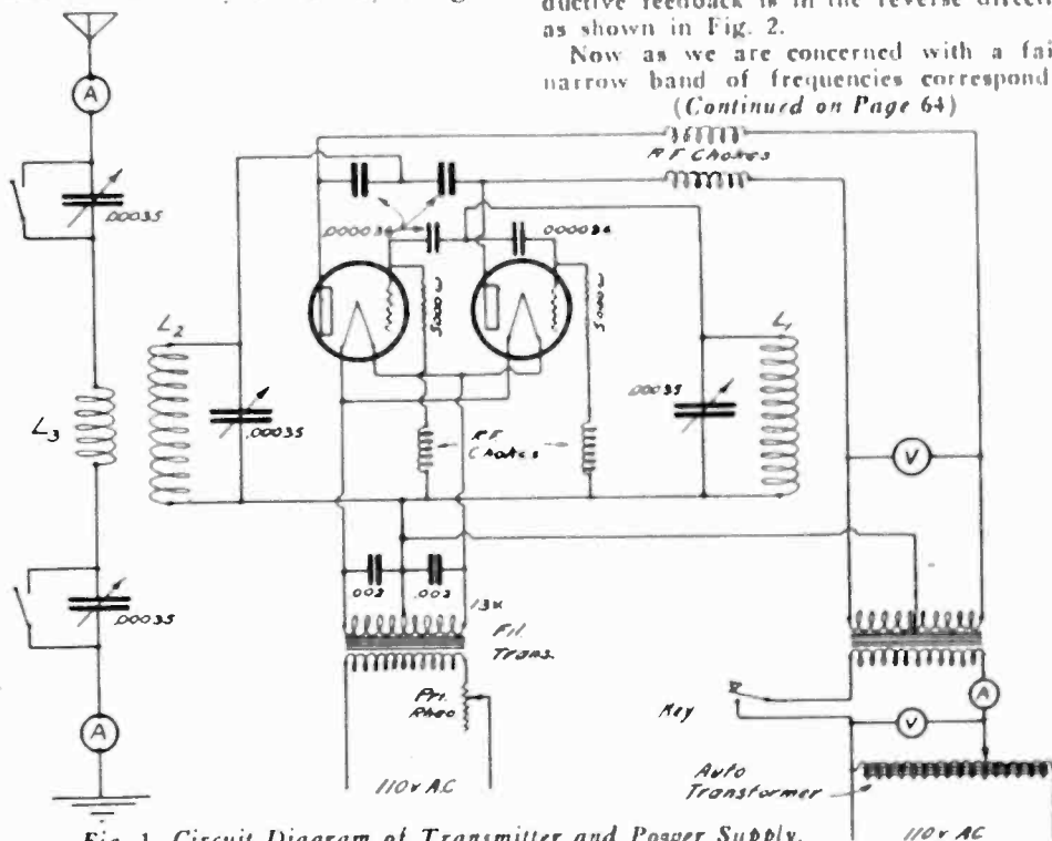
Fig. 1. Circuit Diagram of Transmitter and Power Supply.
