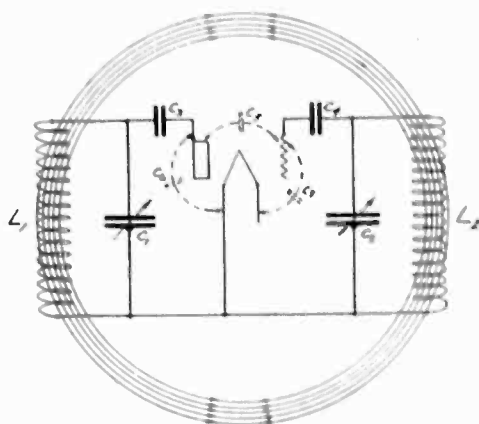
Fig. 2. Theoretical Circuit of Oscillation.
