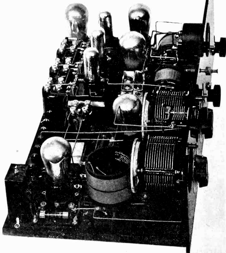
End View of Receiver, Showing Oscillator System.
