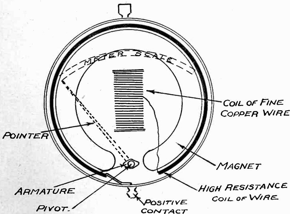
Fig. 1. Polarized Vane Type of Meter.
