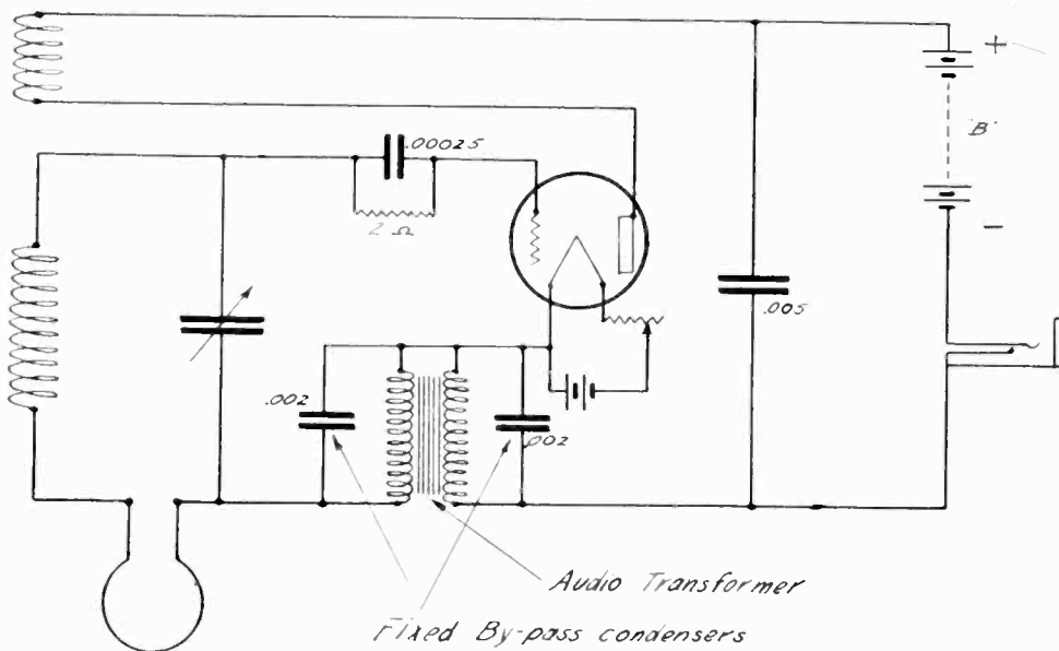
Fig. 3. Modulated Heterodyne Wavemeter.
