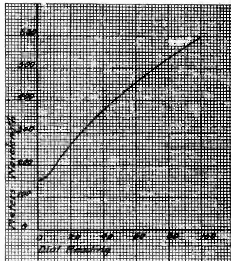
Fig. 5. Typical Calibration Curve of Wavemeter.
