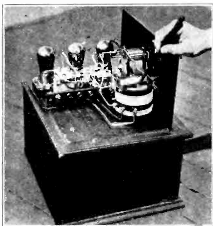
Fig. 2. Internal construction of 40-150 meter receiver.
