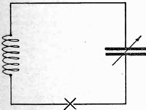
Fig. 1. Simple Wavemeter Circuit.
