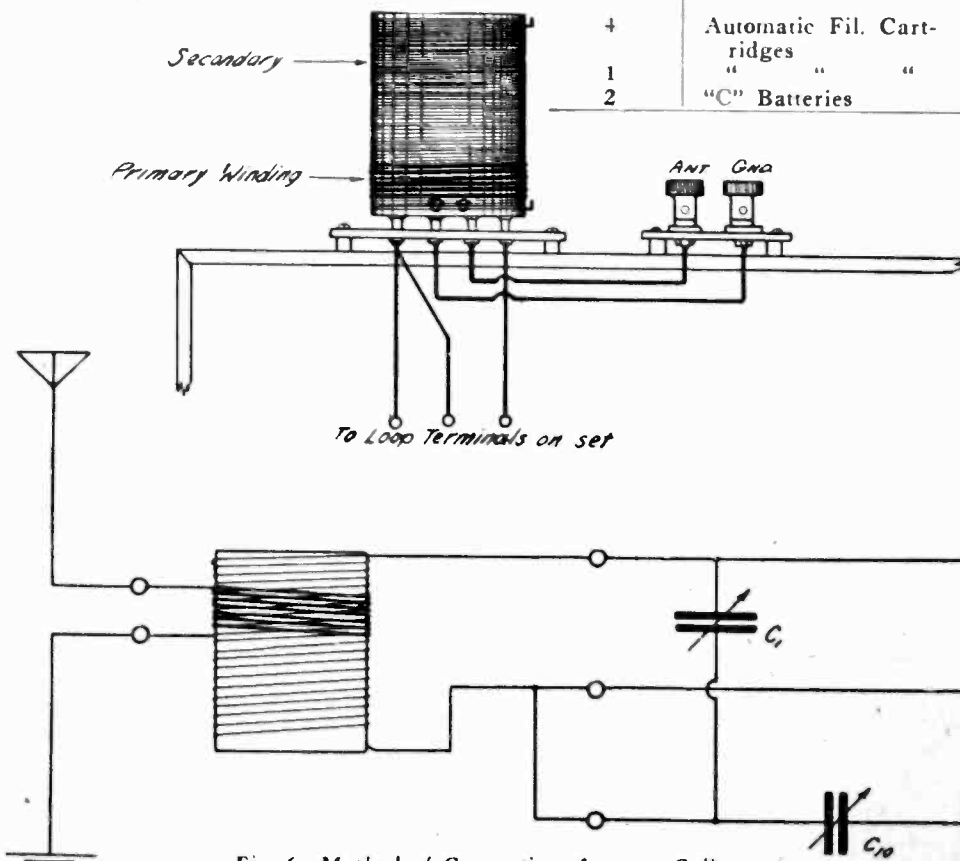
Fig. 6. Method of Connecting Antenna Coils.
