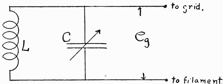
Fig. 4. Typical Tuned Circuit.
