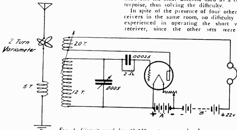
Fig. 1. Circuit used for 40-150 meter wave band.
