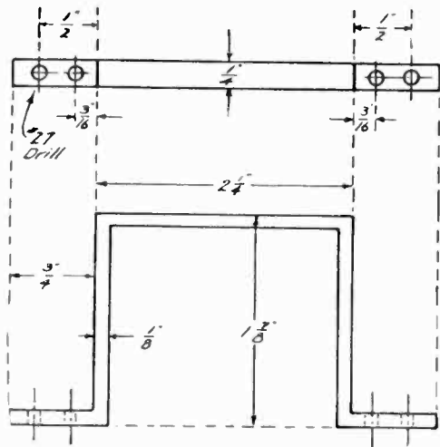
Fig. 5. Details of Brackets for Shelf.
