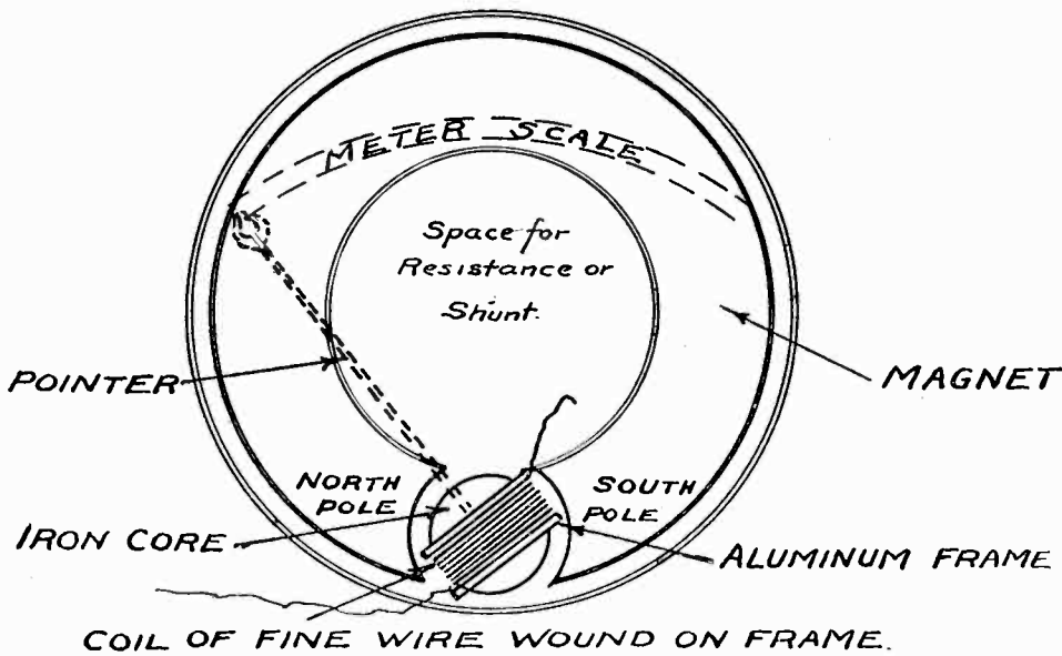
Fig. 3. Moving Coil Type of Meter.
