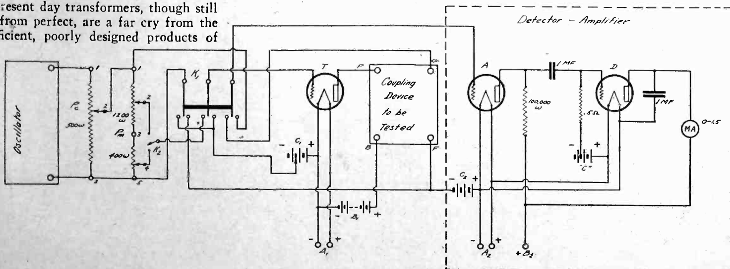
Fig. 1. Circuit Used in Audio Frequency Tests.
