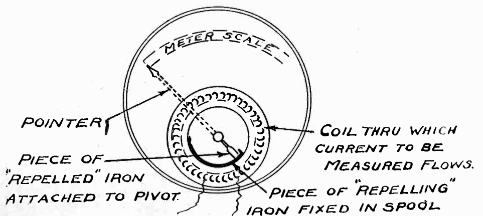
Fig. 2. Repulsion Type of Meter.
