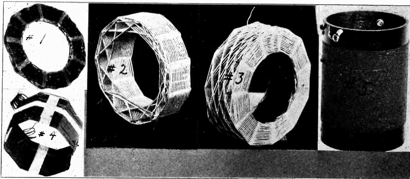
Fig. 2. The Five Coils Tested.
