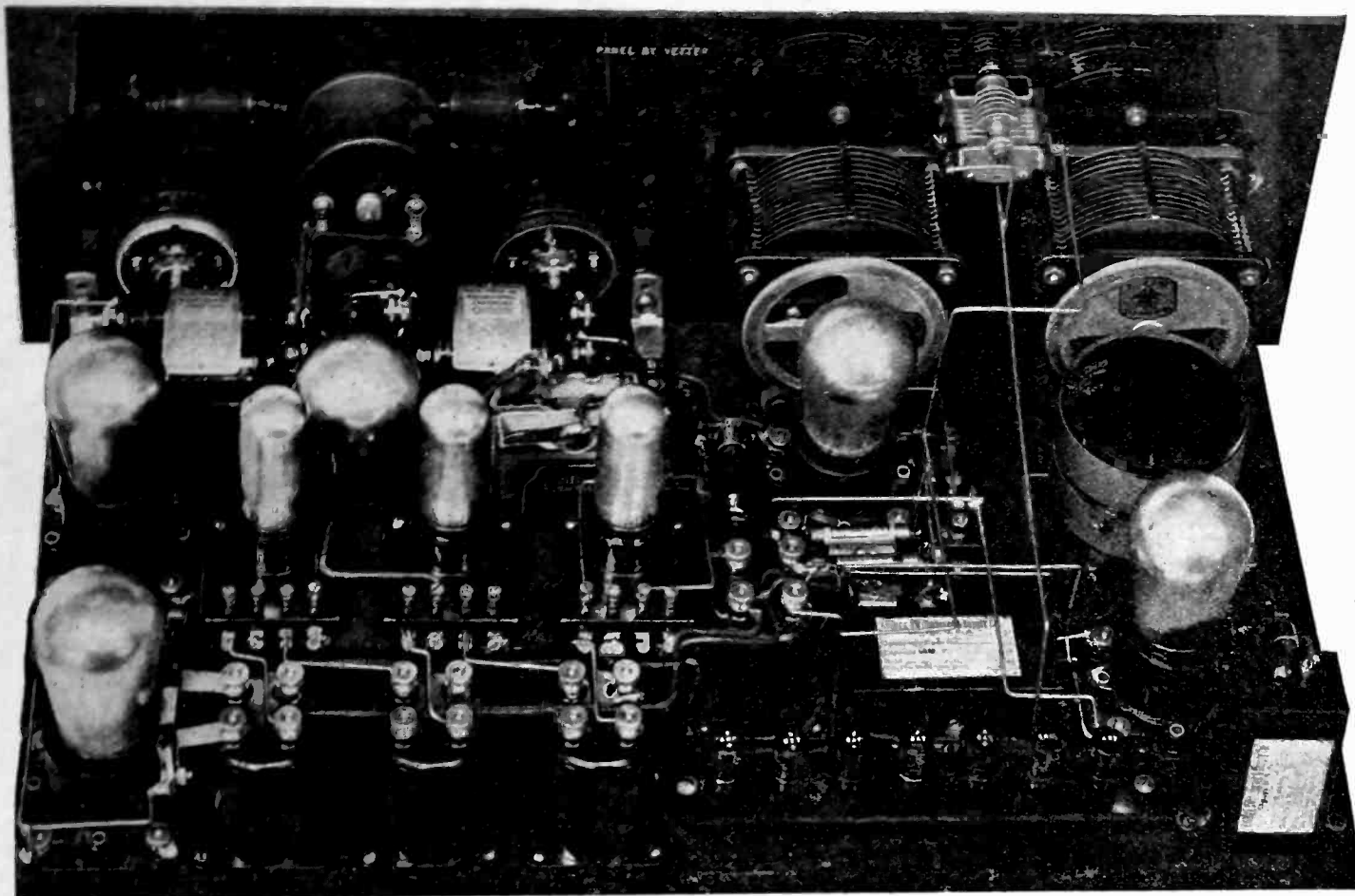
Rear View of Baseboard Model.
