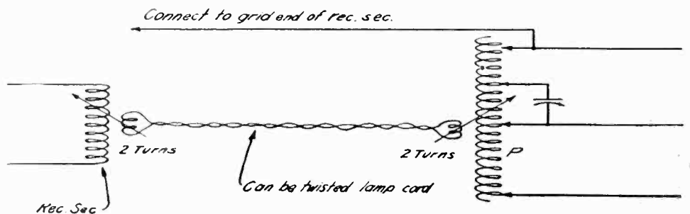
Fig. 2. Method of coupling transmitter to receiver.
