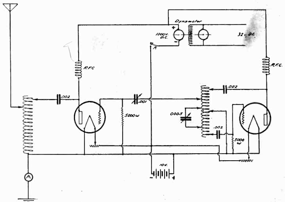
Fig. 1. Transmitter circuit for "IDALIA."
