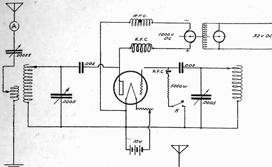
Fig. 2. Circuit of transmitter of "ELOISE."
