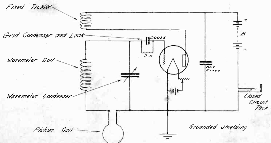
Fig. 2. Heterodyne Wavemeter Circuit.
