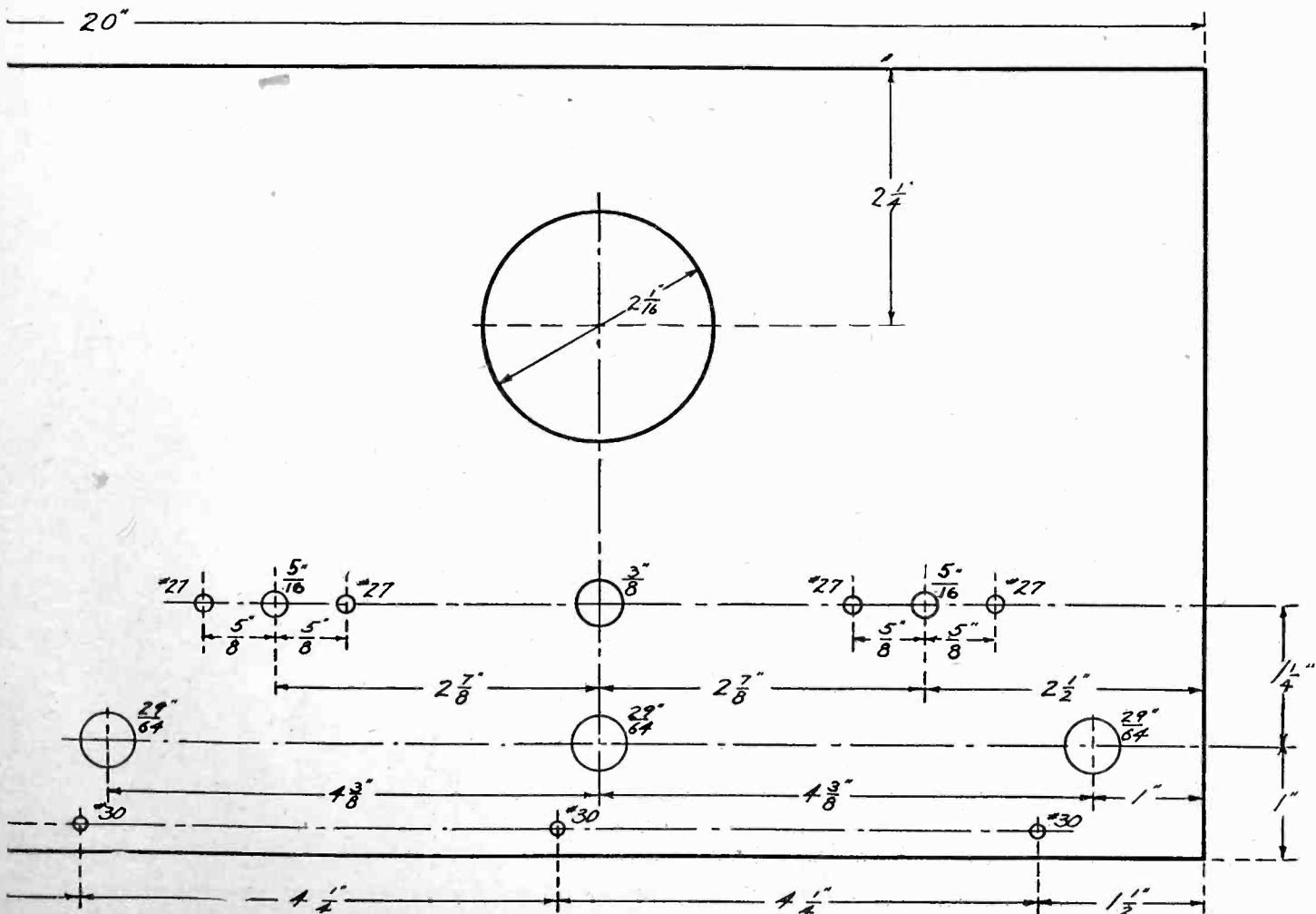
Fig. 2. Template for Drilling Panel.
