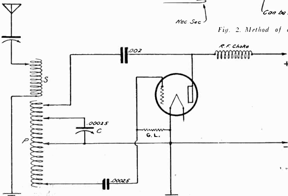
Fig. 1 Hartley circuit arranged for transmitting.
