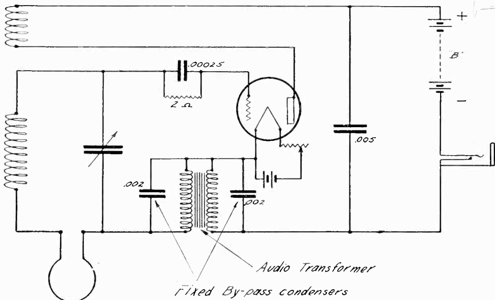
Fig. 3. Modulated Heterodyne Wavemeter.
