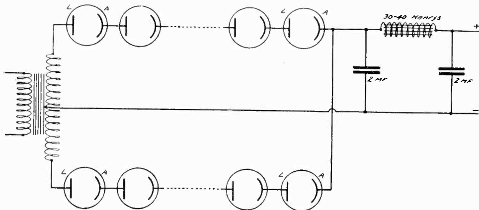
Fig. 2. Center Tap Method of Rectification.
