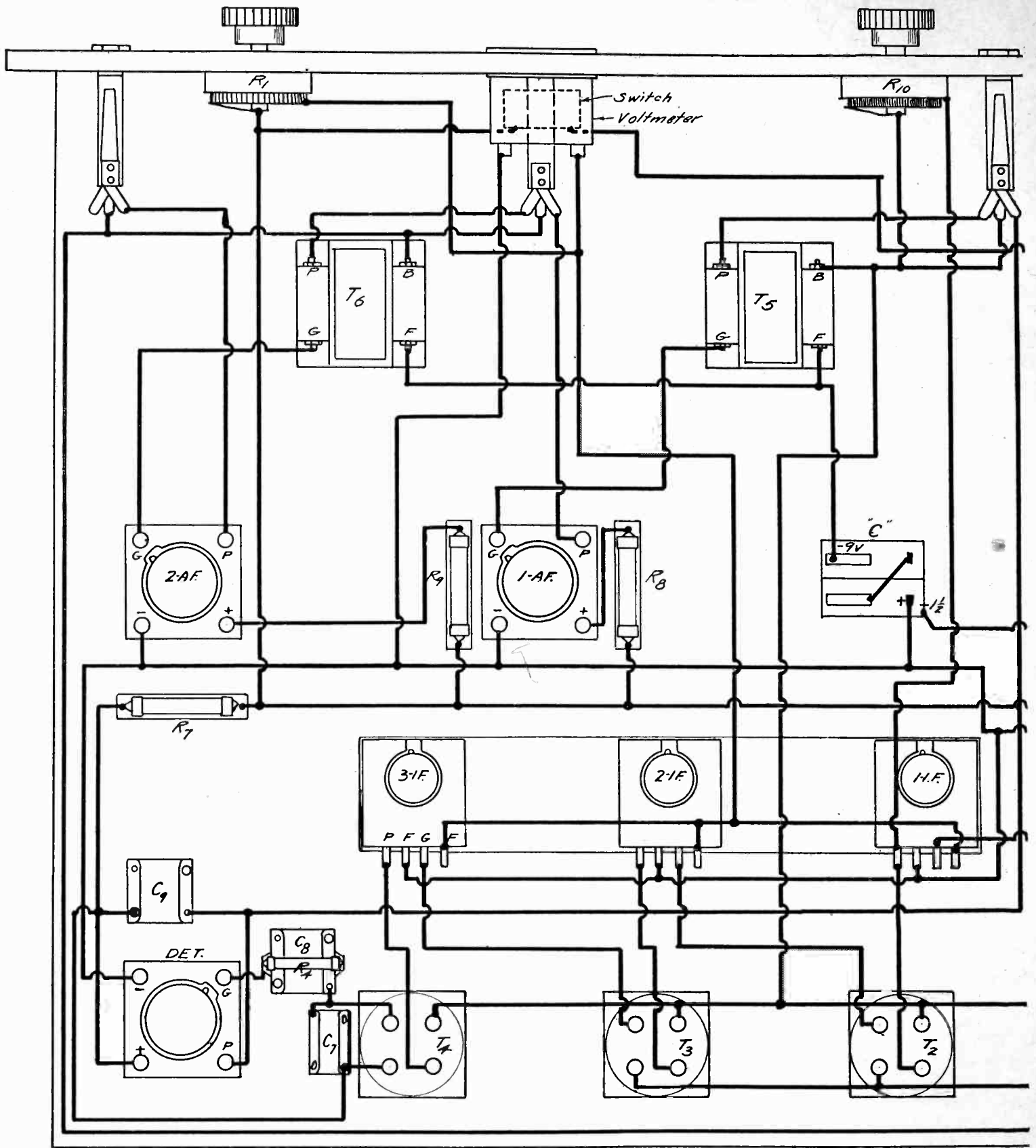
Fig. 4. Pictorial Wiring Diagram, Showing
