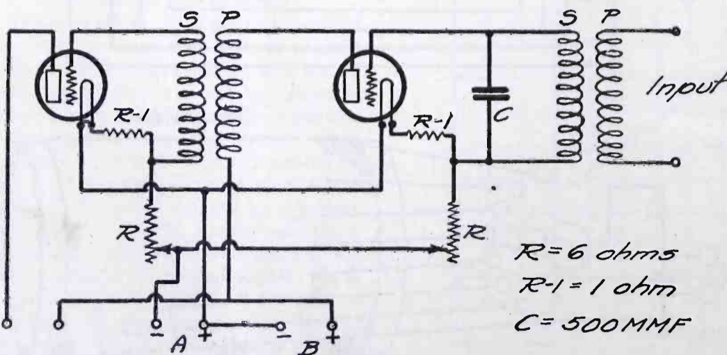
Fig. 2. Two-Step Amplifier Hook-up
