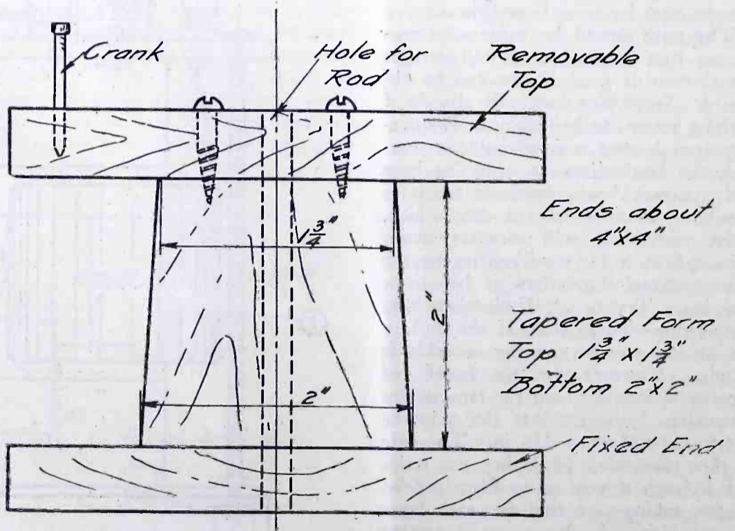
Fig. 6. Form for Winding Coils
