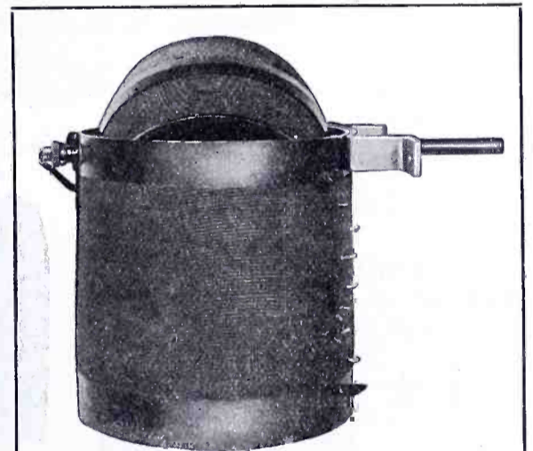
Catalogue No. 167.....$5.50 SE-AR-DE VARIO COUPLER (Bracket Type)
