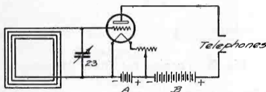
Fig. 5. The Simplest Tube Circuit, Which Receives Without Coils or Aerial
