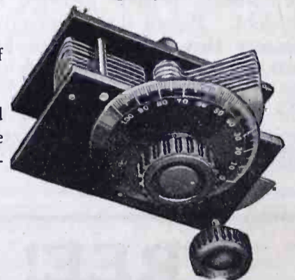
TYPE 17 and 31 P. C. S. CONDENSERS WITH VERNIERS ATTACHED
