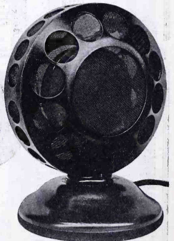
Fig 85. Capacitative Transmitter Microphone
