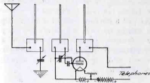
Fig. 2. Three Spiderwebs with Detector Tube
