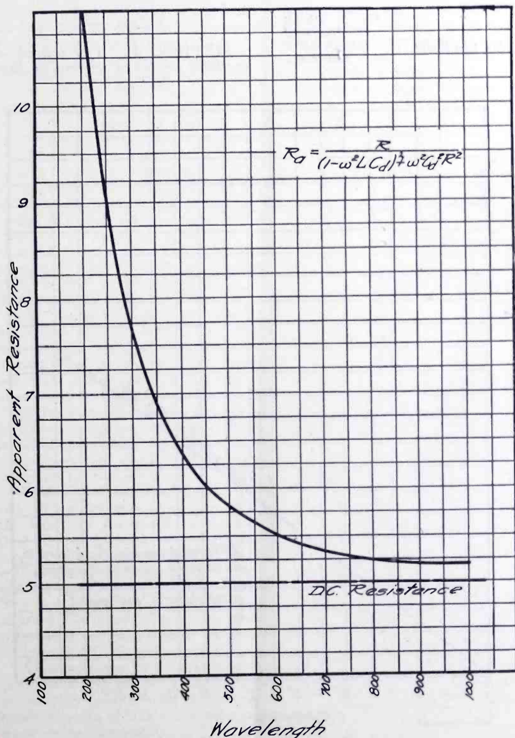
Fig. 4. Variation of Apparent Resistance with Frequency Because of Distributed Capacity
