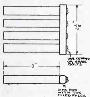
Fig. 1. Positive Electrode Made from Four Carbons from Old Dry Cell.
