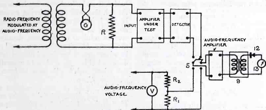
Fig. 2. Simplified Diagram of Circuits for Measurement of Voltage Amplification of Radio Frequency Amplifier
