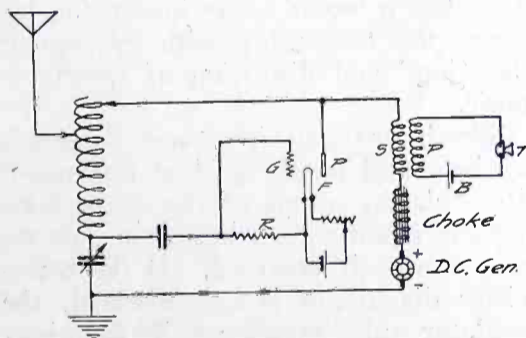
Fig. 81. Simple Form of Modulation Circuit
