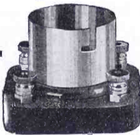
KING QUALITY VACUUM TUBE SOCKET Base of black or mahogany finished genuine moulded Bakelite with mirror finish; tube and terminal binding posts of brass, nickel plated and highly polished.
