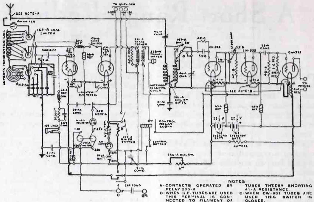
Fig. 2. Receiver Circuit.
