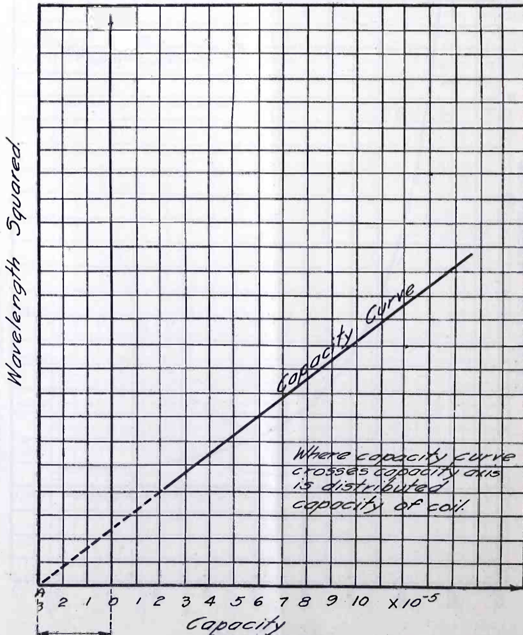
Fig. 8. Plot for Determining Distributed Capacity
