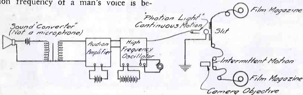
Fig. 1. Sound Recording System
