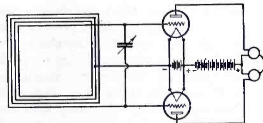
Fig. 7. Push-pull Circuits without Transformers
