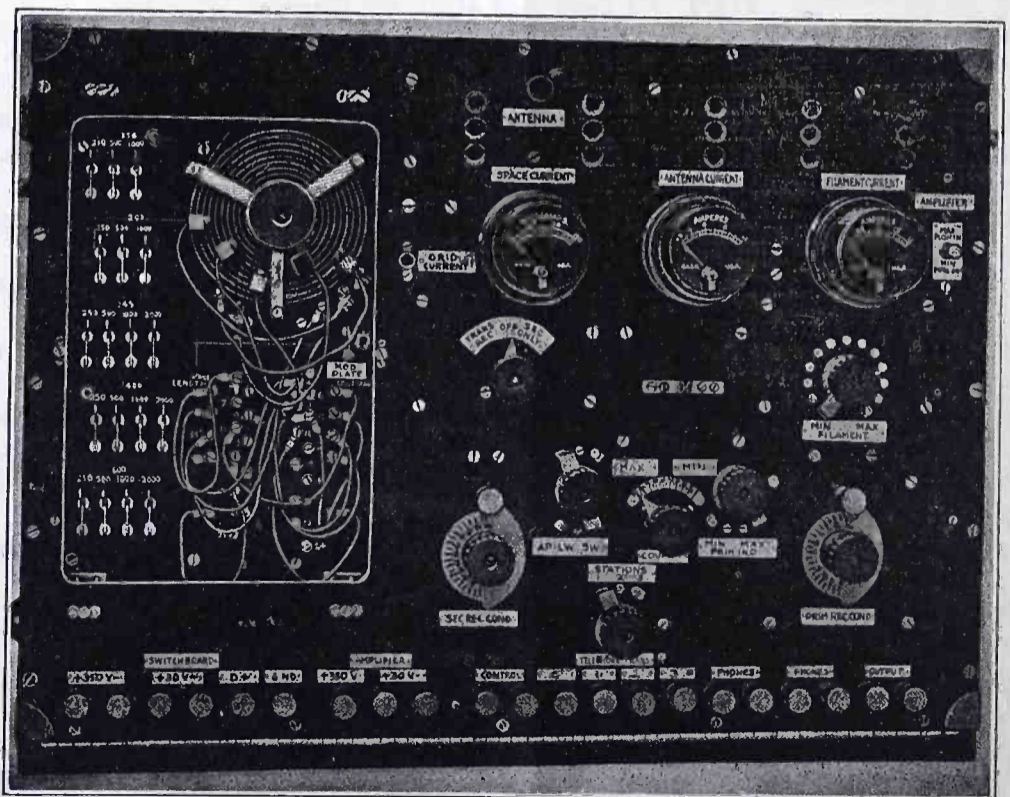
Fig. 4. Transmitter-Receiver Unit
