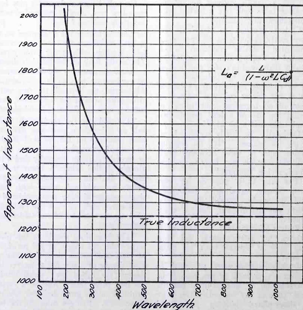
Fig. 3. Variation of Apparent Inductance with Frequency Because of Distributed Capacity
