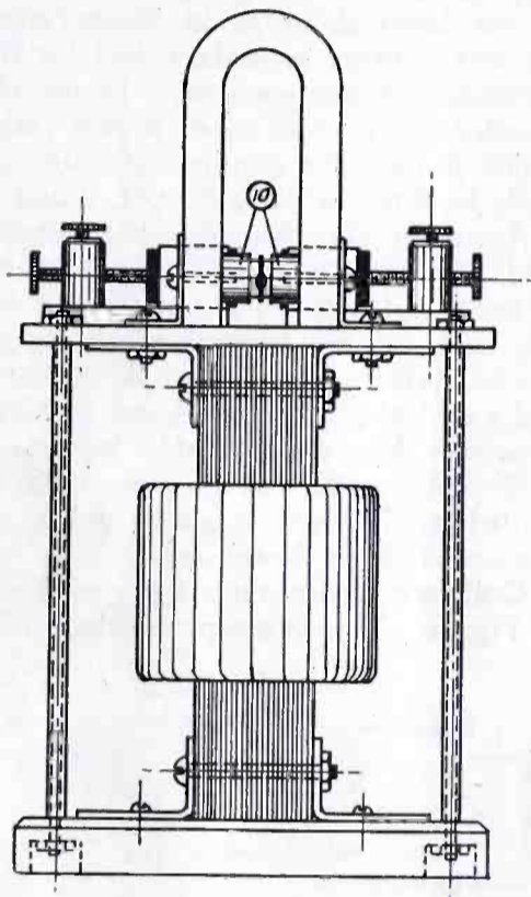
Fig. 3. End View
