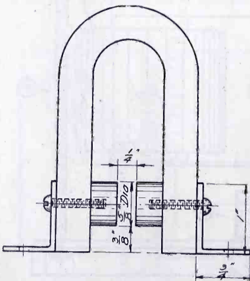
Fig. 4. Magnet Detail
