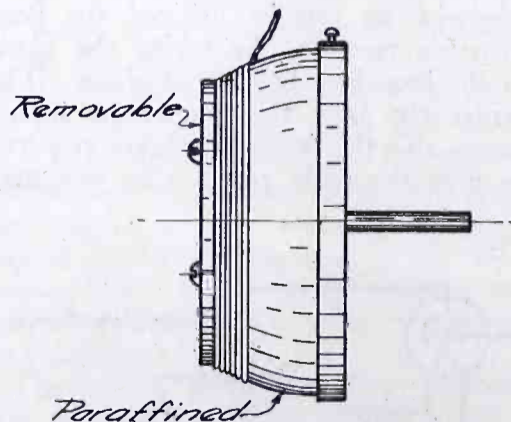
Fig. 10. Winding the Stator Coil
