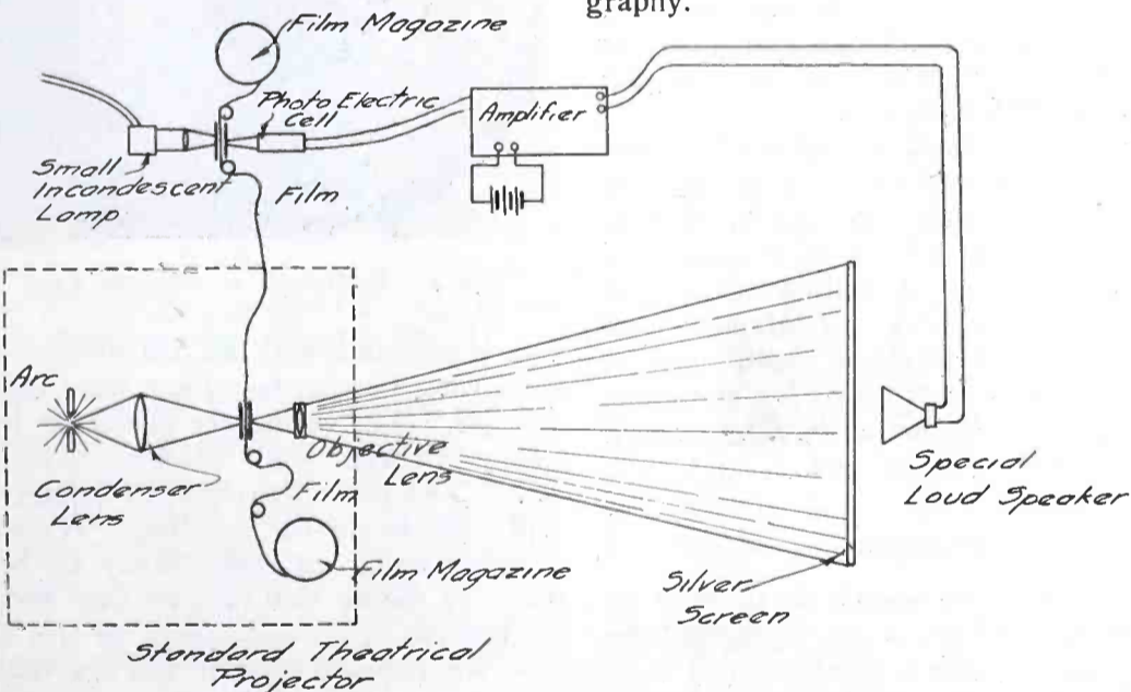
Fig. 3. Method of Synchronizing Sound and Motion Photography
