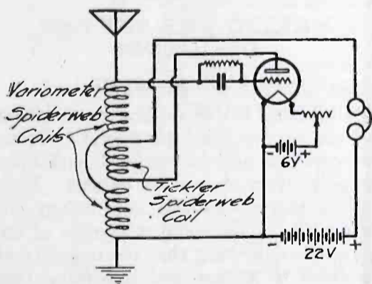
Fig. 3. Regenerative Circuit with Variometer Made of Two Spiderwebs
