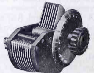
TYPE 17 P. C. ROUND CONDENSER Capacity, .0005 Mfd.
