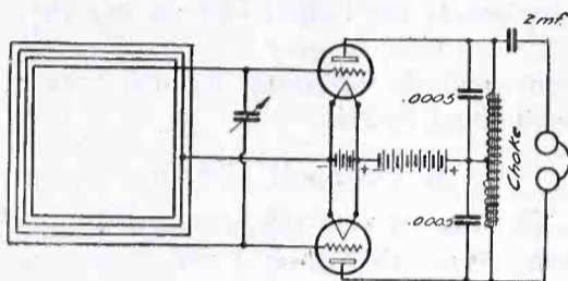
Fig. 8. Push-pull Circuit without Transformers
