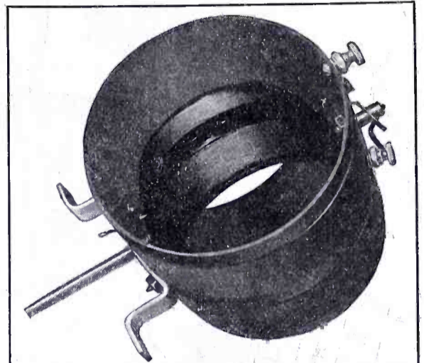
Catalogue No. 166.....$5.50 SE-AR-DE VARIO COUPLER (Center Rotor Type)
