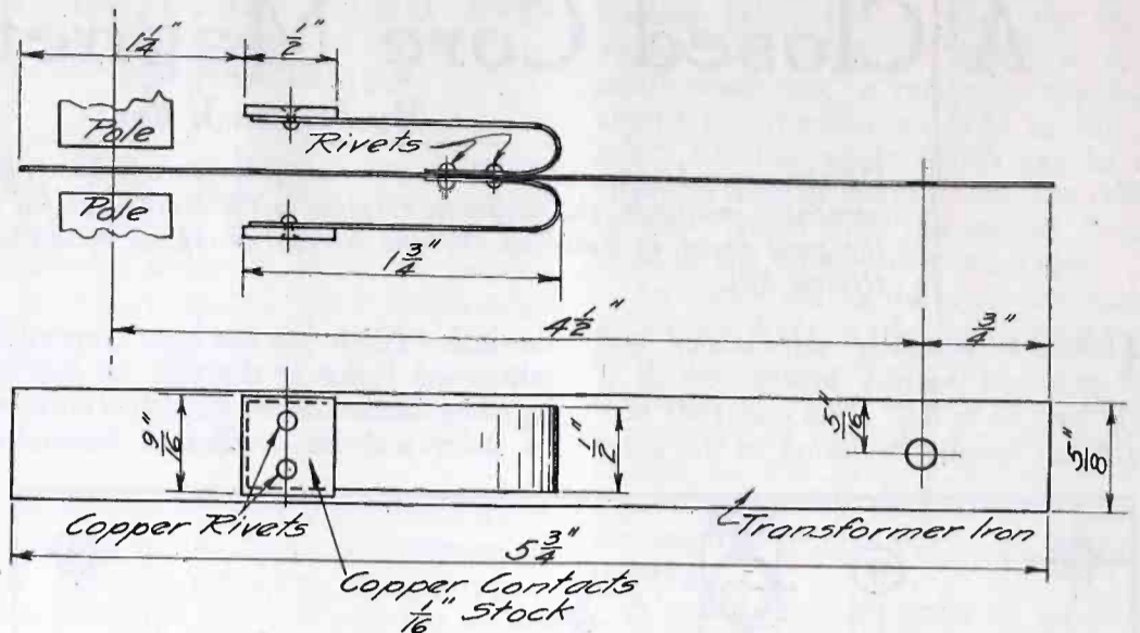
Fig. 5. Commutator Detail
