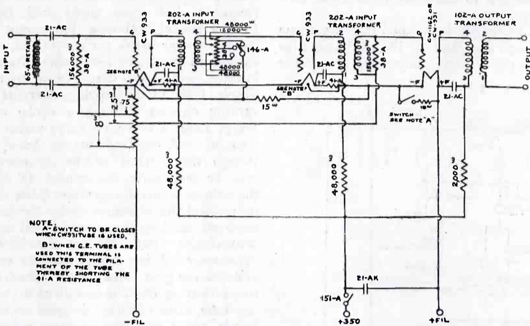
Fig. 3. Amplifier Circuit Diagram
