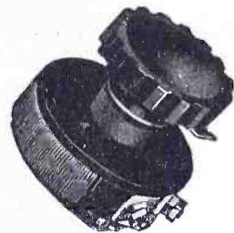
KING QUALITY Rheostat. R-630 Resistance valve 6.5 ohms. Special Brass Panel Bushing insures smooth operation. Genuine Bakelite Base.
