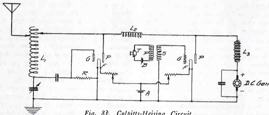
Fig. 83. Colpitts-Heising Circuit
