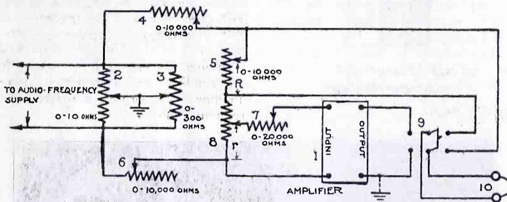
Fig. 1. Circuits for Measuring Audio-Frequency Voltage Amplification
