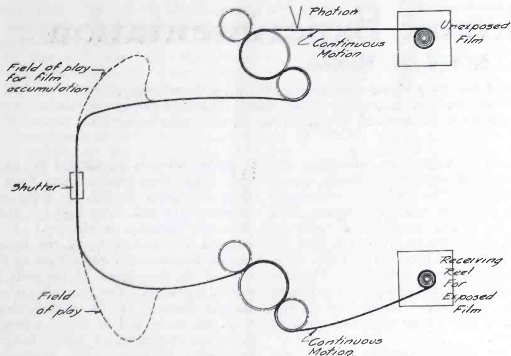
Fig. 2. Sound Projection System.
