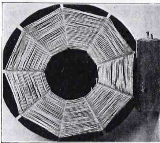
Fig. 1. Spiderweb or Pancake Coil
