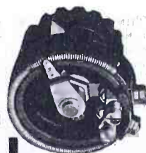
KING QUALITY Rheostat. R-630 Resistance valve 6.5 ohms. Special Brass Panel Bushing insures smooth operation. Genuine Bakelite Base.
