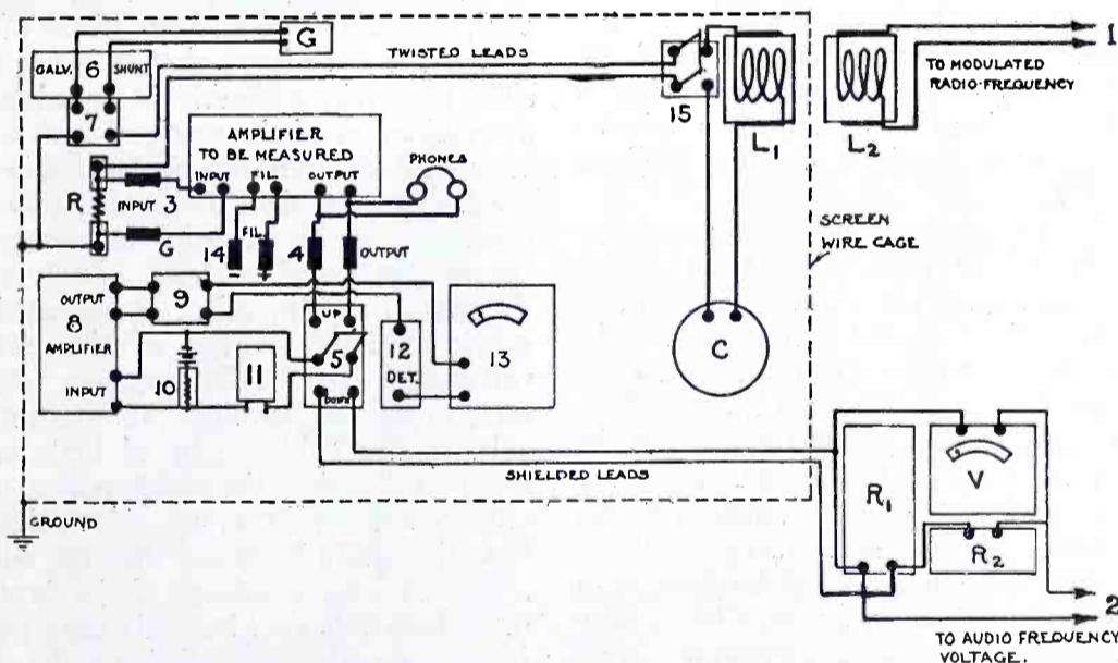
Fig. 3. Circuit for Measurement of Radio-Frequency Voltage Amplification
