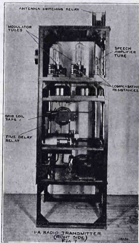
Fig. 84. Side View of 500-Watt Western Electric Broadcasting Set
