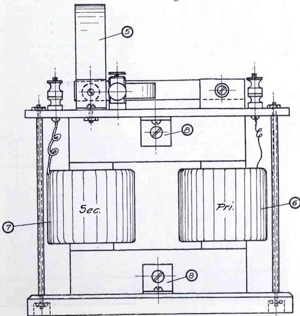
Fig. 2. Side View
