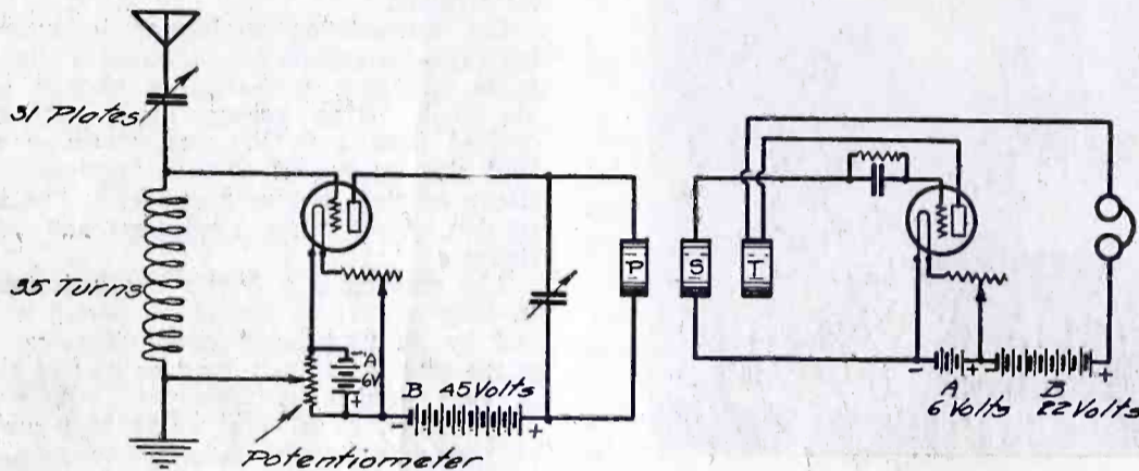
Radio Frequency Amplifier with Honeycomb or Spiderweb Tuner.
