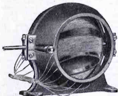
Pioneer Variocoupler
