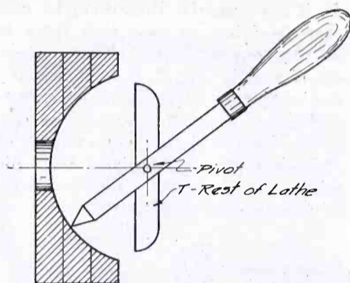
Fig. 9. Turning the Stator Mounting
