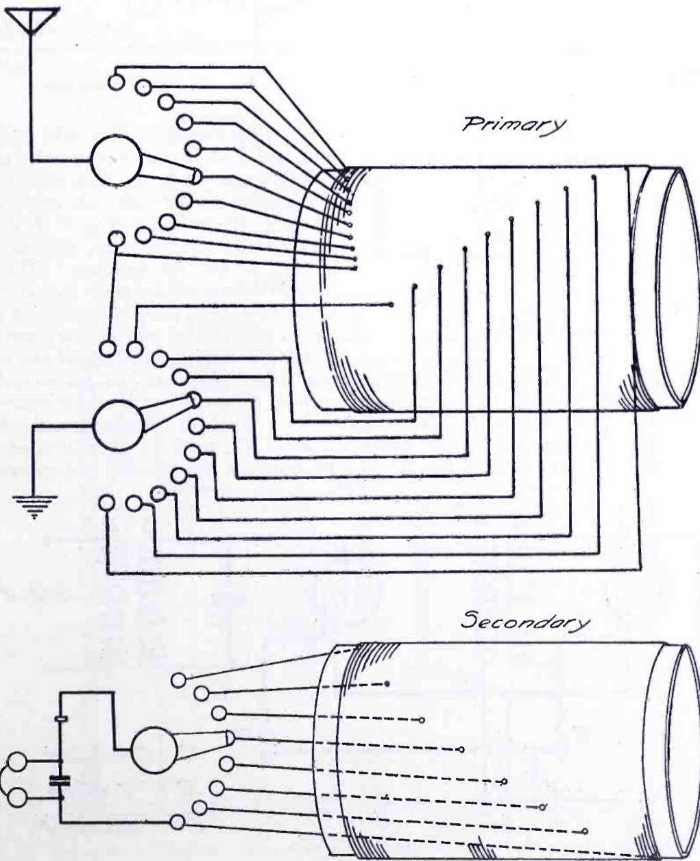
Loose Coupler Construction
