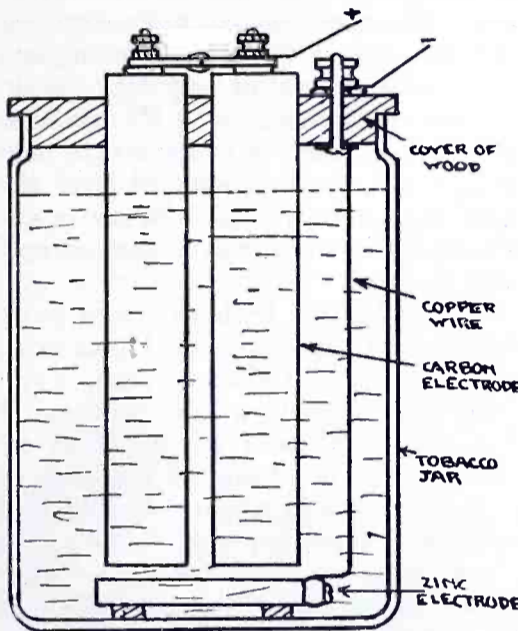
Fig. 3. Battery Assembly
