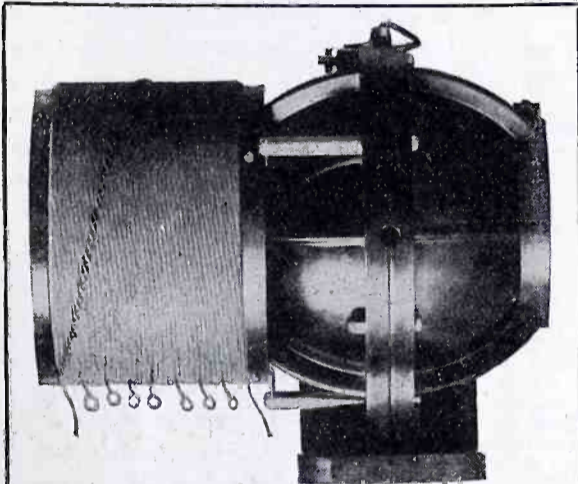
Catalogue No. 165.....$13.00 SE-AR-DE RADIOMETER WITH B. W. INDUCTANCE
