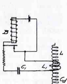
Fig. 6. Circuit for Measuring Distributed Capacity
