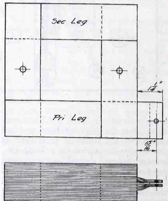
Fig. 7a. Core Dimensions
