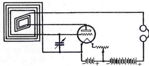
Fig. 6. Regenerative Loop Circuit
