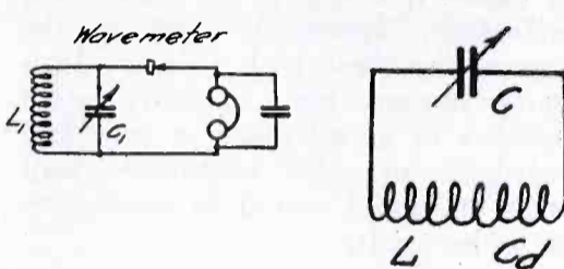
Fig. 7. Circuit for Graphical Measurement of Distributed Capacity
