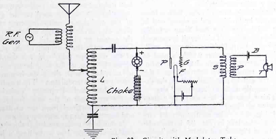
Fig. 82. Circuit with Modulator Tube
