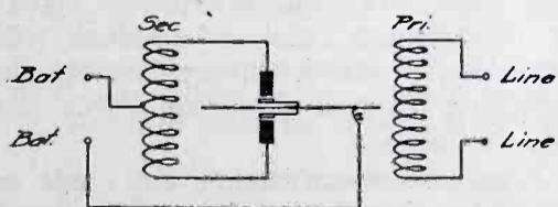
Fig. 8. Diagram of Connections
