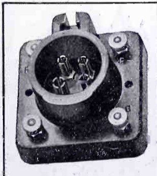
Catalogue No. 199, $1.00 SE-AR-DE Socket for WD11 Tube, positive contacts.
