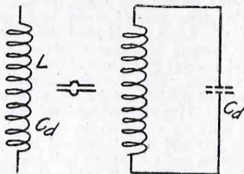
Fig. 2. "Lumped" Representative of Distributed Capacity
