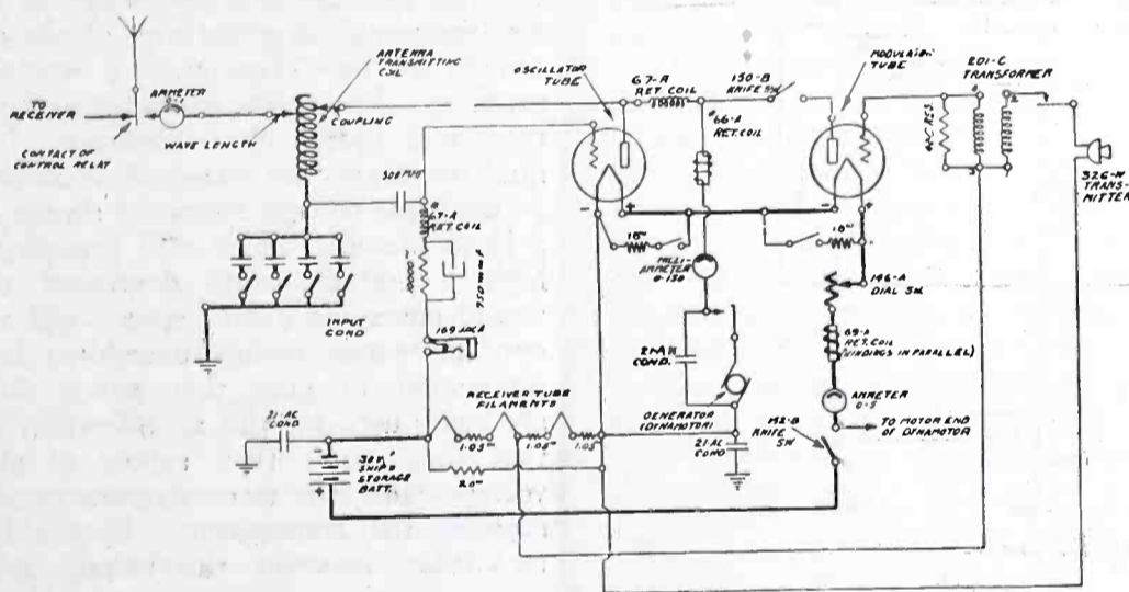
Fig. 1. Oscillator and Modulator Circuits
