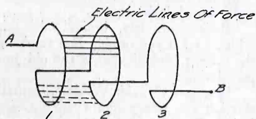
Fig. 1. Distributed Capacity in Induction Coils
