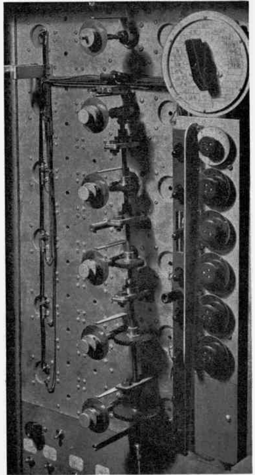
FIG. 4 One of the steering drives showing the helical gears and the shafts of the six phase shifters.
