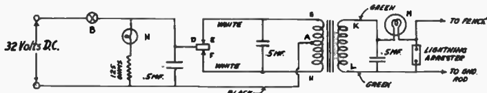
Diagram of electric fence control for 32-volt farm-lighting system.
