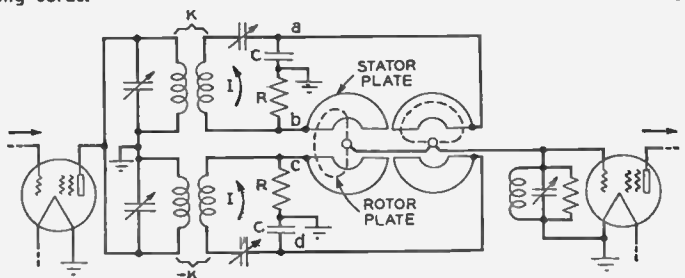
FIG. 2 The transmission lines from the antennas terminate in coaxial jacks and are connected to the input circuits by coaxial patching cords.
