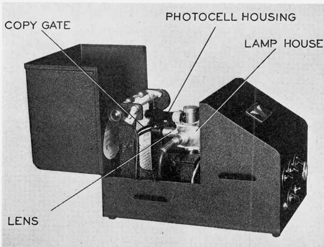
Finch transmitter, with cover hinged back to facilitate loading. All controls are located at convenient position on front panel of unit. The device plugs into any 500 ohm line and works at maximum signal level of zero decibels. It is easily operated and maintained.
