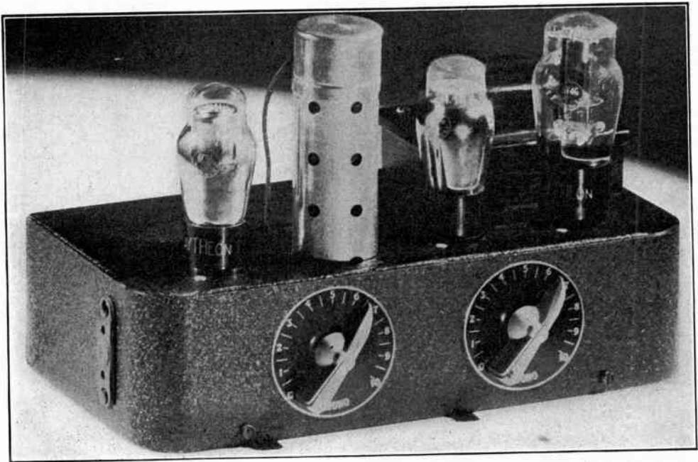
FIG. 2 View of the commercially-made expander.
