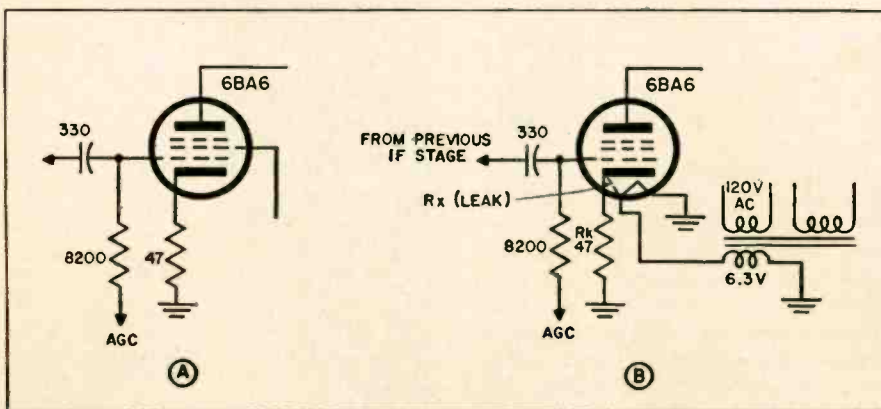
Fig. 6—K-F leakage shunts heater winding across R_k , applies 60 cps bias to tube.
