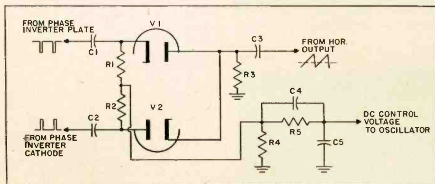
This twin-diode phase detector controls horizontal oscillator frequency in many TV sets.
