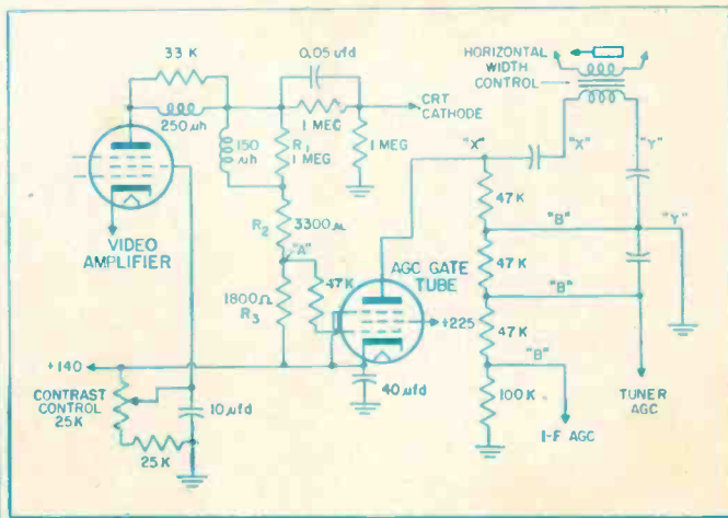
Fig. 4—Keyed agc system using a video signal source for input.
