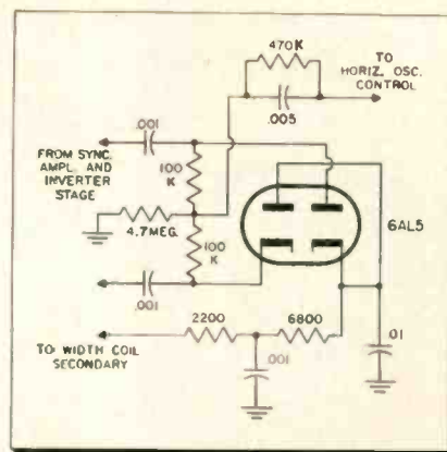
Fig. 8—Hum pickup is common in phase detectors, and other circuits using high value components.
