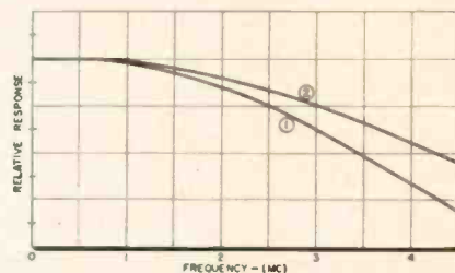
Fig. 6—Scopes with slow roll-off characteristics. Scope 1 rolls off faster than scope 2.
