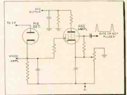
Fig. 5—Keyed system with threshold control.
