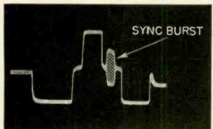
Fig. 3—Burst in output of a color generator.
