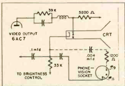
Retrace blanking circuit, early Zenith sets.
