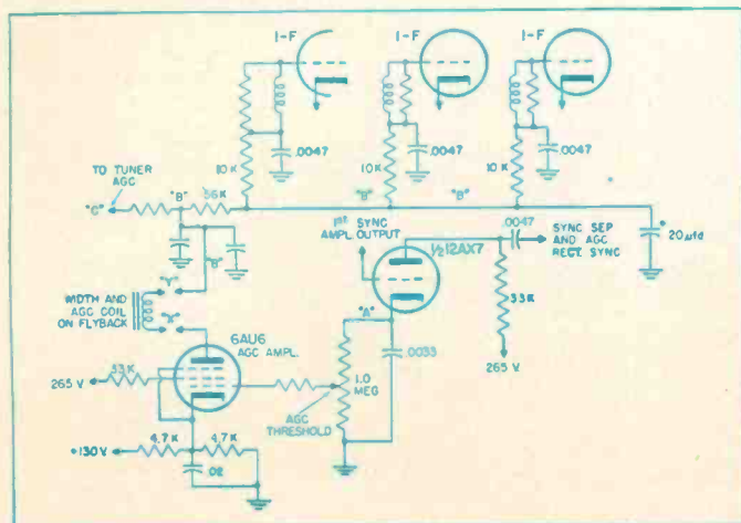
Fig. 3—Keyed agc system with rectified source of agc voltage.
