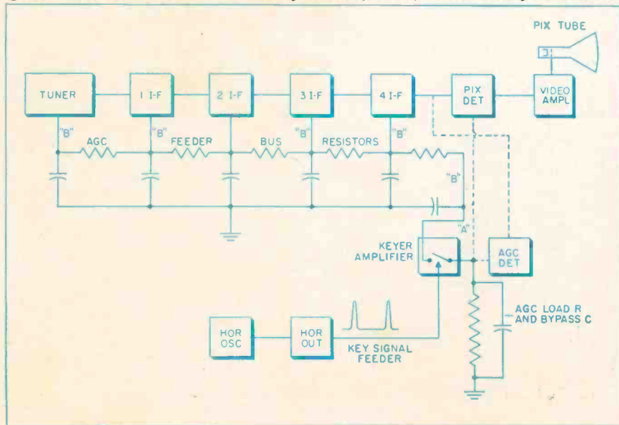
Fig. 1—Simplified diagram of keyed agc system. Broken lines show alternate use of a separate agc detector to obtain demodulated video signal for keyer tube, instead of using video detector.
