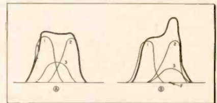
Fig. 7—Hum leakage may shift the resonant frequency of one i-f stage, producing oscillation due to the excessive gain.
