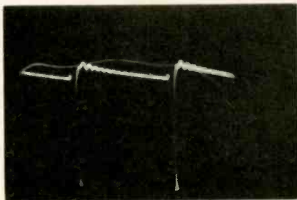
Fig. 7—Ringing in a sweep-circuit waveform.
