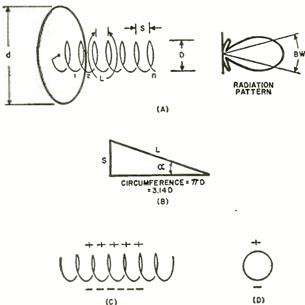
Fig. 1. (A) Dimensions and radiation pattern. (B) Pitch angle. (C) Charge distribution, side and (D) end views.
