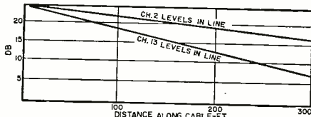
Fig. 3. Cable losses increase with greater lengths and higher channels.
