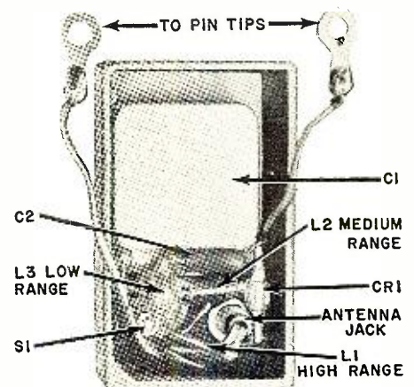
Fig. 4. Inside view of the compact adapter, with parts locations shown.
