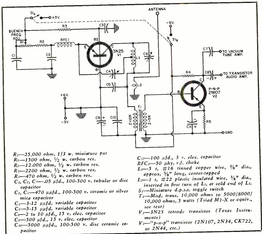
Fig. 2. Complete schematic diagram and parts list for the superregen receiver.
