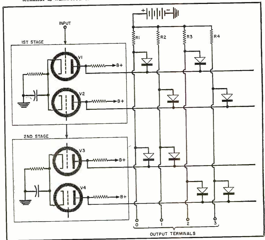
Fig. 5. The diode matrix consists of an array of vertical and horizontal wires, some of which are connected by diodes. As input pulses are applied to flip-flop, output pulse will transfer from one output terminal to the next. Each output terminal is numbered to indicate the required number of input circuit pulses.
