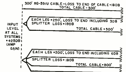
Fig. 5. How splitters can increase cable coverage with a given loss.
