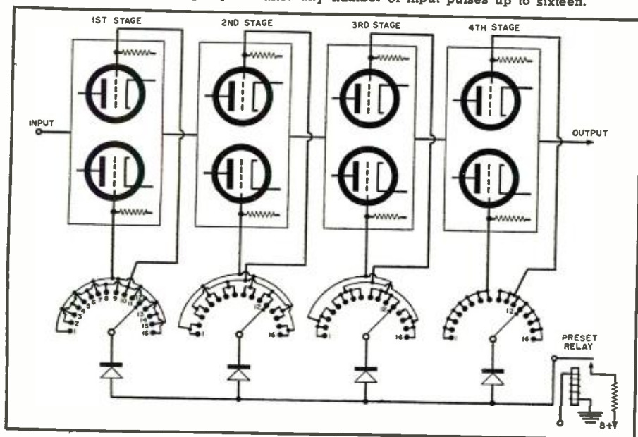
Fig. 1. The circuit of a basic preset counter is shown here. When the relay is energized, a positive potential is applied to one of the two grids for each stage. Which grids will receive this positive voltage is determined by the positions to which the switches are preset. The circuit can be adjusted to produce an output pulse after any number of input pulses up to sixteen.
