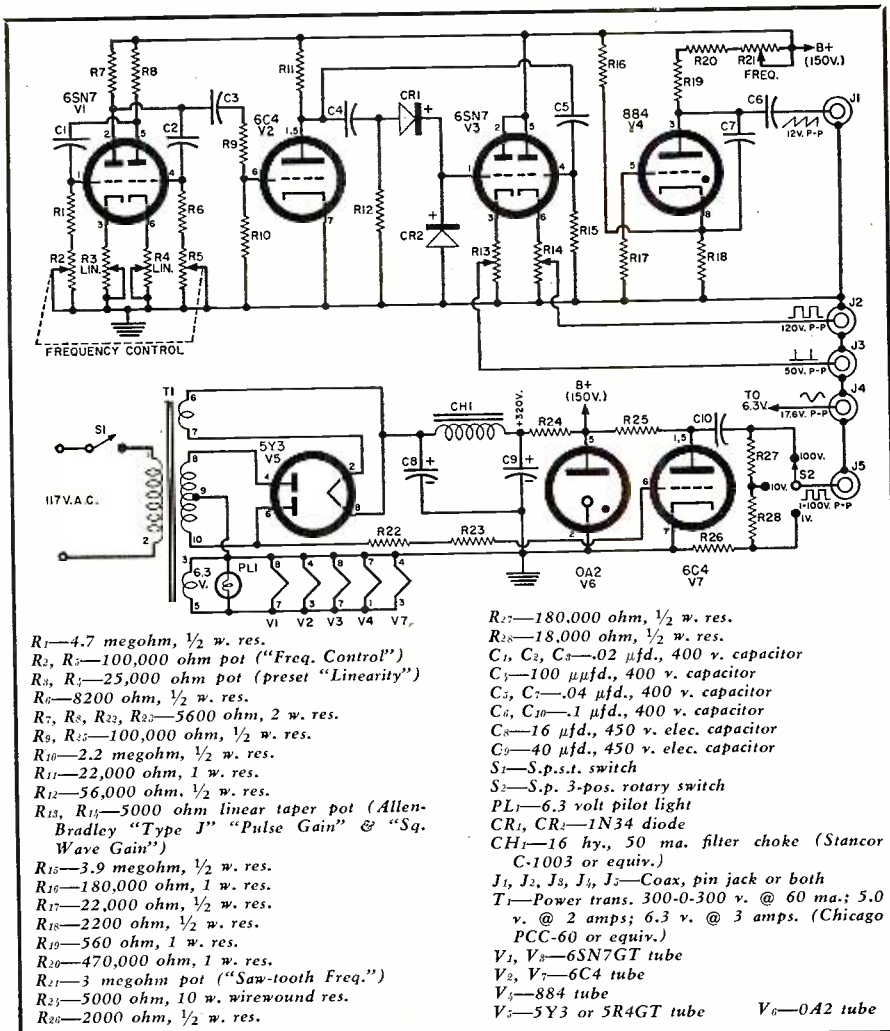
Fig. 1. Complete circuit diagram and parts listing of the accessory test unit.
