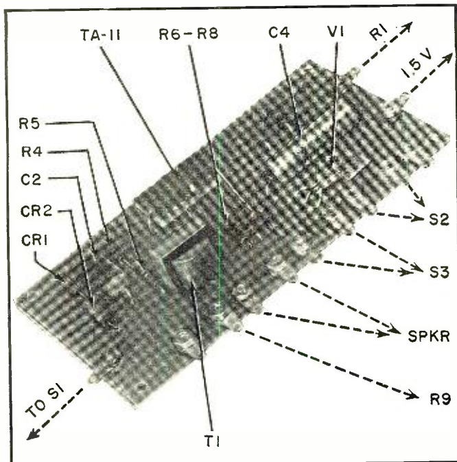
Fig. 3. The circuit board, with most components mounted.
