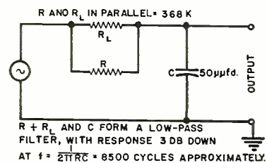
Fig. 10. (A) Effect of using a voltage divider as load resistor for piezoelectric cartridge is shown here. (B) Equivalent circuit of Fig. 10A at high frequencies.
