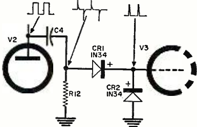
Fig. 3. Partial schematic showing pulse formation and then clipping by the diodes.
