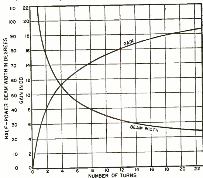
Fig. 2. Antenna gain and beamwidth shown as a function of the number of turns, for a helix having a circumference equal to one wavelength along with a pitch angle of 12.5 degrees.
