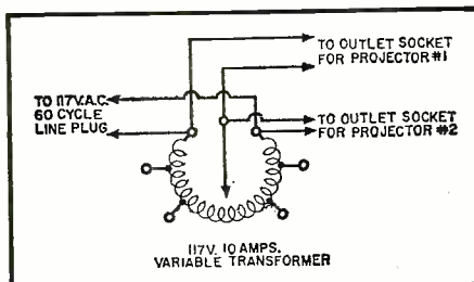
Fig. 1. Wiring diagram for fade control which permits operation of two projectors.
