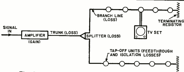
Fig. 1. This simplified layout diagram of a multi-set installation shows all the principal elements.
