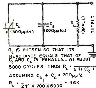
Fig. 13. Use of small load resistor makes crystal cartridge velocity-responsive unit.
