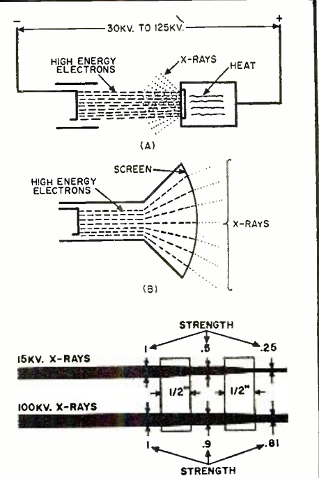
Fig. 3. When x-rays pass through such media as glass, there is much more absorption of soft x-rays (top diagram) than of the hard radiation shown below.
