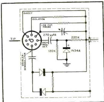
Fig. 4. Suggested circuits for various probe functions. Values not shown may vary. Each circuit connects to separate point on octal socket at one end, but all terminate in common lead to scope.
