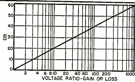
Fig. 2. A graph like the one shown can be used to convert voltage gain and loss ratios into decibels for more convenient system calculations.
