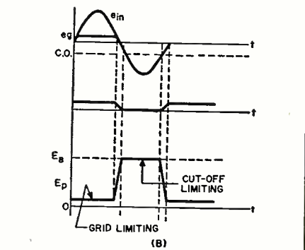
Fig. 5. (A) A combination of grid and cut-off limiting produces 60 cps square waves.
