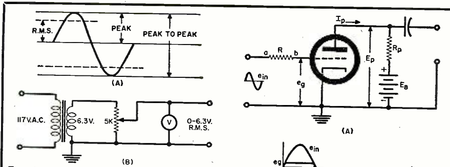
Fig. 2. (A) Sine-wave relations discussed. (B) A simple scope calibrator may be built.
