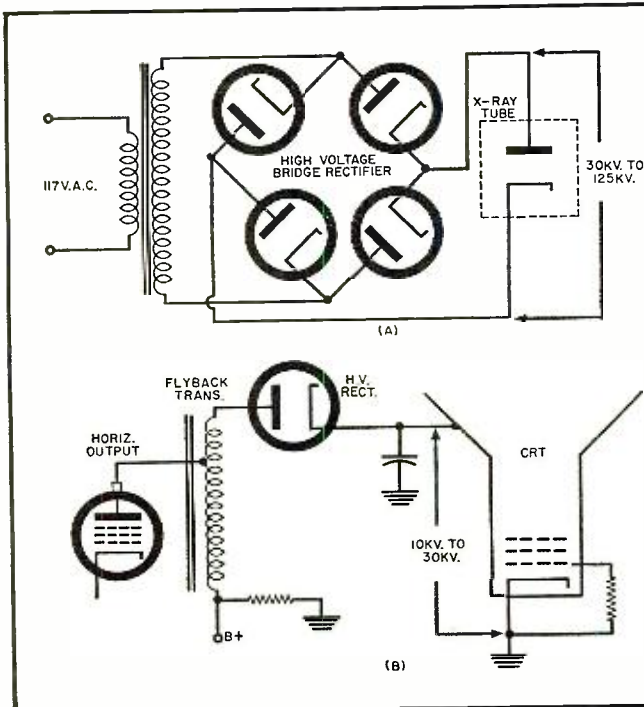
Fig. 1. The circuit for generating x-rays (A) is a big uncle to the more familiar television high-voltage circuit of (B).
