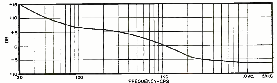
Fig. 6. Variation of the groove amplitude with frequency due to RIAA recording equalization, assuming there is a constant signal input at all the frequencies depicted.
