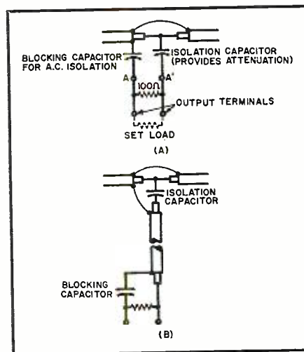
Fig. 7. Typical tap-off configurations: combined type (A) and separated type (B).
