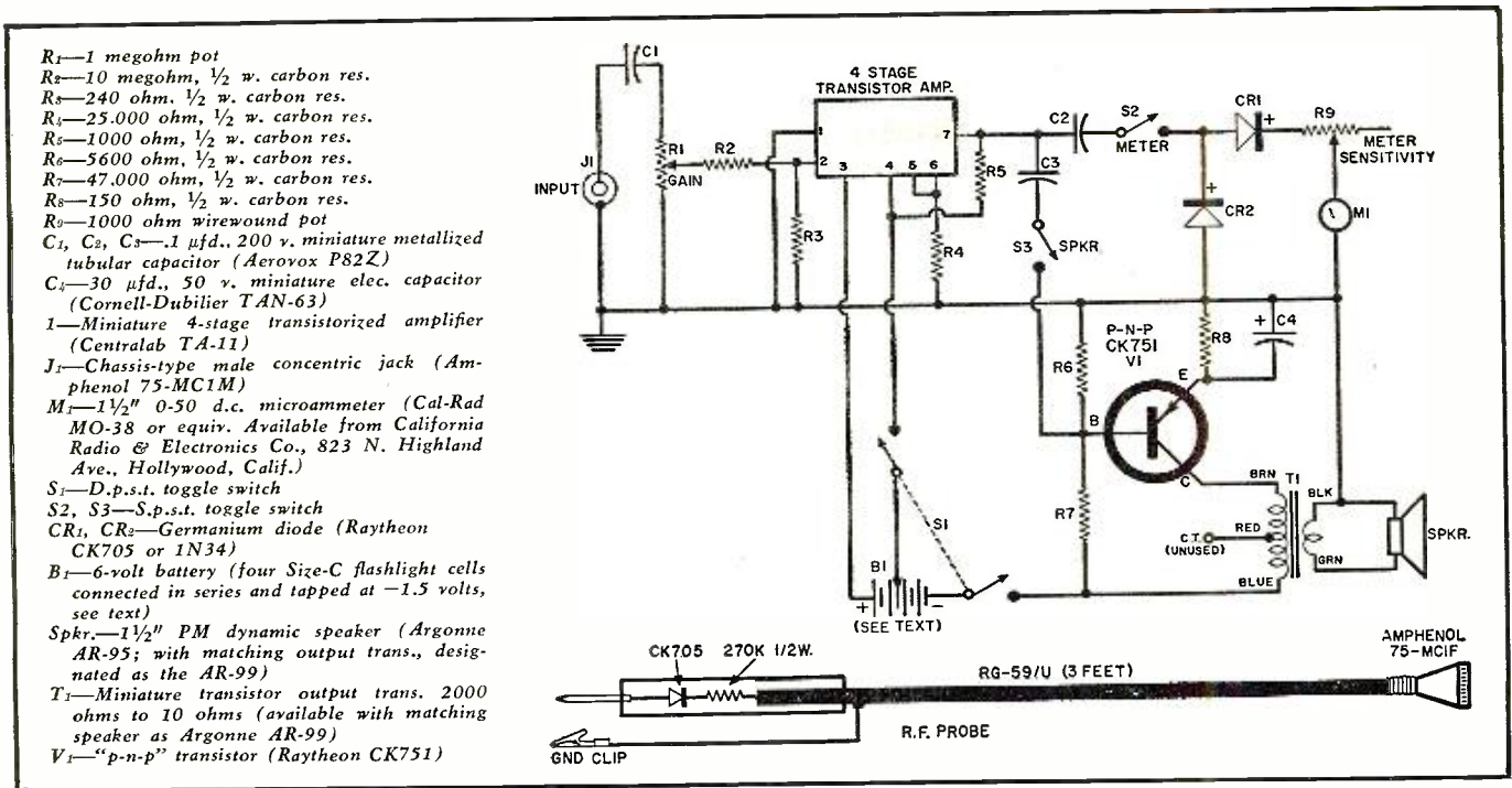
Fig. 2. The signal tracer circuit built around the packaged transistor amplifier. The auxiliary r.f. probe is also shown.
