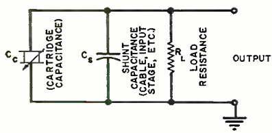
Fig. 7. Circuit parameters that are associated with a piezoelectric cartridge.
