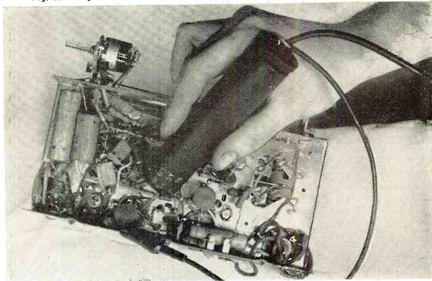
Fig. 3. The probe in use. Note the identifying function markings on the body.
