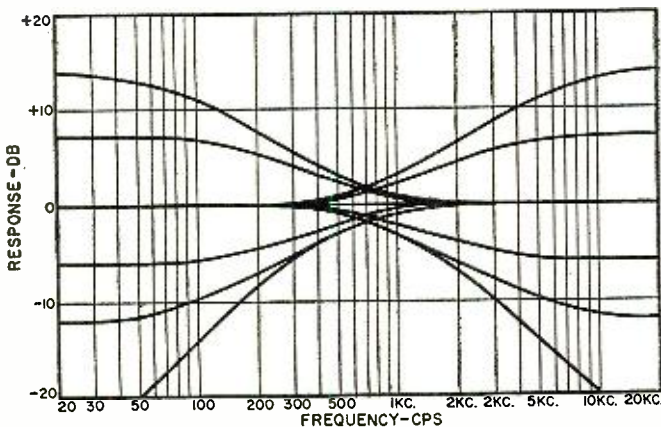
Fig. 1. Here are typical frequency response changes that are produced by the tone controls in a high-fidelity amplifier.
