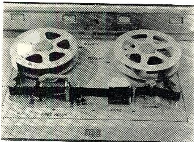
Close-up view of transport with cover plate removed.
