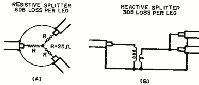
Fig. 4. Line splitters may be resistive (A) or of the reactive type (B).
