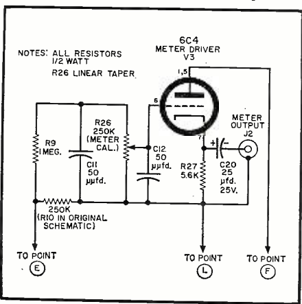
Fig. 1. Simple circuit changes permit the addition of a vu meter to tape amplifier.
