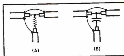
Fig. 6. Resistive (A) and capacitive (B) methods for tapping a feeder line.
