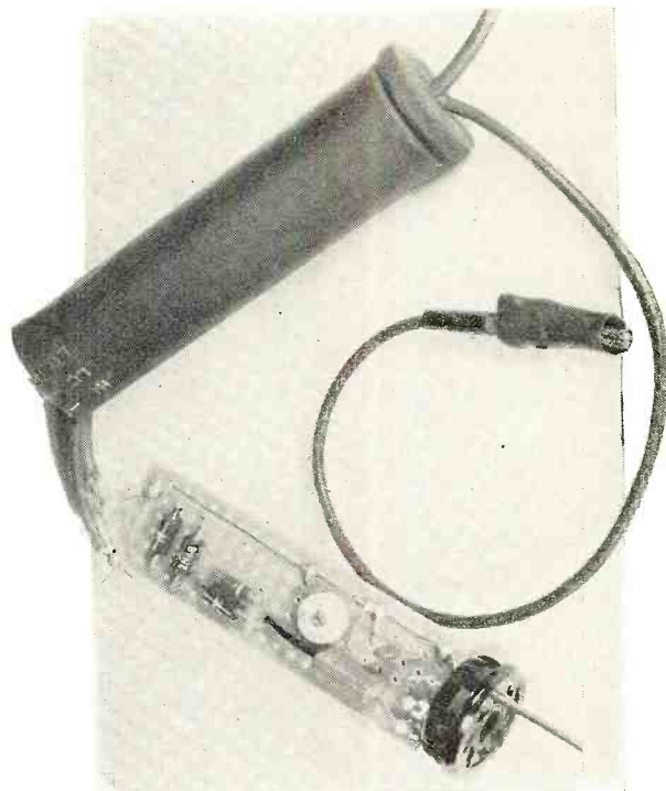
Fig. 1. When the component board is slid into the tubular housing with only the socket showing, this version of the multi-purpose probe will be complete.
