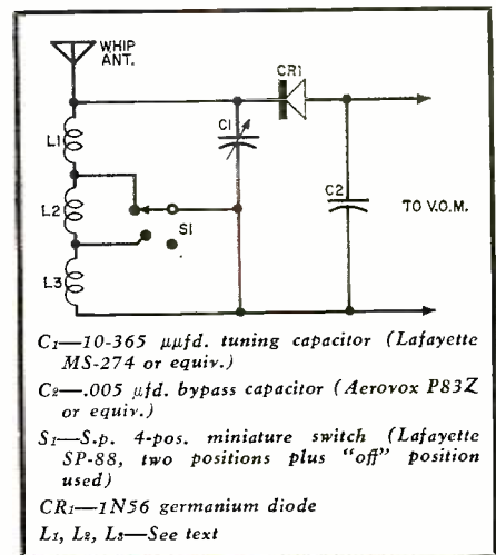
Fig. 3. Schematic and parts list for the simple, wide-range fs adapter.
