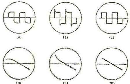
Fig. 5. Square waves may be used (A, B, and C) to adjust a low-capacitance probe. The scope's own sweep oscillator can also be used (D, E, and F) for this purpose.
