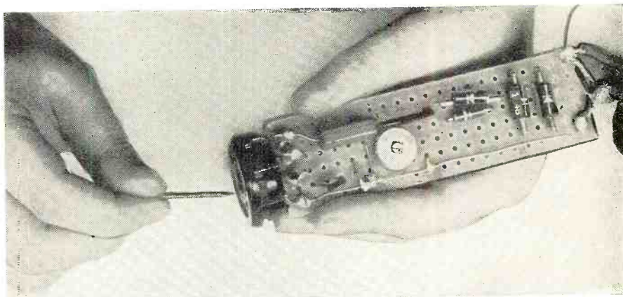
Fig. 2. Inserting the tip in the various socket holes selects probe function.
