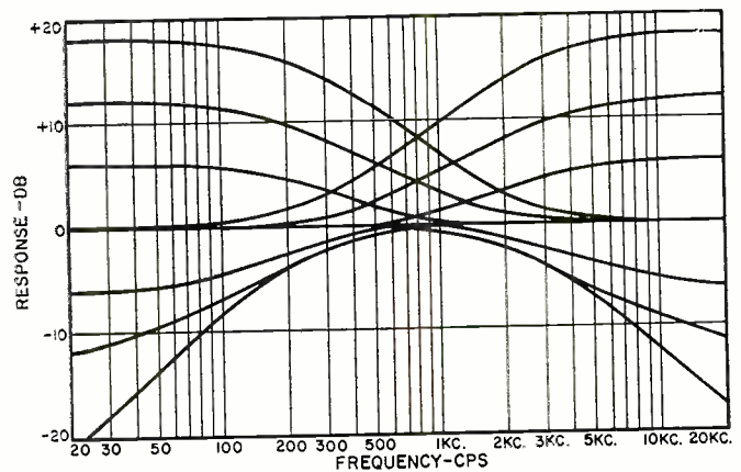
Fig. 2. Shown here are the response changes that would provide more suitable control in a public-address amplifier.
