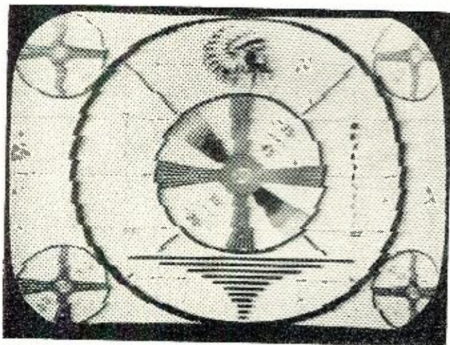
Fig. 4. Test pattern resulting from slight guide misadjustment. This shows the group of picture lines each head covers and the result of a timing error which was purposely induced in this case. This condition is called "picture skewing" and it is corrected for by automatic compensation.
