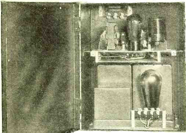
Fig. 3—An "inside" view of the extension coupling unit
