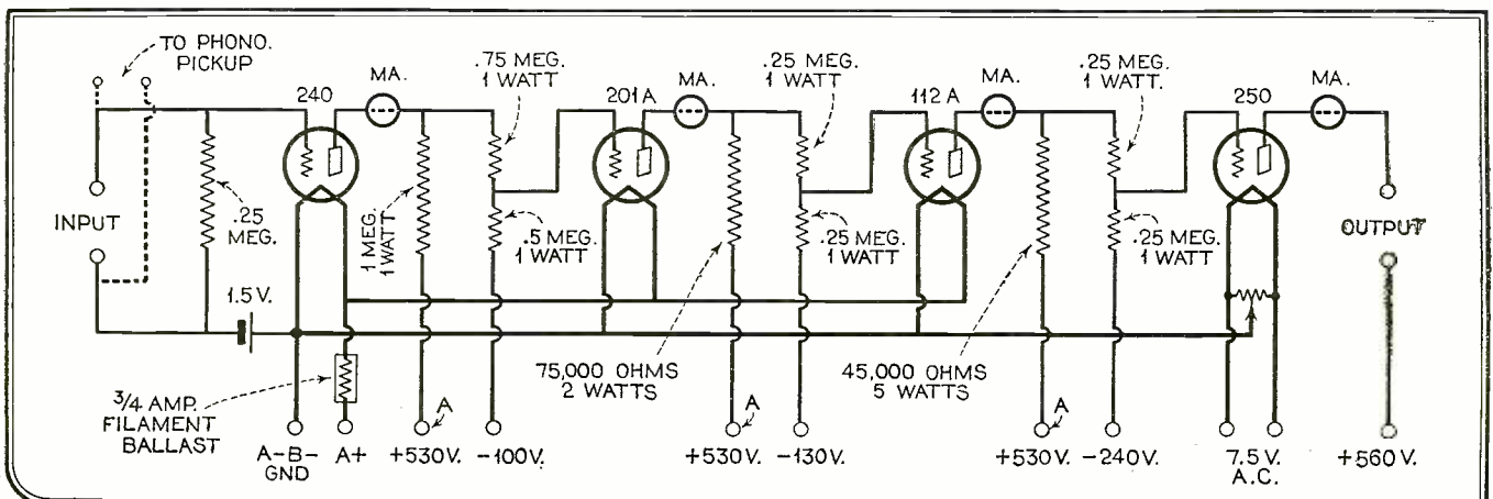
Fig. 3—This is the actual circuit, showing values of parts employed, which was used in the construction of the amplifier illustrated in the upper right corner of the following page
