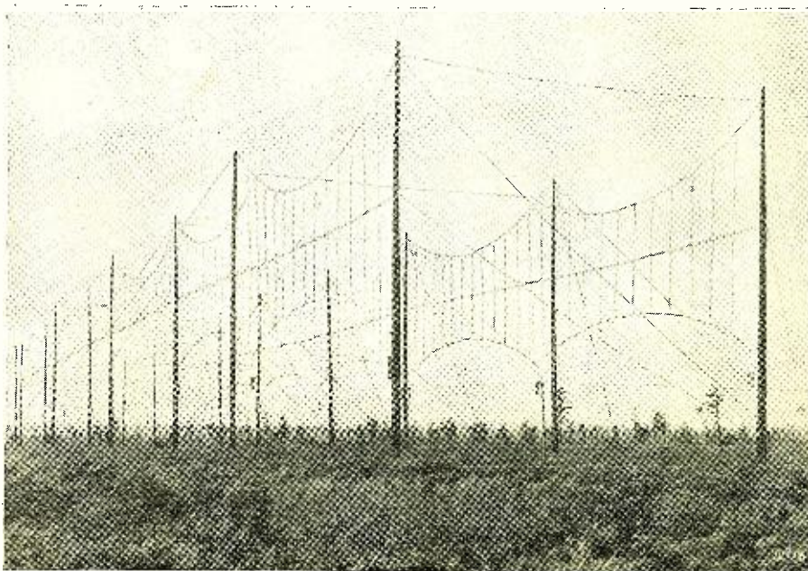
Aerial network at the Rocky Point station which forms an important link in international short-wave communication
