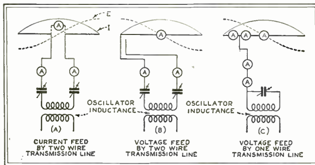
Fig. 3—Three types of short-wave transmitting antenna which will work satisfactorily on 42 meters or from 83 to 85 meters. A is a \frac{1}{4} \lambda antenna, B a vertical antenna with 2-wire feed, and C a horizontal Hertz, \frac{1}{2} \lambda , for 84-85 meters or full-wave for 42 meters
