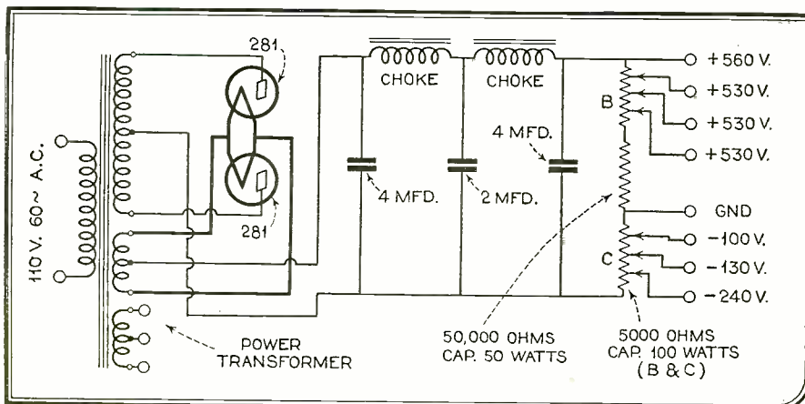
Fig. 4—The circuit of the power supply device which provides the necessary "B" and "C" voltage for the operation of the amplifier described by Mr. Morgan
