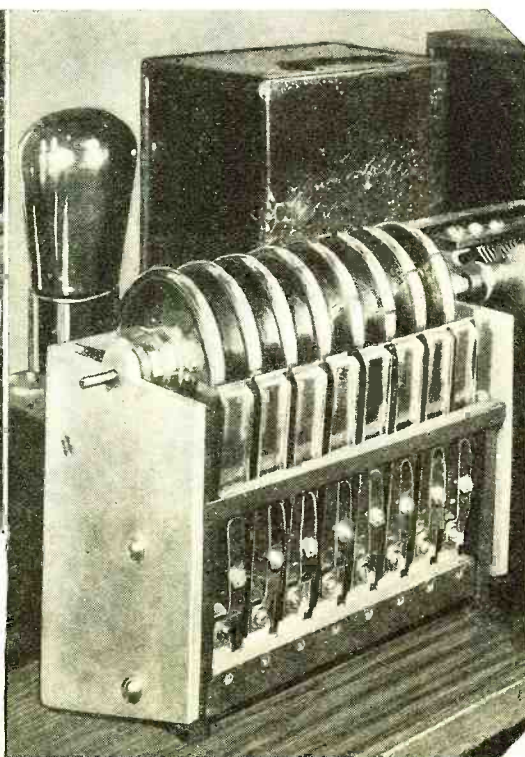
Above and to the right are shown the rectangular push buttons, motor and selector switches of the Carter system of automatic tuning. Pressing the button causes the motor to rotate the condenser shaft to a stopping point determined by the cam and switch (at the right), which is connected to the button pressed
