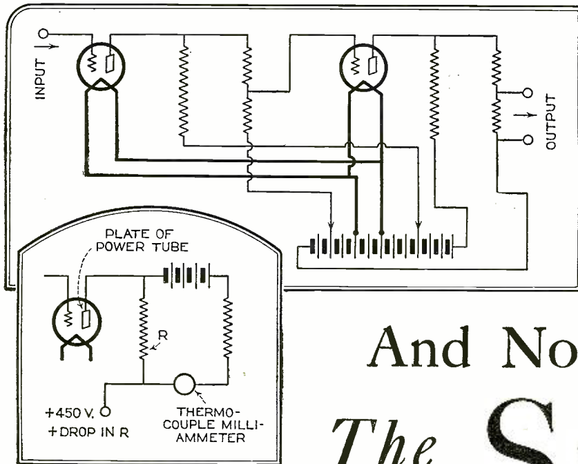
Fig. 1 (top) shows the fundamental circuit which was chosen as the most practical for straight resistance coupling. Fig. 2, below, shows the balancing-out system employed to gain a wide frequency response of from 0 to 20,000 cycles per second
