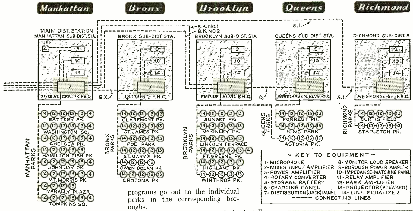
Fig. 2—Some idea of the problem of distributing the concerts from a central point to the other city parks may be obtained from the diagram above
