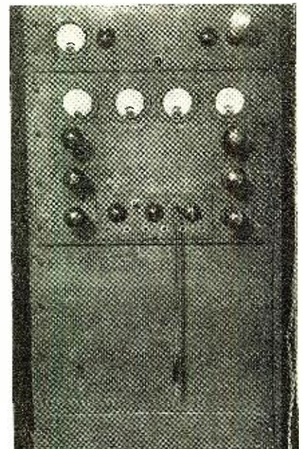
Fig. 3—The Samson amplifier rack located in the basement under the bandstand. Here the concerts are monitored and amplified before being sent to the other parks
