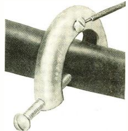
Fig. 4—Speedy connection ground clamp
