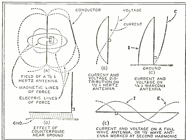
Fig. 1—At A is shown a \frac{1}{2}\lambda Hertz antenna, with the absorption effect of a nearby conductor indicator. B shows the voltage and current distribution of this type of antenna, while in C the same is indicated for a \frac{1}{4}\lambda Marconi antenna. With the latter a counterpoise, as shown in D, may be used. E shows the voltage and current distribution of a full-wave antenna worked at its second harmonic
