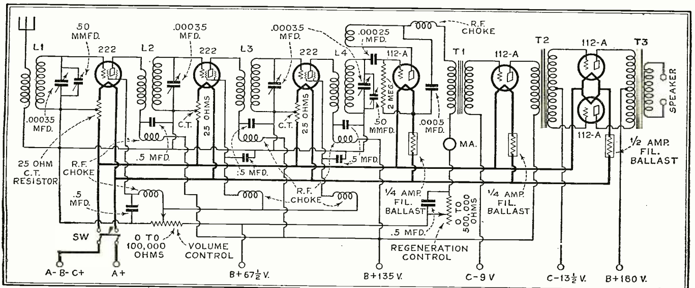
Fig. 1. This is the complete circuit of the d.c. model Radio News-Elco Boat Receiver. The coils used are standard Remler broadcast coils, No. 562 and 564, the latter being used in the detector circuit. All the other parts employed have their values indicated on the diagram
