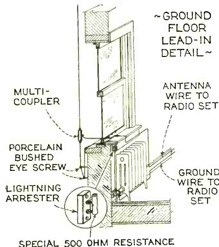
Fig. 4—Circuit details of the multi-coupler system of antenna installation. One antenna will feed as many as twenty receivers
