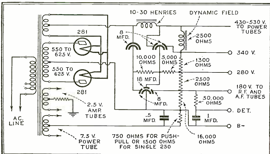
Fig. 1 The "power supply" circuit, featuring the electrolytic condensers in the filter section. All values of parts used are indicated
