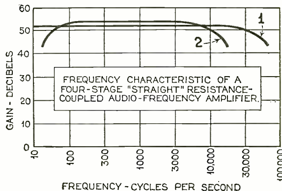
Fig. 5—The curve 1 shows the frequency characteristic obtained when an output resistance and balancing battery are employed in the amplifier circuit (as in Fig. 2). Curve 2 shows the frequency characteristic of the amplifier when a choke coil and condenser couples the loud speaker to the amplifier
