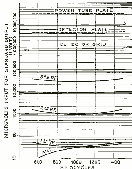
Fig. 3. Analysis of sensitivity in automobile receiver
