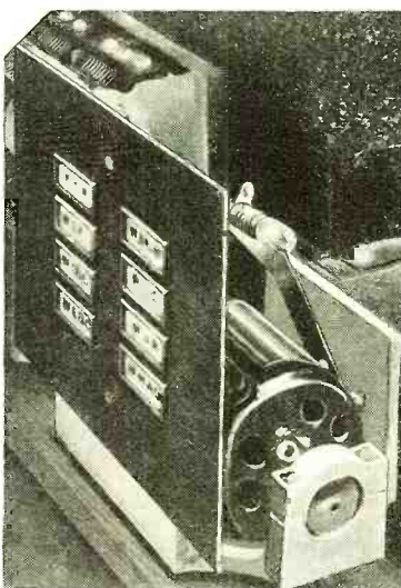
Above and to the right are shown the rectangular push buttons, motor and selector switches of the Carter system of automatic tuning. Pressing the button causes the motor to rotate the condenser shaft to a stopping point determined by the cam and switch (at the right), which is connected to the button pressed
