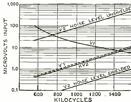
Fig. 2. The relation between useful receiver sensitivity and ignition interference level. V_2 = microvolts input for nearly complete shielding, V_2' = microvolts input for no shielding, V_1' = common sensitivity characteristic of a receiver
