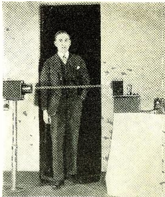
Photo-electric tube device for counting persons passing through a doorway
