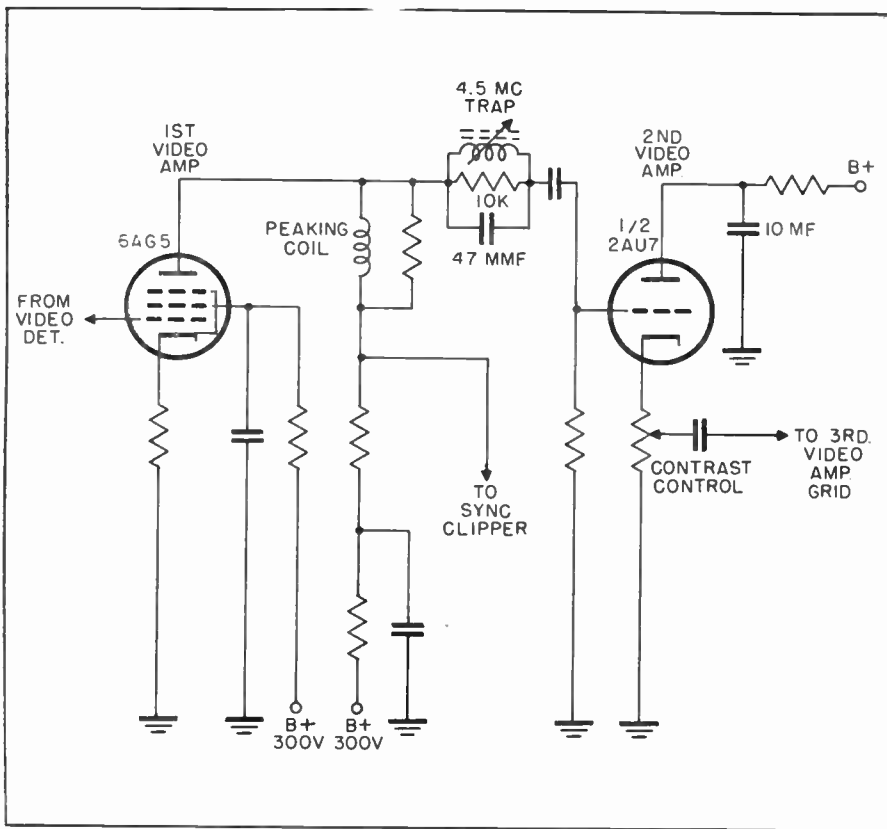
Fig. 2 Simplified schematic diagram showing the 4.5 Mc wavetrap which has been incorporated in the interstage circuit of the video amplifiers in the DuMont Model RA-105
