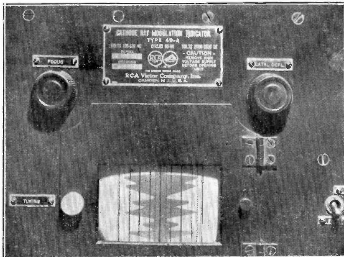
Oscillograph pattern of music transmitted over WBEN. The technicians strive to keep the edges of the pattern clean-cut at all times.
