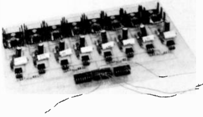
FIG. 6—CONNECTION to the AC controller is made through DIP header. Ribbon cable may be used instead of individual wires.
