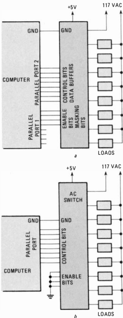
FIG. 8—IF SEVERAL PARALLEL PORTS are available at computer, use hookup shown in a; with only one port, use that in b.
