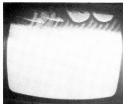
FIG. 9—WHITEOUT caused by severe hum modulation. An open-filter capacitor in antenna-booster power supply was source.
