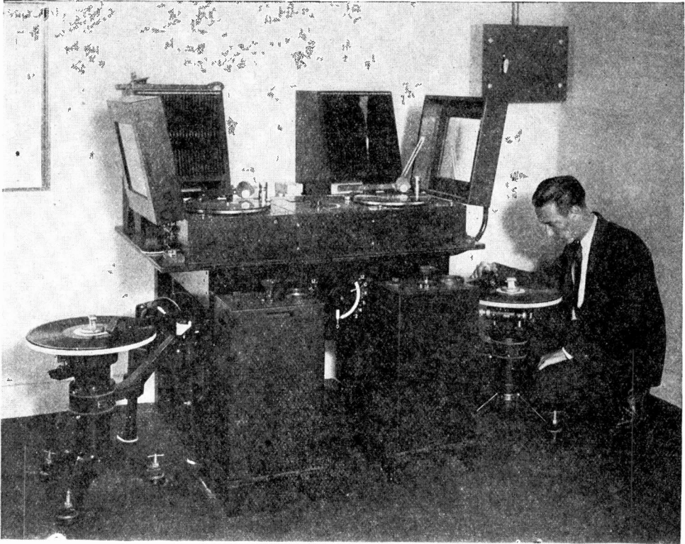
This photo shows the equipment used at station WOR for the broadcasting of recorded programs. A total of four turn-tables is available.
