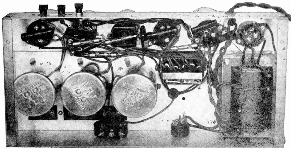
Under view of the chassis. Lower left, shielded radio-frequency coils. Right: Power transformer. To the left of the latter is the block of by-pass condensers. On the front side of the chassis are the volume control (below the second and third shields) and the power switch.
