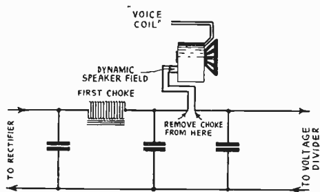
CONNECTION OF A DYNAMIC SPEAKER FIELD FOR USE AS A FILTER CHOKE IN A "B" ELIMINATOR.
