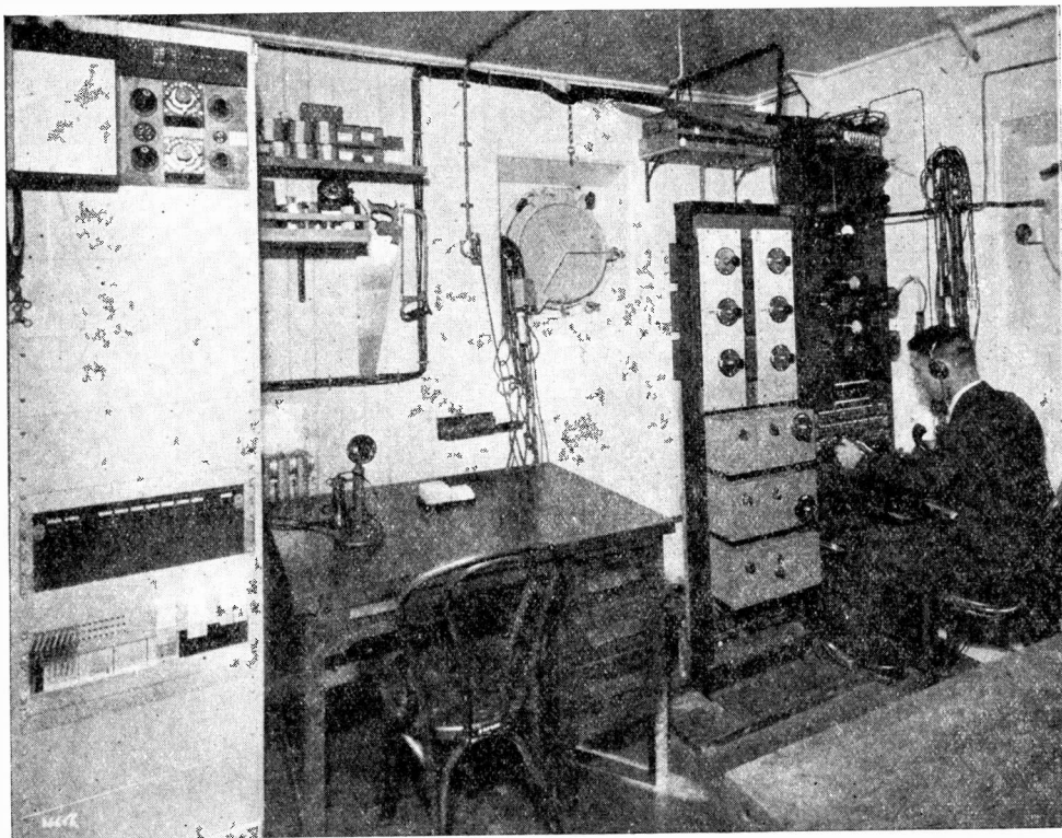
Interior of the deck house on the steamer Leviathan, which houses the short-wave radio equipment. To the right is the receiving set, where voices from shore telephones are received by radio from the Deal, N. J., station.
