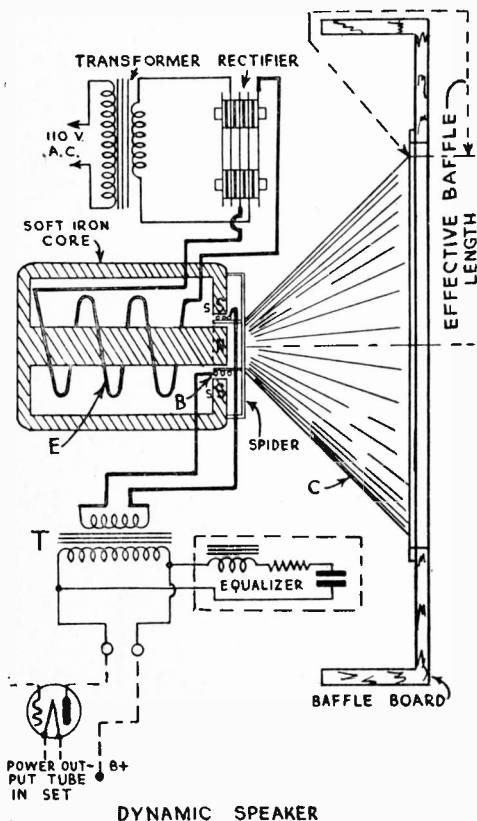
Fig. 3: A typical electrodynamic speaker layout.
