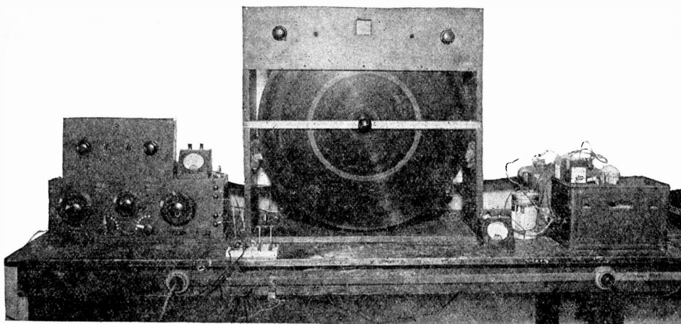
A typical experimental receiver constructed by an amateur. The best images this apparatus can reproduce are about 1\frac{1}{4} inches square, and are built up on the plates of a neon-gas lamp. The big disc is motor driven, and must be balanced with extreme care. Great stuff for the dabbler, but certainly not practical for the public.
