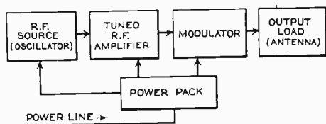
FUNCTIONAL DIAGRAM OF THE TRANSMITTER
