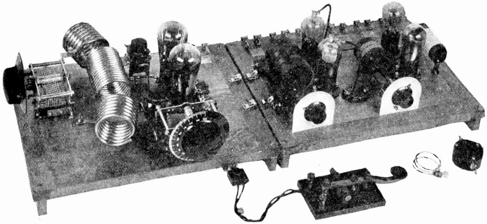
ABOVE: A more complicated transmitter employing six tubes in a push-pull hook-up. This outfit also makes use of parts such as found in any ordinary receiving set. By means of this transmitter, communication is established quite regularly between Hartford, Conn. and points in Australia and New Zealand.
