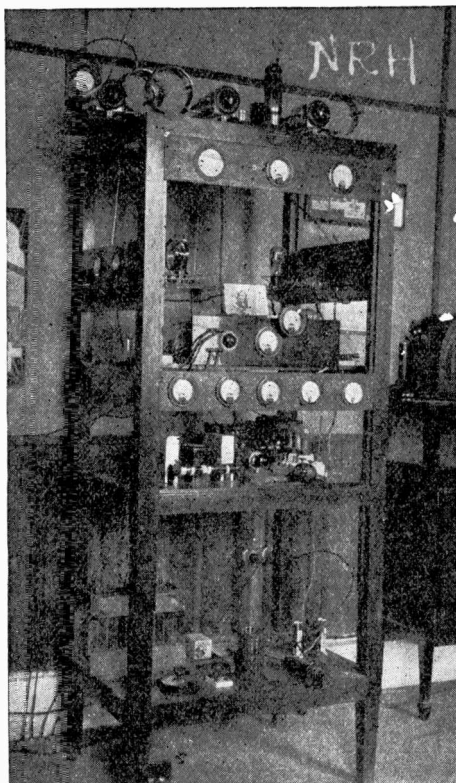
Above: This looks like a big frame, but the actual transmitter on it has an output of only 7\frac{1}{2} watts. Señor Cespedes pieced the whole outfit together himself, working patiently with only the assistance of magazine articles and letters from American amateurs. Left: The youngest member of the Cespedes family, who is as familiar with his father's microphone as he is with his own rattle.
