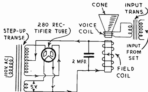
CIRCUIT OF DYNAMIC SPEAKER WITH TUBE RECTIFIER
