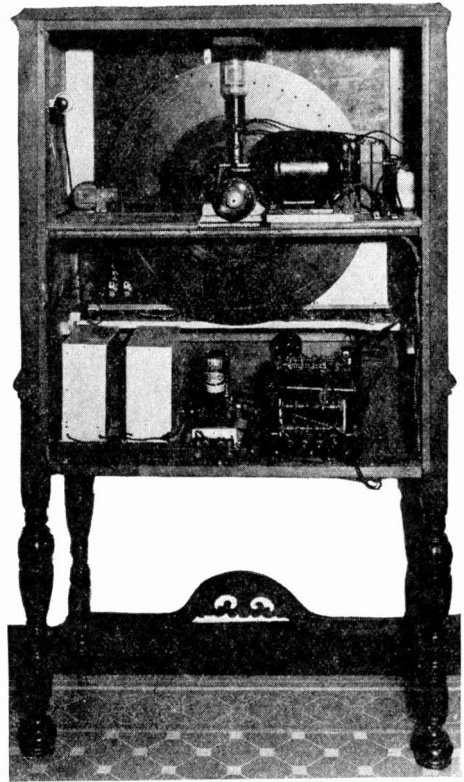
A special television receiver built by John Geloso of the Pilot company more than two years ago and used successfully for the reproduction of images broadcast by WRNY, Coytesville, N. J. Both the R.F. and the A.F. circuits are of highly special design and cost a young fortune to build. Flickering images about 1½ inches square were obtained when reception conditions were favorable.
