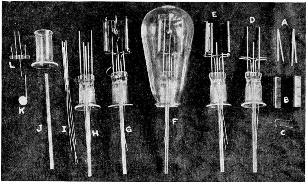
The Pilotron 280 broken down to show its construction: A, filaments. B, plates. C, filament hooks. D, stem with wires formed. E, stem with plates and filaments mounted but not supported. F, completed tube without base. G, stem assembly complete with supporting bead. H, formed stem with unformed wires. I, connecting and supporting wires. J, unformed stem and exhausting tube. K, "getter" cup. L, center supporting bead.
