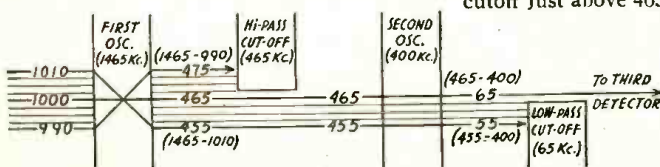
Fig. 4—Path of signals through the Griffin receiver's channels. Fig. 5, right—Hookup of the most essential parts of the circuit.
