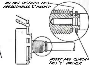
This pre-assembled "C" washer needs no adjustment—just insert and clinch it.
