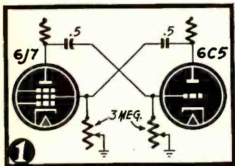
Fig. 1—Fundamental circuit of the device.
