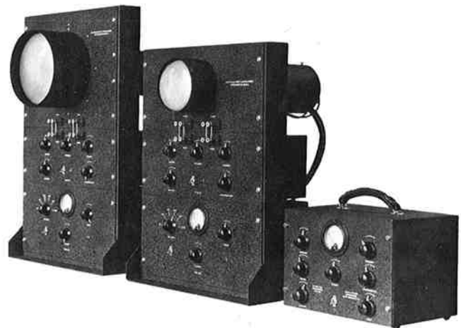
Early Du Mont oscillographs, built by Link Radio for the Allen Du Mont Labs in the 1933-35 period.
