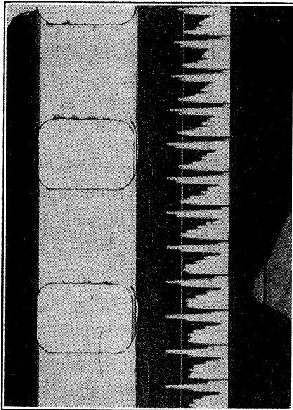
Fig. 19. Voice and piano fundamental approx. 450 cycles per sec.
