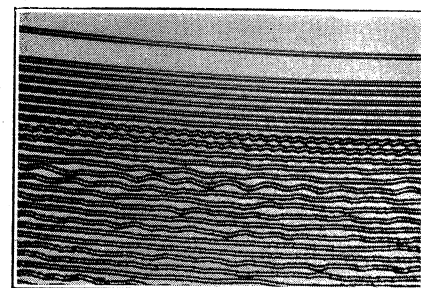
Fig. 18. Steam whistle approx. 1000 cycles per sec.
