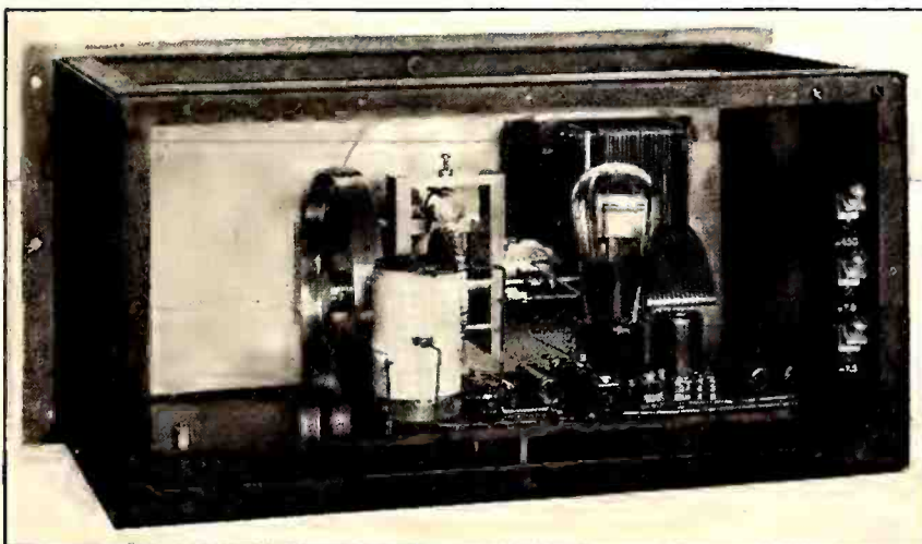
Rear view of the high-frequency oscillator panel.
