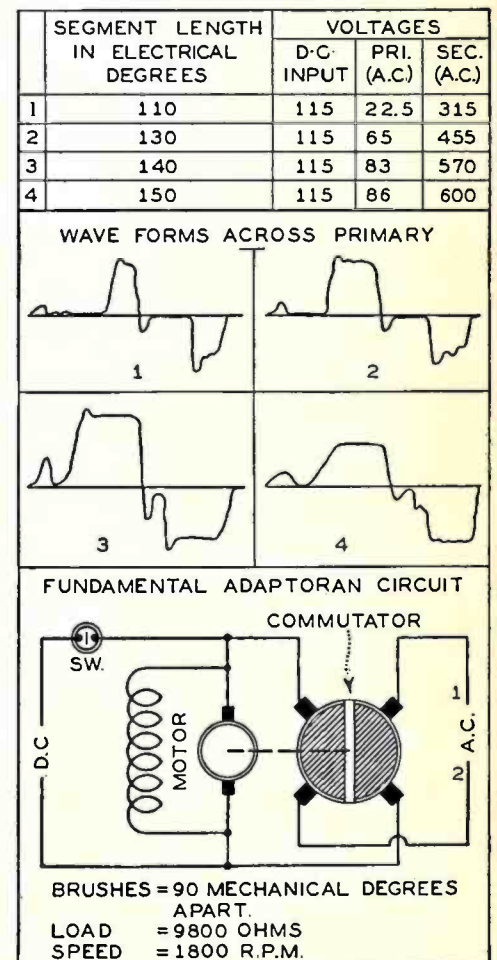
Fig. 4—Effect of varying length of commutator segments.
