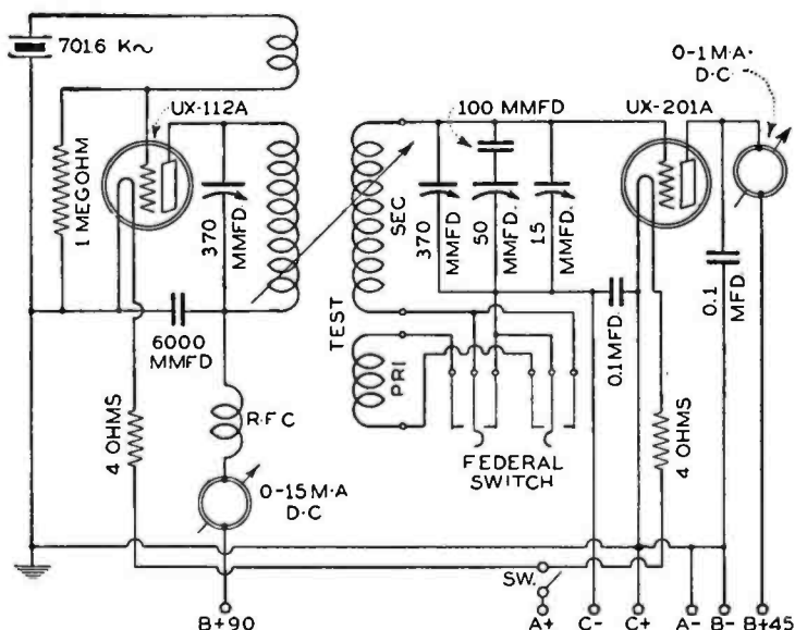
Fig. 1—Circuit for checking low-inductance r.f. transformers. A crystal oscillator supplies the power and the coil under test is connected in the grid circuit of the V.T. voltmeter tube. The secondary is first checked alone and then primary and secondary are connected, series aiding, to test both windings and the mutual inductance between them.
