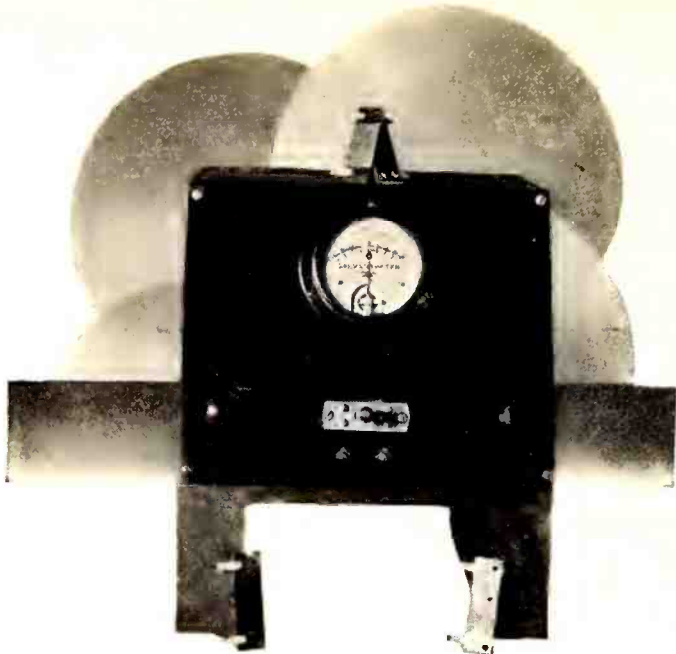
This device for measuring the resistance of wire-wound resistors within 1 per cent. is attached to each winding machine.
