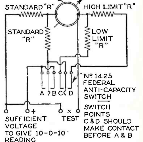
Fig. 4— Wire-wound resistors are checked within 1 per cent. by means of this bridge system which is attached to the winding machine. Changes in battery potential do not affect its accuracy.
