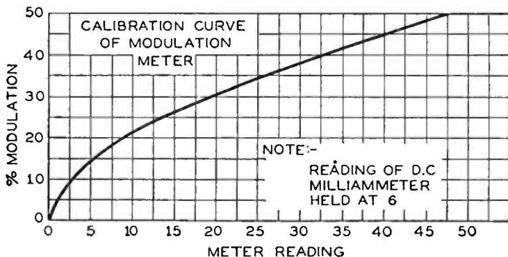
Fig. 3—Modulation meter calibration curve.
