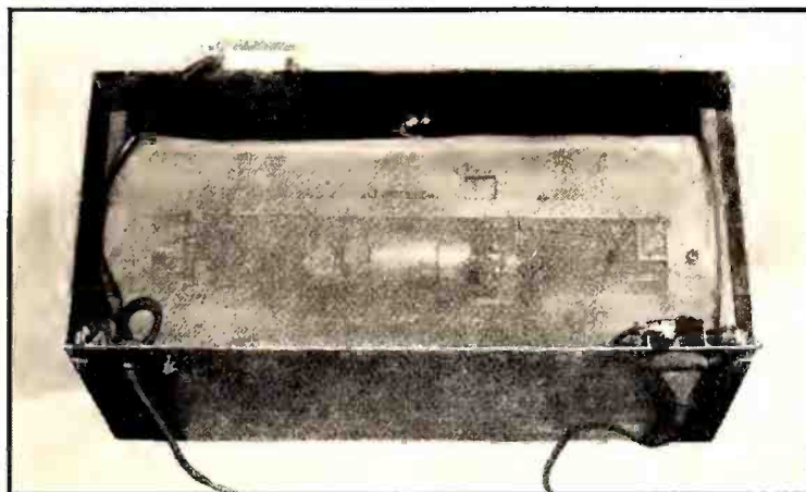
View of Adaptoron with front shield removed.
