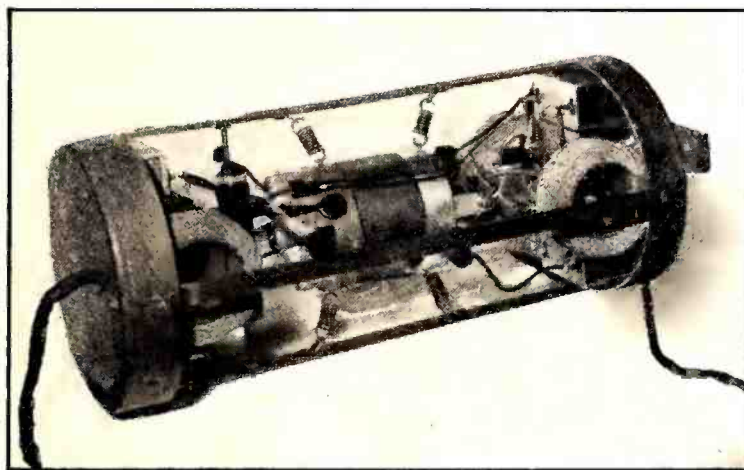
The Adaptoron chassis with both shields removed.
