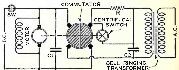
Fig. 2—The bell-ringing Adaptoron circuit.
