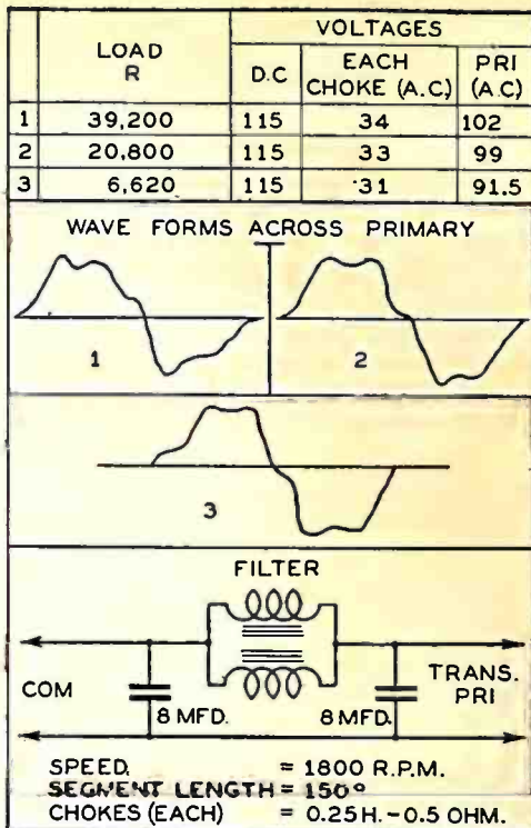
Fig. 8—Effect of varying load resistance.
