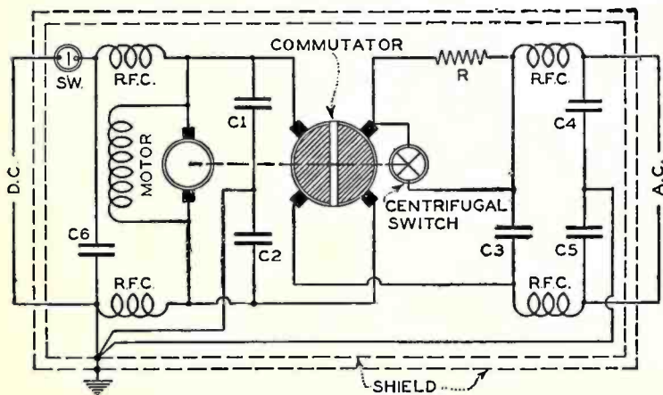
Fig. 3—The Adaptoron for radio use.
