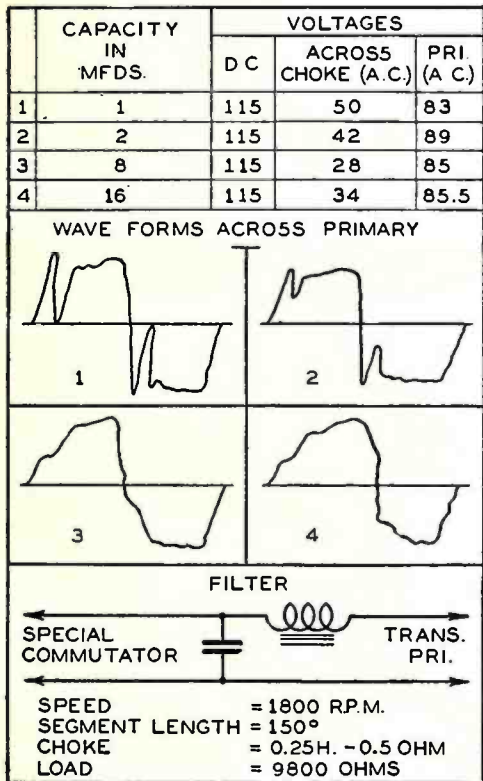
Fig. 5—Effect of parallel capacity and series inductance.
