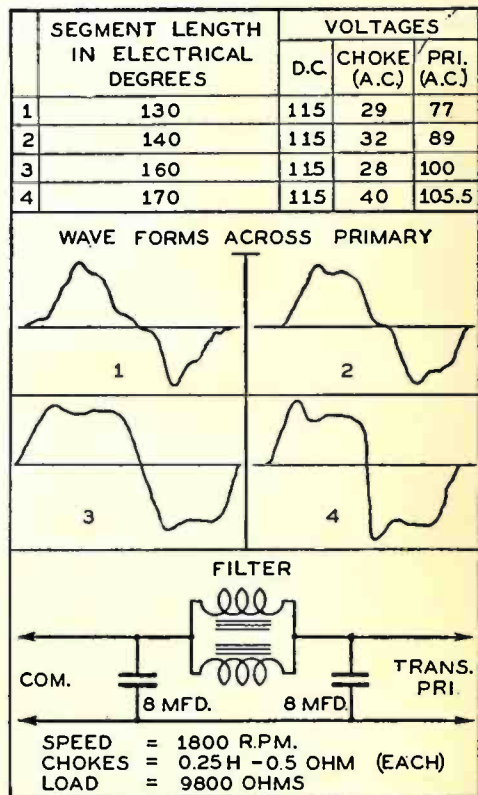
Fig. 9—Effect of changing segment length.
