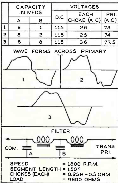
Fig. 7—Effect of different capacity combinations.
