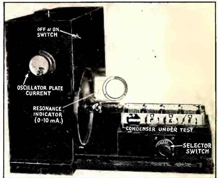
An instrument for rapidly testing gang condensers.
