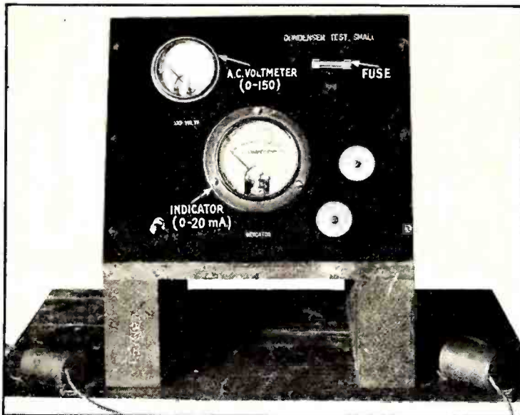
This apparatus measures the capacity of small by-pass condensers. The schematic diagram is shown in Fig. 5.
