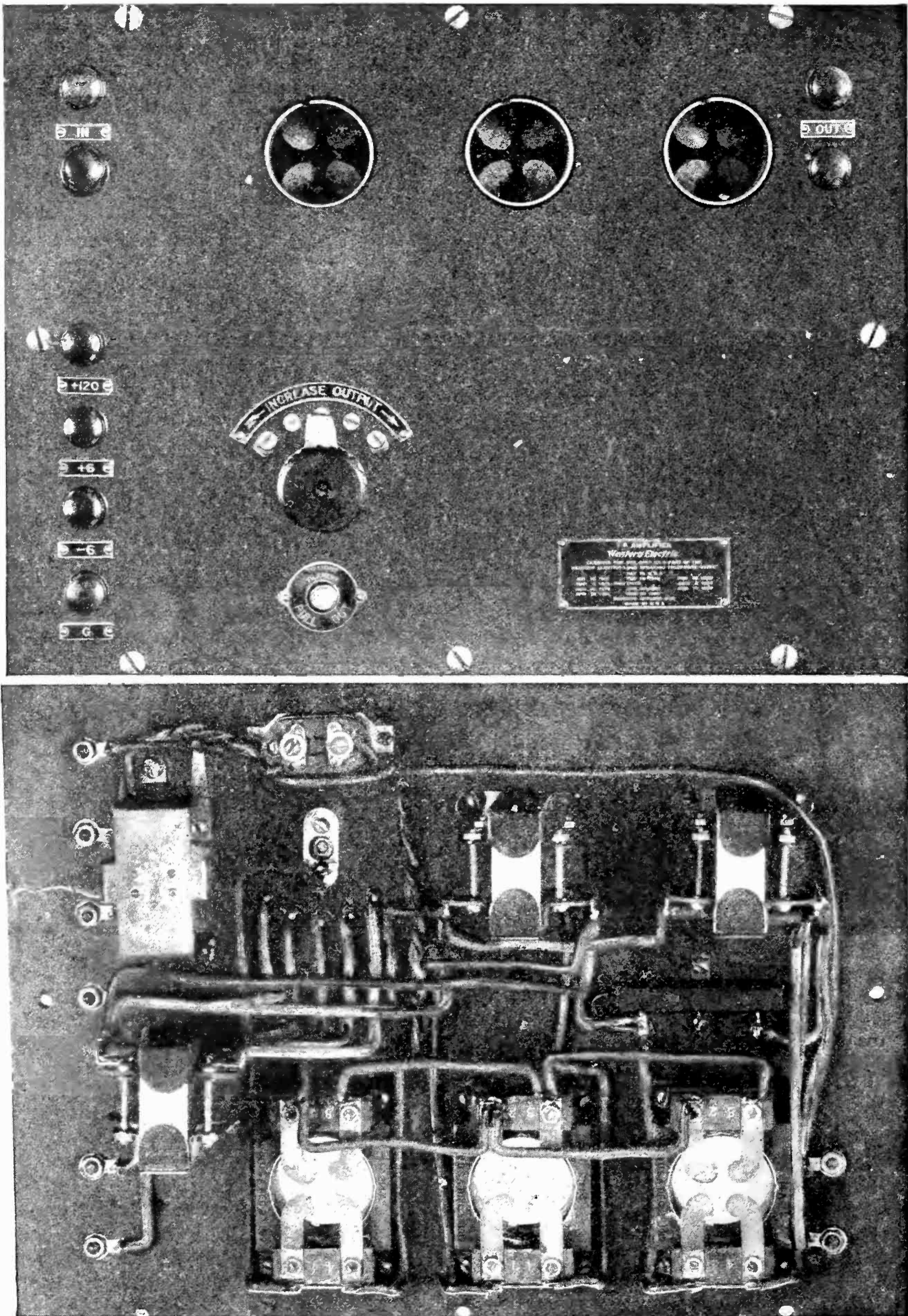
AN EARLY TYPE OF HIGH QUALITY PUSH PULL AMPLIFIER A front and rear view of one of the first high quality amplifiers to be put on the market. It is of the push-pull type, and made by the Western Electric Company
