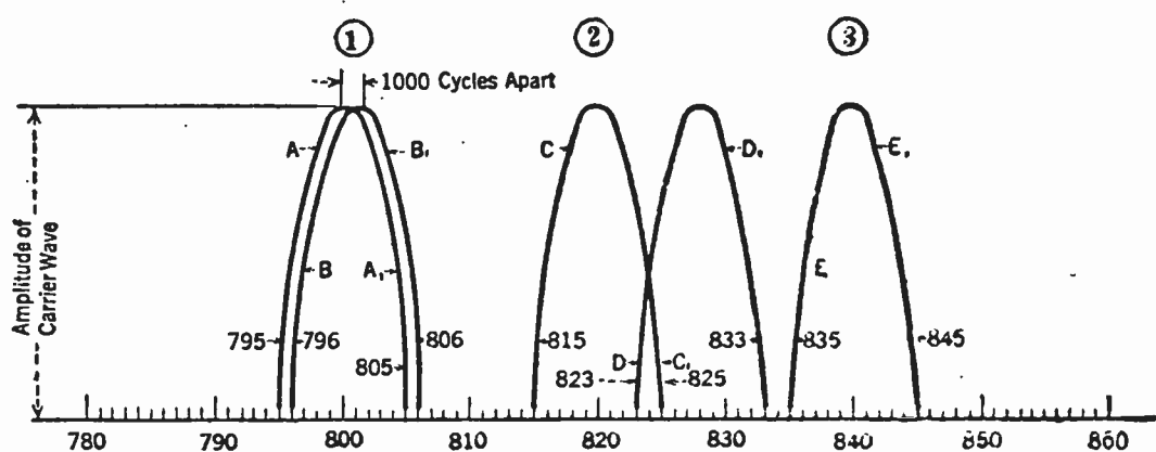
HOW BEAT NOTES ARE PRODUCED
