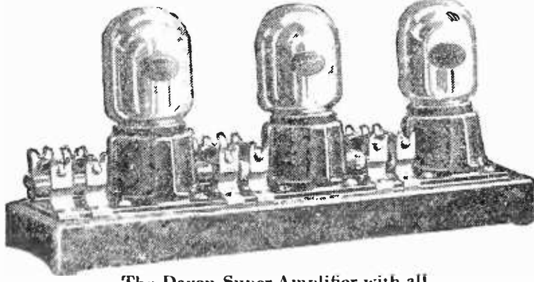
The Daven Super Amplifier with all labor of assembly eliminated $15.00
