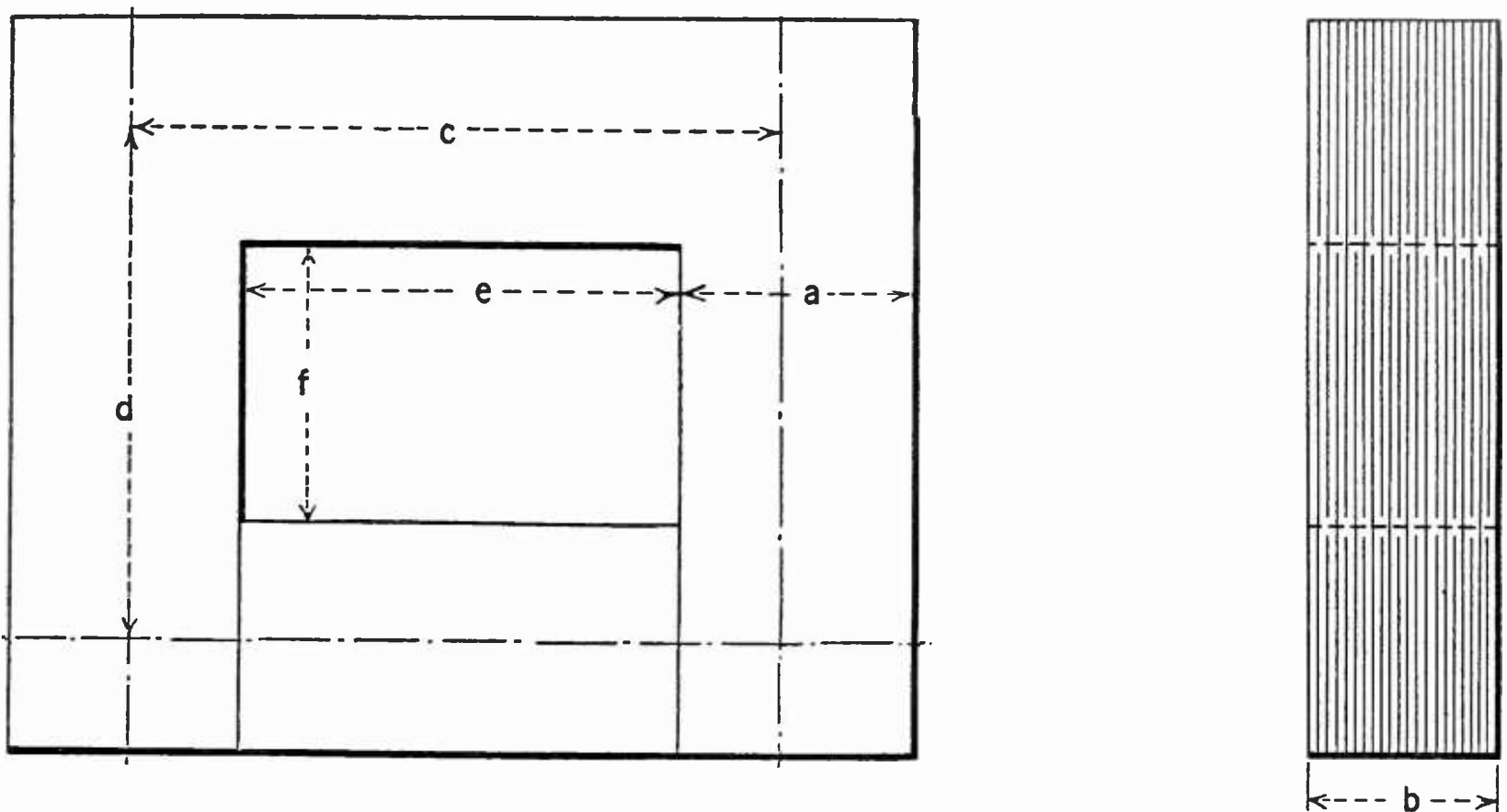
TRANSFORMER CORE
