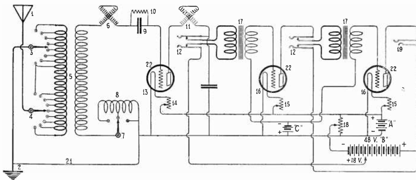
FIG. 5. CIRCUIT DIAGRAM FOR MR. BARTHOLOMEW'S COMPLETE RECEIVER
