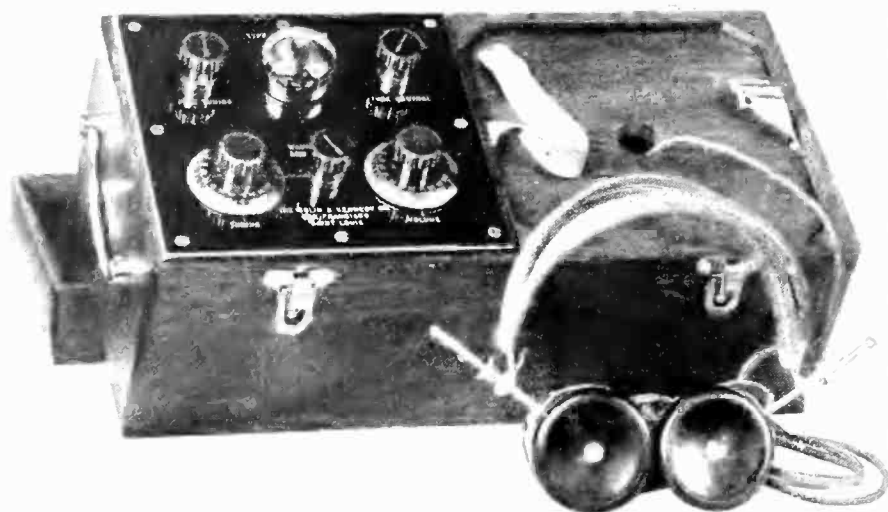
THE COLIN B. KENNEDY PORTABLE
