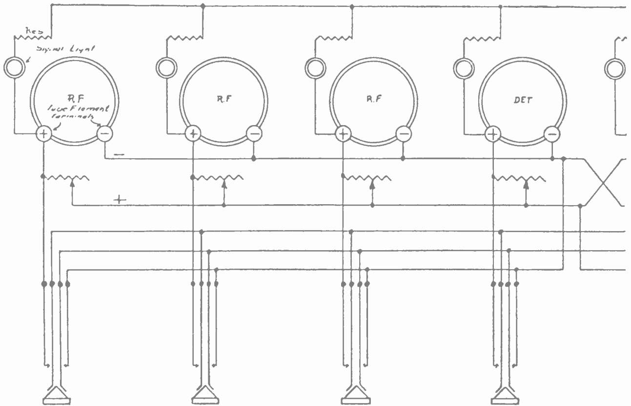
THIS DIAGRAM SHOWS THE VOLTAGE-CONTROL AND INDICATING-LIGHT—
