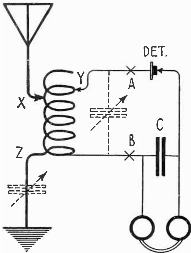
FIG. 2 An efficient and simpler circuit
