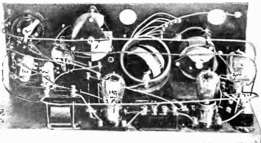
THE INVERSE DUPLEX SET MADE BY THE AUTHOR
