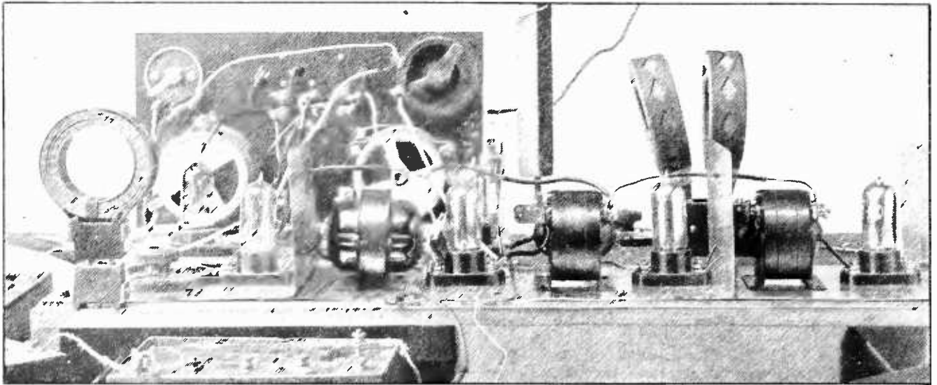
REAR VIEW OF THE EXPERIMENTAL SUPER-HETERODYNE SET
