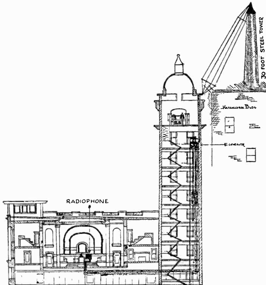
Drawing showing details of the radio installation
