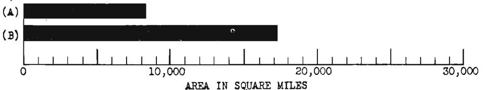
Fig. 4 Number of square miles inside 0.5 millivolt contour for (A) 1000 WATTS and (B) 5000 WATTS on 1000 kilocycles, average antenna efficiency and average conductivity.
