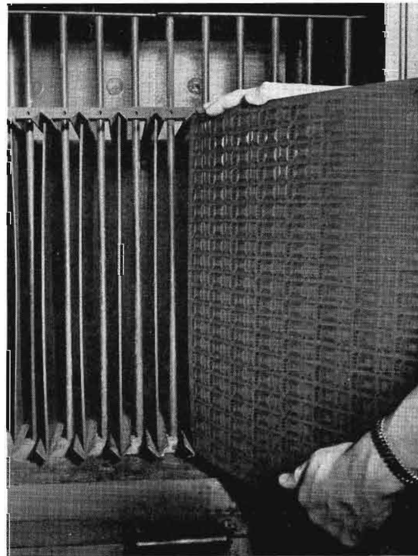
Here, the sheet of printed circuits, with all unwanted areas etched away by an acid bath, goes into a bake oven, as one of the final production steps.
