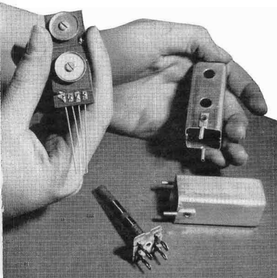
A complete printed circuit i.f. transformer and its shield (in hands) are compared with older type components (on table) to show comparative sizes.
