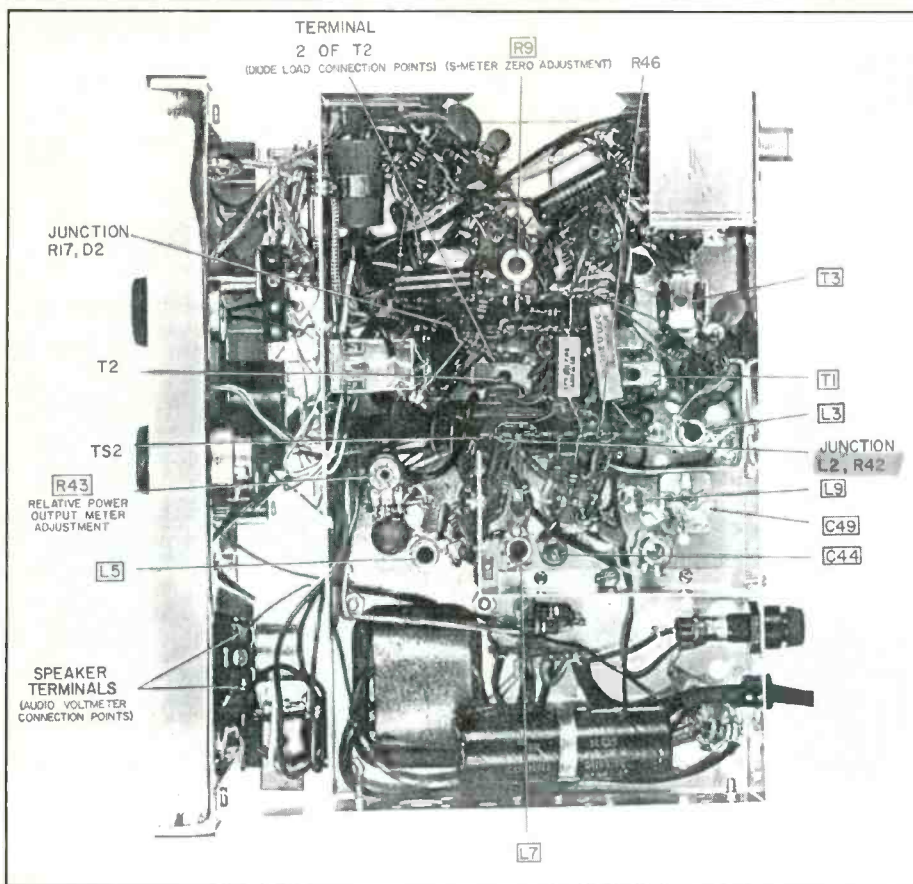
Figure 5. Top view of the alignment points. Both cores must be tuned from the top of the chassis.
