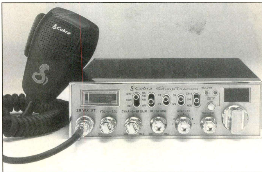
Cobra's 29 WX ST mobile CB includes the seven NOAA weather channels and features instant channel 9 or 19 access at the flick of a switch. (Courtesy Cobra Electronics Corp.)
