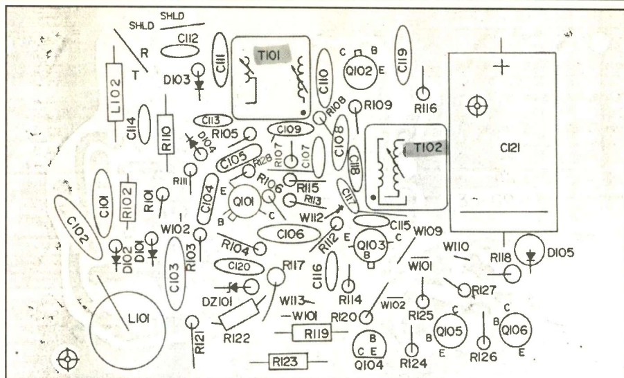
Figure 3. Tuning up the synthesizer.
