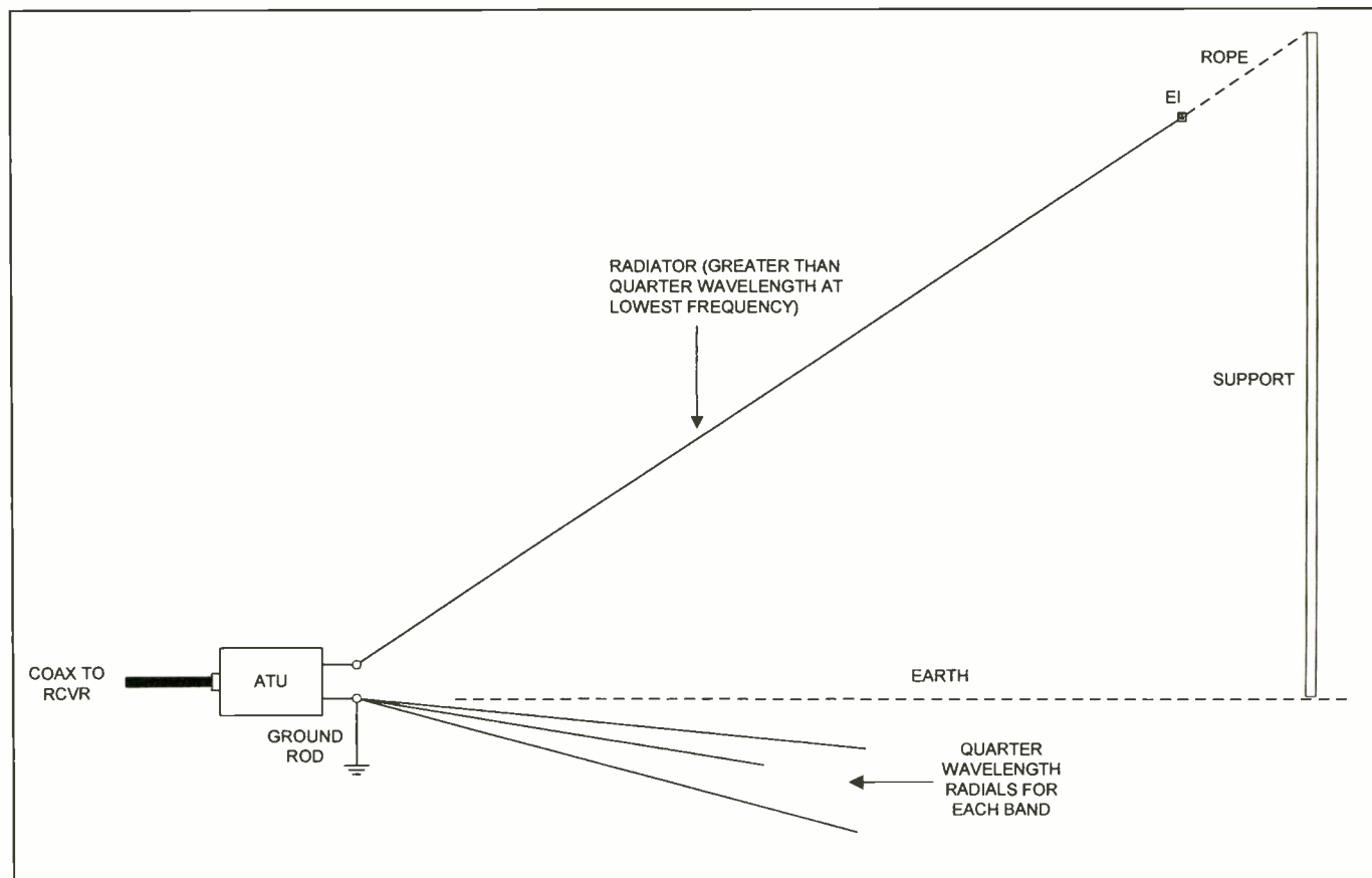
Figure 1. Random length, ATU-tuned multi-band antenna.
