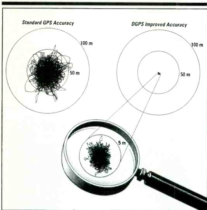
Differential beacon reception added to the GPS set improves GPS accuracy by 10 times! (Photo courtesy Leica)
