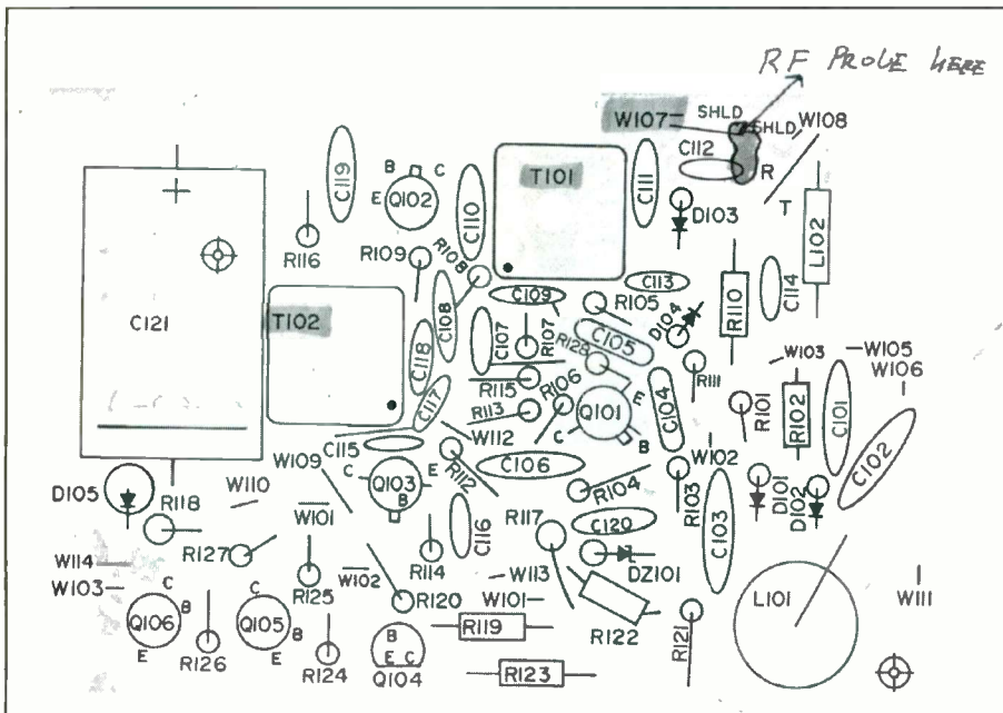
Figure 3a. Bottom view of the alignment and test instrument connection points.
