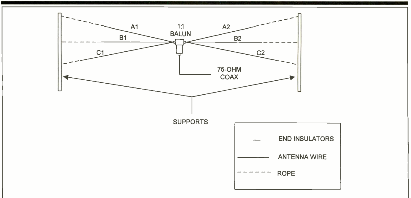
Figure 3. Multi-band dipole antenna.
