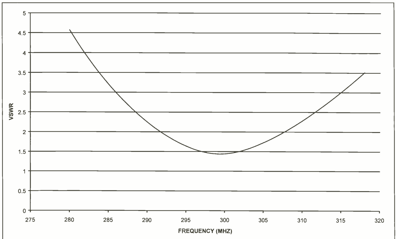
Figure 4. Typical VSWR curve.
