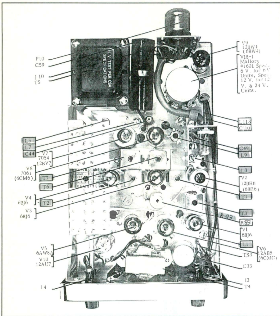
Figure 2: Top view of the Messenger II.
