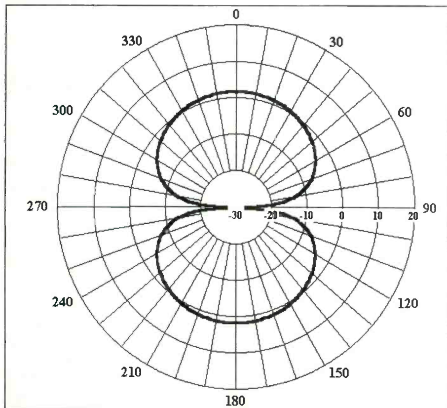
Figure 2. Figure-8 dipole horizontal pattern.
