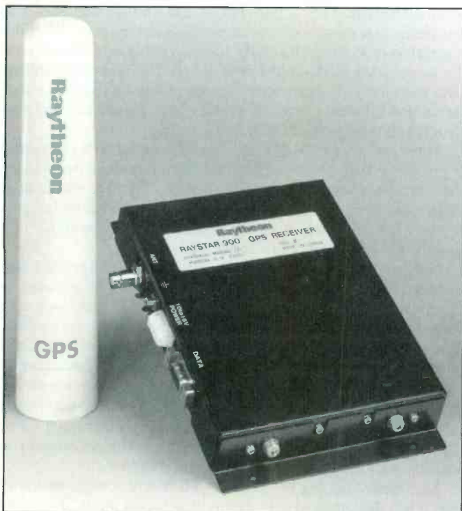
The "black box" differential GPS beacon receiver tunes 200 to 500 kHz for spot-on position accuracy. It plugs into the GPS NMEA port.
