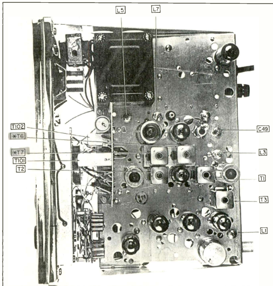
Figure 4. The frequency synthesizer board view from the foil side.
