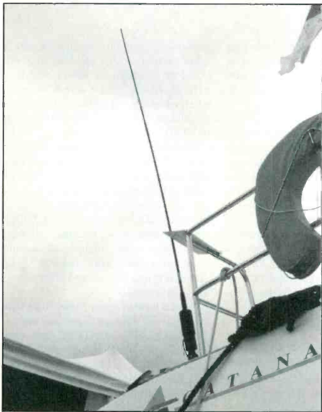
Low-frequency, base-loaded differential beacon receiver antenna system.
