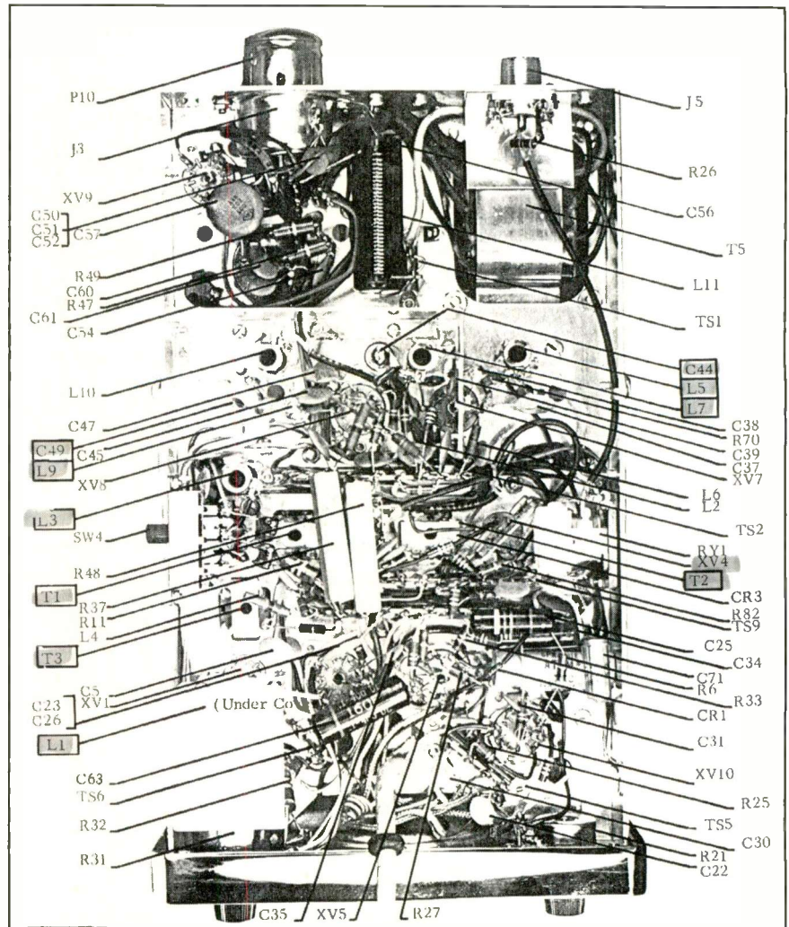
Figure 1. Bottom view of the Messenger II.
