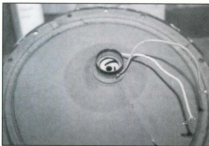
Some early speaker cones could be easily removed for service or repair. Note the voice coil bobbin at the rear. The spider centering support can be seen at the bottom of the voice coil.
