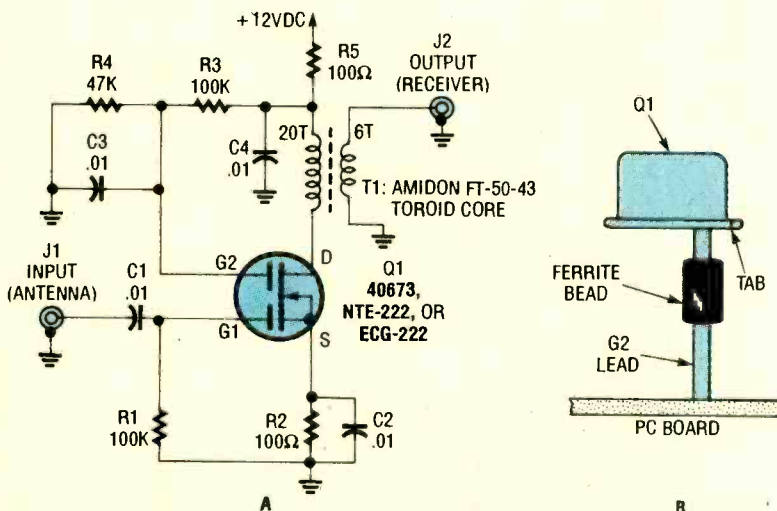
Fig. 2. This is a general-purpose HF preamplifier based on the 40673 MOSFET device. As shown, a ferrite bead should be placed on the G2 lead of Q1 to eliminate several possible problems.
