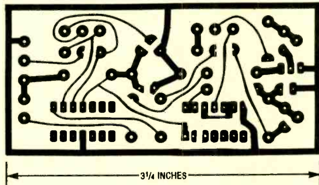
Fig. 11. The author's prototype was assembled on a small printed-circuit board that measures about 3\frac{1}{4} by 1\frac{1}{16} inches. A full-size template of that printed-circuit pattern is shown here.
