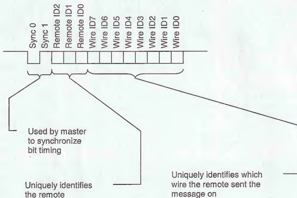
Fig. 10. Message bit format. Three bits are used to encode the remote unit's ID, and eight bits are used to indicate the wire number.
