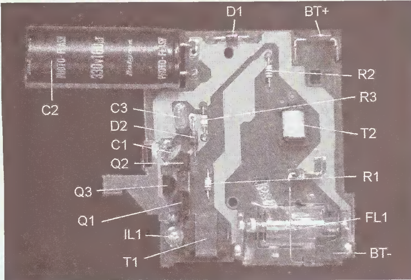
Fig. 2. This photo shows the top view of the flash circuit.
