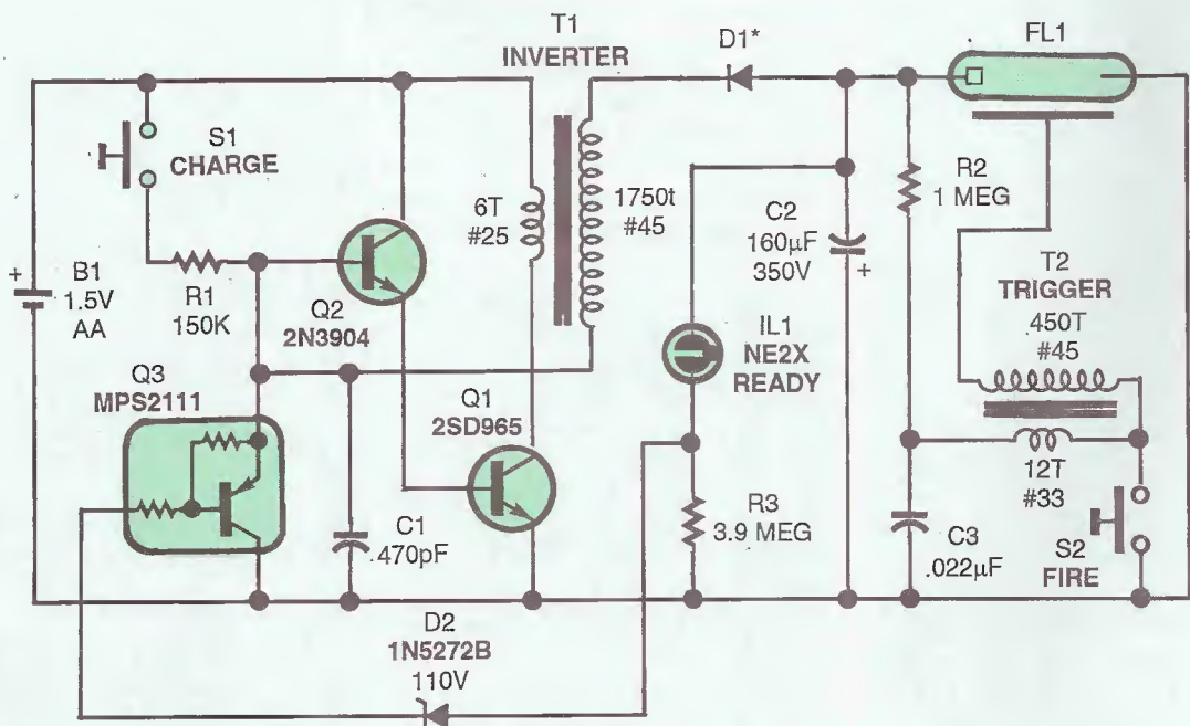
Fig. 1. The Kodak MAX single-use 35-mm pocket camera, with flash, has a flash unit that runs from a single 1.5 -volt alkaline cell and generates over 300 V DC for the flash tube.
