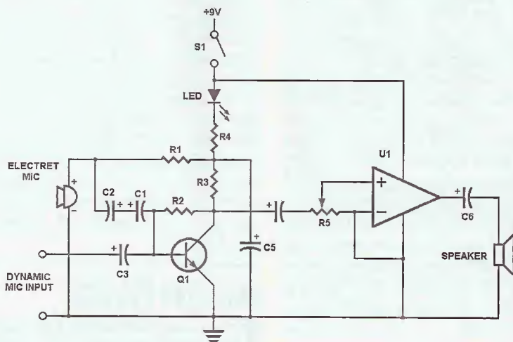
Fig. 1. This "generic" microphone pre-amp and output-amplifier circuit uses capacitors generously throughout the circuit for varying reasons.
