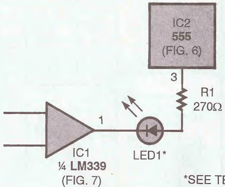
Fig. 8. A 555's output supplies the positive voltage for the LED during its timing cycle, and the oscillating LM 339 supplies the ground return for the LED's cathode.
