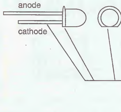
Fig. 17. LED Lead Identification. The flat side of the LED body and/or the short lead indicates the cathode.
