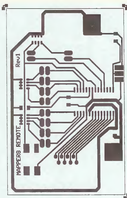
Fig. 13. Remote Unit Foil Pattern. A finished size of 3.15 inches by 1.97 inches will allow the board to be used as the cover of the case specified in the Parts List.
