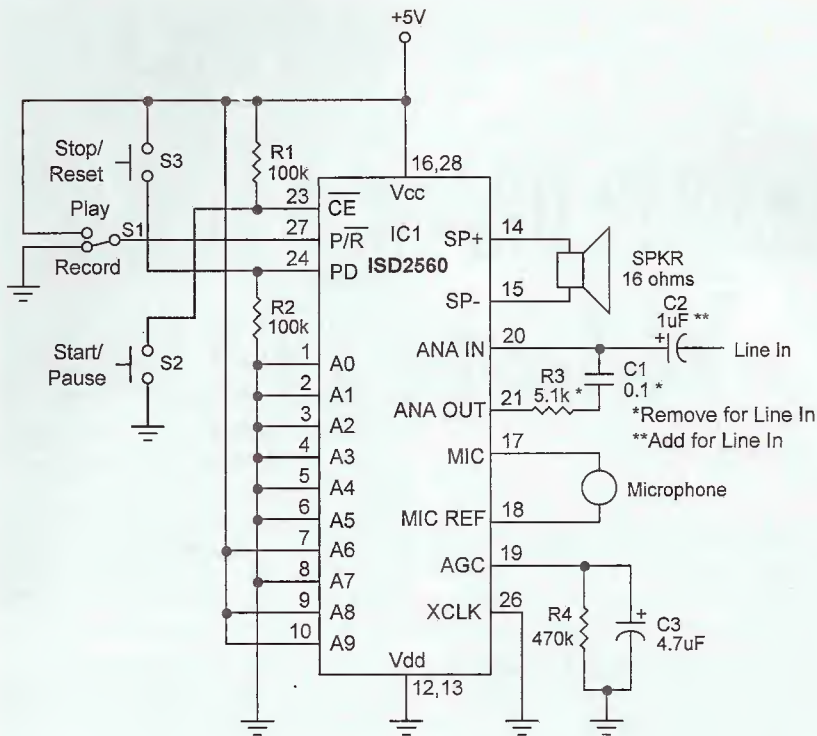
Fig. 3. This is a simple, push-button ISD2560 playback/recorder. The circuit is shown wired for a dynamic microphone input; for Line In recording alter the circuit as indicated.
