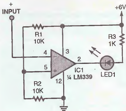
Fig. 3. In the inverting circuit configuration shown here, when the input at pin 4 is above 3 volts the output is low, and when below 3 volts the output is high. The LED is also turned on when the output is low.
