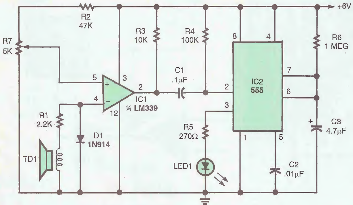
Fig. 6. This circuit offers a timed-on indicator using a super-bright LED. The comparator in this version is connected in an inverting configuration with a high output when no input signal is present.
