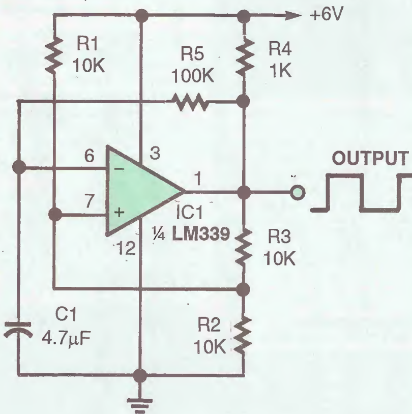
Fig. 7. The LM 339 comparator can easily be turned into an oscillator, as shown here. Components R5 and C1 form the RC timing network that sets the frequency.
