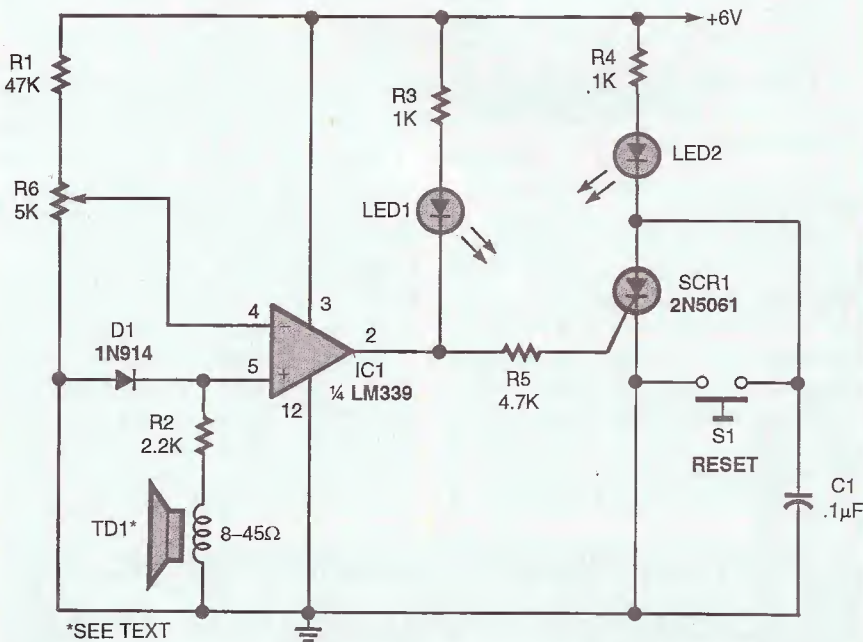
Fig. 5. Looking at this comparator circuit we see that the 5-k potentiometer (R6) sets the input sensitivity from 0 to near 600 millivolts. Diode D1 protects the comparator's input from a negative input pulse greater than .6-volts.
