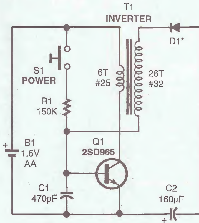
Fig. 6. By rewinding the inverter transformer, any output voltage up to about 350 V DC can be obtained from a 1.5-volt alkaline cell.
