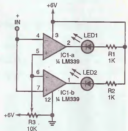
Fig. 10. The inputs of two comparators can be cross connected, as shown in this circuit, to produce dual and opposite outputs. By using this arrangement both a timed and a latched output can be produced in one target circuit.
