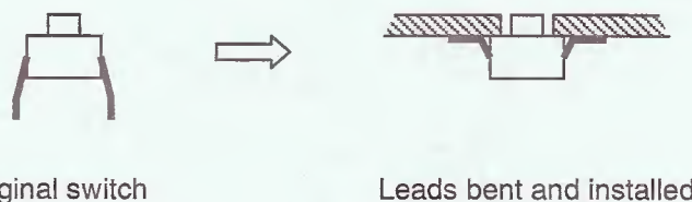
Fig. 16. Bend the four leads of SW2 as shown and surface mount it to the "inside" of the board.
