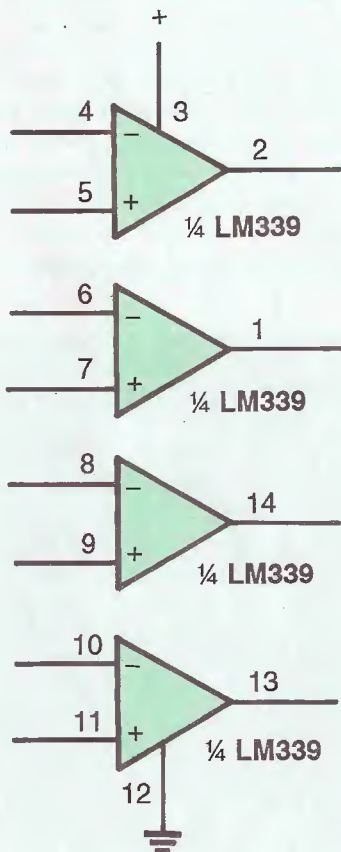
Fig. 1. There are four independent voltage comparators in the 14-pin package. The LM 339's pin out is shown above. Note that pin 3 is positive and pin 12 is ground.
