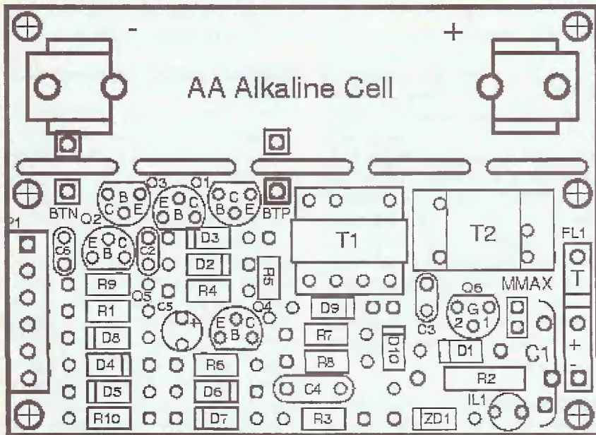
Fig. 5. Here is the PCB Layout shown at 200%.
