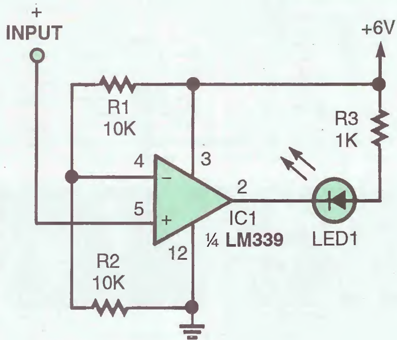
Fig. 2. In this non-inverting comparator-circuit configuration, when the input voltage at pin 5 is above 3 volts the output is high, and when below 3 volts the output is low. The LED is turned on when the output is low.
