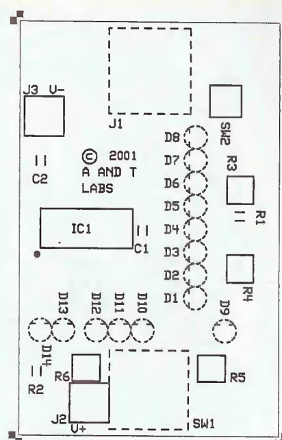
Fig. 14. Master Unit Parts Placement Diagram. Solid outlines indicate where components are surface mounted and soldered to the trace side of the board. Dashed outlines indicate where through-hole components are mounted on the opposite side.
