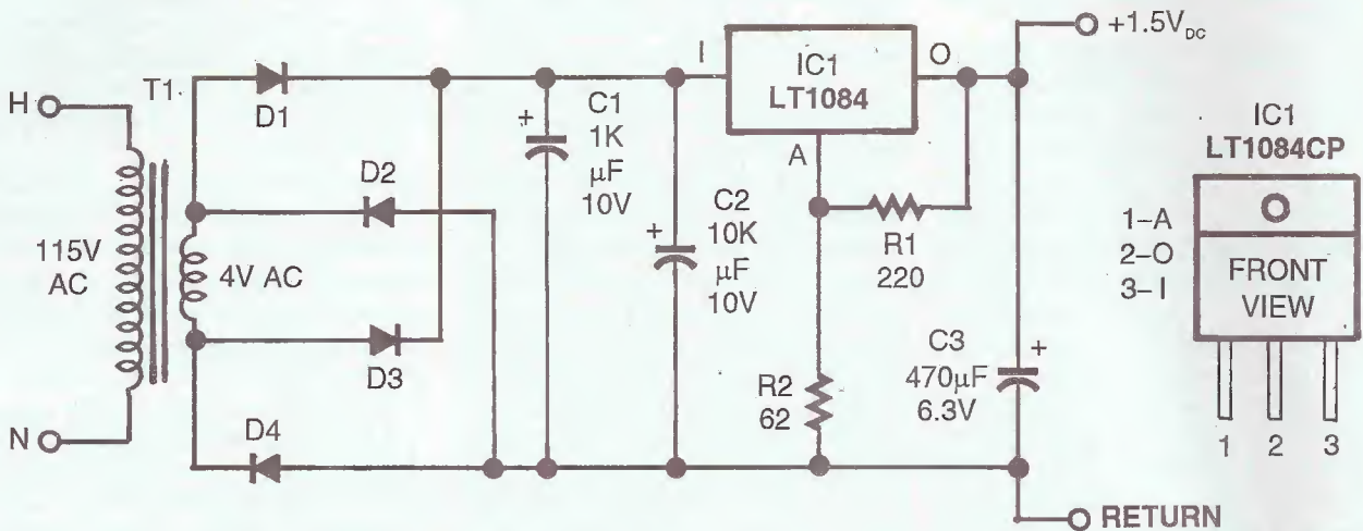
Fig. 7. The regulator (IC1) is an LT1084CP, which is similar to an LM317 but is a low-dropout type rated at 5 A max.
