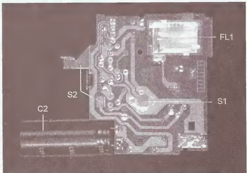
Fig. 3. Here is a photo of the flash circuit that shows the bottom-mounted components.
