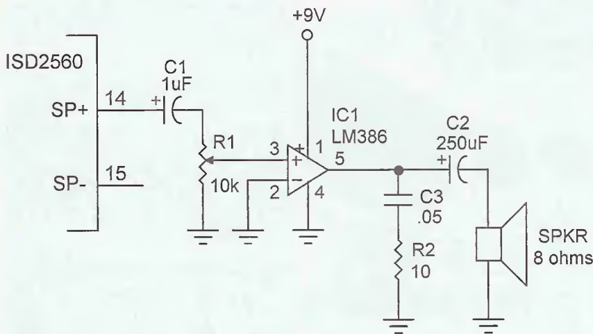
Fig. 2. The audio output of the ISD2560 is a weak 12.5-mW. This circuit boosts the volume by 20 fold. For louder sounds, place a 10-µF capacitor across pins 1 and 8.
