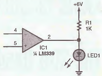
Fig. 4. This circuit modifies the comparator's output to reverse the LED on/off function. This easy change can be beneficial when using the output as an indicator.
