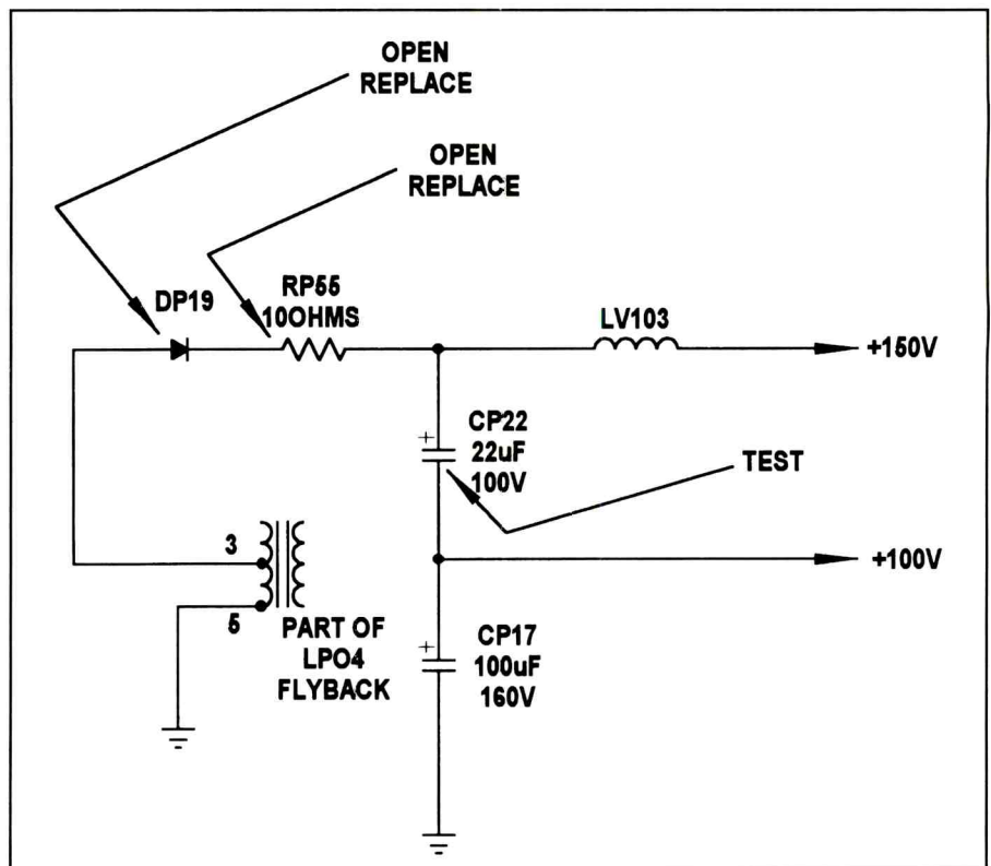
Figure 6. If the symptom is excessive brightness followed by shutdown, replace DP09 and RP55.
