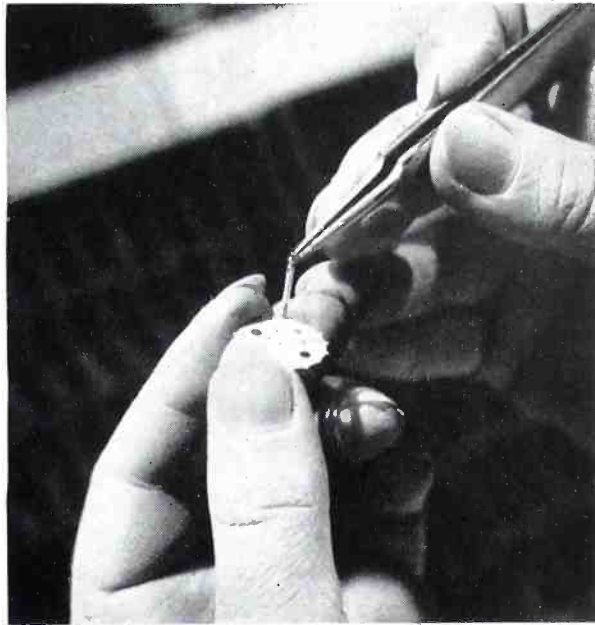
5 Assembling coated cathode on a mica base is the first operation. Deft fingers and a steady hand are required for this and the succeeding operations.
