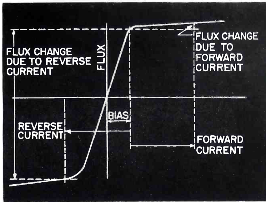
Figure 2 — Graph showing high ratio of sensitivity to reverse as compared to forward currents, achieved by use of saturated permalloy tape for the core.
