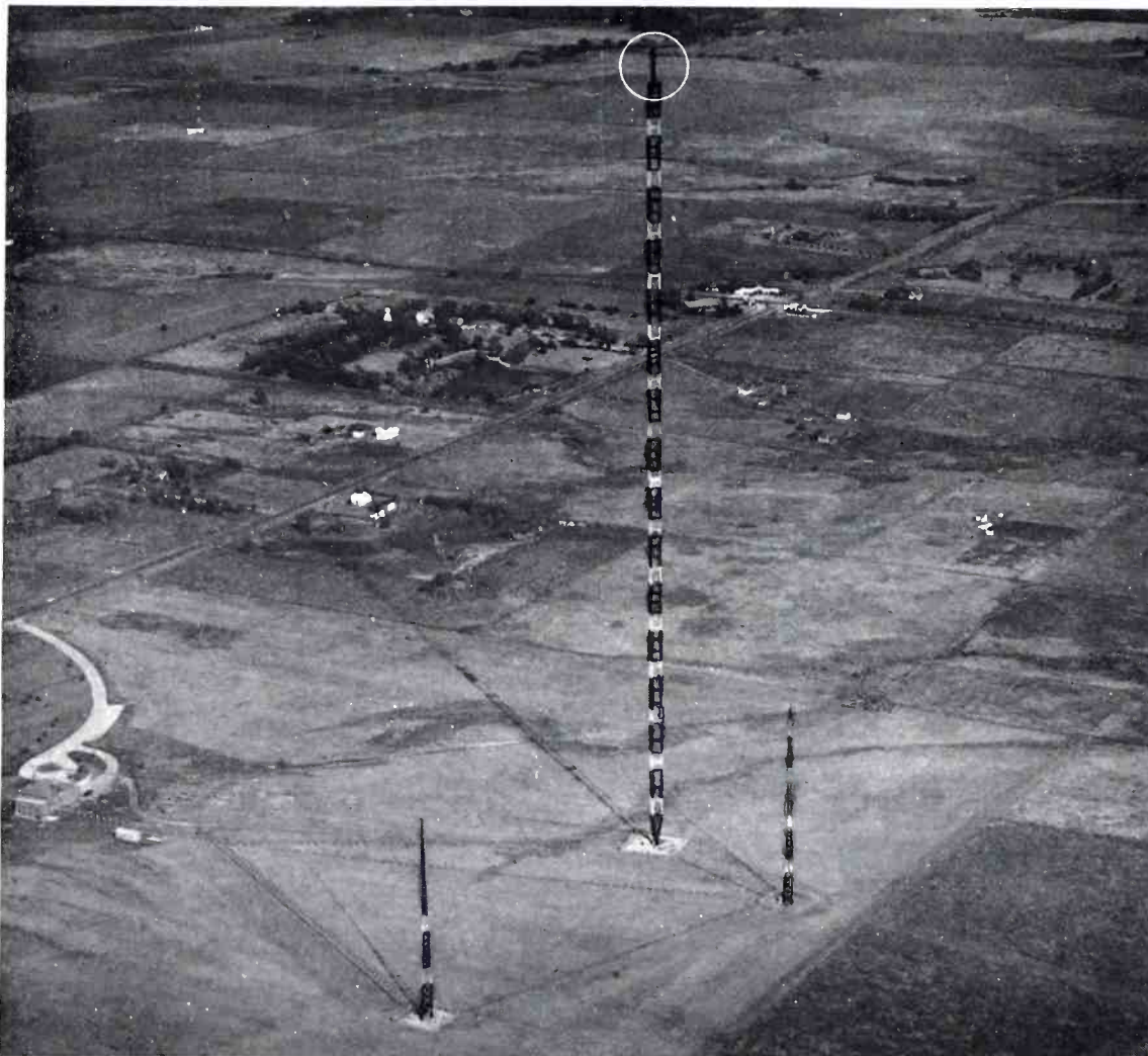
Dwarfing the two 250-foot antennas nearby, WKY's giant 959-foot antenna tower structure — tallest in the land — stands with its Clover-Leaf and airplane beacon aloft. Raising of Clover-Leaf took only one day.
