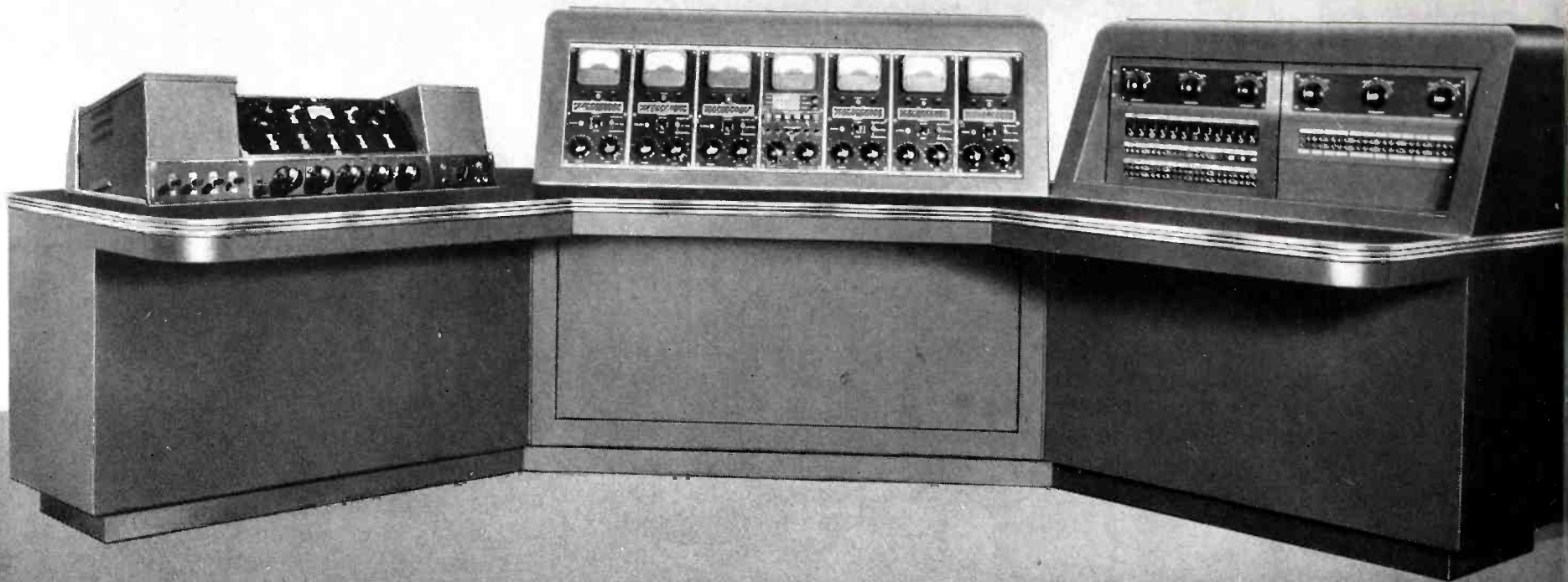
Console for new Master Program Dispatching System at WHDH. In center section is the Relay Type Program Dispatching equipment, composed of a Group Release Unit and six line units. Section at right is an Auxiliary Panel. Left is a Western Electric 23C Speech Input Console, used for the control of Studio 1.
