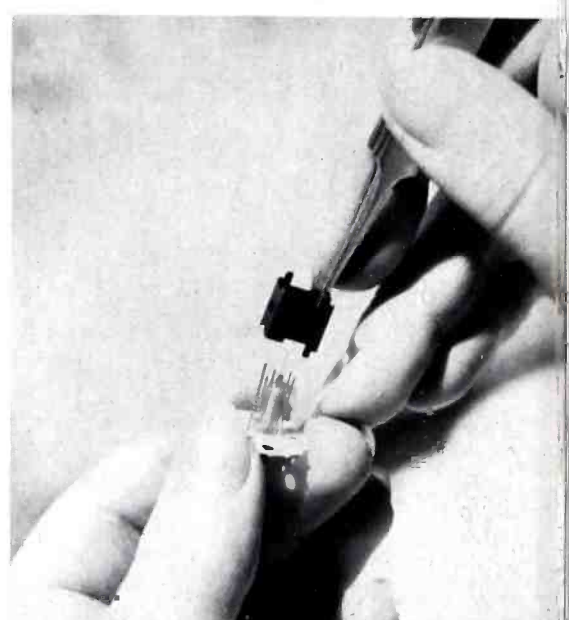
8 In another delicate operation, rectangular metal anode is lowered into its position on the mica base around the assembled cathode and grids.
