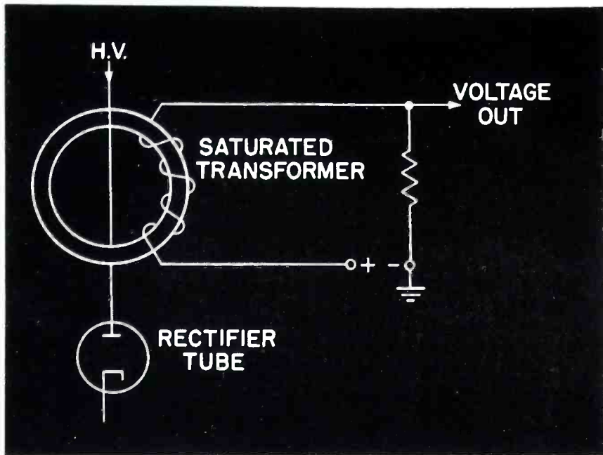
Figure 1 — Toroidal core — saturated by running small d-c through multi-turn secondary at ground potential — is responsive only to reverse currents in tube.
