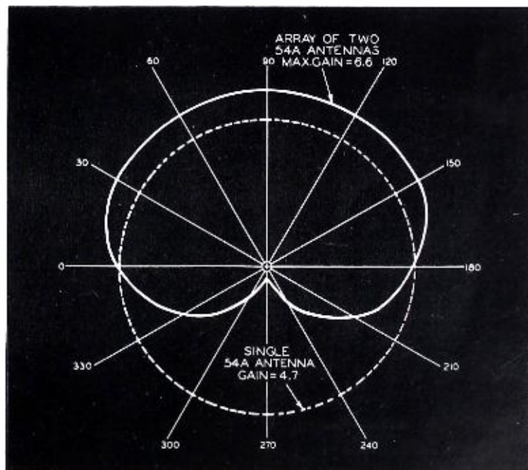
Maximum array gain is 9.4. Figure 2 (right) is a useful pattern where transmitter site lies near one side of area to be served. Maximum array gain here is 6.6.
