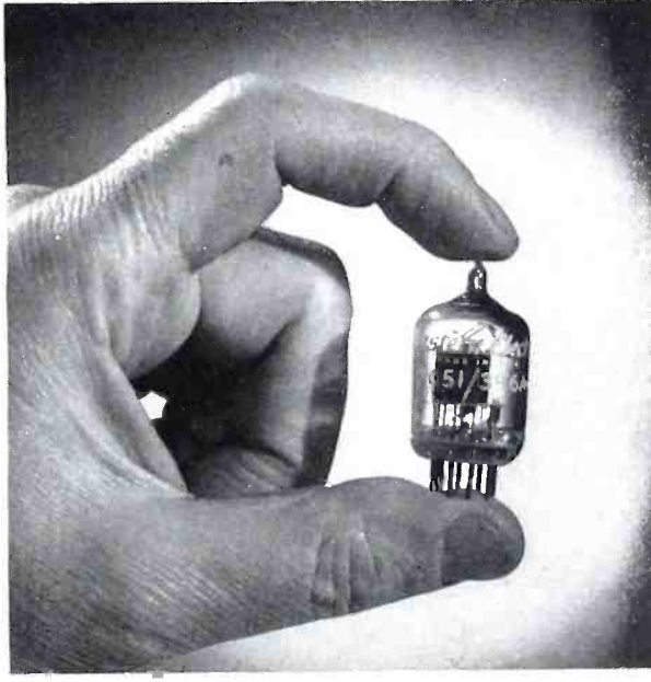
17 A finished miniature tube—manufactured carefully, tested thoroughly and aged properly—ready to go to work in a countless variety of electronic circuits.
