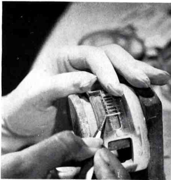
1 Preparation of components is the first step. Here cathode elements, with welding tabs attached, are assembled in a jig prior to spraying.
