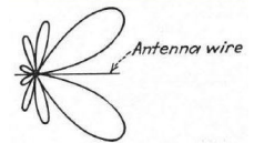
Figure 1: Long Wire Sensitivity Pattern
