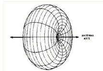
Figure 2: Short Random Wire Sensitivity Pattern
