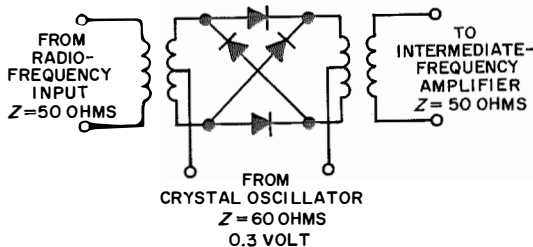
Figure 4—Diagram of ring modulator.
