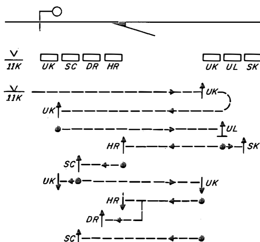
Figure 7—Typical sequence of operations for circuits in Figure 6.
