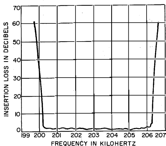
Figure 11—Insertion loss of a single-sideband electro-mechanical filter for use at a carrier frequency of 200 kilohertz.
