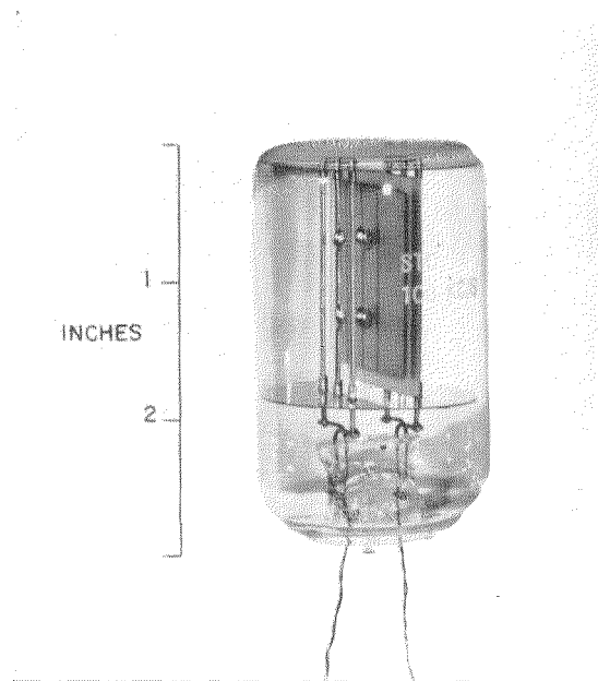
Figure 2— GT -cut resonator at 100 kilohertz.
