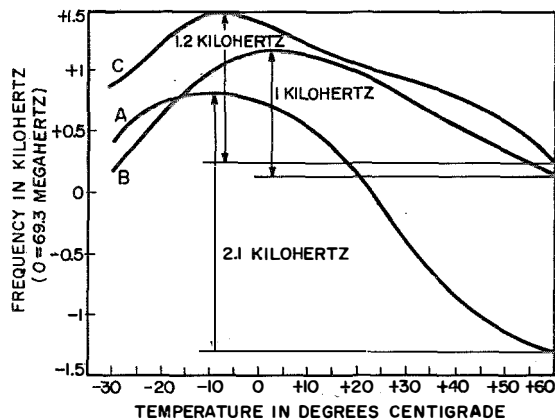
Figure 8—Frequency variation of typical crystal oscillator as a function of temperature. Curve A shows the variation of the crystal alone, curve B of the crystal-oscillator circuit with maximum compensation, and curve C of the same circuit using economically acceptable compensation.
