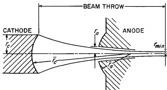
Figure 1—Beam parameters.
