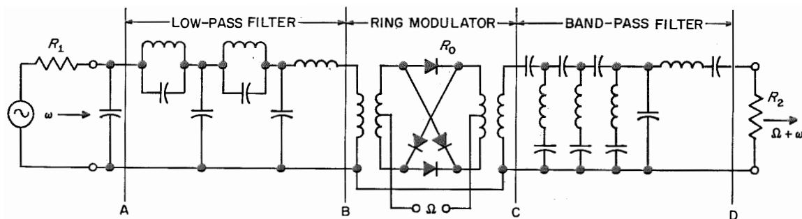
Figure 1—Selective frequency translator.
