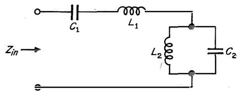
Figure 4—Equivalent electrical circuit of a mechanically coupled pair.
