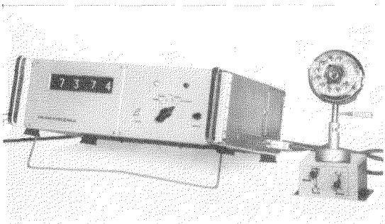
Figure 4—Time measuring set for telephone-dial inspection.
