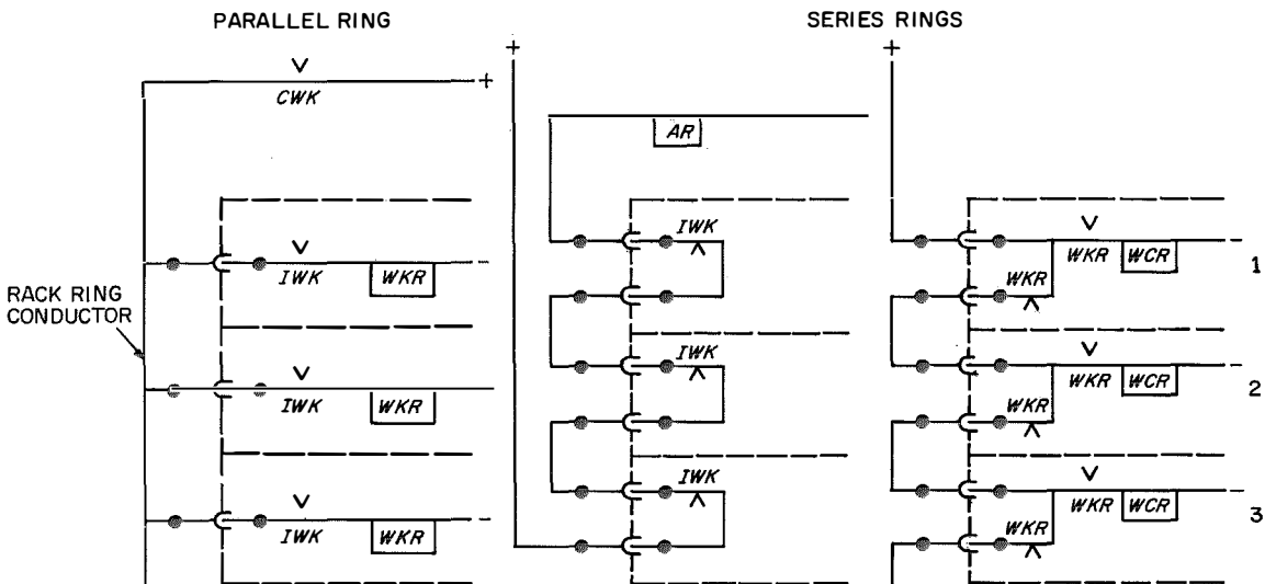
Figure 10—Ring conductors.
