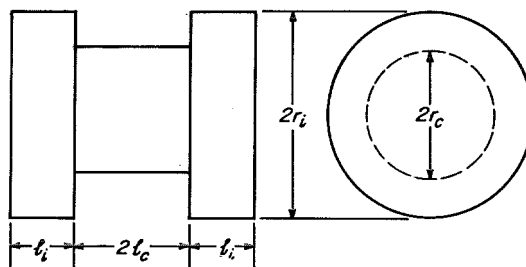
Figure 2—Mass-loaded resonator.
