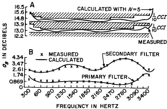
Figure 6—Calculation and measurement of the transmission loss as a function of frequency of (A) the entire translator pass band, and (B) of the primary and secondary filters separately with resistance terminations. The two areas delineated by the shaded regions (in which the curves of (A) lie) correspond to 1/10 of the maximum distortion permitted by the recommendations of the Comité Consultatif International Télégraphique et Téléphonique (1/10 CCI).
