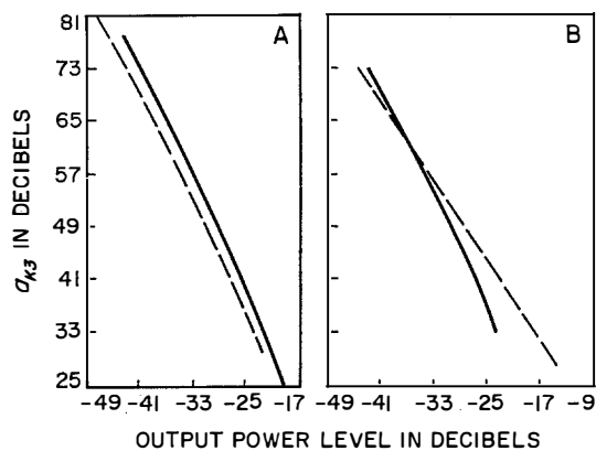
Figure 11—Measured attenuation of third harmonic a_{K3} plotted against translator output for ( A ) conversion from low to high frequency, and for ( B ) conversion from high to low frequency. The solid curves are with linearizing resistors and the broken curves are without linearizing resistors.
