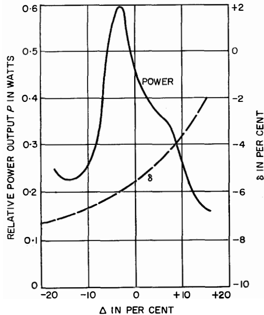
Figure 7—Theoretical tuning curves for \alpha_0 = 0.2 and \alpha_1 = 0.4 .
