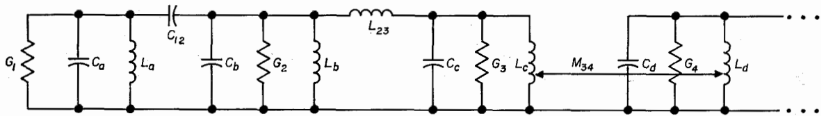
Figure 4A—Node networks using parallel resonant circuits. Each node Q is given by Q_r = R_r/X_{0r} , where the node capacitance (or inductance) is the capacitance or inductance existing across a node when all other nodes are short-circuited. For the three types of coupling shown: K_{12} = C_{12}/(C_1C_2)^{1/2} , K_{23} = (L_2L_3)^{1/2}/L_{23} , and K_{34} = M_{34}/(L_3L_4)^{1/2} . Any adjacent pair of resonators may be coupled by any of the three methods shown and then equivalent T's can be substituted for capacitive or inductive \pi 's if advantageous. Each node must resonate at f_0 with all other nodes short-circuited.
