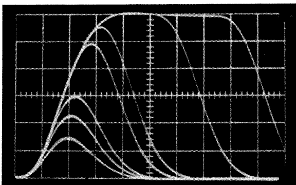
Figure 7C—Filter output as a function of pulse input width (constant input amplitude). The input pulse widths are 1.5, 1.0, 0.50, 0.40, 0.20, 0.15, and 0.10 microsecond. Sweep speed was 0.18 \pm 10 percent microsecond per centimeter.
