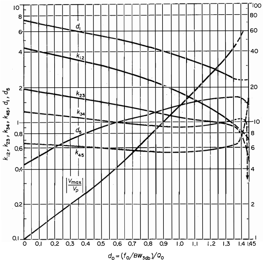
Figure 5—Minimum-transducer-loss 3-decibel-down normalized k 's and q 's required to produce an n = 5 gaussian-approximation amplitude shape. d = (f_0 / BW_{3db}) / Q and k = K / (BW_{3db} / f_0) .
