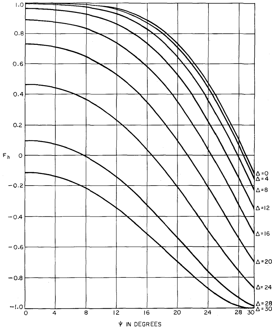
Figure 11—Variation of F_{h_s}(\Delta, \psi) as a function of the azimuthal angle \psi for different values of angle of elevation \Delta in degrees and for s_i/\lambda = 4 .
