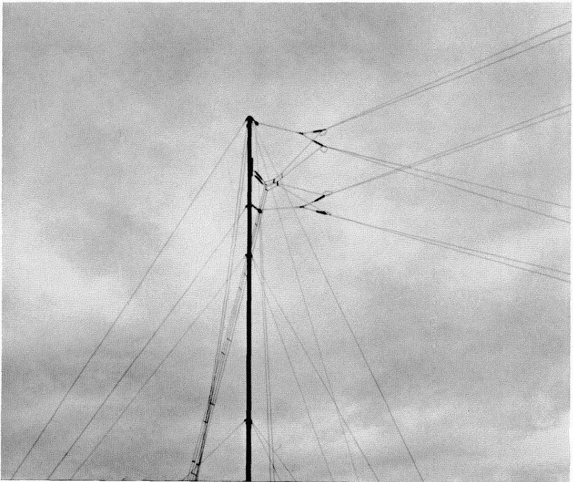
Figure 4—Four-wire down-lead transmission line and driving arrangement in stacked rhombic array.
