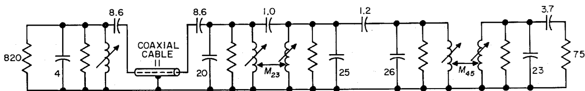
Figure 8B—An exactly equivalent network described in section 7.2 enables a piece of coaxial cable to be incorporated in the K_{12} circuit.
