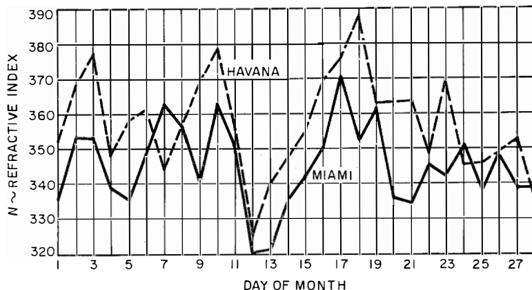
Figure 2—Surface refractivity, 19:00 Eastern Standard Time, February 1955; at Miami and Havana. The correlation coefficient is 0.60.
