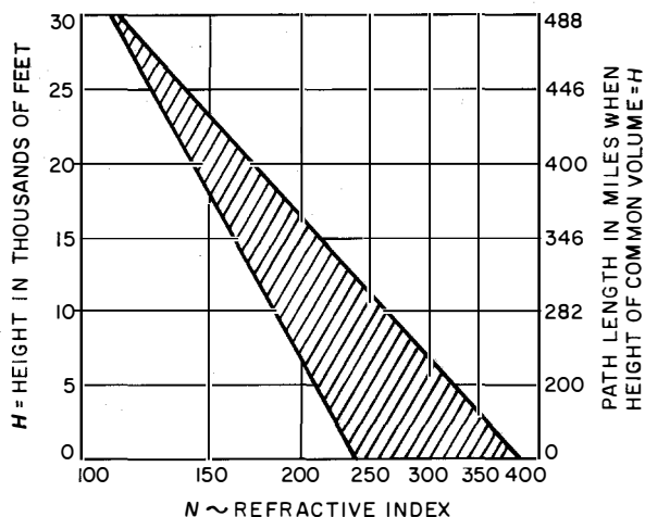
Figure 1—Variation of refractive index with height.
