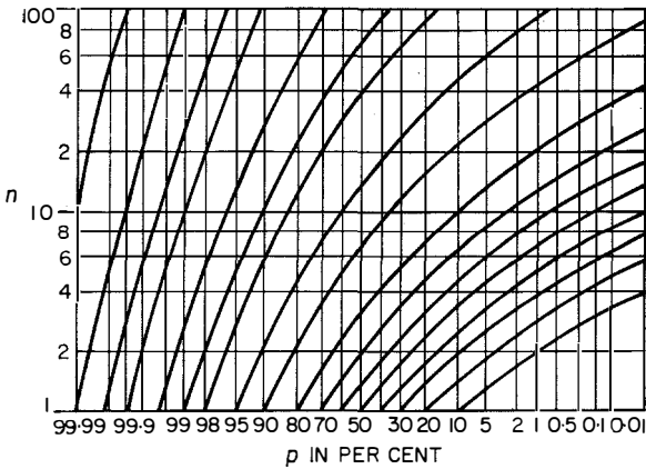
Figure 4—Curves for transforming probability scales. Used in connection with (19) for statistical summation; z_n = p^n .
