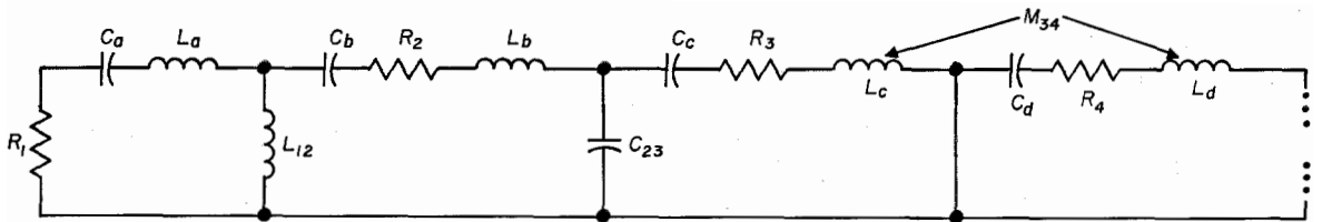
Figure 4B—For mesh networks using series resonant circuits. Each mesh Q is given by Q_r = X_{0r}/R_r , where the mesh inductance (or capacitance) is the resultant capacitance in series with a mesh when all other meshes are open-circuited. For the three types of coupling shown, K_{12} = L_{12}/(L_1L_2)^{1/2} , K_{23} = (C_2C_3)^{1/2}/C_{23} , and K_{34} = M_{34}/(L_3L_4)^{1/2} . Any adjacent pair of resonators may be coupled by any of the three methods shown; then, if advantageous, equivalent \pi 's can be substituted for capacitive or inductive T's. Each mesh must resonate at f_0 with all other meshes open-circuited.
