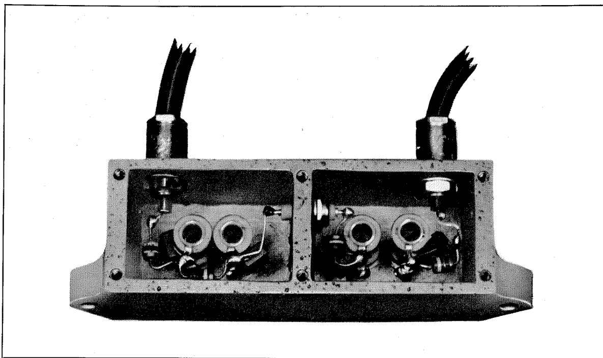
Figure 9—An embodiment of the 70-megacycle band-pass 5th-order gaussian-approximation filter synthesized in the band-pass design example of section 7.2. The first resonator of this filter is contained in another unit.
