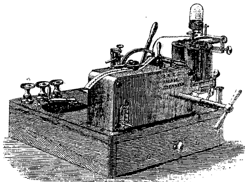
Figure 4—Undulator (Lauritzen's Undulating Inkwriter).
