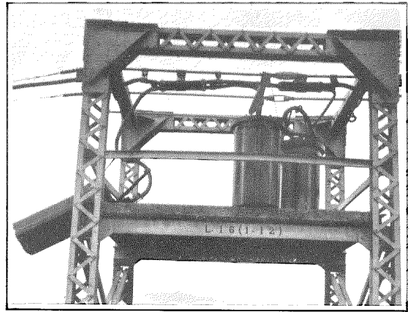
Figure 4—A Loading Coil Case Which Barely Escaped Dropping Down from the Tower.
