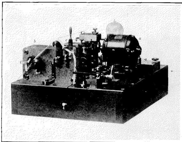
Figure 6—Motor-driven Undulator.
