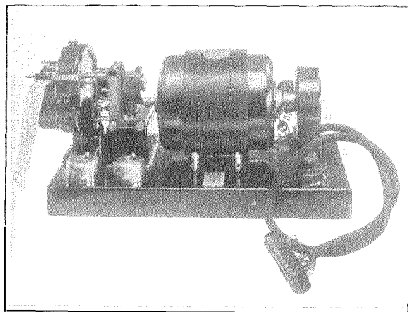
Figure 15—Teleprinter Auto-transmitter.
