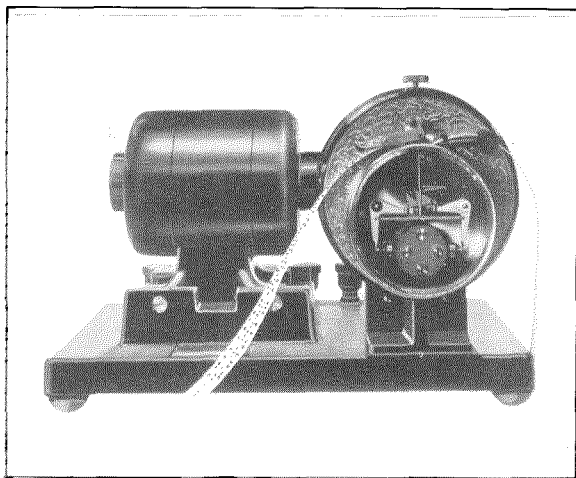
Figure 10—Morse Transmitter.
