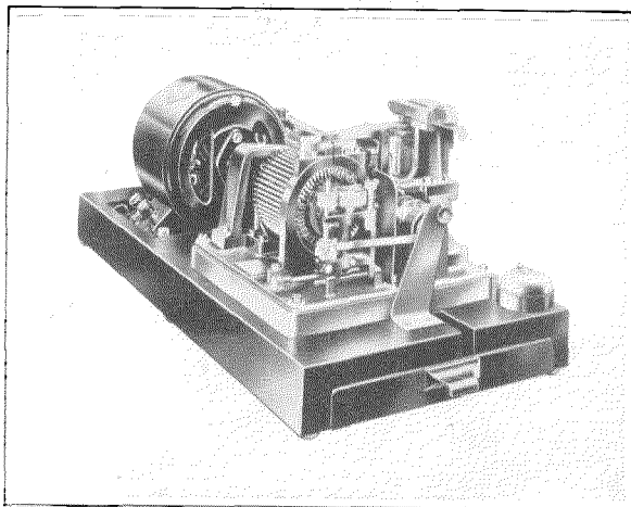
Figure 12—Morse Tape Printer.
