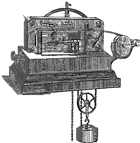
Figure 2—Transmitter (Wheatstone's Automatic System).
