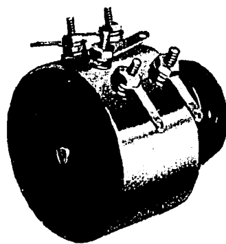
No. 890. Double depth metal shell unit in rheostat or potentiometer type. Rotors in same electrical connection. Composition elements, 5,000 ohms to 1 megohm in each unit. Diameter, 1 7-8 in. Depth of shell, 1 3-16 in.
