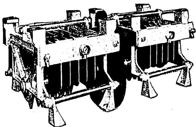
Fixed and Variable Transmitting Condensers for High Voltages.
