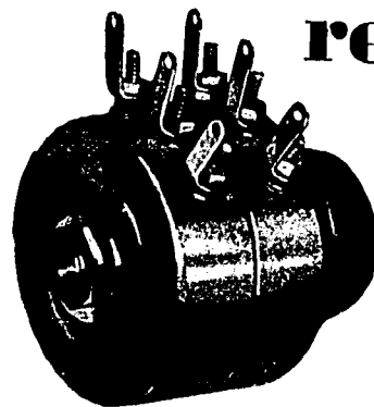
No. 280-280. Combination metal shell wire wound and composition elements. Wire wound up to 15,000 ohms. Composi- tion, 5,000 to 1 megohm. Rheostat or poten- tiometer type in either unit. Units insulated from each other. Diameter, 1 11-16 in. Depth of shell, 1 3-8 in.
