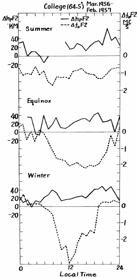
Fig. 1—Observed mean daily variations of \Delta f_0F_2 (dotted line, right ordinate) and of \Delta h_pF_2 (full line, left ordinate) at College (auroral zone) in three seasons. The variation is the mean of notable deviations during the years indicated in the figure. (After Sato.)
