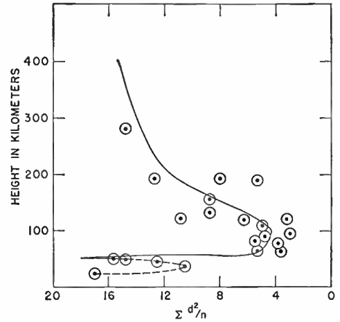
Fig. 3—Results of triangulation between Cactus Peak and Palomar Mountain according to St. Amant, Pettit, Roach, and Williams [3].
