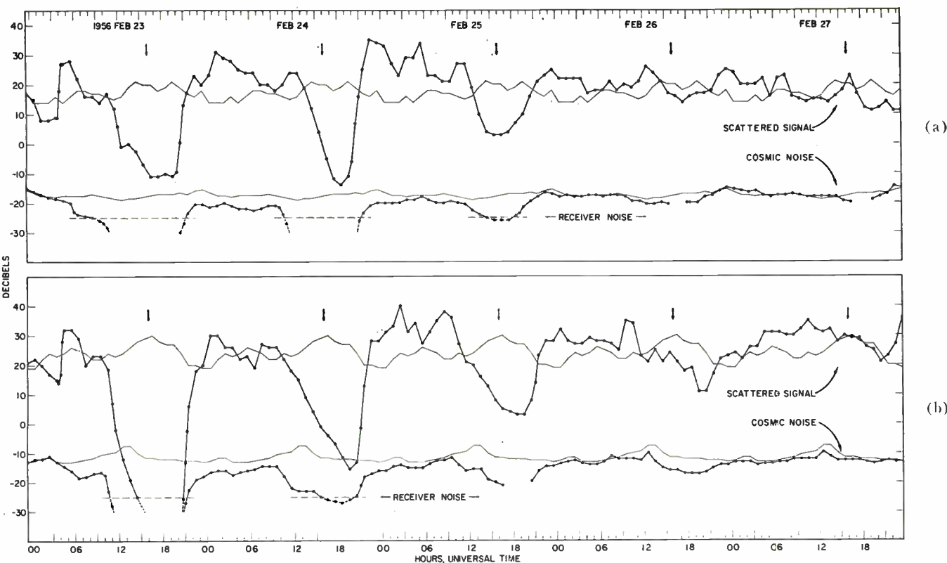
Fig. 1—Observed variations with time of intensity of signals and background cosmic noise at the same frequency with the same antenna. Normal variations indicated by the thin line. Vertical arrows indicate local apparent noon at path midpoint. (a) Observations at Søndre Strømfjord, Greenland, of signals from Thule, Greenland, and background cosmic noise, at 31.5 mc. (b) Observations at Søndre Strømfjord of signals from Goose Bay, Labrador, and background cosmic noise, at 32.2 mc.
