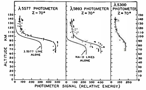
Fig. 2—Variation of airglow intensities with height from a rocket flight, according to Koomen, Scolnik, and Tousey [2].
