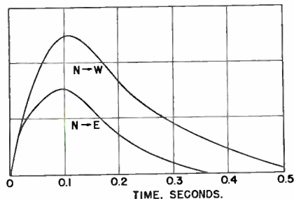
Fig. 2—Records taken by Van Valkenburg at Stanford illustrating the polarization effect. 25 The transmission was circularly polarized with a North to West rotation. Presence of a received echo with a North to East rotation results when the transverse reflection coefficient differs from the longitudinal. The frequency was 23.1 mc, the date June 3, 1950.
