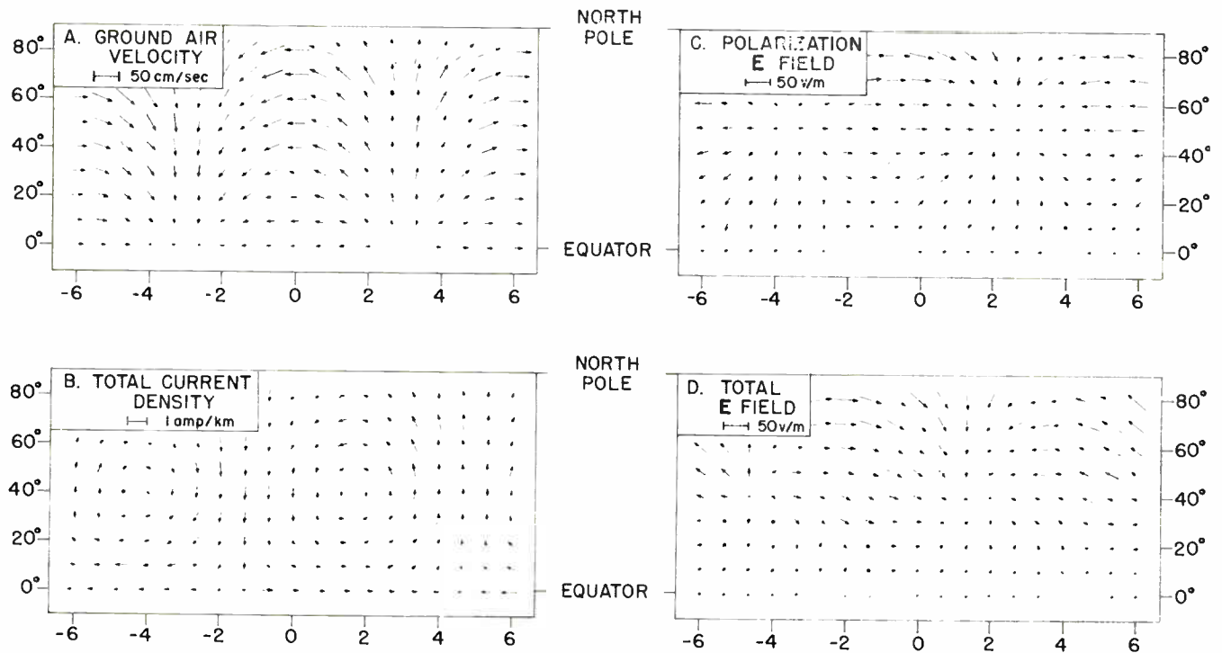
Fig. 2—Patterns of winds, currents, and horizontal electric fields in the dynamo theory of semidiurnal geomagnetic variations. 29 The winds shown, and the other vectors deduced, are based on the winds derived for the solar component at ground level. The horizontal scale measures hours after the times of maximum pressure—1000 and 2200 solar hours, 0100 and 1300 lunar hours, local time. This scale can be converted directly into longitude difference from the meridian of maximum pressure, using 1 hour = 15°. In this sense, only one quadrant of the globe is depicted; the others may be deduced from symmetry.
