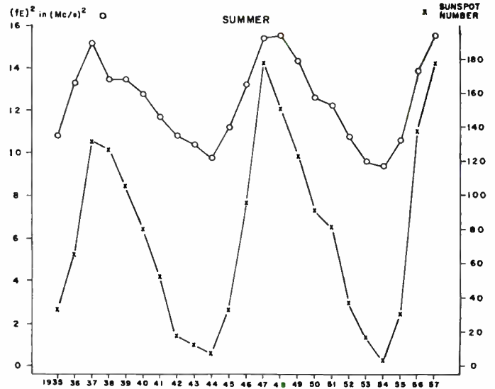
Fig. 4—Variation of average summer noon (fE)^2 at Slough, and of R (sunspot number), over the years 1935–1957.
