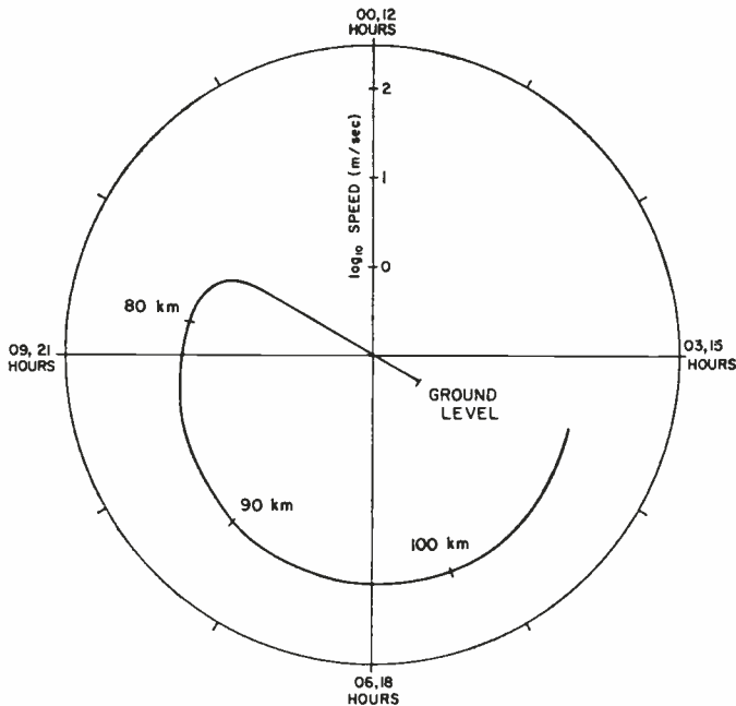
Fig. 3—Tentative representation of height variations in the amplitude and phase time 38 of the observed eastwards wind component in the solar semidiurnal tide.
