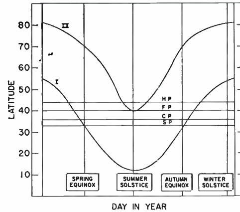
Fig. 13—Suggested double mechanism to explain the seasonal variation of 5577.
