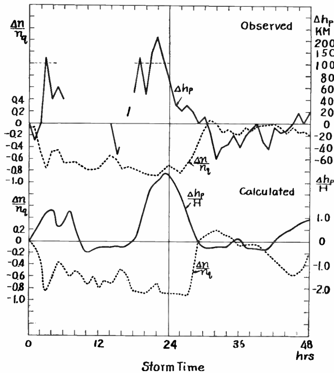
(c) Washington, 1h (Local Time) May 12, 1949.
