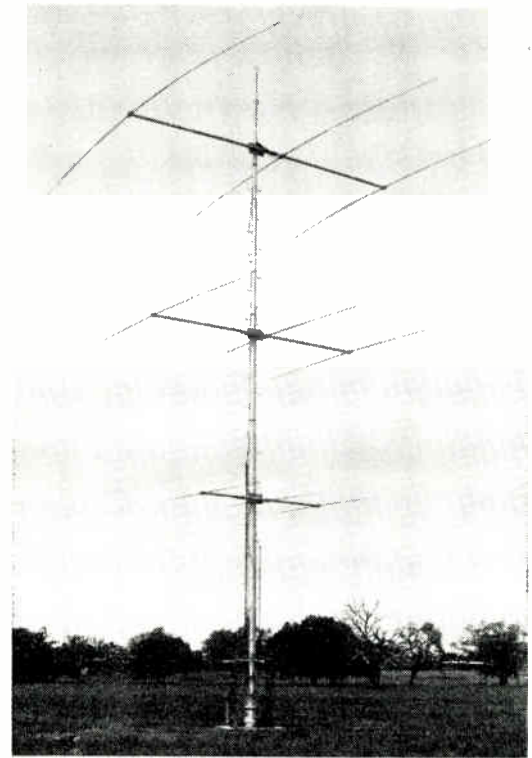
Fig. 3—Stanford IGY backscatter sounder antenna.
