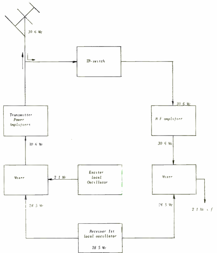
Fig. 5—Simplified illustration of transmitter-receiver frequency interlock scheme.
