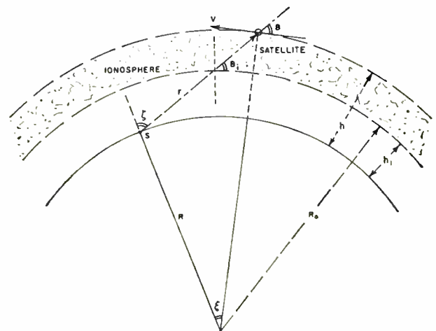
Fig. 7—Sketch of satellite passage used for derivation of ionospheric effects on Doppler tracking records.
