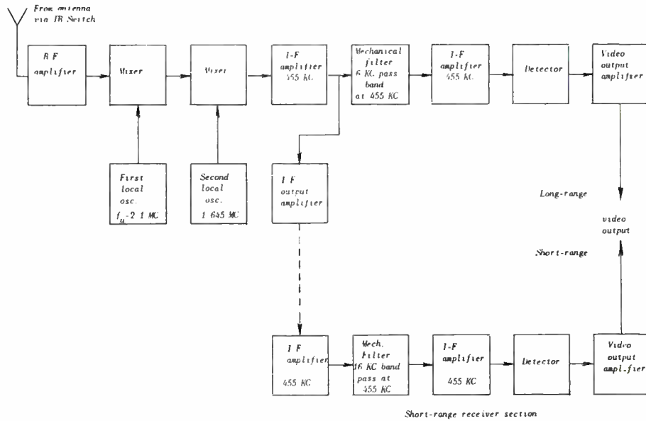
Fig. 11—Block diagram of long- and short-range receivers.
