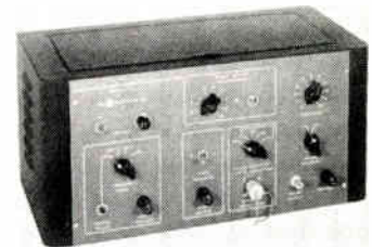
Fig. 1 - Rese Model 1051 Millimicrosecond Current Pulse Generator.
