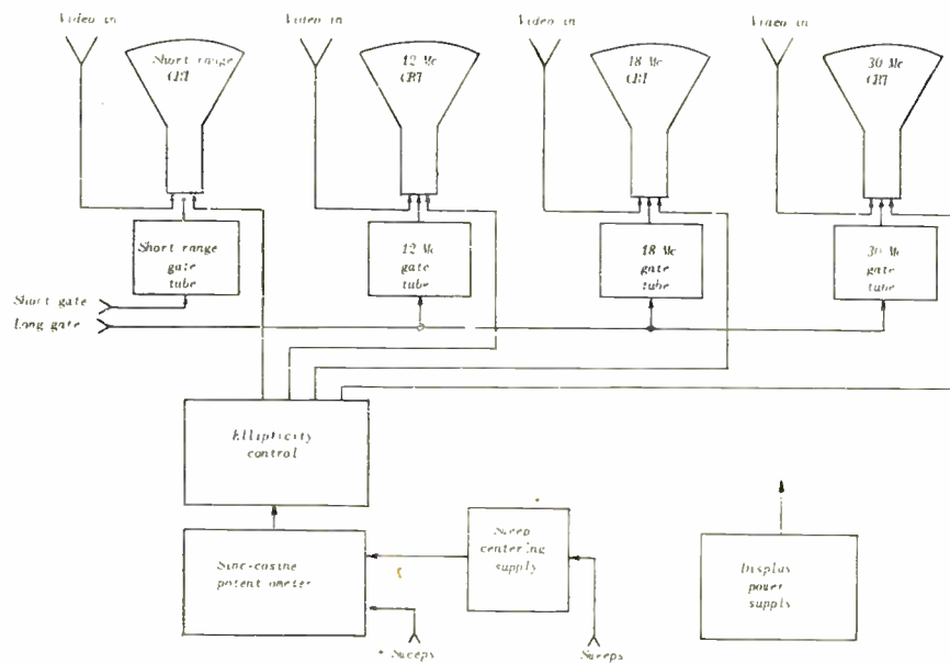
Fig. 13—Block diagram of display unit.
