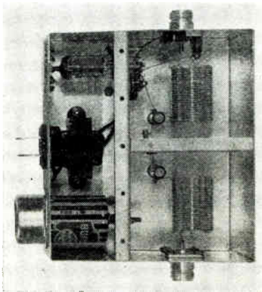
Fig. 10—Interior view of TR switch.
