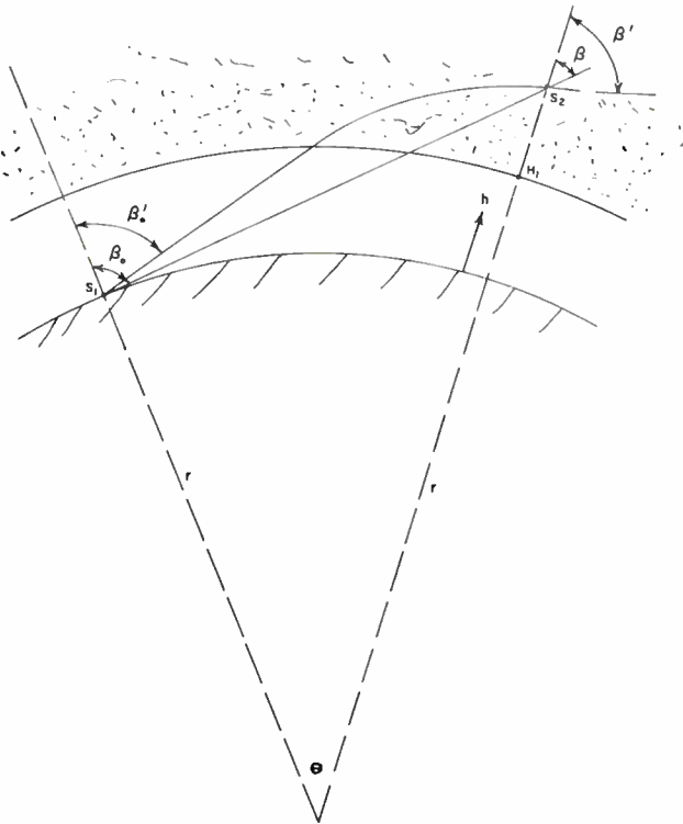
Fig. 5—Sketch of geometry used in relating refraction effects to measured angles of signal arrival.
