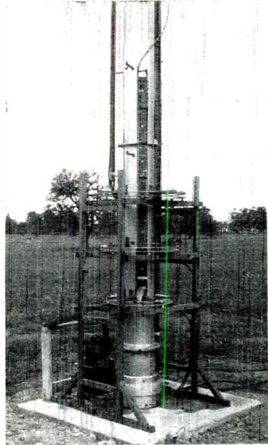
Fig. 8—Detail view of antenna support, rotary drive, and RF link coupling system.
