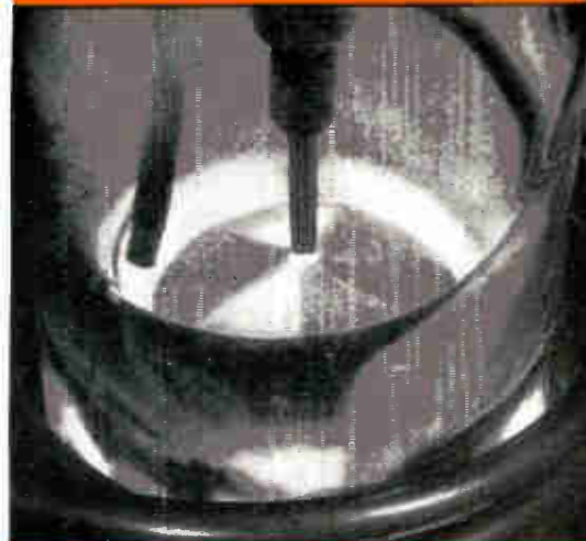
Rigid cleanliness test requires three-sixteenths inch clearance between test crystal and crucible.
