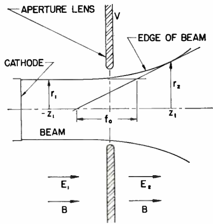
Fig. 1—Aperture-lens configuration.
