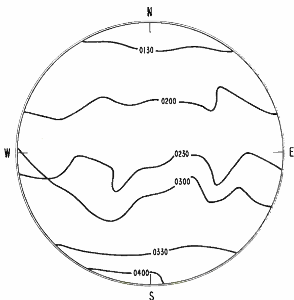
Fig. 7—Movement of 300 R isophote, Fritz Peak, October 31, 1956.
