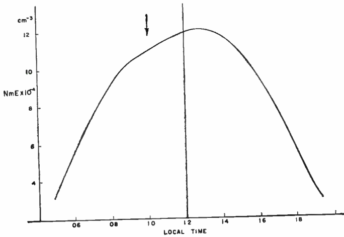
Fig. 2—Summer diurnal variation of Nm(E) at Slough.
