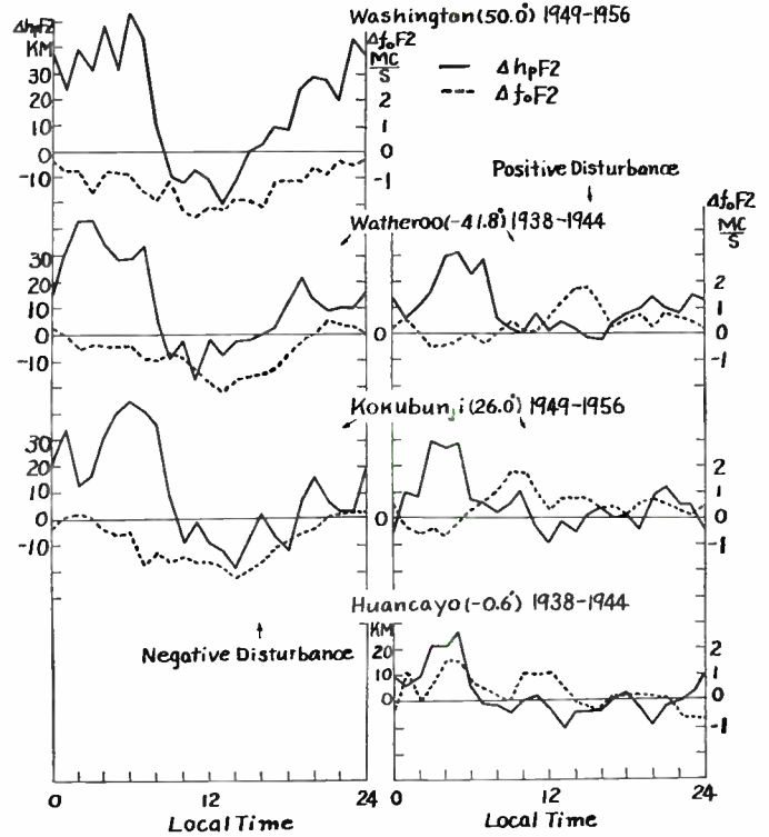
Fig. 2—Observed mean daily variations of \Delta f_0F_2 (dotted line, right ordinate) and of \Delta h_pF_2 (full line, left ordinate) in negative and positive disturbances for four stations below the auroral zone (number is geomagnetic latitude). The variation is the mean of notable deviations during the years indicated in the figure. (After Sato.)
