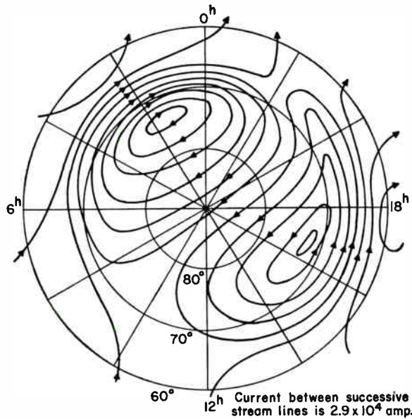
Fig. 1—Mean equivalent current system for polar magnetic storms during Second Polar Year (after T. Nagata). The world-wide current system for geomagnetic latitudes above 60^\circ north is shown as a function of local time. The current between successive stream lines is 2.9 \times 10^4 amperes.
