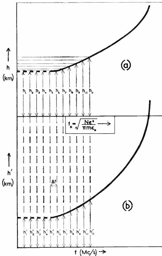
Fig. 1—(a) An N(h) profile replotted as an f_N(h) curve, showing laminations at a frequency interval \Delta f at heights h_1, h_2, \dots, h_n, \dots . (b) Corresponding values h'_1, h'_2, \dots, h'_n, \dots of virtual height are shown on the h'(f) curve. The continuous curves correspond to the parts of the h'(f) curve actually observed and the broken lines to the assumed form for frequencies below the limit of the apparatus.
