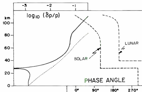
Fig. 1—Height variation of amplitude (solid line) and phase angle 23 (broken lines) in semidiurnal tides. 12,20 The amplitude scale shown applies to the solar component; the variation for the lunar component is similar, but the absolute value is diminished by a factor of 10 or more. The dotted curve represents the variation which would have occurred, had the energy flow been exactly constant in height for the assumed atmosphere. Zero phase angle corresponds to the time of (solar or lunar) transit; maximum pressure is taken to occur at 1000 and 2200 solar hours, 0100 and 1300 lunar hours, local time. 29
