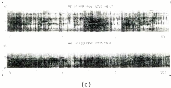
Fig. 8—Multistation whistler showing conjugate relationship. (a) Wellington (WE), Dunedin (DU), Unalaska (UN), and Kotzebue (KO). (b) College (CO), Seattle (SE), Stanford (ST), Boulder (BO). (c) Bermuda (BE), Washington (WA). Note: The whistlers at Bermuda and Washington were very weak but they are distinctly observable aurally on the magnetic tapes and can be identified on the original spectrograms just before the 1-second marks.
