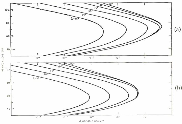
Fig. 8—Calculated specific absorption distribution at 32 mc as a function of geomagnetic latitude resulting from the abnormal ionospheric layers. (a) For midday equilibrium. (b) For nighttime equilibrium.
