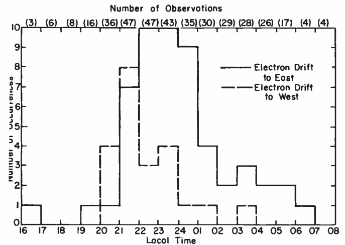
Fig. 3—Nocturnal variation of the direction of electron drift motions in auroral ionization. The number of occurrences of electron drift to the east (solid line) and to the west (broken line) is shown as a function of time at College, Alaska. The number of days when observations were made at each hour is listed along the top.
