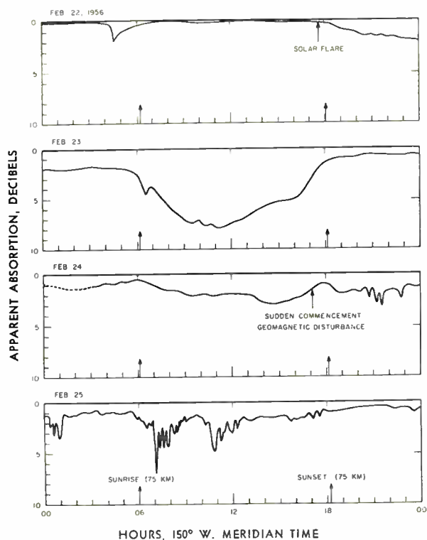
Fig. 2—Apparent absorption of cosmic noise at 30 mc recorded with a wide-beam antenna directed vertically at College, Alaska.
