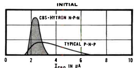
Comparative Life Tests NPN vs. PNP Switching Transistors.
