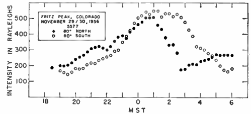
Fig. 4—Synchronous variations of 5577.
