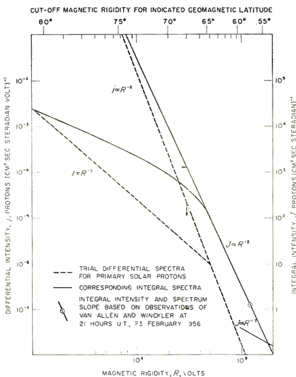
Fig. 4—Trial magnetic-rigidity spectra.
