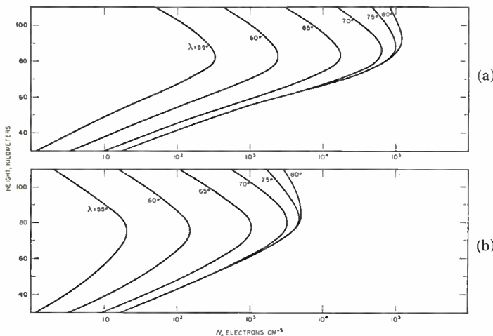
Fig. 7—Calculated electron-density distributions as a function of geomagnetic latitude for the abnormal ionospheric layers. (a) For midday equilibrium. (b) For nighttime equilibrium.
