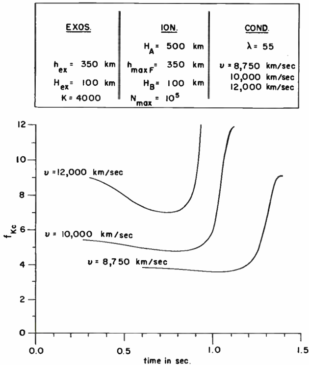
Fig. 15—VLF emissions theory. Example of influence of velocity.
