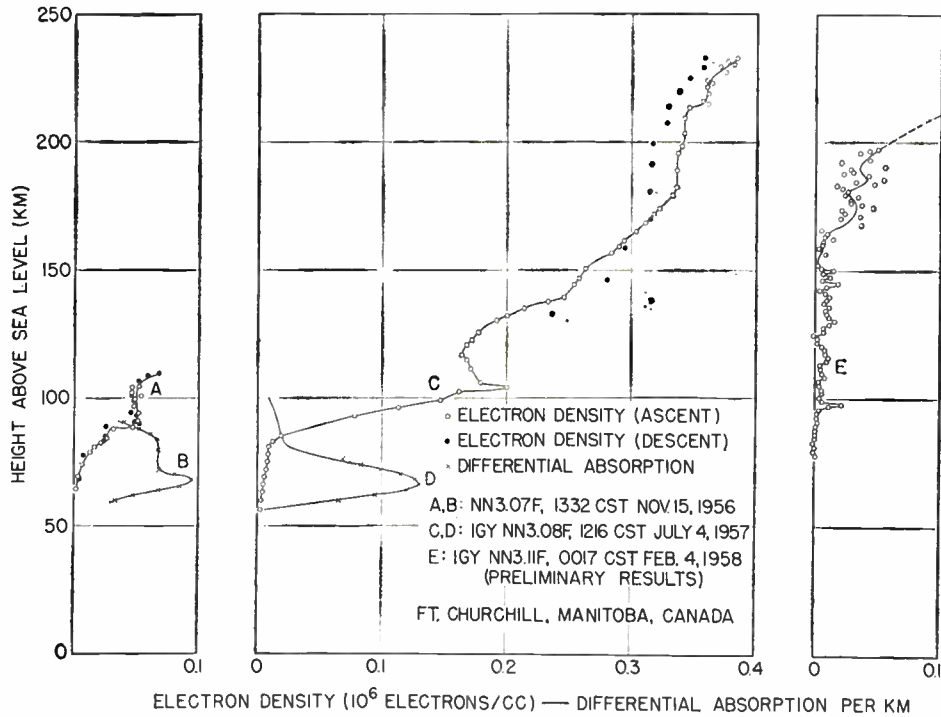
Fig. 4—Electron densities measured on a winter day, summer day, and winter night, above Fort Churchill. Differential absorption on 7.75 mc below E region is shown for both daytime flights. 2
