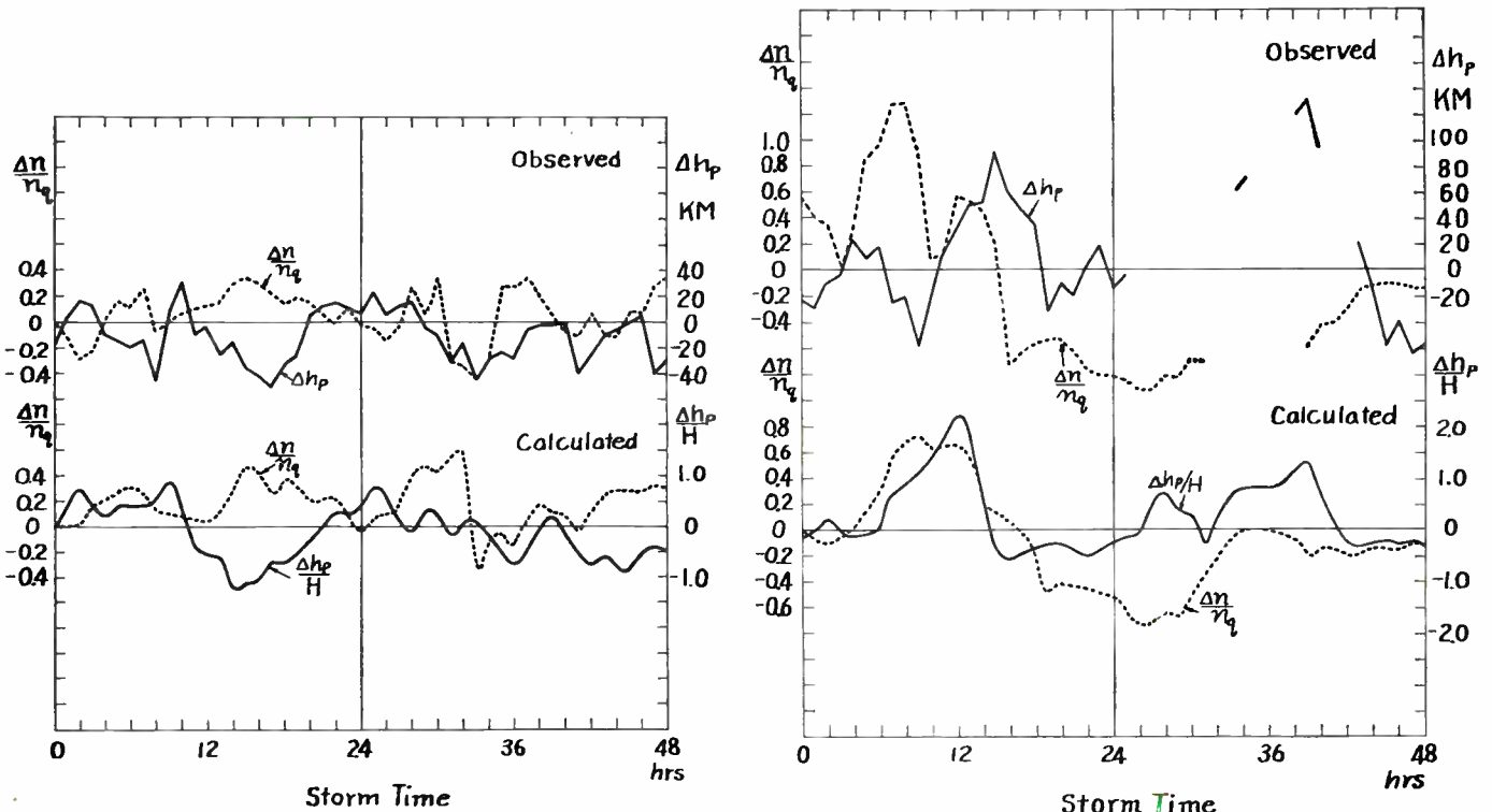
(a) Huancayo, 20h (Local Time), July 2, 1939.
