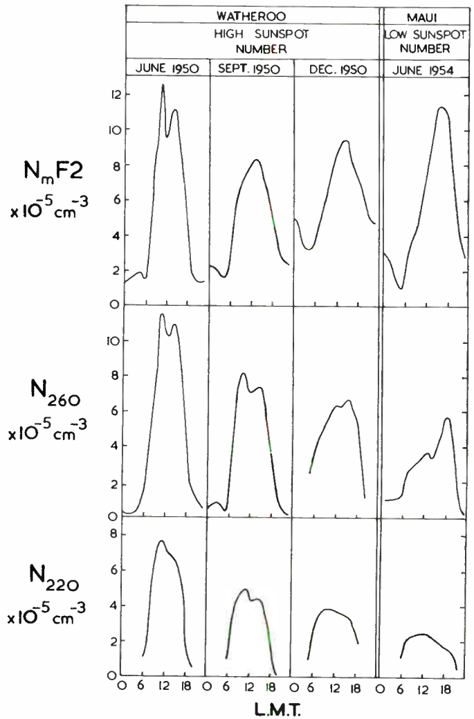
Fig. 8—For ten International Quiet Days in each month, the average variation of NmF_2 and of the electron density at 260 and 220 km ( N_{260} and N_{220} ). Results obtained for Watheroo in a year of high sunspot number and for Maui in a year of low sunspot number.
