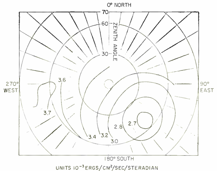
Fig. 9—Lyman- \alpha intensity contours in the night sky. The smallest intensity contour loop contains the antisolar direction. No correction to the data was made for the contribution of discrete sources between 1225 and 1350 Å which appear in the West. (NRL Aerobee 31, March 28, 1957, 2200. 19 )
