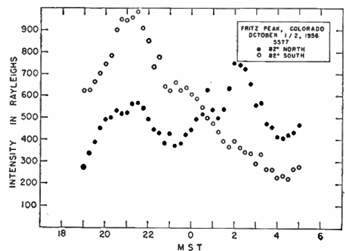
Fig. 5—Nonsynchronous variations of 5577.
