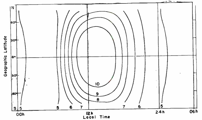
Fig. 5—Theoretical f_0 F_2 contours for Chapman region.
