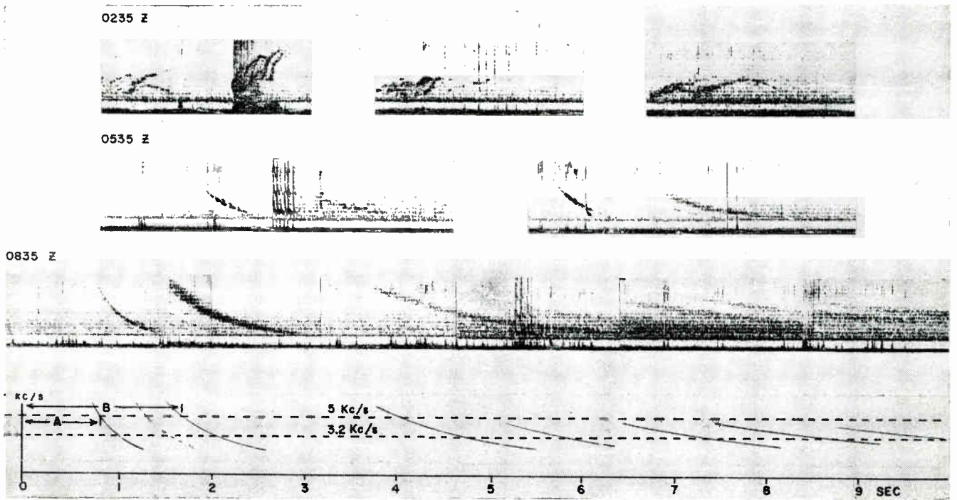
Fig. 1—Unalaska, November 11, 1956.
