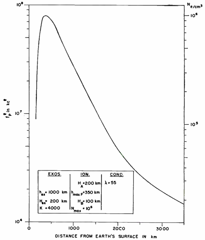
Fig. 13—VLF emissions theory. Model distribution of electronic density.
