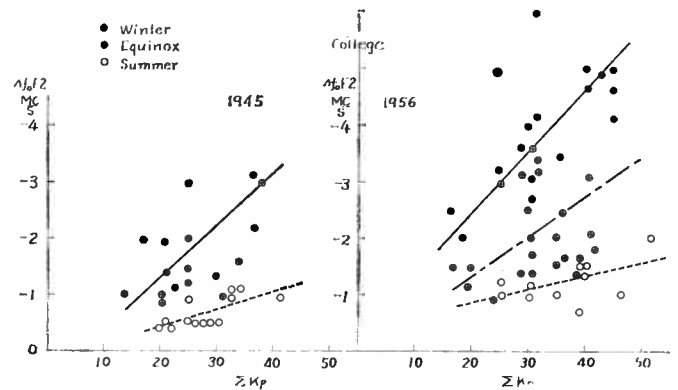
Fig. 5—Relation between the mean value of \Delta f_0 F_2 during three hours centered on noon, and \Sigma K_p (a daily sum of K_p indexes) at College in 1945 (a year near sunspot minimum) and in 1956 (a year near sunspot maximum). (After Sato.)
