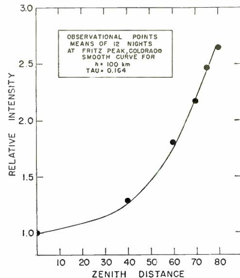
Fig. 1—Change in intensity of airglow 5577 with zenith distance; the smooth curve corresponds to an emission height of 100 km and an extinction coefficient, tau, of 0.164.
