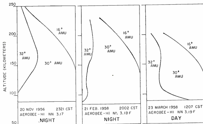
Fig. 6—Positive-ion composition of the ionosphere above Fort Churchill. The relative abundance of an ion at a particular altitude is represented by the horizontal width of the area assigned to the ion. 11
