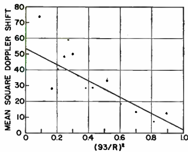
Fig. 4—Mean-square body-Doppler shift caused by wind motion vs (93/R)^2 = \sin^2 \alpha , where \alpha is the elevation angle of the ray to the meteor, and R is the slant range. The curve, based on 330 echoes recorded by Manning, Peterson, and Villard, on July 27, 1949, from 0230 to 0500 LST, demonstrates the wind velocities to be predominantly horizontal. The frequency was 23.1 mc.
