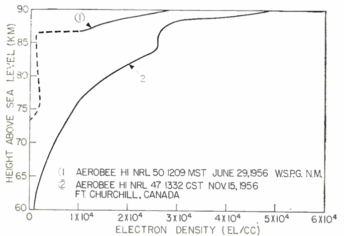
Fig. 5—Electron densities below E region under normal daytime conditions at White Sands, and during polar blackout at Fort Churchill. 1
