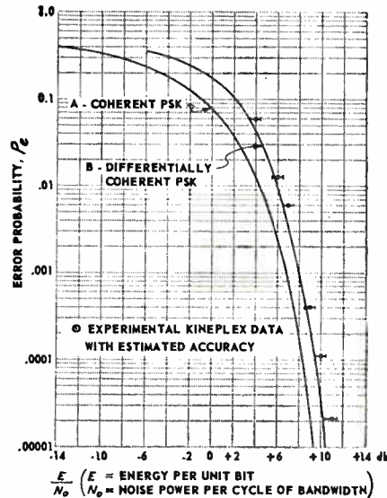
Fig. 1—Error probability of phase-shift keyed systems.
