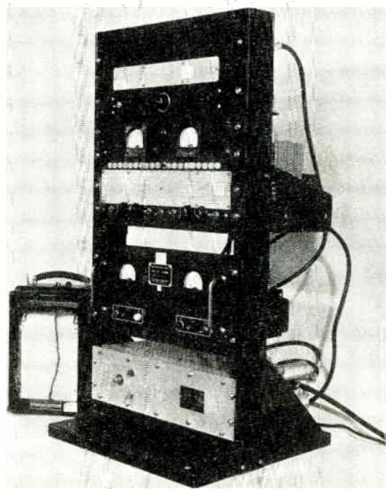
Fig. 2—The riometer.
