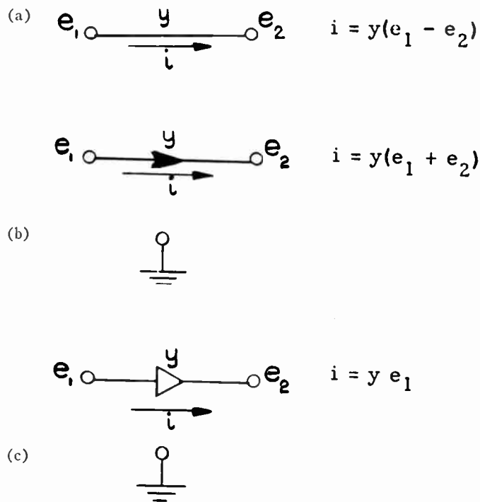
Fig. 1—Basic branch elements: (a) the reciprocal branch (resistor), (b) the antireciprocal branch (gyristor), and (c) the unilateral branch (unistor).
