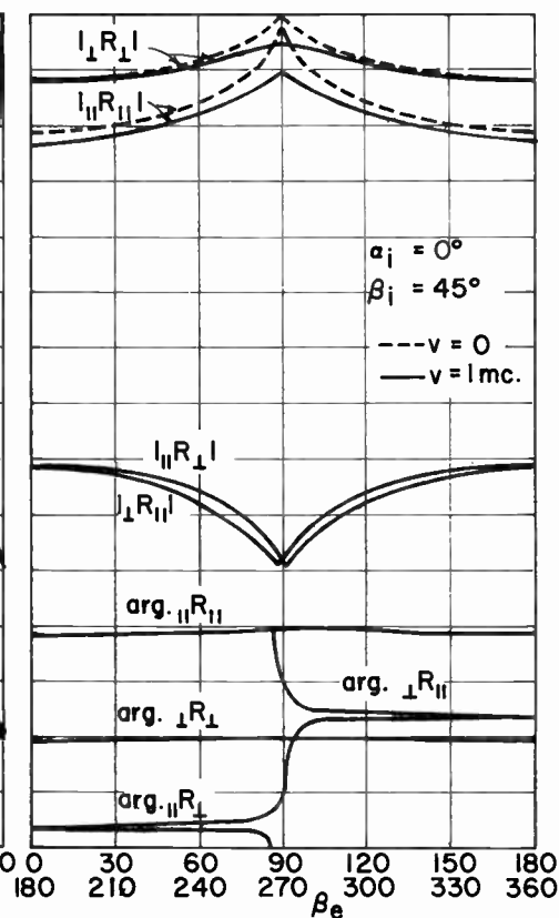
Fig. 3—Reflection coefficients vs direction of earth's field.
