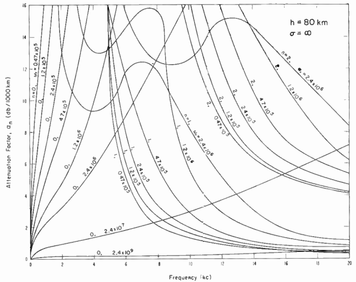
Fig. 3—Same as Fig. 1 with h=80 km.
