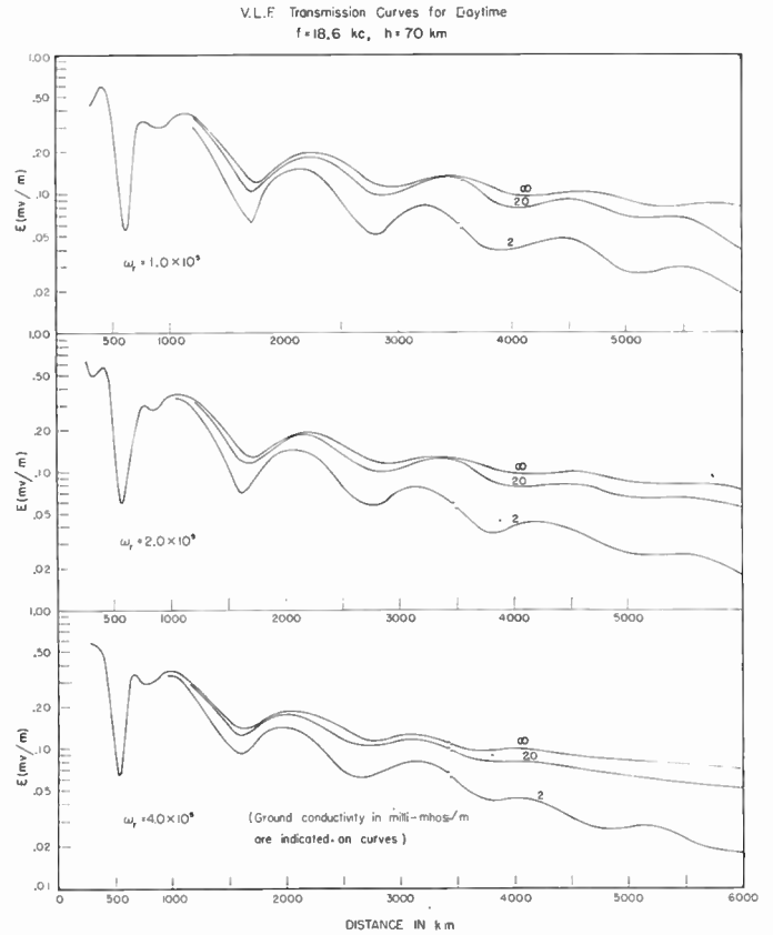
Fig. 7—Calculated field-strength-vs-distance curves for 18.6 kc for ground conductivities of 2, 20 and \infty in millimhos/meter and \omega_r values of 1.0, 2.0, and 4.0 \times 10^8 . (The height is taken to be 70 km corresponding to typical daytime conditions.)
