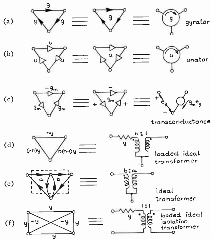
Fig. 3—Branch models of linear devices.
