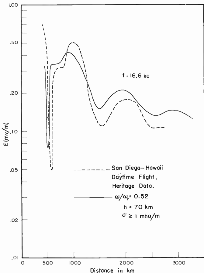
Fig. 4—An experimental field-strength-vs-distance curve for 16.6 kc over sea and the corresponding calculated curve assuming \omega/\omega_r=0.52 or \omega_r=2.0 \times 10^5 , h=70 km and \sigma \geq 1 mho/meter.
