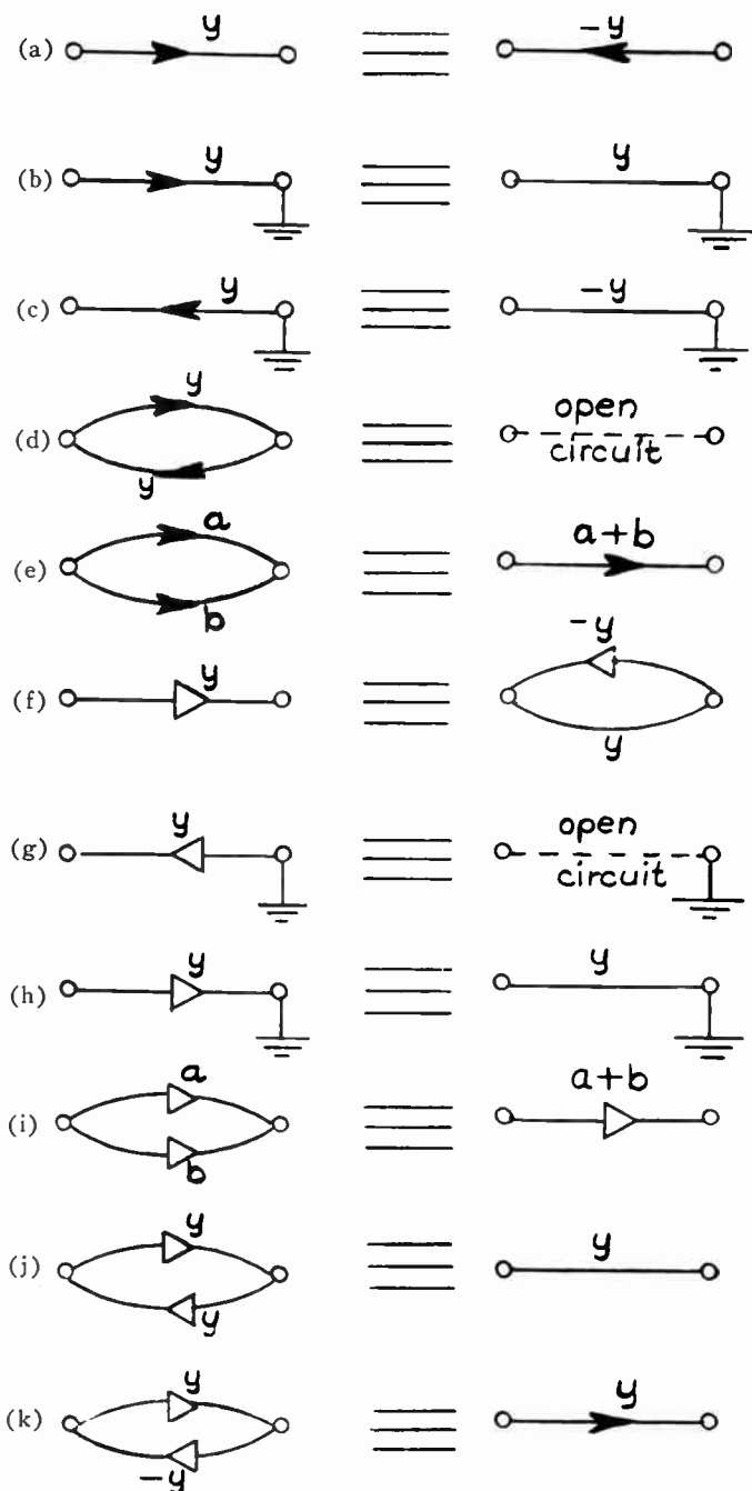
Fig. 2—Some elementary equivalences.
