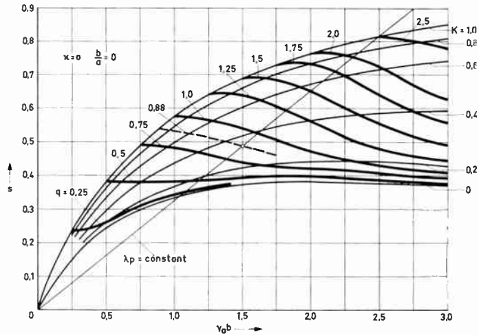
Fig. 5—Plot of the plasma frequency reduction factor s as a function of \gamma_0 b with q = \gamma_0 b_c \sqrt{B_c/B} and K as parameters; \kappa = 0 , b/a = 0 . Intersection points with the straight line through the origin yield s and b for a given plasma wavelength.
