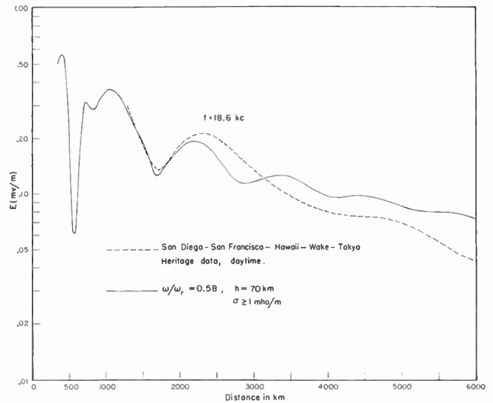
Fig. 5—An experimental field-strength-vs-distance curve for 18.6 kc over sea and the corresponding calculated curve assuming \omega/\omega_r=0.58 or \omega_r=2.0 \times 10^5 , h=70 km and \sigma \geq 1 mho/meter.
