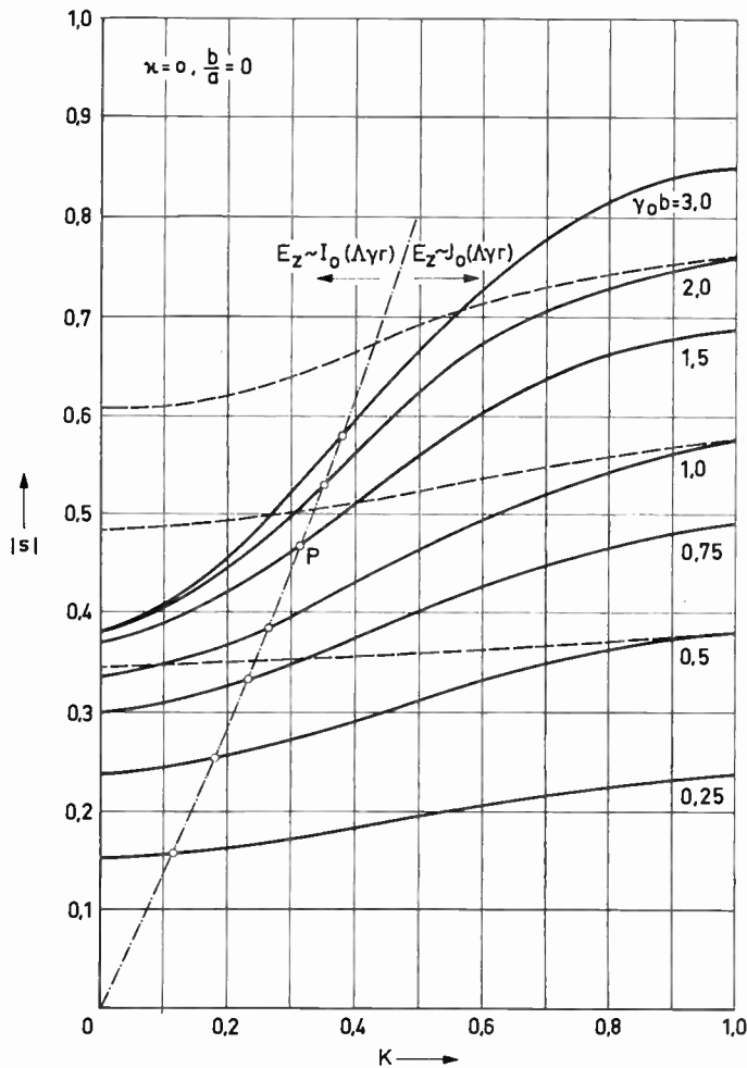
Fig. 4—Plot of the plasma frequency reduction factor as a function of the magnetic flux parameter K = b_c^2 B_c / b^2 B (--- according to Brewer). The index c denotes the cathode. On the left and right side of the - · - · - line the axial electric field component is given by the modified Bessel function I_0(\Lambda\gamma r) and the Bessel function J_0(\Lambda\gamma r) respectively.
