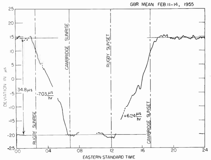
Fig. 10—The diurnal variation of the time of arrival of the gbr signal, derived from the data of Fig. 9.
