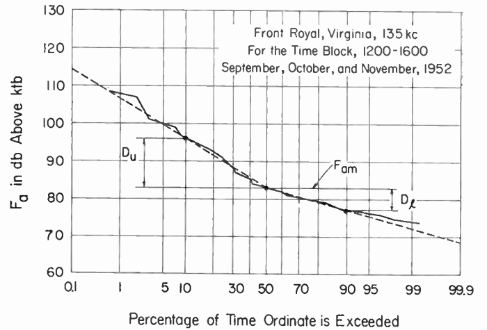
Fig. 6—Typical amplitude-time distribution of hourly noise levels.
