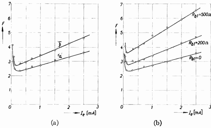
Fig. 21—Noise figures (grounded base) of junction transistors of approximately equal \alpha values as dependent on I_e . Diagram (a) curve a : R_b \approx 400 ohms, \alpha = 0.987 , curve b : R_b \approx 600 ohms, \alpha = 0.988 . Diagram (b) Transistor of curve a of diagram (a), with added base resistances R_{b1} of 0.200 and 500 ohms respectively. The 200-ohm curve approximately coincides with the curve b of diagram (a). Frequency was 7.24 kc.
