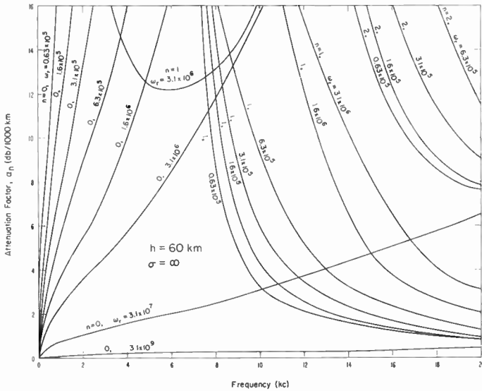
Fig. 1—The attenuation factor in decibels per 1000 km of path length as a function of the frequency in kilocycles. The mode number and the value of \omega_r are indicated on each curve. The conductivity, \sigma , of the ground is taken to be infinite and the height of the ionospheric reflecting layer is a height, h , of 60 km.
