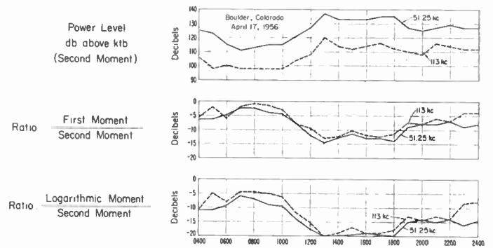
Fig. 5—Typical diurnal variations of atmospheric noise.
