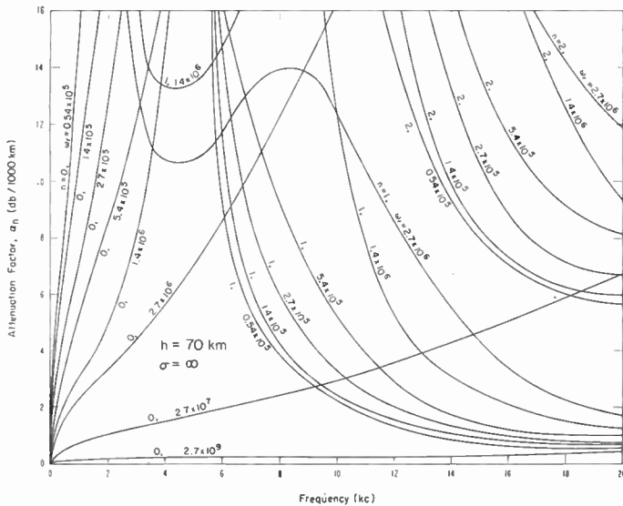
Fig. 2—Same as Fig. 1 with h=70 km.
