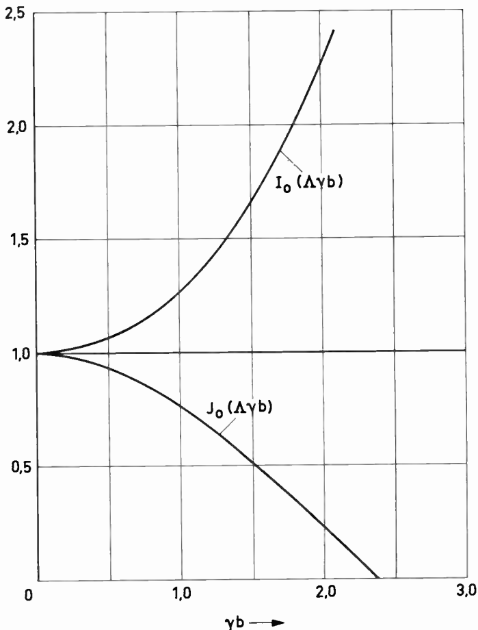
Fig. 7—Configuration of the axial electric field component E_z as a function of the radius r . E_z \approx J_0(\Lambda\gamma r) for s^2 > 2K^2/1 - K^2 ; E_z \approx I_0(\Lambda\gamma r) for s^2 < 2K^2/1 - K^2 ; E_z = \text{constant} for s^2 = 2K^2/1 - K^2 .
