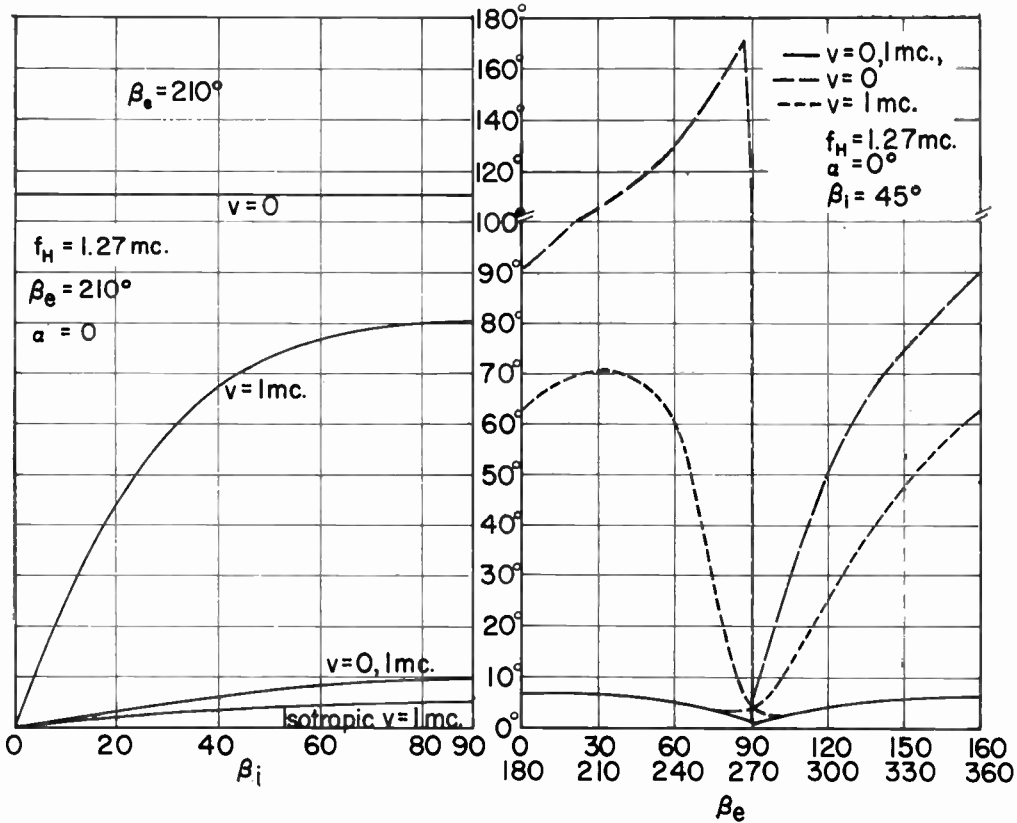
Fig. 4—Wave normal direction vs vertical angle of incidence.
