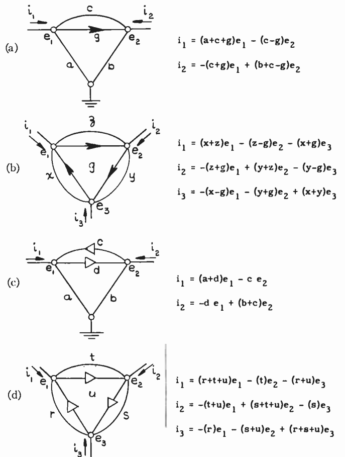
Fig. 4—Some general models of arbitrary three-terminal devices.
