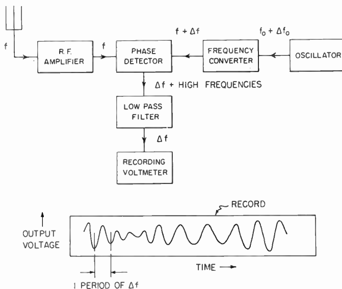
Fig. 2—A block diagram of a simple frequency comparator that can have narrow noise bandwidth.
