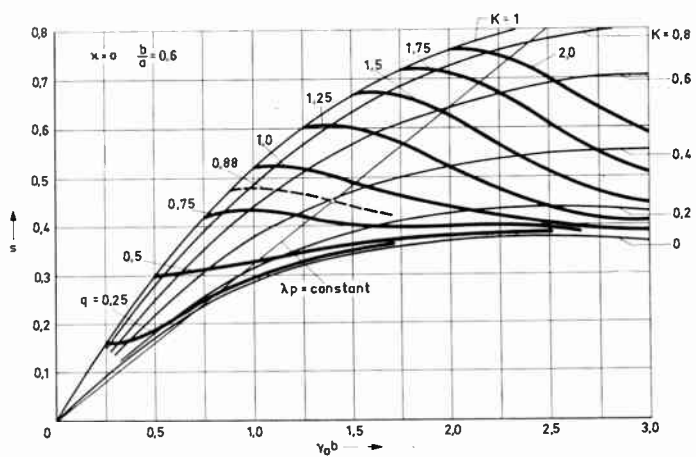
Fig. 6—Plot of the plasma frequency reduction factor s as a function of \gamma_0 b with q = \gamma_0 b_c \sqrt{B_c/B} and K as parameters; \kappa = 0 , b/a = 0.6 .
