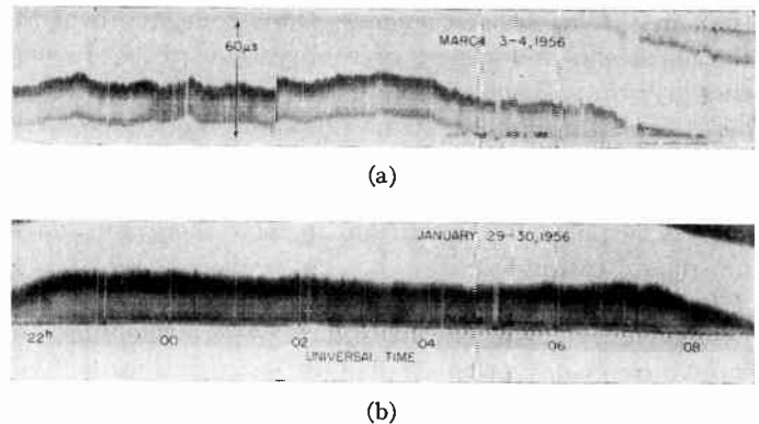
Fig. 15—(a) A gbr phase record during a night of high magnetic activity, and (b) a corresponding record on a magnetically quiet night. Note: Discontinuities in the upper record at 0.16 hours and 0.68 hours U.T. were caused by retuning the transmitting antenna and not by magnetic activity. Usually the deviations in frequency are not greater than \pm 2 or 3 parts in 10^9 , but occasionally there are frequency deviations of as much as 1 or 2 parts in 10^8 that persist for two or three minutes at a time. As an aid in judging these values, it should be mentioned that a 45^\circ slope, in these photographic records, corresponds to a frequency difference of about 1/10^8 . It is seen that high magnetic activity greatly increases errors of measurement for intervals of a few minutes, but has little effect when the frequency measurement duration is many hours.
