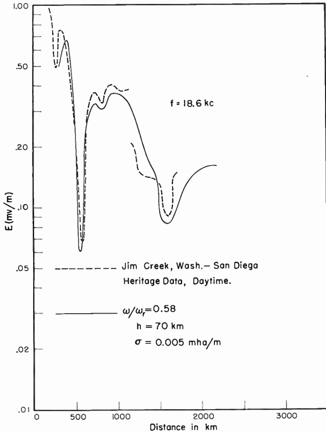
Fig. 6—An experimental-field-strength-vs-distance curve for 18.6 kc over land and the corresponding calculated curve assuming \omega/\omega_r = 0.58 or \omega_r = 2.0 \times 10^8 , h = 70 km and \sigma = 5 millimhos/meter.
