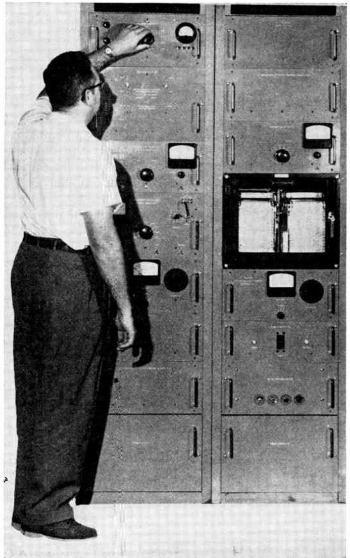
Fig. 1—Radio noise recorder developed at the National Bureau of Standards.
