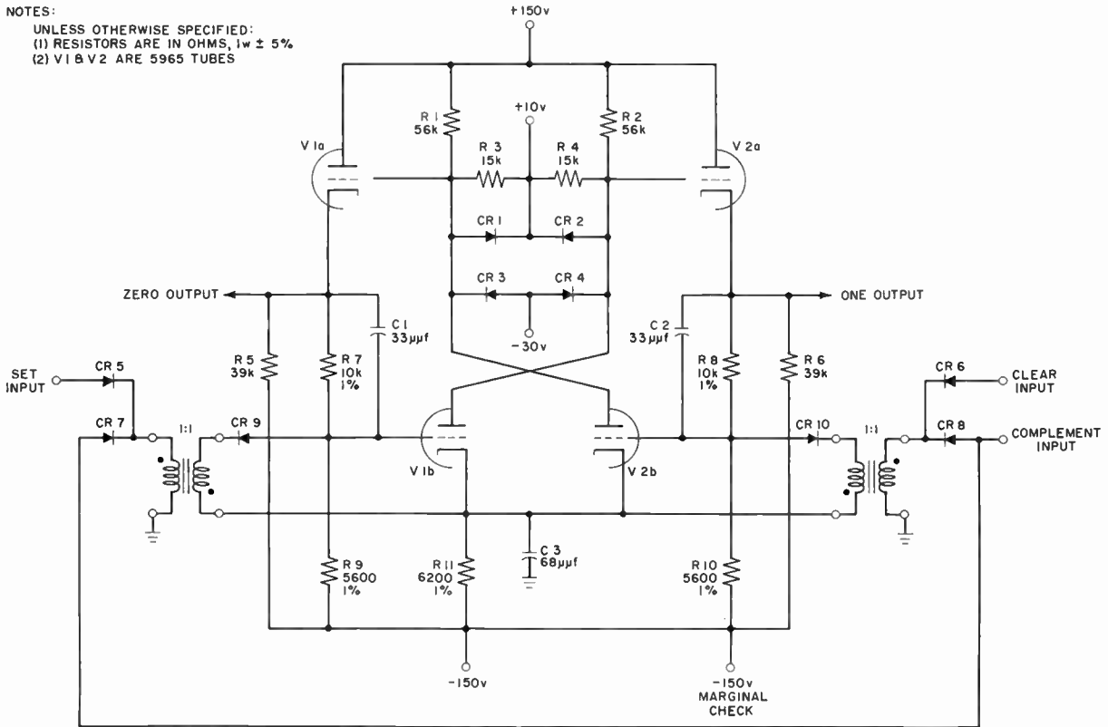
Fig. 5—High-speed flip-flop.
