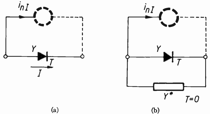
Fig. 2—(a) Semiconductor diode completed by an additional noise source i_{nr} (dotted circle) to restore quasithermal equilibrium. (b) Diode of (a) with an admittance Y^* of absolute temperature T=0 connected to its terminals. This entire circuit is approximately in quasi-thermal equilibrium.
