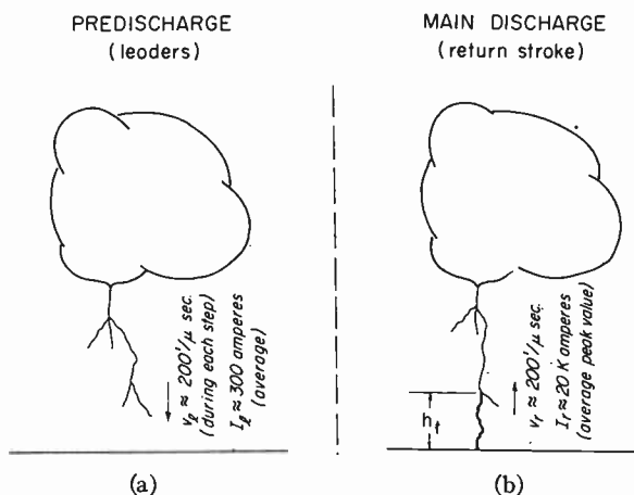
Fig. 1—Lightning discharge.
