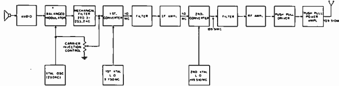
Fig. 1—Single-sideband transmitter.
