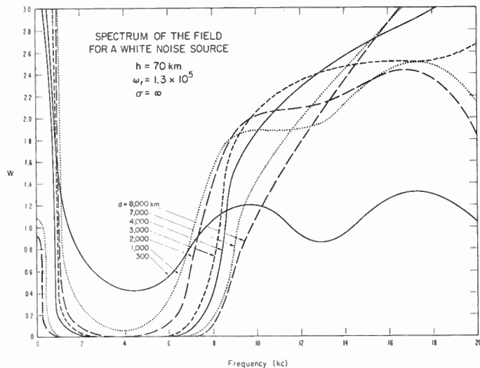
Fig. 6—The spectrum function W , at various distances, is shown plotted as a function of frequency for h = 70 km, \omega_r = 1.3 \times 10^5 , and \sigma = \infty . W in this case corresponds to the field for a dipole source whose radiated power is constant with respect to frequency.
