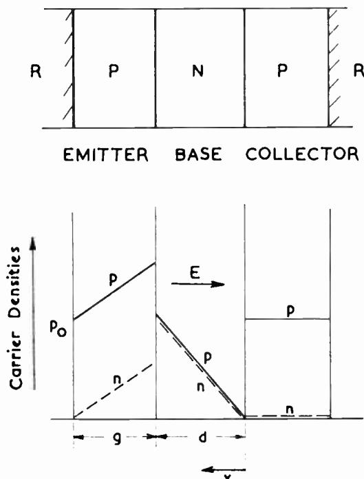
Fig. 9—RPNP transistor.
