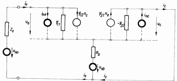
Fig. 8—Grounded base connection of junction transistor, showing two noise current sources and one noise voltage source of transistor as well as one noise voltage source corresponding to the source impedance Z_0 at the input.
