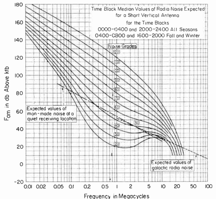
Fig. 8—Variation of noise level with frequency.
