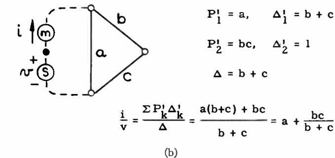
Fig. 9—Calculation of (a) input impedance and (b) input admittance.
