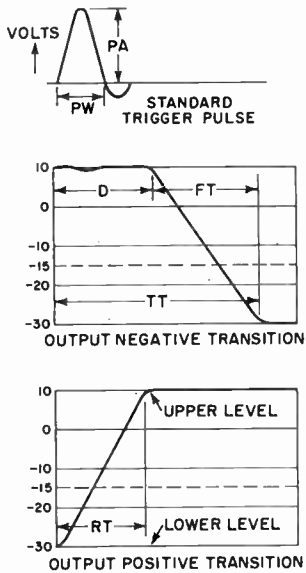
Fig. 6—Input and output waveforms.
