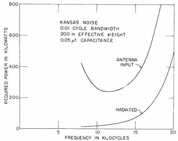
Fig. 18—An estimate of the power required to provide standard frequency service all over the world from a single vlf station.
