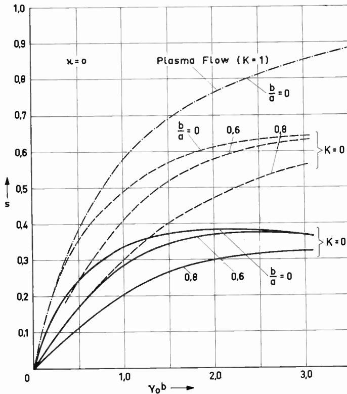
Fig. 2—Plot of the plasma frequency reduction factor s as a function of \gamma_0 b (for the plasma ( K=1 ) and Brillouin (beam ( K=0 ) (--- according to Rigrod and Lewis; — according to Labus and Pöschl)). Space charge parameter \kappa = \omega_p / \omega = 0 ; b = radius of the solid beam, a = radius of a conducting drift tube.
