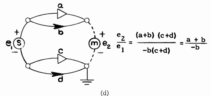
Fig. 10—Some simple network transmissions which illustrate the topological rules.
