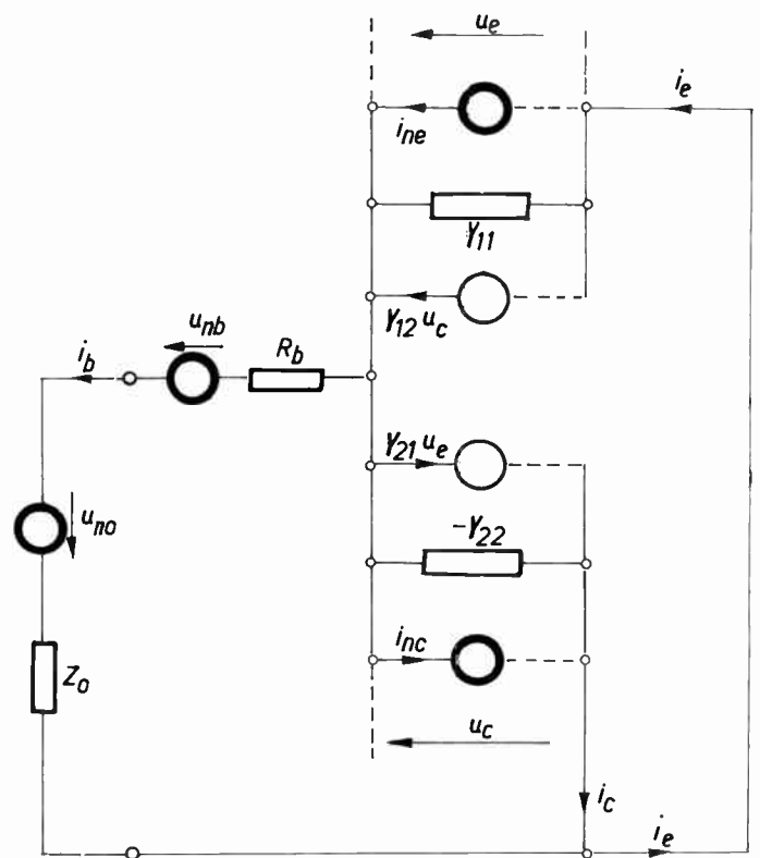
Fig. 10—Grounded collector circuit, similar to Fig. 8.
