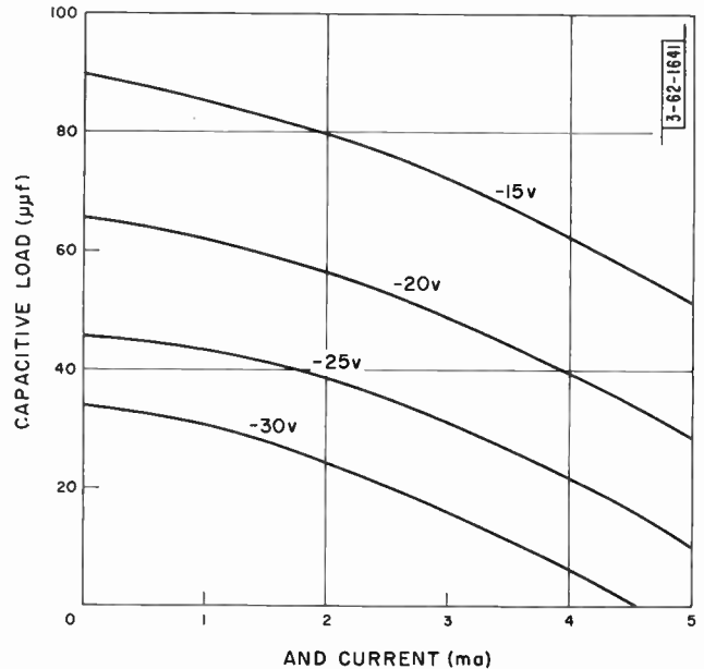
Fig. 7—Maximum load for less than 0.5 µsec fall time.
