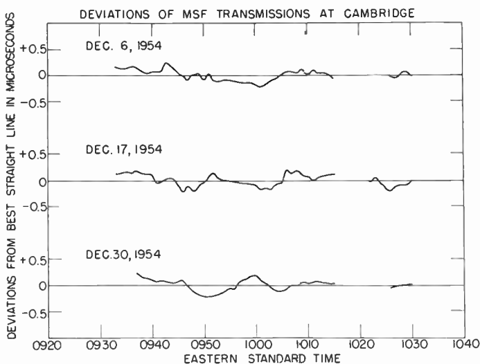
Fig. 6—Examples of the fluctuations in the time of arrival of the 60-kc standard frequency signal from msf, Rugby, received at Cambridge, Mass.
