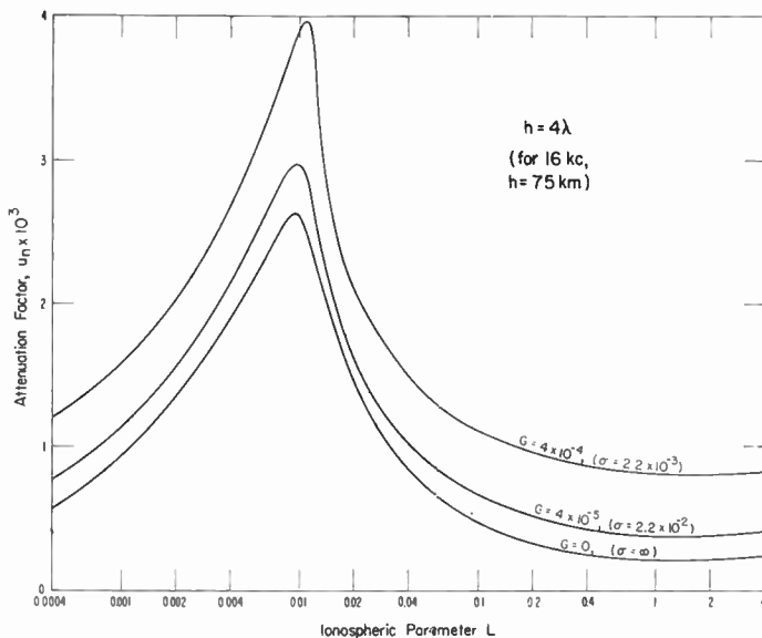
Fig. 2—The attenuation factor as a function of the reciprocal of the effective ionospheric conductivity for various ground conductivities for n=1 .
