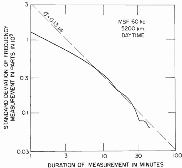
Fig. 7—The standard deviation of measurement of the frequency of the msf signal as a function of the duration of the measurement.
