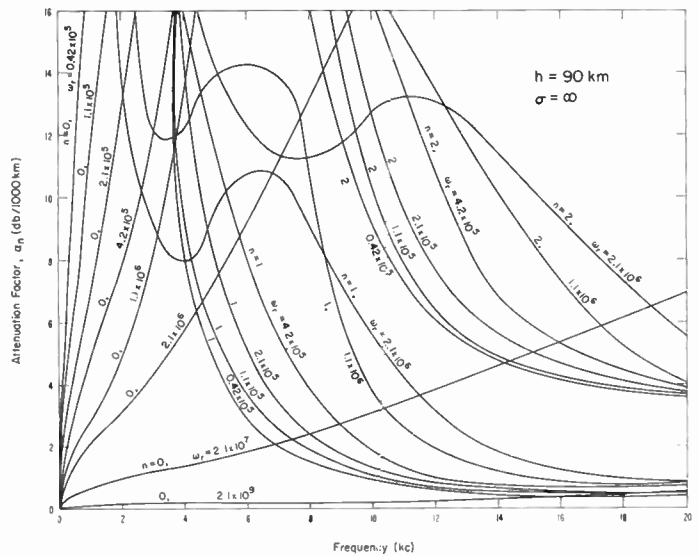
Fig. 4—Same as Fig. 1 with h=90 km.
