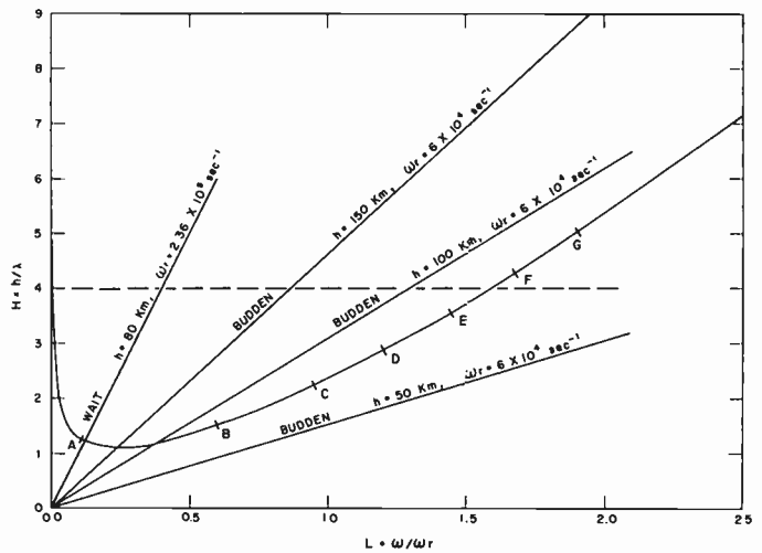
Fig. 1—The curve is the locus of points for which simultaneously \partial f(C)/\partial C = 0 and |f(C)| = 1 . The points A, B, C, \dots , indicate values of L and H for which two mode points coincide.
