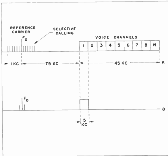
Fig. 2—Radio central transmitter spectrum. (a)—Entire spectrum transmitted by the central; (b)—Portion of spectrum selected by subscriber no. 1.
