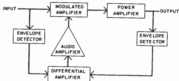
Fig. 6—Envelope feedback circuit for AM.
