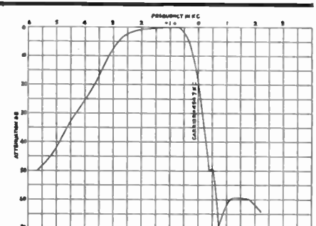
CRYSTAL-TOROID SINGLE SIDE-BAND FILTER TYPE TX-455-5B
