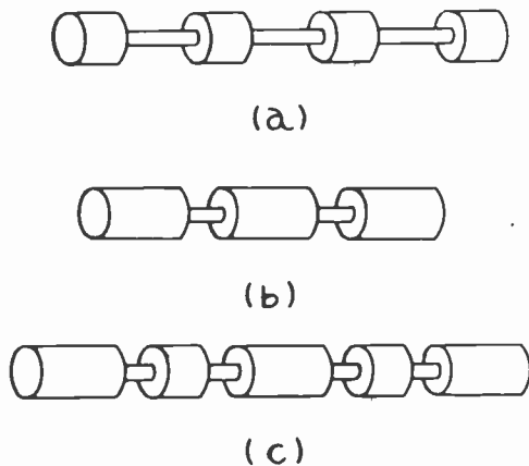
Fig. 1—(a) Slug-coupled filter, normally operated in the longitudinal mode of vibration. (b) Neck-coupled filter, normally operated in the torsional mode of vibration. (c) Neck-coupled filter with multiple couplers, normally used for narrow-band torsional mode filters.
