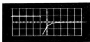
Fig. 1—Recovery characteristic of type S-6 silicon diode under normal operation in circuit for measuring reverse current transient. Scale: Vert = 1.0 v/cm Horiz = 0.1 μsec/cm.
