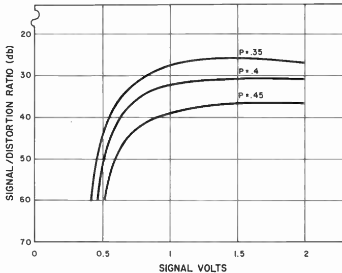
Fig. 5—Distortion vs signal level for other bias points.
