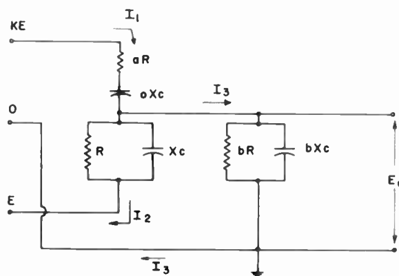
Fig. 13—The "M-Derived" phase-shift network.
