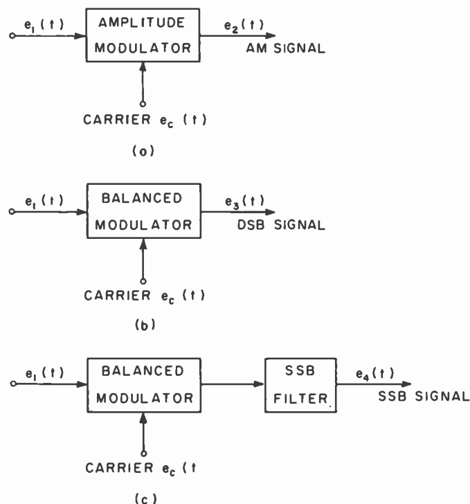
Fig. 1—Modulation systems.
