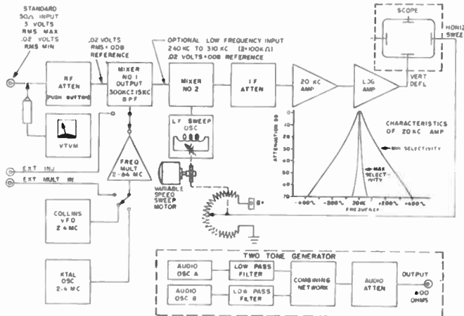
Fig. 4—Block diagram of spectrum analyzer.
