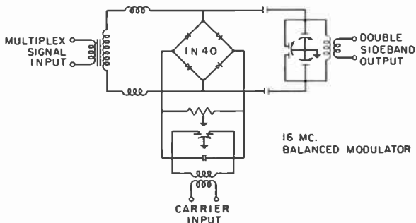
Fig. 18—Sixteen-mc balanced modulator diagram.
