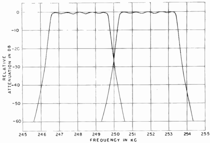
Fig. 5—Response curves of 250 kc upper- and lower-sideband filters having 9 mechanical resonators.
