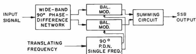
Fig. 2—Phasing method of SSB generation.
