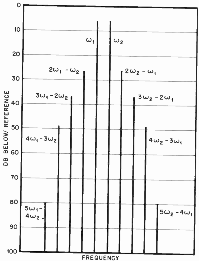
Fig. 3—Spectra from two equal signals.
