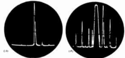
These two oscillograms show hum components in a hand extending 300 c/s on either side of the carrier in an i.s.b. transmitter. (A) Carrier and 100-c/s hum component at -29 db as displayed with Spectrum Analyzer in low-sensitivity condition. (B) Expanded view, as given with sensitivity increased by 30 db, revealing further components at -300, -200, -100, -50, +50, +200 and +300 c/s.
