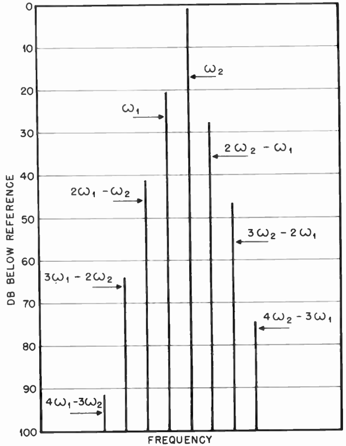
Fig. 6—Single-sideband spectra carrier 20 db down.
