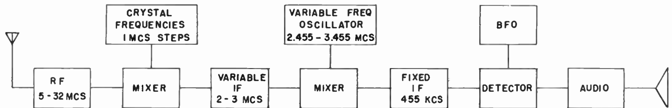
HIGHLY SIMPLIFIED BLOCK DIAGRAM R-392 URR/AN/GRC-19
