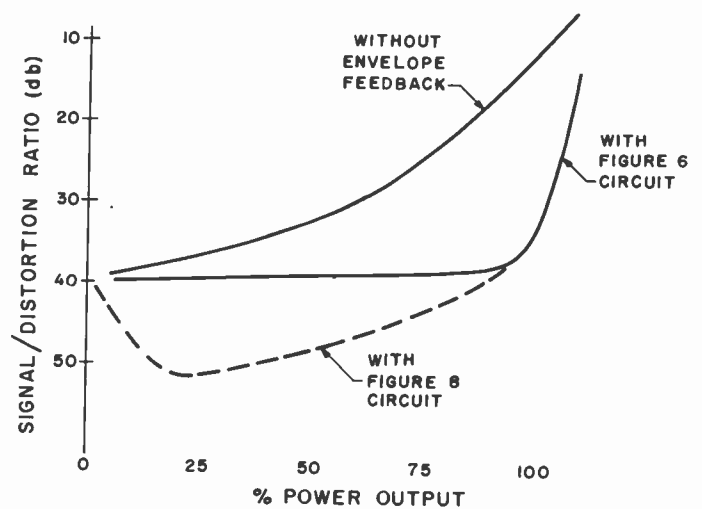
Fig. 7—Distortion reduction by envelope feedback.
