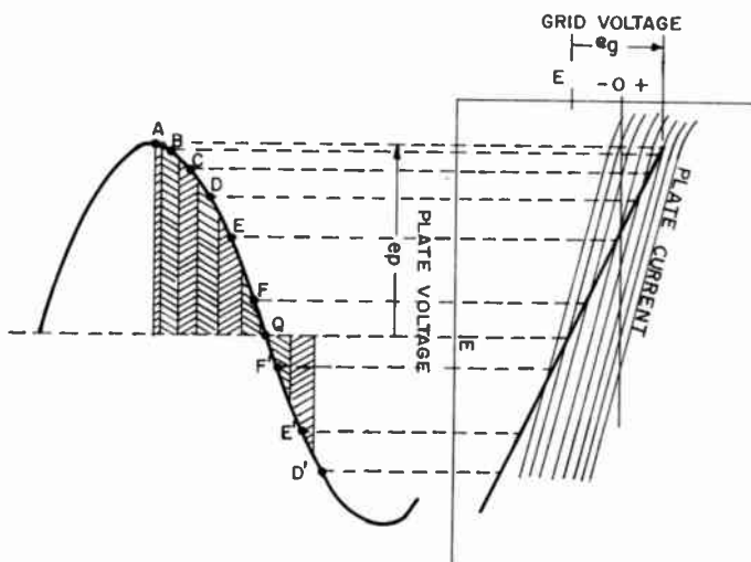
Fig. 11—Principle of graphical analysis.
