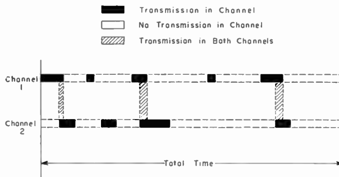
Fig. 9—Example of channel activity—two-channel system.
