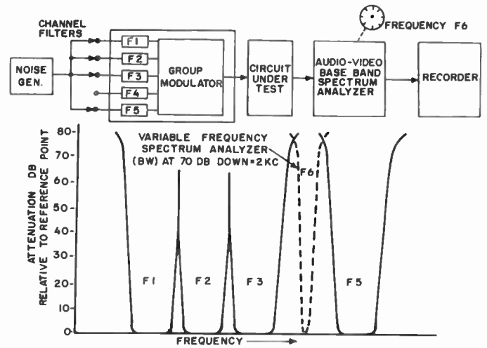
Fig. 8—Variable frequency noise-loaded intermodulation distortion test set; block diagram and selective curves.
