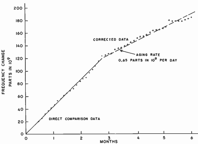
Fig. 8—Long-term frequency stability of a typical reference frequency oscillator. (Direct comparison data represents errors derived from time comparison with WWV. Corrected data represents errors derived from time comparison with WWV after having corrected data per WWV's time correction bulletin.)
