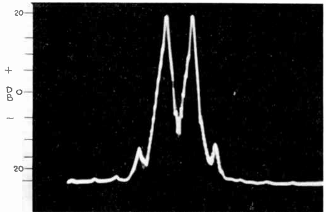
Fig. 6—Two-carrier test pattern at power output of approximately 10 kw, rms, per carrier. Third-order distortion products are about 32 db down. Separation of carriers is 2150 cycles.
