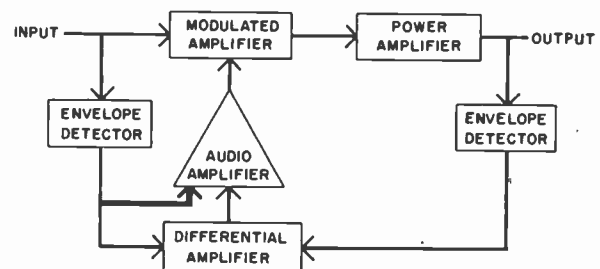
Fig. 8—Envelope feedback circuit for single sideband.
