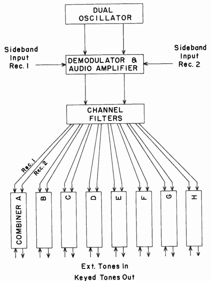
Fig. 5—Block diagram of the telegraph combining system.
