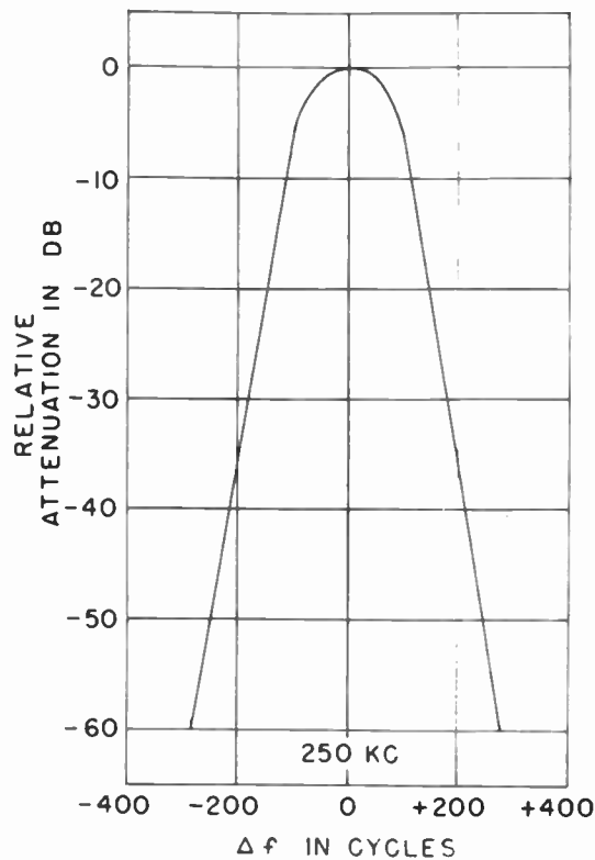
Fig. 4—Response of a 250 kc carrier filter with 200-cycle bandwidth.
