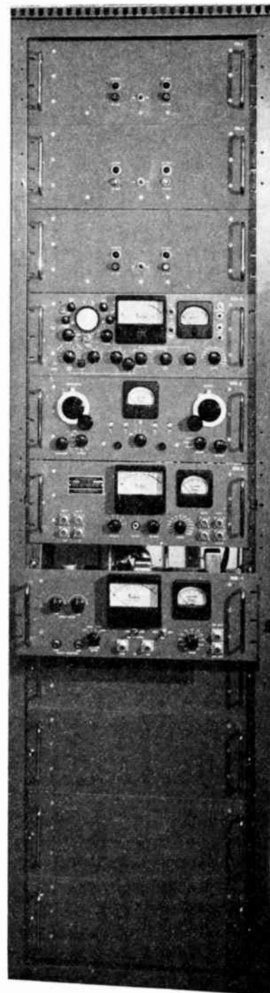
Fig. 2—SSB53-2A. Kahn Research Laboratories' twin sideband adapter.
