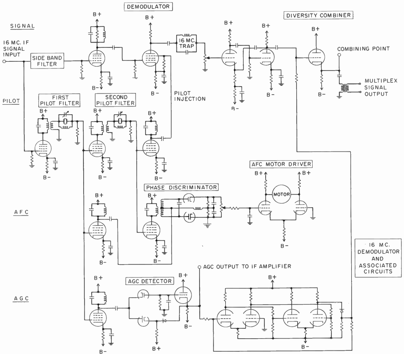
Fig. 31—Receiver 16-mc demodulator and associated circuits.
