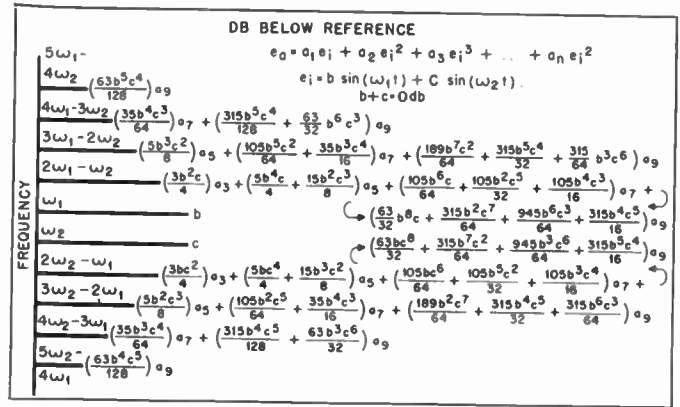
Fig. 2—Single-sideband splatter spectra due to nonlinearities.
