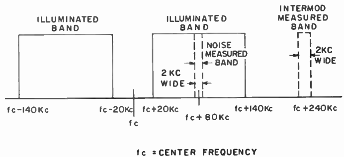
Fig. 22—Noise modulated signal for intermodulation distortion measurement.
