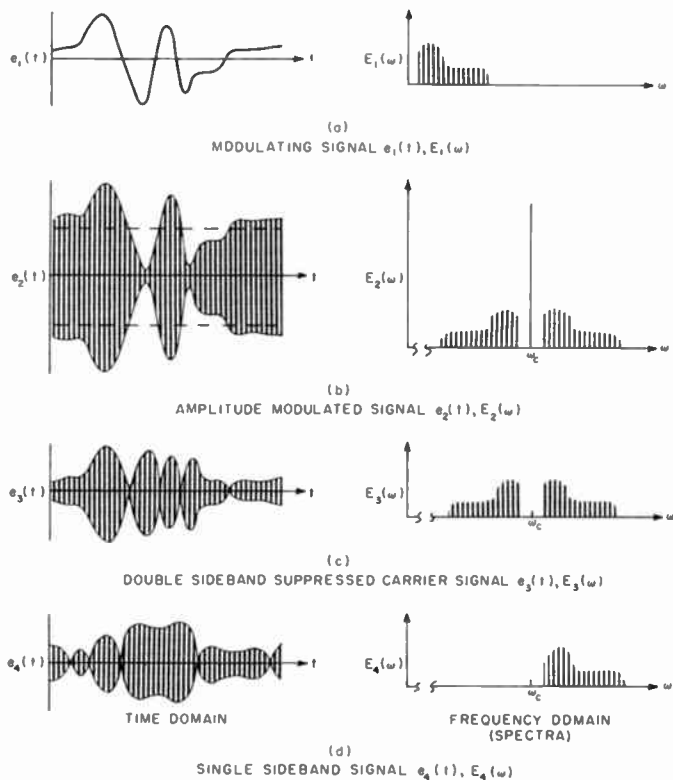
Fig. 2—Signal representations.
