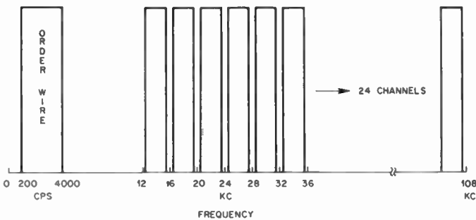
Fig. 4—Typical spectrum allocation—frequency division multiplex voice channels. CCIF channel allocation for twenty-four-channel system.
