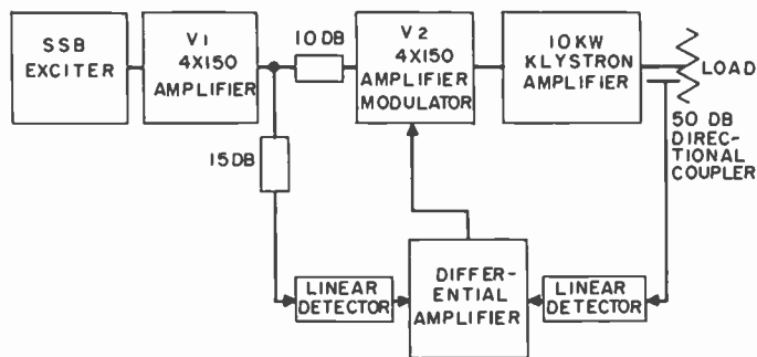
Fig. 24—Balanced envelope feedback arrangement.
