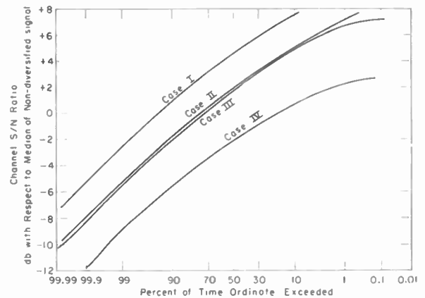
Fig. 11—Combined distributions for various cases. Case I: Twenty-four channels, \tau=0.10 , fourth-order maximal-ratio diversity. Case II: Twenty-four channels, \tau=0.25 , fourth-order maximal-ratio diversity. Case III: Sixty channels, \tau=0.10 , fourth-order maximal-ratio diversity. Case IV: Sixty channels, \tau=0.25 , fourth-order maximal-ratio diversity.
