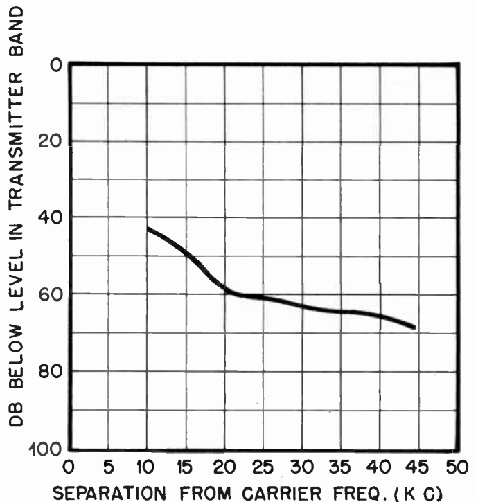
Fig. 9—Measurements on a SSB suppressed carrier transmitter modulated with voice [5].
