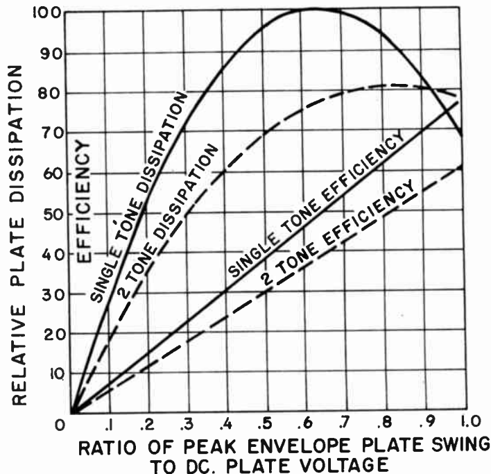
Fig. 9— P_d vs signal level of theoretical class B tube.
