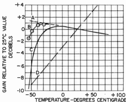
Fig. 2—Effect of ambient temperature on the gain of a four-stage transistor amplifier.
