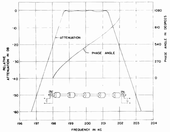
Fig. 6—200-kc Slug-coupled longitudinal band-pass filter.
