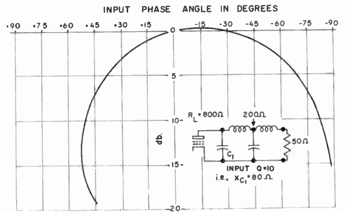
Fig. 5—Phase-gain plot of input of a Pi-L network.
