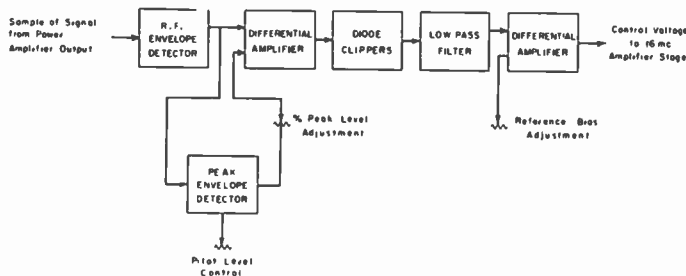
Fig. 19—Output power regulator block diagram.
