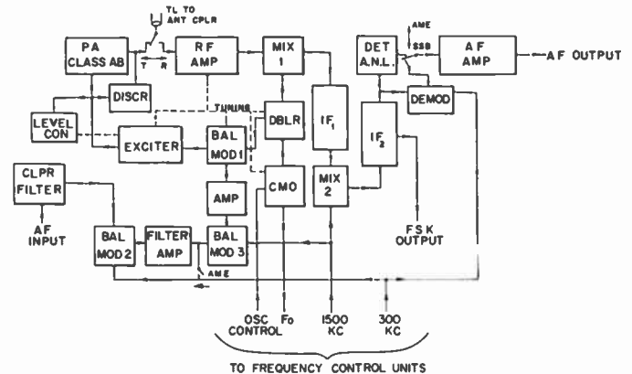
Fig. 7—Block diagram of the SSB conversion.
