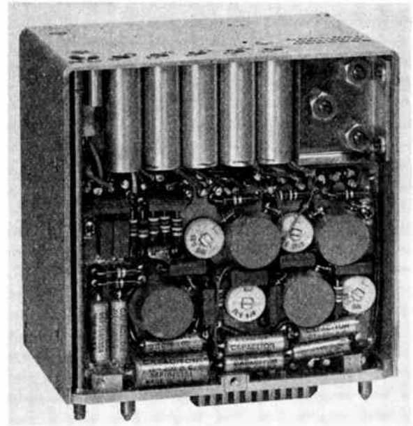
Fig. 10—Photograph of a typical airborne reference frequency oscillator.
