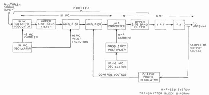
Fig. 17—Transmitter block diagram.
