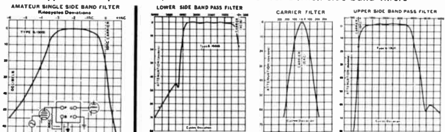
5-15,000 AMATEUR SINGLE SIDE-BAND FILTER
