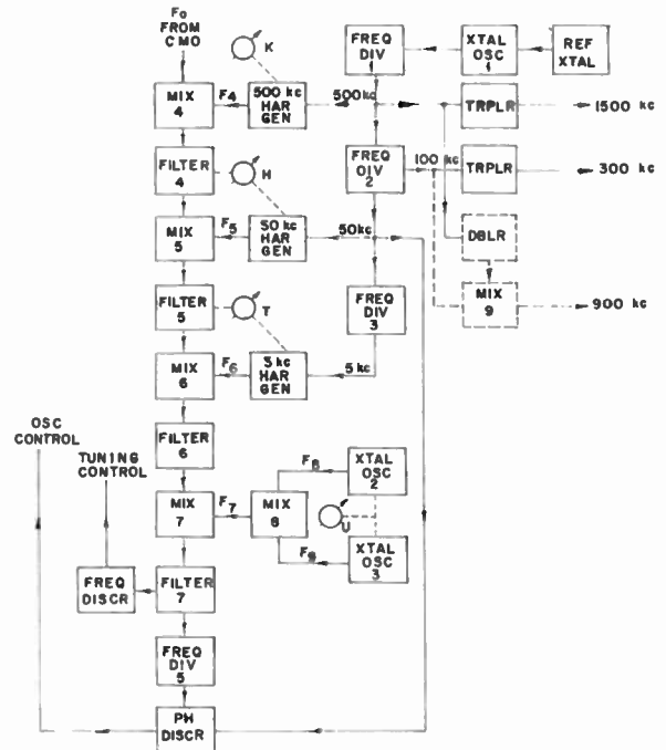
Fig. 5—Block diagram of the frequency-control units.
