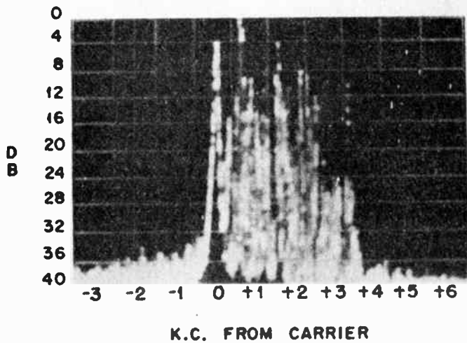
Fig. 10—SSB spectrum input to driver.
