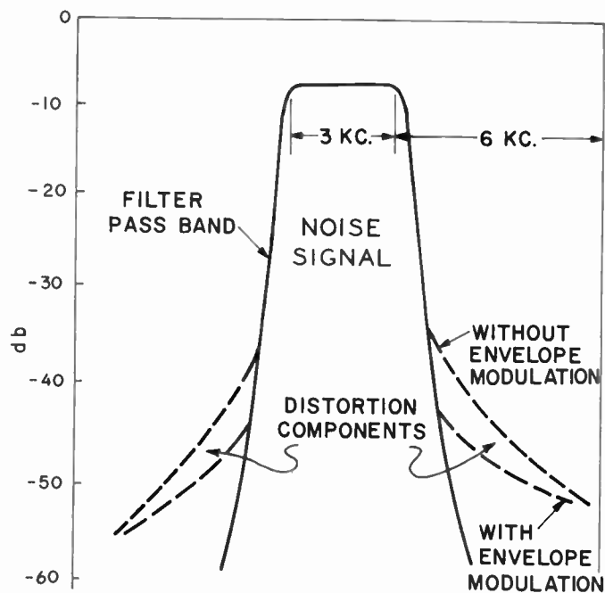
Fig. 12—Distortion components with and without envelope modulation.
