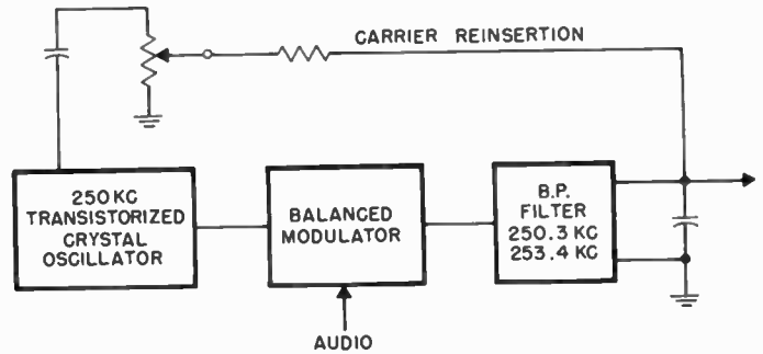
Fig. 12—Method of controlling amount of carrier transmitted.
