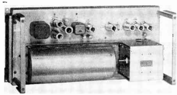
Fig. 5—Photograph of a typical reference frequency oscillator for ground station use.
