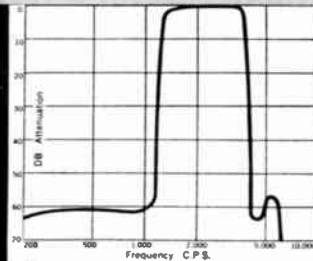
FREQUENCY RESPONSE Typical Band-Pass Filter
