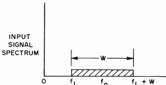
Fig. 4—Input signal spectrum.
