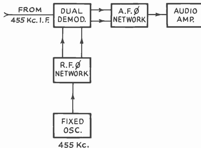
Fig. 6—Phasing-type single-sideband adapter for receivers.
