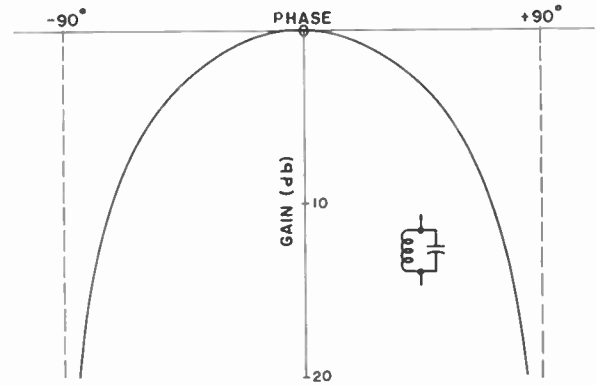
Fig. 3—Phase-gain of infinite Q -tuned circuits.
