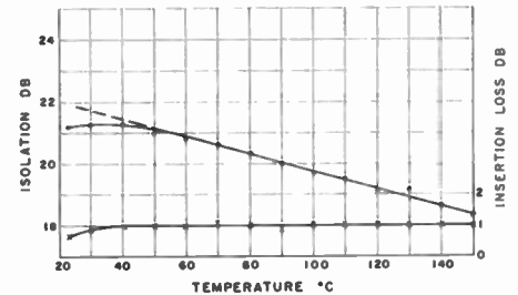
Fig. 3—Switching action is given as a function of temperature for the 1N263. The isolation is shown by the curve using solid dots and the insertion loss is shown by the curve using crosses.
