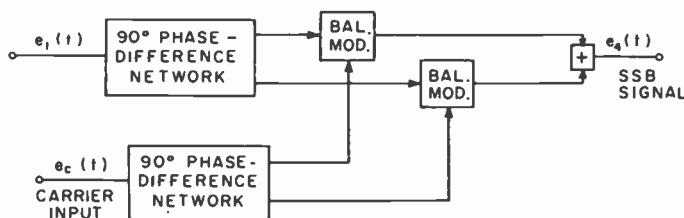
Fig. 4—Phasing method of SSB generation.
