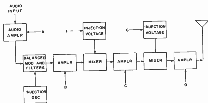
Fig. 7—SSB system gain block diagram.
