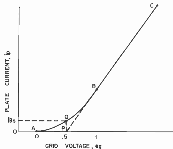
Fig. 4—Ideal tube characteristic for class AB operation.
