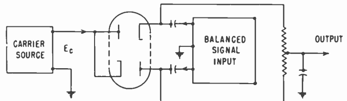
Fig. 5—Example of exalted carrier demodulator suitable for use in the phase-shift method. The two signal sources may be interchanged provided suitable voltage ratios are maintained.
