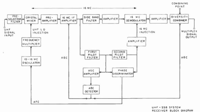
Fig. 29—Receiver block diagram.
