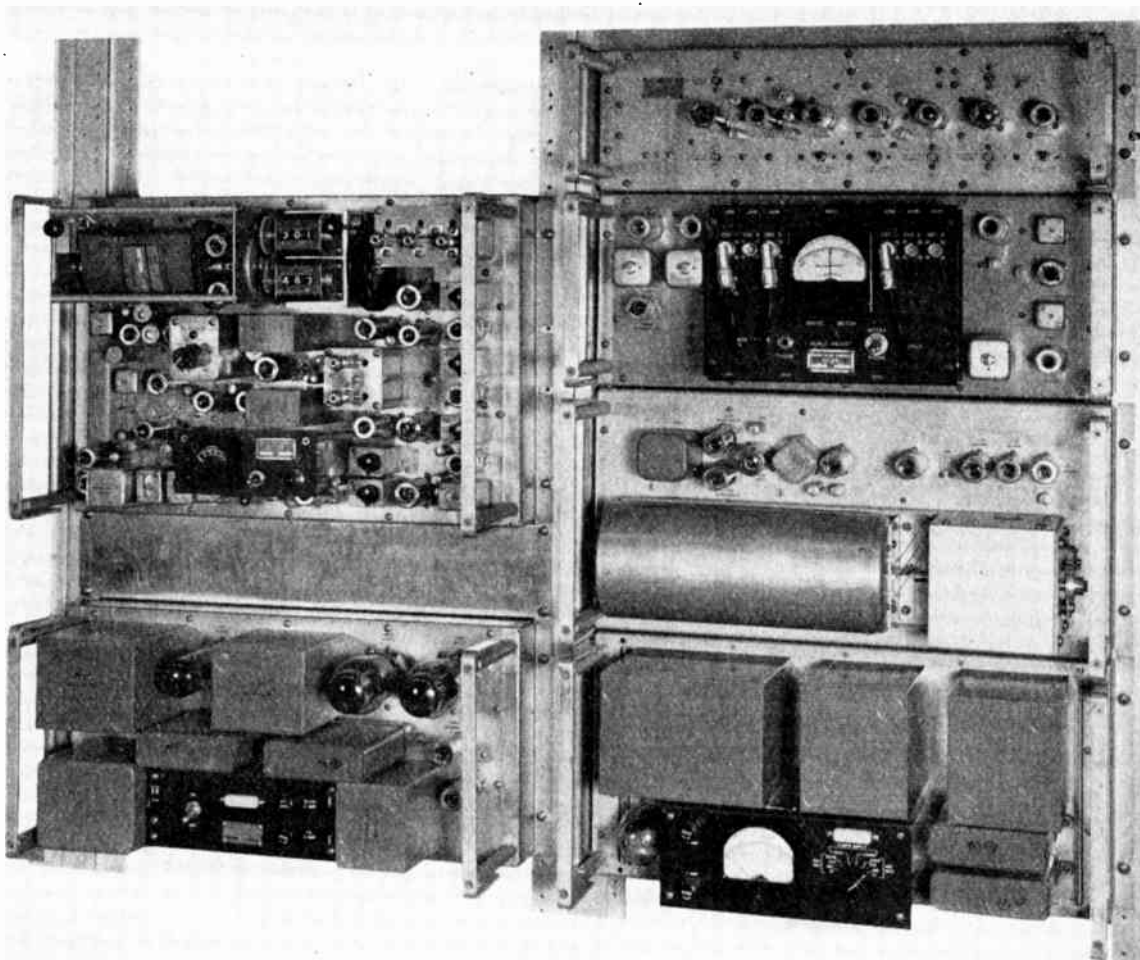
Fig. 2—Frequency generating equipment.
