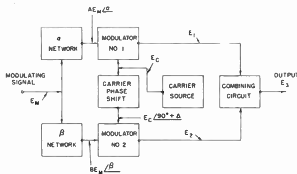
Fig. 2—Practical embodiment of phase-shift method.
