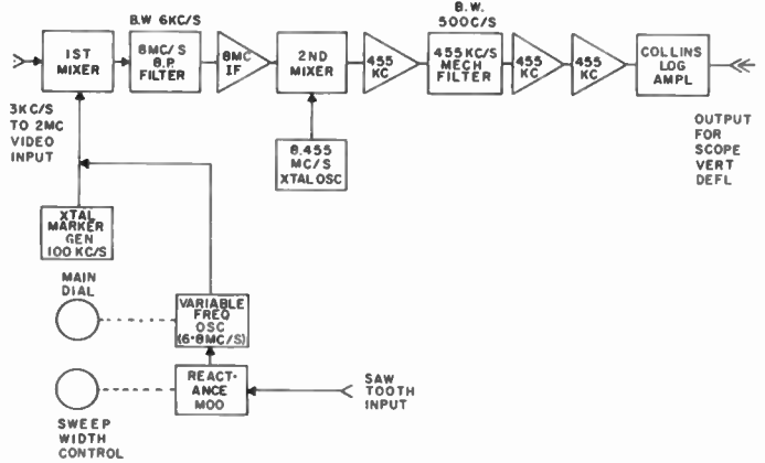
Fig. 9—Base-band (audio-video) spectrum analyzer; block diagram.
