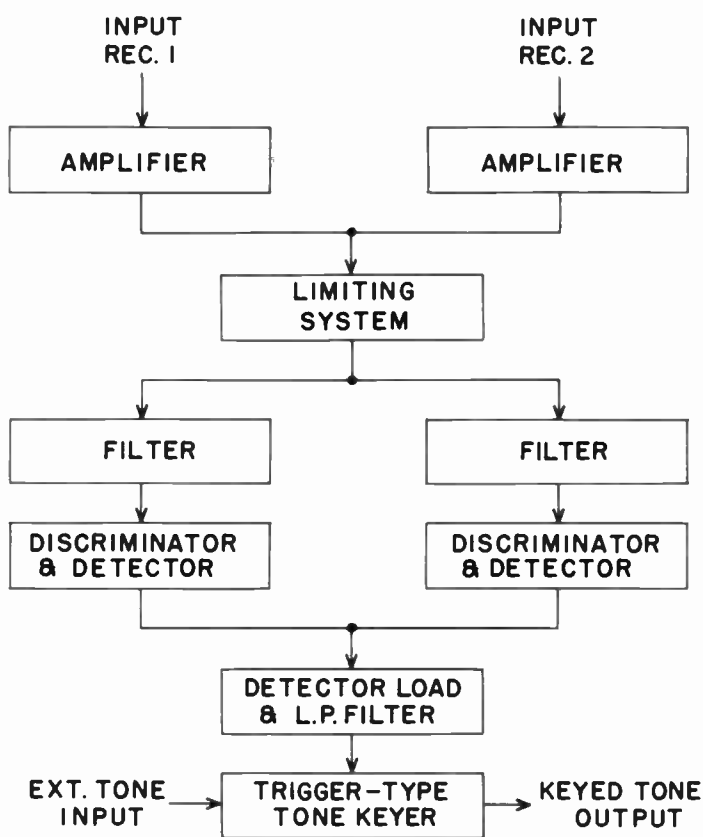
Fig. 6—Block diagram of the individual-channel telegraph combiner.
