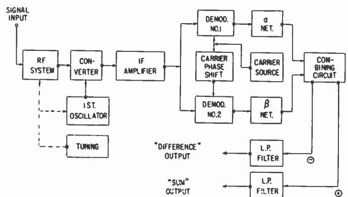
Fig. 3—Typical application of the phase-shift method in a superheterodyne type of receiver. The low-pass filters in output channels define effective bandwidth of each channel.
