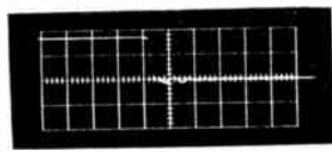
Fig. 2—Recovery characteristic of type S-6 silicon diode operated at avalanche breakdown. Scale: Vert = 0.5 v/cm Horiz = 0.1 μsec/cm.
