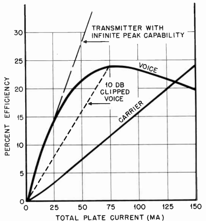
Fig. 15—SSB power amplifier efficiency. Tube: 829 B. E_s = 200 v. Bias = -26 v. Peak power = 140 w.
