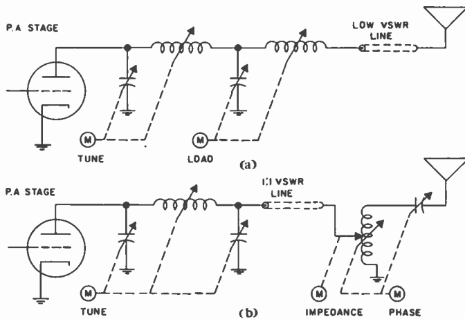
Fig. 5—(a) Pi-L output network. (b) Pi network with external antenna coupler.
