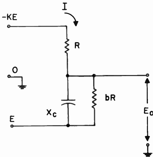
Fig. 10—A modified "basic" phase-shift network.
