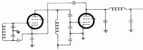
Fig. 1—Two-stage rf power amplifier with feedback.
