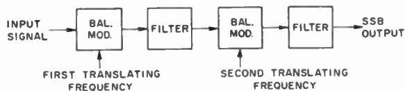
Fig. 1—Filter method of SSB generation.
