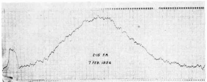
Fig. 1—Transit of sun through antenna beam of 7.5 mm radiometer. One division on time scale equals one-quarter minute.
