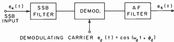
Fig. 3—Demodulation of SSB signal.
