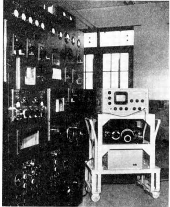
Fig. 5—Transmitter may be operated either linear or Class C using frequency transposition type of exciter. Panoramic equipment for distortion measurement at the right.
