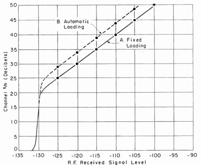
Fig. 14—FM receiver transfer function (6 db N.F., twenty-four channels). Curve A: Fixed Holbrook loading allowance. Curve B: With automatic load control, assuming \tau=0.10 .
