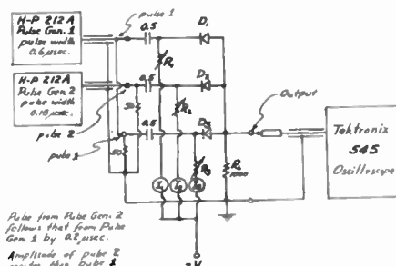
Fig. 3—Three-input diode logical AND circuit.
