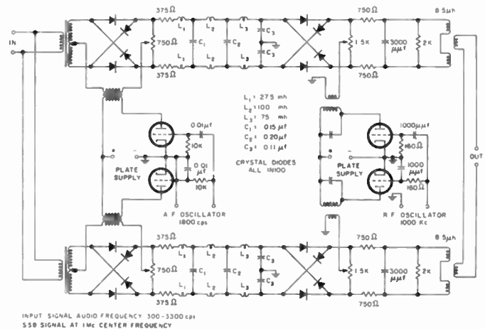
Fig. 7—Single-sideband generator.
