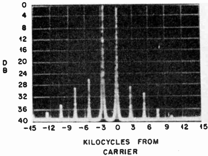
Fig. 4—Two-tone spectrum.
