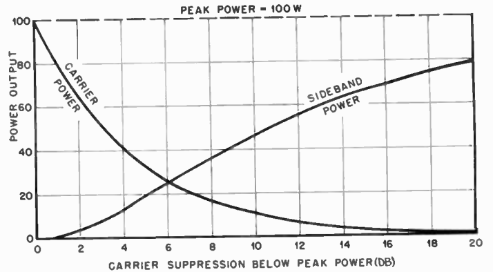
Fig. 13—Variation of sideband power with carrier suppression. (Linear final-peak power limited.)
