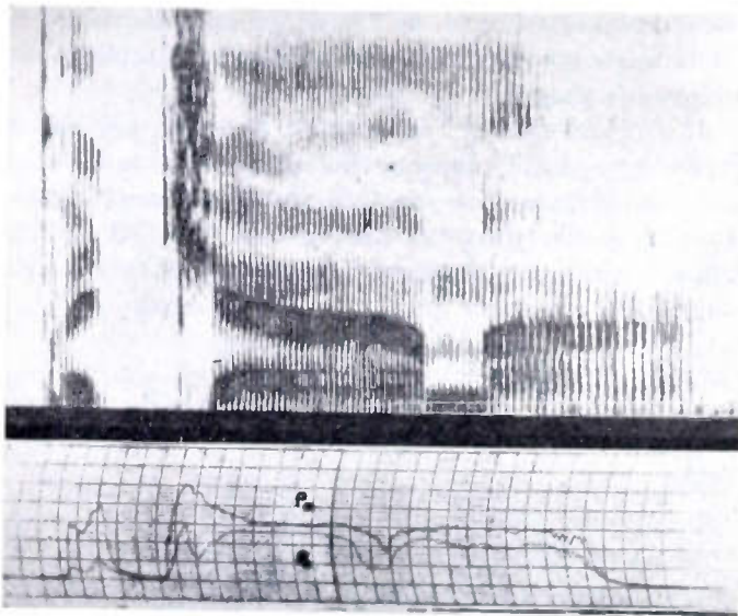
Fig. 3—Spectrogram and P_m and P_0 graphs of "pajama."
