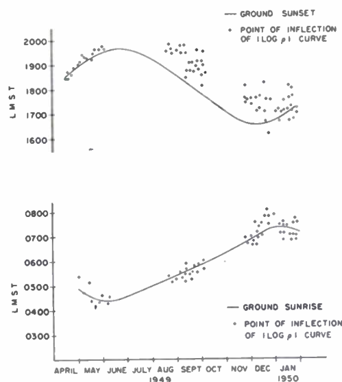
Fig. 4—Sunrise and sunset correlation.
