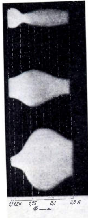
Fig. 3—Experimental inversion spectra of the multiphase systems.
