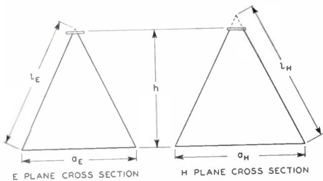
Fig. 2—Nomenclature for horn flared in both planes.
