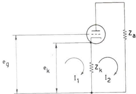
Fig. 5—Amplifier stage with differential input.
