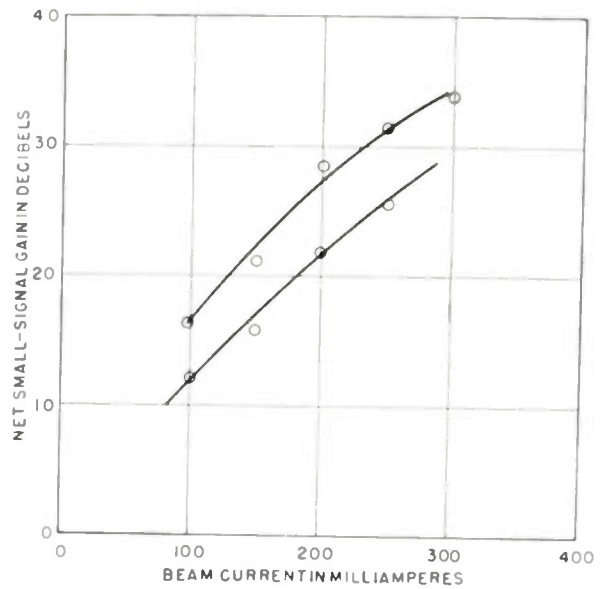
Fig. 9—Small-signal gain plotted against beam current. The values of V_0 in kilovolts and frequency in megacycles for the upper curve are 3.6 and 4,650 and, for the lower curve, 4.6 and 4,550.
