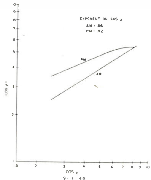
Fig. 3— |\log \rho| versus \cos \chi for 9/11/49.
