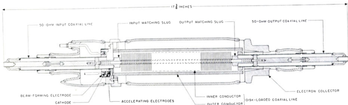
Fig. 7—Experimental tube.
