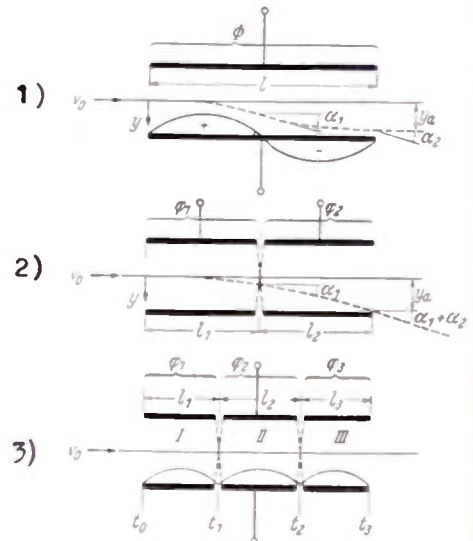
Fig. 1—(1) Single-, (2) two-, and (3) three-phase deflecting field.
