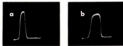
Fig. 2: (a) 0.01 \mu sec pulse through -hp- 460B Amplifier (b) 0.02 \mu sec pulse through 3 amplifiers in cascade
