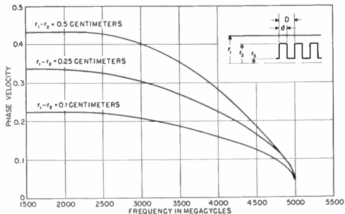
Fig. 3—Approximate theoretical phase velocity for a tube in which d/D = 0.135 and which has dimensions in centimeters of r_2 = 1.2 , r_3 = 0.4 , and D = 0.15 .
