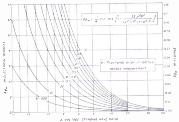
Fig. 4—Curves of maximum error in nodal position determined from positions of equal-response voltages of
