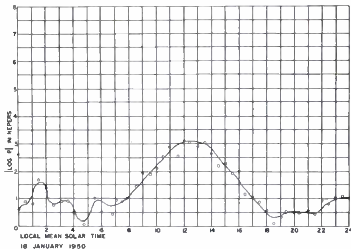
Fig. 1— |\log \rho| versus time for 1/18/50.
