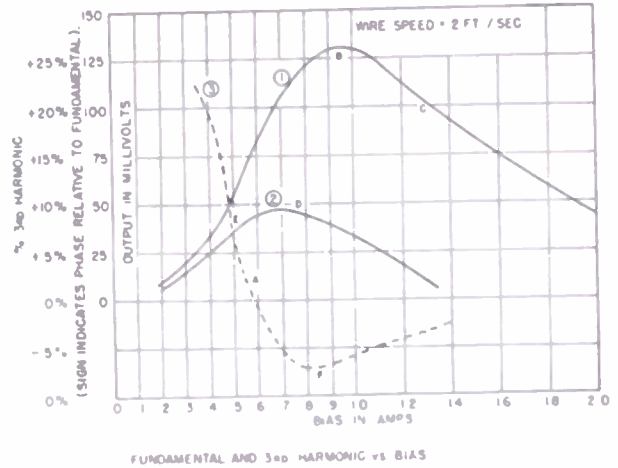
Fig. 4—Experimental results.
