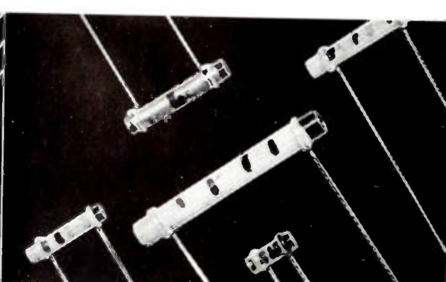
TC (Temperature Compensating) Tubulars—Type TCZ show no capacitance change over wide range of temperature. Type TCN have special ceramic body to vary capacitance according to temperature. Bulletin No. 42-18.
