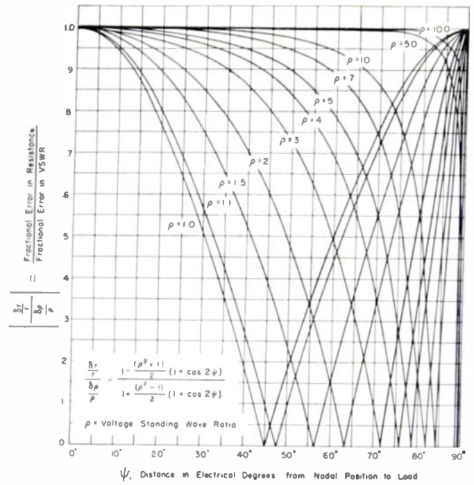
Fig. 5—Curves for determining errors in resistance caused by small errors in measurement of VSWR.
