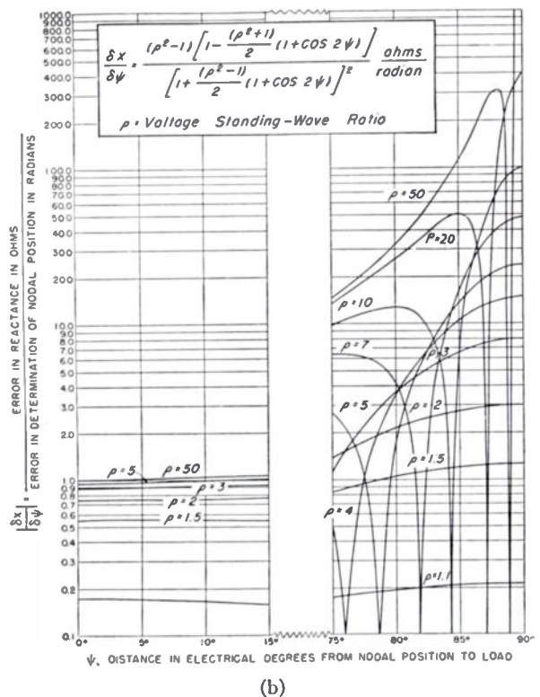
Fig. 8 (b)—Supplementary curves for determining errors in reactance caused by small errors in measurement of nodal position for values of \psi near 0^\circ or 90^\circ .
