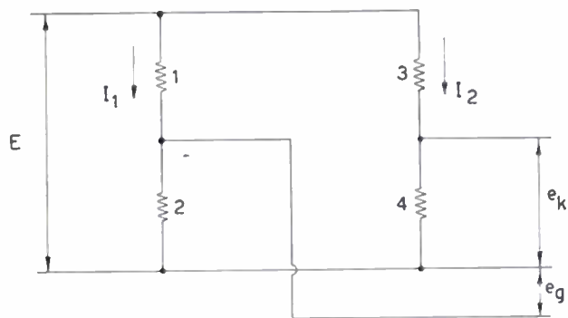
Fig. 7—Bridge circuit connected to the differential amplifier.
