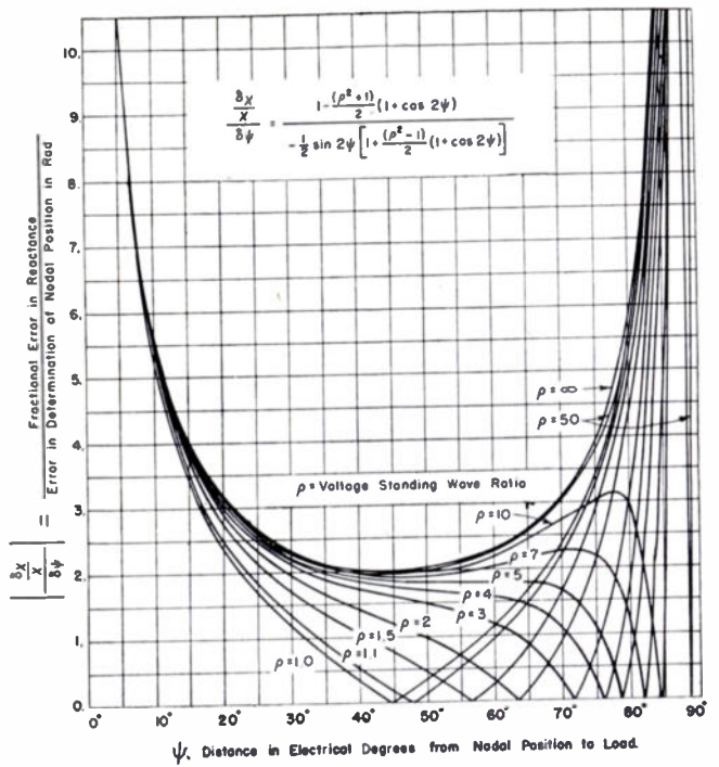
Fig. 8(a)—Curves for determining errors in reactance caused by small errors in measurement of nodal position.
