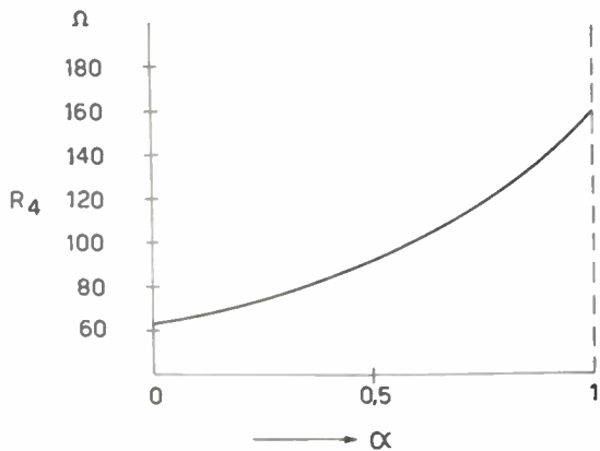
Fig. 6—Cathode input impedance of a differential amplifier stage as a function of voltage ratio \alpha .
