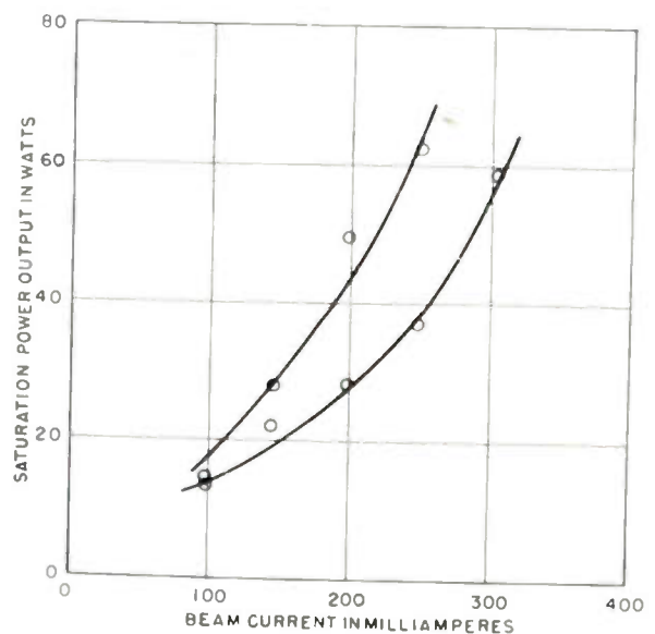
Fig. 10—Saturation power output plotted against beam current. In the upper curve, V_0=4.9 kv, f=4,550 Mc, and the gain is 16.9 db. The values for the lower curve are, respectively, 4.0, 4,650, and 20.
