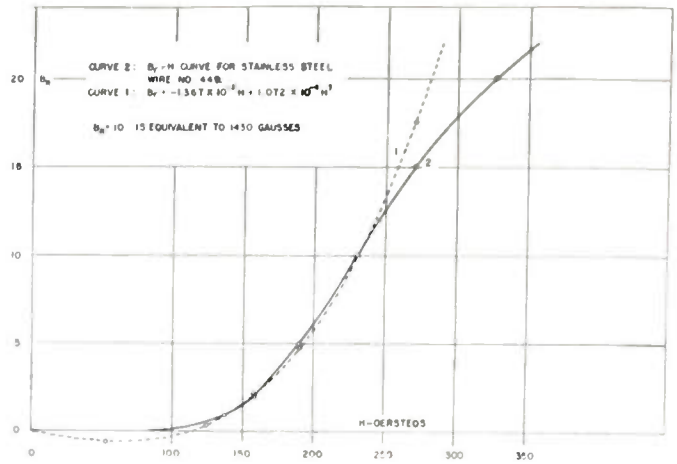
Fig. 2—Cubic or third-order fit to the B_r - H curve.
