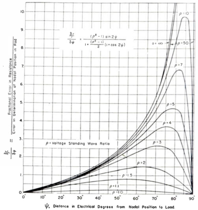
Fig. 6—Curves for determining errors in resistance caused by small errors in measurement of nodal position.
