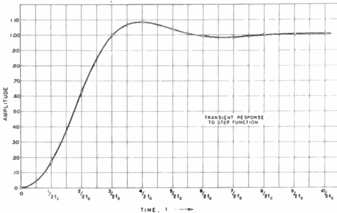
Fig. 3—Transient response curve.
