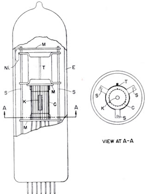
Fig. 1—Sliding target tube.
