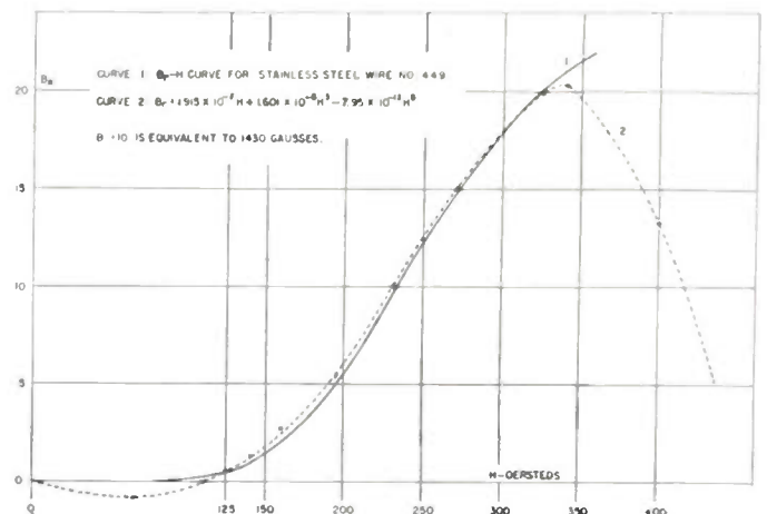
Fig. 3—Fifth-order fit to the B_r - H curve.
