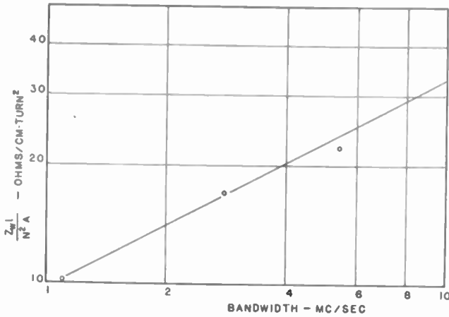
Fig. 8—Wide-band impedance versus bandwidth for 0.002-inch hipersil. Slope of line = 0.5.
