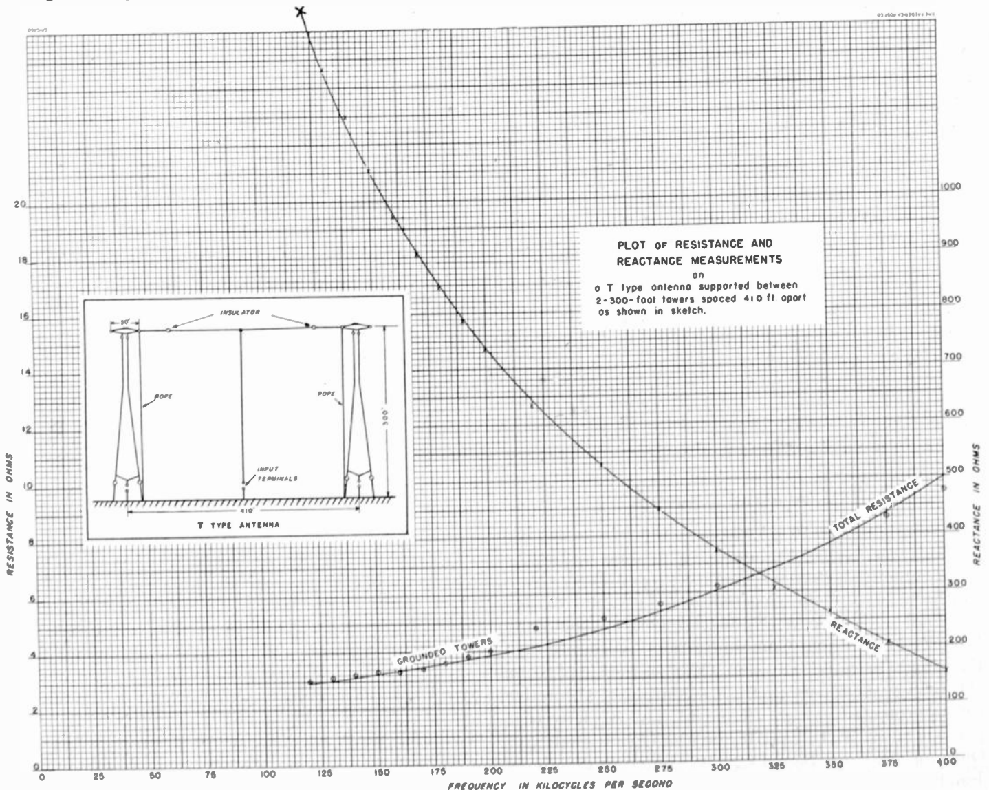
Fig. 15(b)—Plot of resistance and reactance measurements for a T-type antenna.
