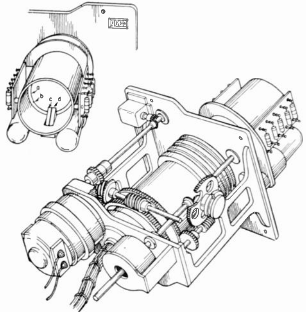
Fig. 9—Perspective view of an automatic range-tracking mechanism employing an intensity-modulated signal displayed on a circular sweep and a photocell tracking system. Intensity-modulated signal (b) is displayed upon the circular trace (a) of a 2-inch cathode-ray tube. Split prisms (c) and (d) reflect light onto type 931 photomultipliers. The photomultiplier assembly is rotatable about the fixed cathode-ray tube by means of a motor-driven worm gear, and the output voltage is obtained through slip rings and is then connected to a power amplifier to drive the motor. Using a circular trace of a 12-microsecond period, an accuracy of roughly 8 yards may be obtained in a full range of several hundred thousand yards. A greater accuracy over a shorter interval may be obtained by employing a circular sweep of a 1.2-microsecond interval. The distance is displayed upon a Veeder-Root counter.
