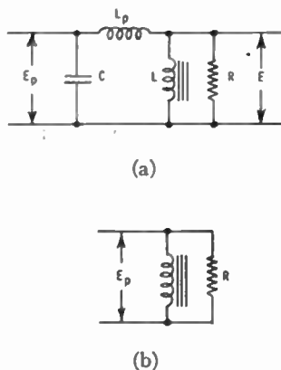
Fig. 2—Equivalent circuits of an iron-core coil.
