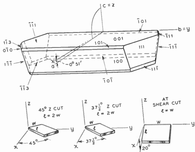
Fig. 16—Zero-temperature-coefficient cuts of DKT crystals.
