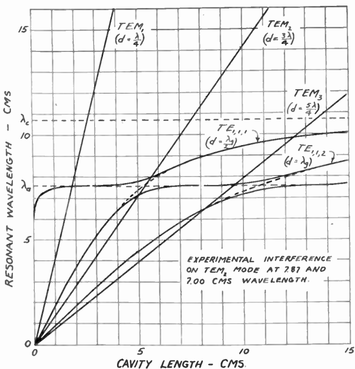
Fig. 7—Calculated TEM and TE_{1,1} resonance characteristics including effect of inner-gap circumferential resonance.
