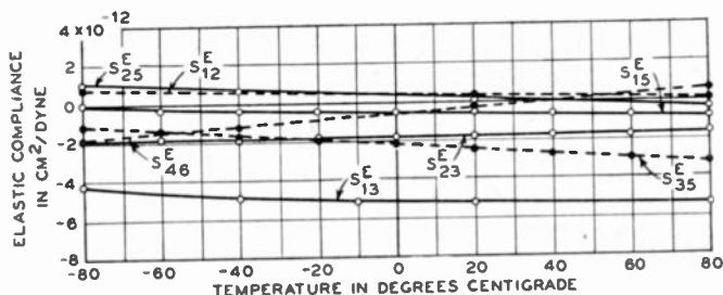
Fig. 5—Cross-coupling elastic compliances for EDT crystals.
