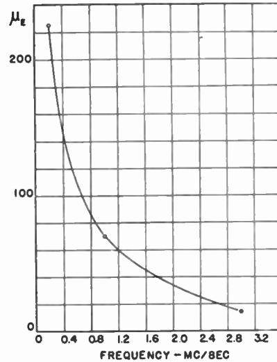
Fig. 18—Dependence of \mu_e of 0.002-inch hipersil on frequency for constant excitation.
