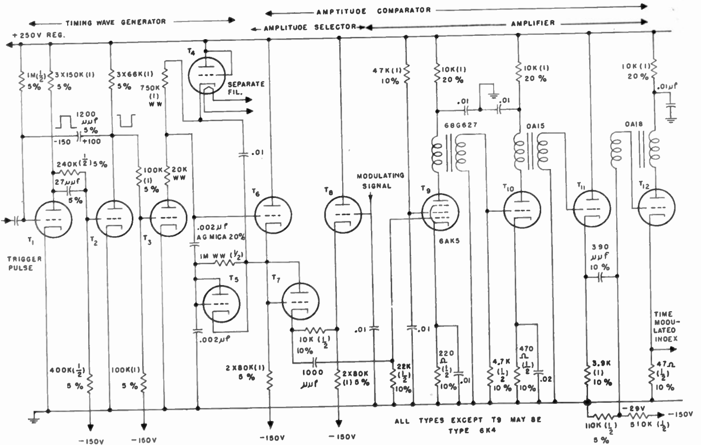
Fig. 12—An accurate time modulator employing a positive-going triangular wave and a diode amplitude selector and regenerative amplifier for amplitude comparison. For the particular constants indicated, this circuit covers a range of 250 microseconds with a linearity of better than 0.1 per cent.
