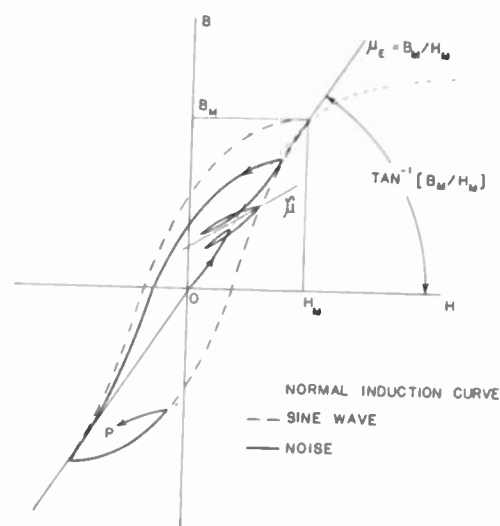
Fig. 1— B - H characteristics.
