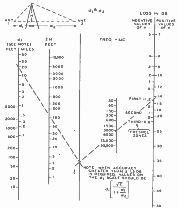
Fig. 8—Shadow loss relative to free space.
