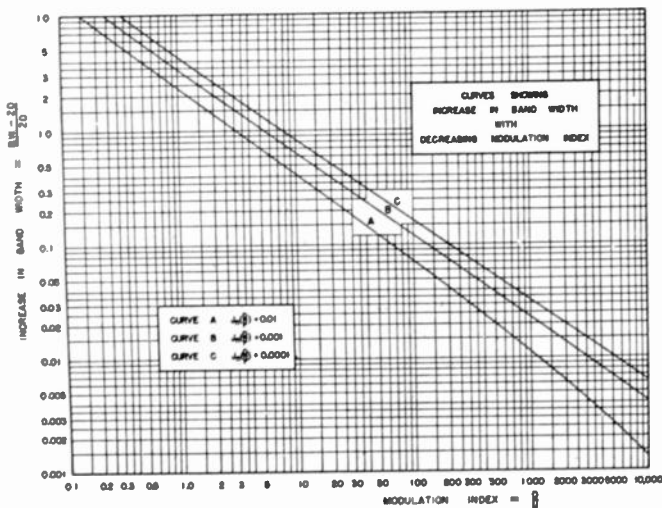
Fig. 5—Variation of bandwidth with modulation index.
