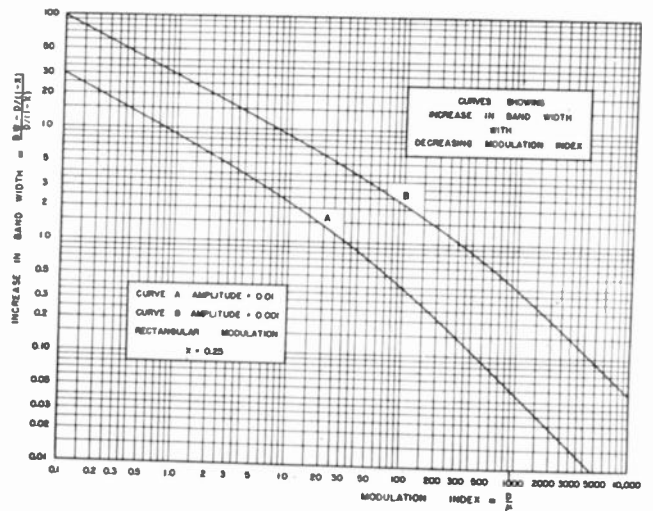
Fig. 12—Variation of bandwidth with modulation index.
