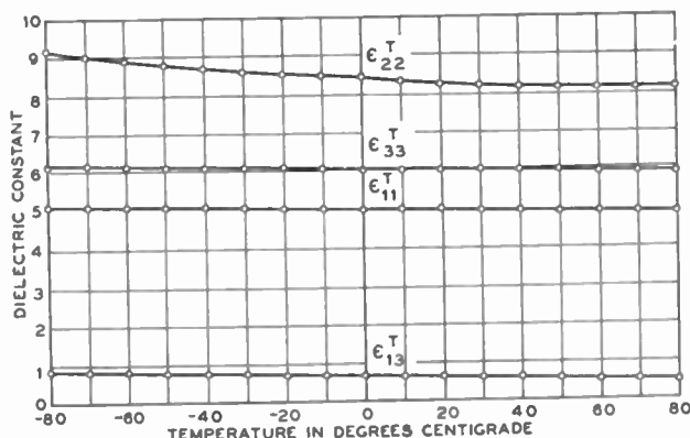
Fig. 7—Four dielectric constants for EDT crystals.
