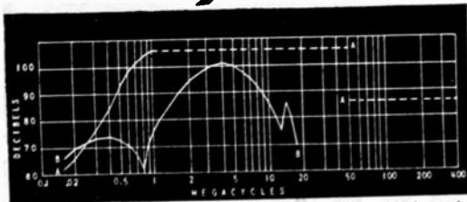
Curve A—Heavy-duty filters; dotted line indicates attenuation beyond range of available measuring equipment. Curve B—Medium-duty filters.
