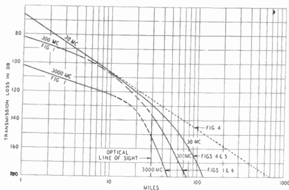
Fig. 11—Transmission over smooth earth at 30, 300, and 300 megacycles; half-wave dipoles at 250 and 30 feet.
