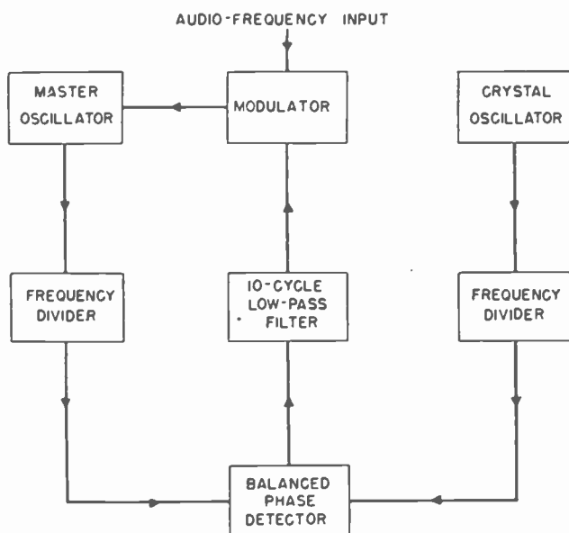
Fig. 2—Schematic diagram of the center-frequency-stabilized modulation system.
