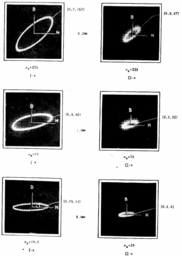
Fig. 16—Sine wave B - H curves for 0.002-inch hipersil for two values of excitation. N = 30 , A = 0.605 centimeter squared, l = 8.85 centimeters. Parentheses indicate peak values of H in oersteds and B in gauss.
