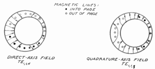
Fig. 9—Two possible TE_{1,1} fields.
