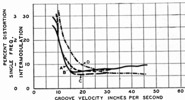
Fig. 5—Comparison of single-frequency and two-frequency (intermodulation) distortion tests. 2.3-mil playback tip radius. A—Single-frequency (400 cycles) distortion, unpolished master B—Single-frequency (400 cycles) distortion, polished master C—Two-frequency (400 and 4000 cycles) distortion, unpolished master D—Two-frequency (400 and 4000 cycles) distortion, polished master.
