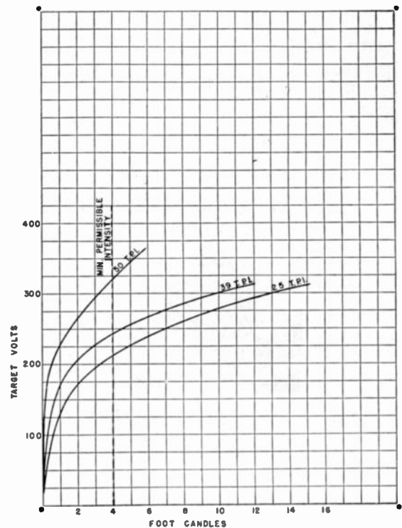
Fig. 3—Brightness as a function of target voltage.
