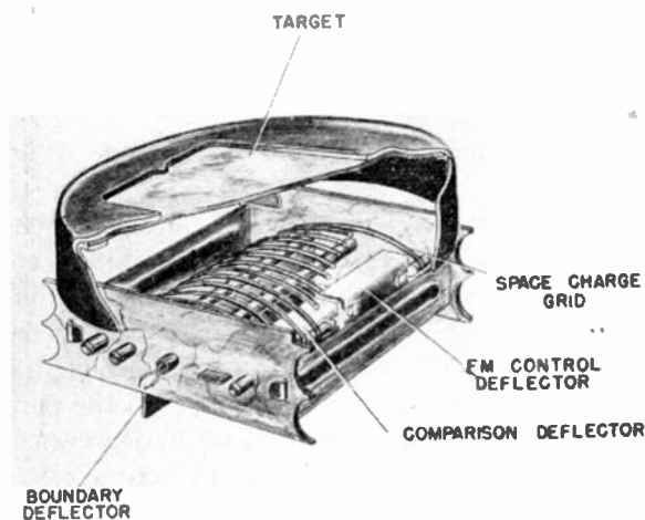
Fig. 1—Space-charge grid and deflector assembly.
