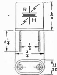
RH-7M Dimensions
