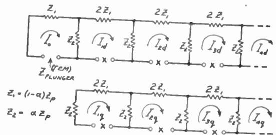
Fig. 10—Equivalent circuit of eccentric plunger.
