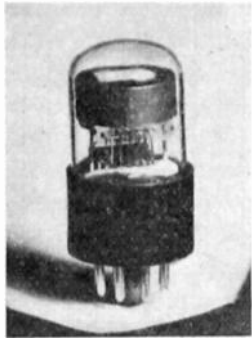
Fig. 4—Photograph of tuning-indicator tube (ZP-601).
