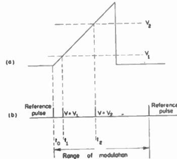
Fig. 11—Electrical time modulation of the spacing between the reference pulse and the pulses occurring at t_1 and t_2 in accordance with the variation of the reference voltage of an amplitude comparator from V_1 to V_2 .
