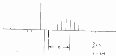
Fig. 10—Spectrum for rectangular modulation.
