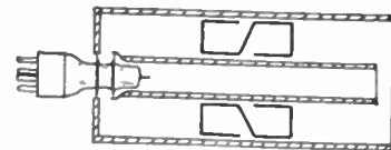
Fig. 1—Coaxial resonator with S plunger.
