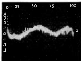
FIGURE 2. Shows performance of modified potentiometer after one million cycles or two million sweeps of PALINEY #7 contact over wire. The initial error was reduced to \pm .12\% and this linearity was maintained throughout the test.
