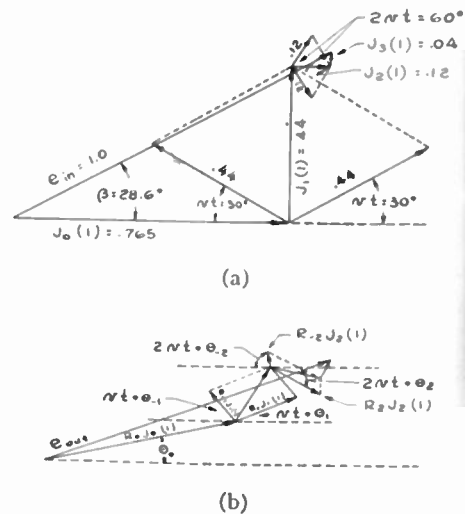
Fig. 1—Vector summation of (a) input signal, and (b) output signal for an arbitrary network (assuming modulation index = 1.0, \nu t = 30^\circ ).
