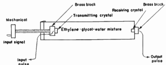
Fig. 18—Electromechanical time modulation obtained from a supersonic delay tank.
