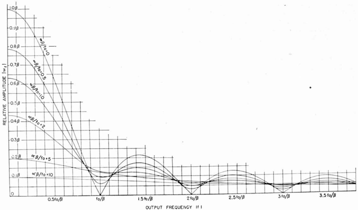
Fig. 3—Relative amplitude versus output frequency. f_0 =generator frequency, \alpha =attenuation constant, \beta =fractional pulse width.
