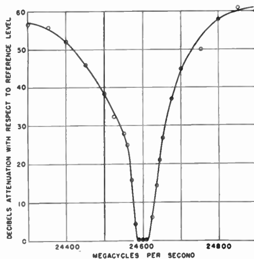
Fig. 8—Attenuation characteristic of filter network.
