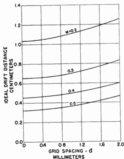
Fig. 4—Effect of grid spacing on S' .
