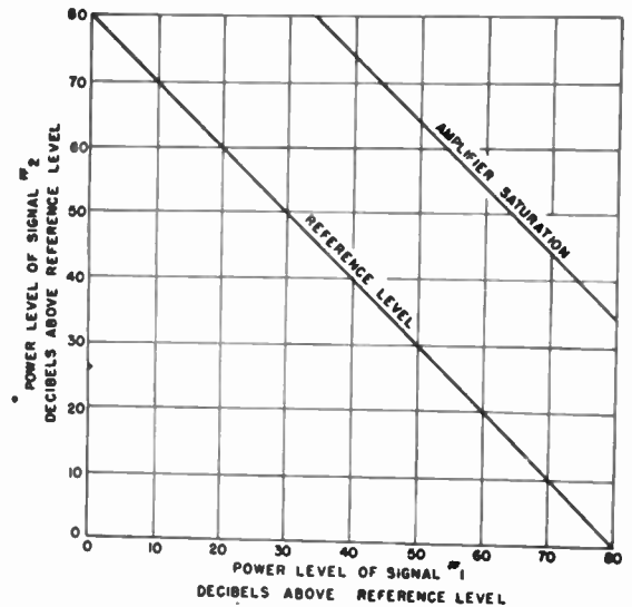
Fig. 6—Response characteristics of the analyzer for typical "cross modulation" of two strong signals in the first mixer crystal. Signal No. 1, 700 megacycles, Signal No. 2, 300 megacycles. Response appears when the analyzer is tuned to 400 megacycles.
