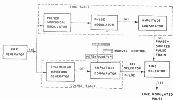
Fig. 20—Block diagram of a double-scale time-modulation system. The over-all accuracy is roughly the product of that of the coarse and fine scales. The two scales are geared together at an appropriate ratio so that a single control of the time-modulated pulse is obtained over the full range of modulation.
