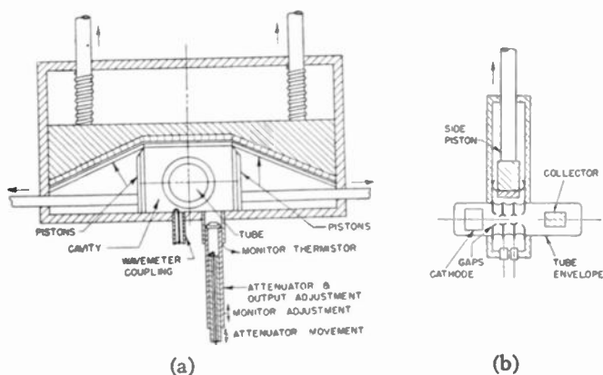
Fig. 7—(a) The oscillator cavity and the attenuator arrangement in the NRL type-F signal generator, showing the cavity-tuning mechanism and the attenuator monitor adjustment. (b) End view of the type-F oscillator cavity showing the position of the 1289 tube.
