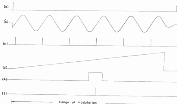
Fig. 21—Wave-form diagram of the double-scale time-modulation system. The pulses at the recurrence frequency are shown in (a), the phase-shifted sinusoid in (b), and the phase-shifted pulse train in (c), (d) shows the triangular timing wave form, (e) the selector pulse, and (f) the selected member of the phase-shifted pulse train. The rate of travel of (c) and (e) are equalized by the gear ratio and the scale factors of the coarse scale.
