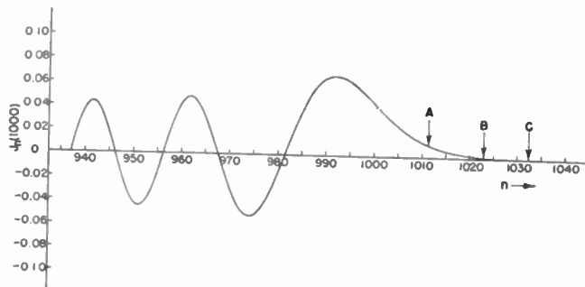
Fig. 2—Graph of J_n(1000) .
