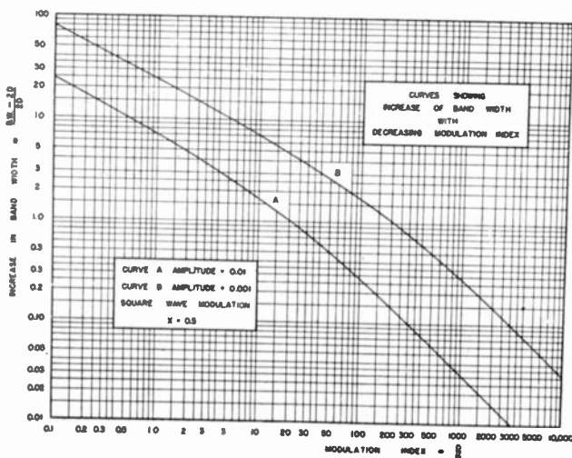
Fig. 11—Variation of bandwidth with modulation index.
