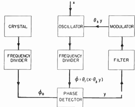
Fig. 10—Center-frequency-stabilizer control loop.
