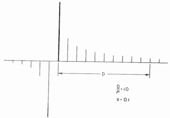
Fig. 18—Spectrum for triangular pulse modulation.
