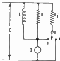
Fig. 3—Circuit for power measurement.
