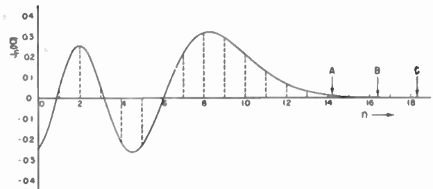
Fig. 1—Graph of J_n(10) .
