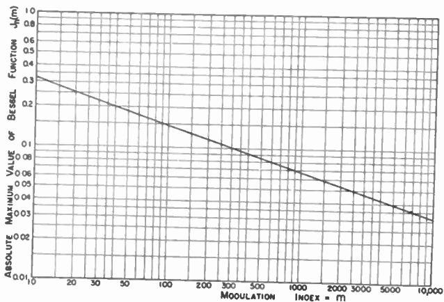
Fig. 3—Absolute maximum value of Bessel function J_n(m) .
