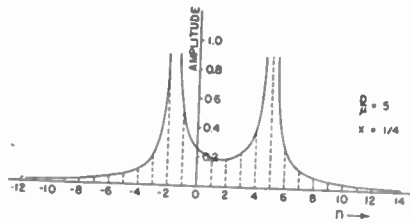
Fig. 9—Limits for side-frequency amplitudes.
