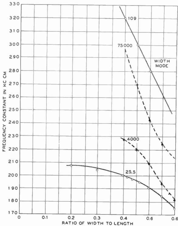
Fig. 13—Frequency spectrum for a Y-cut crystal as a function of the ratio of width to length.
