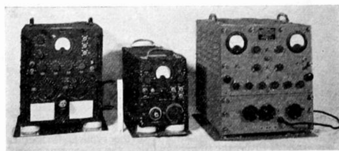
Fig. 1—The Navy-type signal generators. Left to right: LAF (90 to 600 megacycles), LAE (500 to 1350 megacycles), and LAG (1200 to 4000 megacycles).
