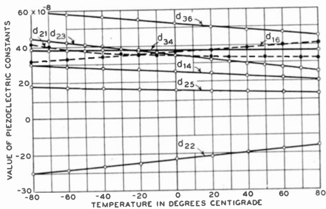
Fig. 6—Eight piezoelectric moduli for EDT crystals.
