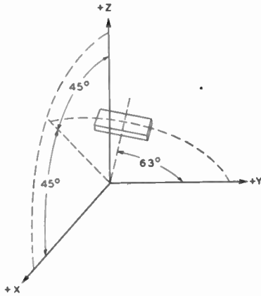
Fig. 9—Orientation for "A"-cut zero-temperature-coefficient crystal.
