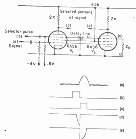
Fig. 6—Adjacent time selectors. The selector pulse is split into two adjacent pulses (b) and (c) of equal duration by delay line L_1 . Portions of the input signal (a) are selected at the plates as indicated at (d) and (e).
