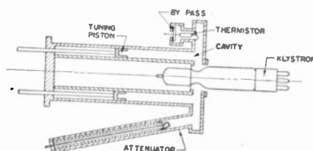
Fig. 6—The oscillator and attenuator assembly of the LAG signal generator.
