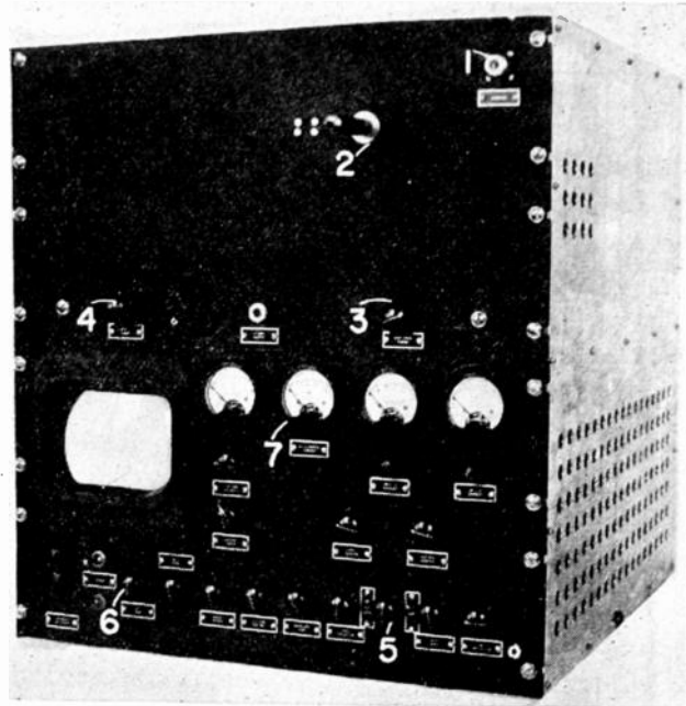
Fig. 1—Front view of analyzer for the frequency range 10 to 3000 megacycles. 1. Signal input. 2. Frequency meter. 3. Main tuning control. 4. Second-beating-oscillator tuning control. 5. "Presentation switch." 6. Gain control. 7. Automatic-frequency-control crystal-current meter.
