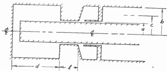
Fig. 5—Idealized coaxial cavity with inner plunger gap.
