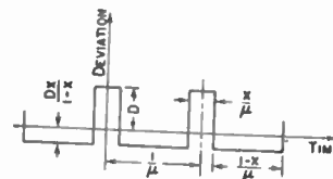
Fig. 7—Modulating signal.
