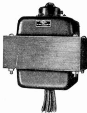
Mounting type 150. 4, hole horizontal mounting. Lead holes on bottom or side of shell. Primary tap changer on top. Ratings 35 to 500 VA.
