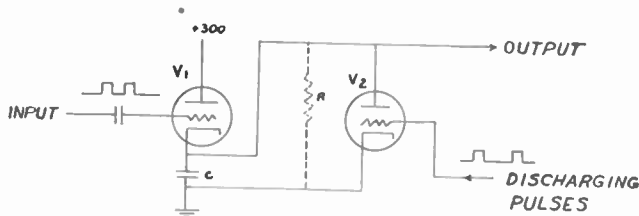
Fig. 4—A pulse-lengthening circuit.
