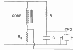
Fig. 15—Circuit for B - H cyclograms.
