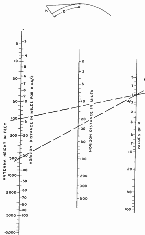
Fig. 7—Distance to the horizon.
