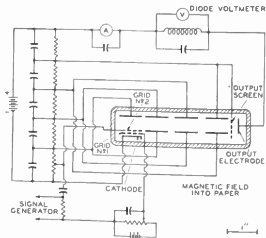
Fig. 1—Magnetic-multiplier setup employed in determination of frequency response.
