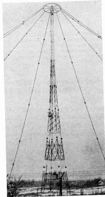
Fig. 4—View of WHK's 300-foot tower with the eight umbrella wires in place.
