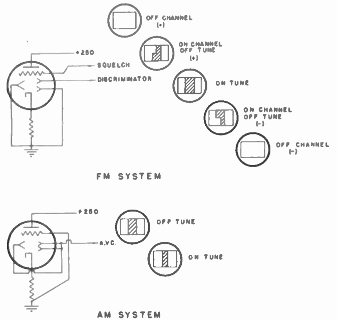
Fig. 5—Circuit diagram and tuning patterns.
