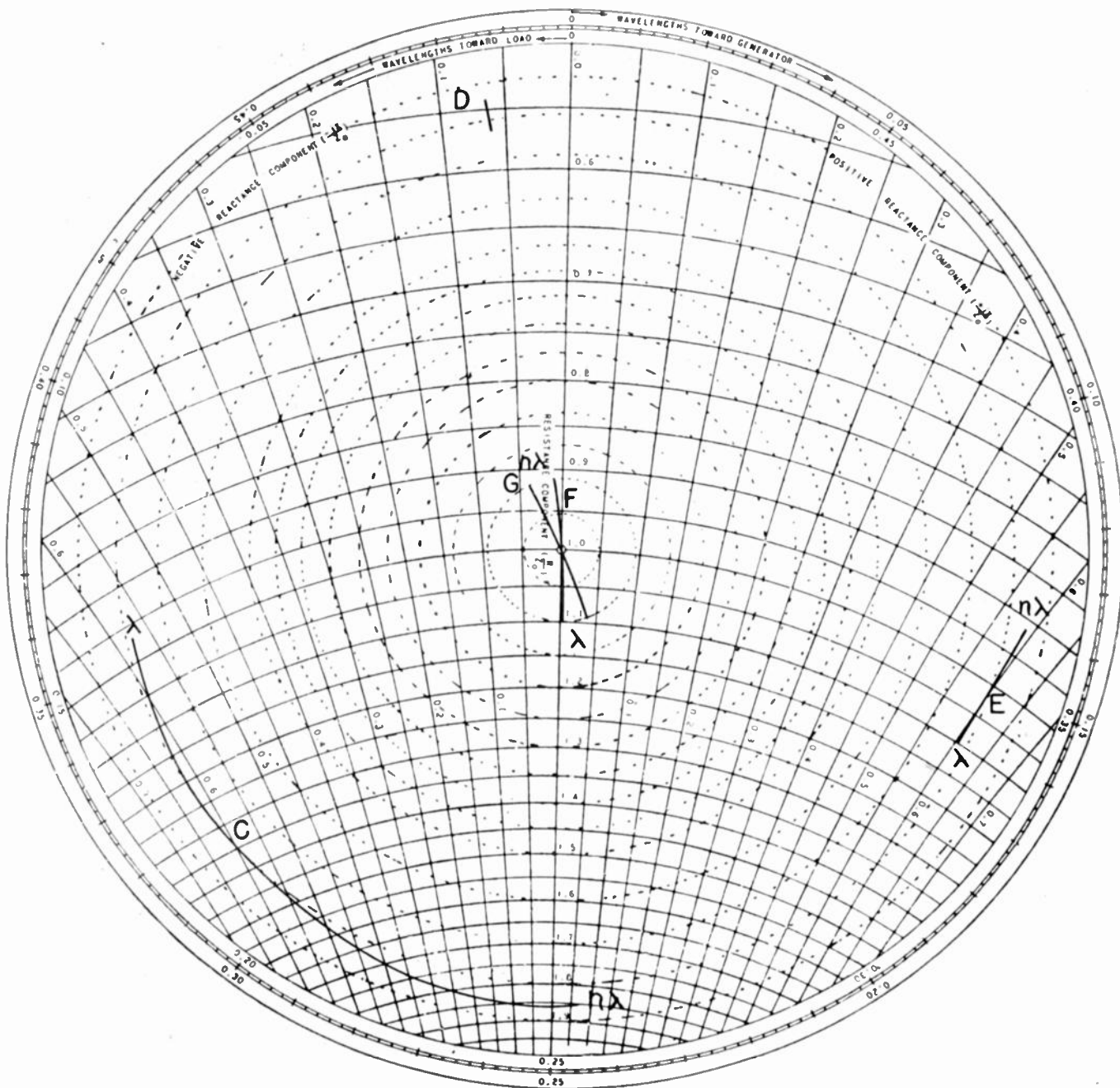
Fig. 3—Enlarged center section of admittance chart.
