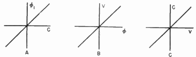
Fig. 11—Center-frequency-stabilizer parameter conversion.
