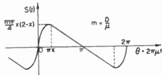
Fig. 15—Variation of phase angle.
