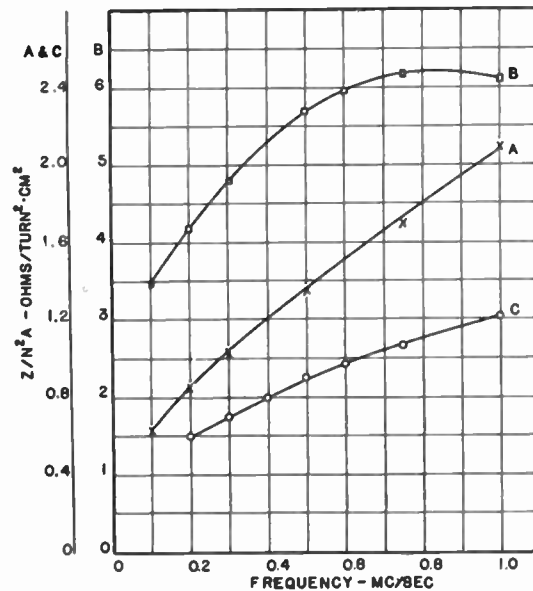
Fig. 7— Z/N^2A versus frequency for three materials.
