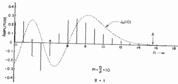
Fig. 16—Spectrum for triangular modulation.
