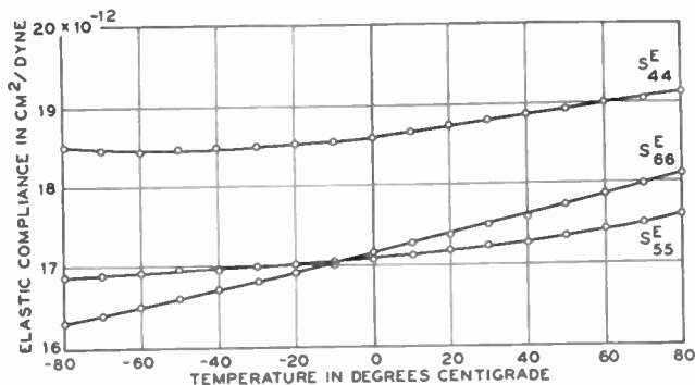
Fig. 4—Shear elastic compliances for EDT crystals.
