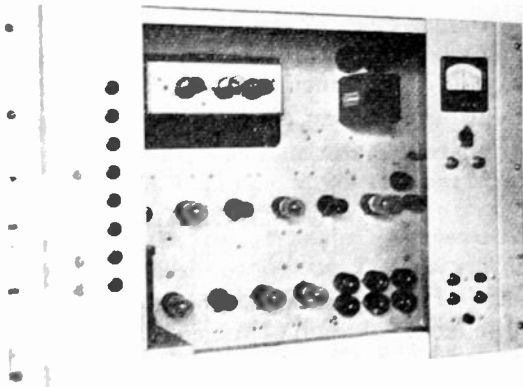
Fig. 7—Federal 1-kilowatt frequency-modulated transmitter. In the upper left is the frequency multiplier and driver stage; next below is the modulator and center-frequency stabilizer. The two lower panels are for the regulated power supply, controls, and contactors. In the lower right is the high-voltage power supply. Above it is the power output stage and the bazooka coupler to the antenna transmission line.
