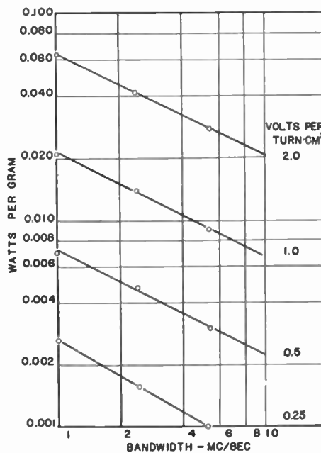
Fig. 12—Core loss versus bandwidth of noise for 0.002-inch hipersil.
