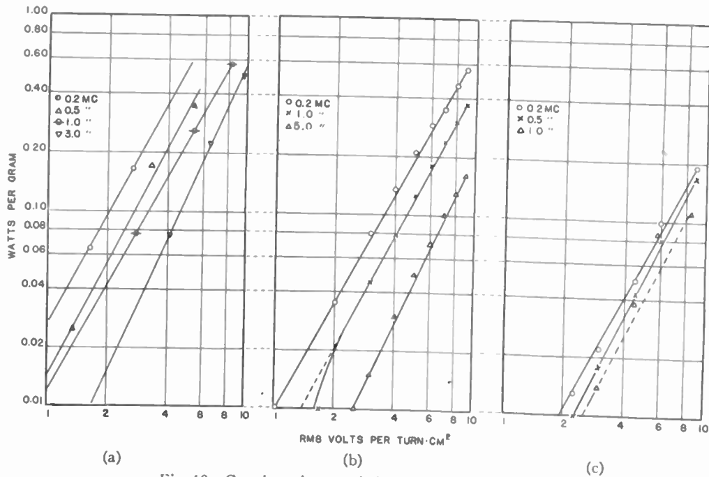
Fig. 10—Core loss characteristics for sine-wave excitation. (a) 0.002-inch hipersil (b) 0.001-inch hipersil (c) 0.001-inch molybdenum permalloy.
