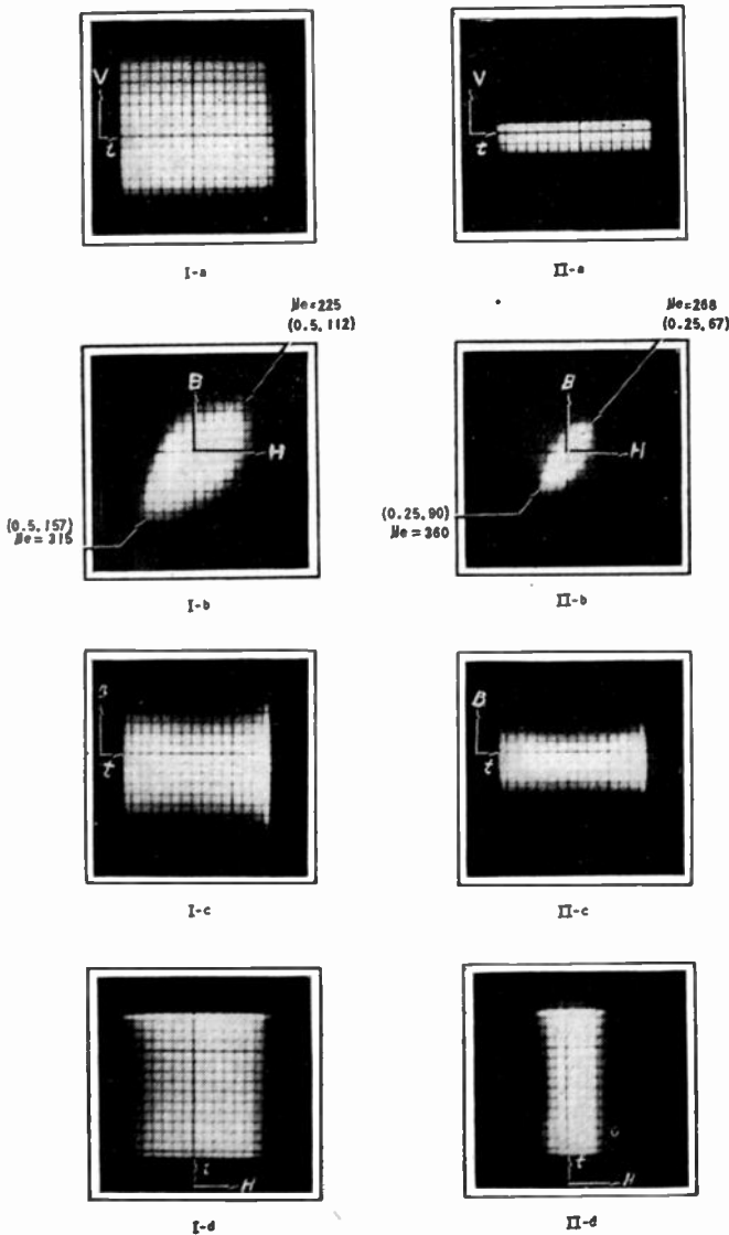
Fig. 17—Noise characteristics of 0.002-inch hipersil. N=30 , A=0.605 centimeter squared, l=8.85 centimeters. Parentheses indicate peak values of H in oersteds, and B in gauss.
