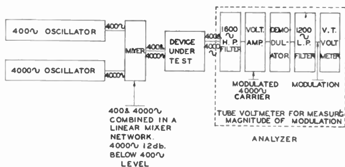
Fig. 1—Intermodulation distortion equipment.
