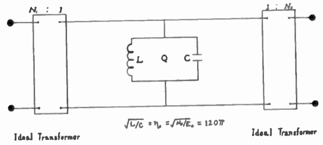
Fig. 1—A unit transducer for one mode.
