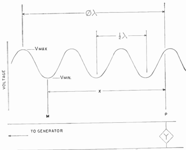
Fig. 2—Standing-wave pattern along the wave guide.
