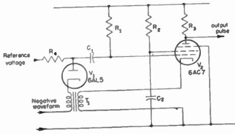
Fig. 10—An amplitude comparator for a negative-going wave. T_1 is a pulse-differentiating transformer.
