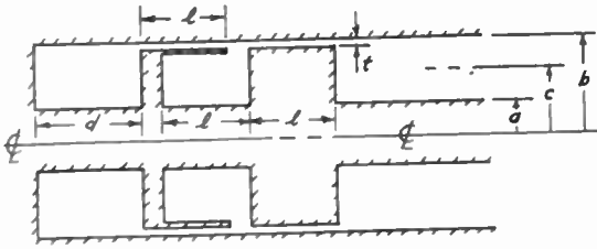
Fig. 2—Conventionalized cavity and plunger for outer-gap resonance.
