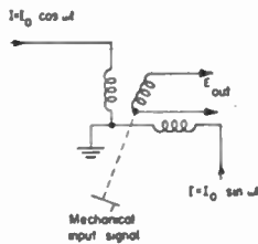
Fig. 14—A synchro used for continuous phase modulation. An accuracy of somewhat better than 1/2 degree is obtained with Bendix autosyns.
