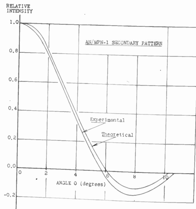
Fig. 3.—The calculated and experimental secondary polar pattern of the AN/MPN-1 radar.
