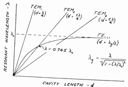
Fig. 6—Simultaneous resonance of the TE_{1,1} and TEM_2 modes in a coaxial cavity.
