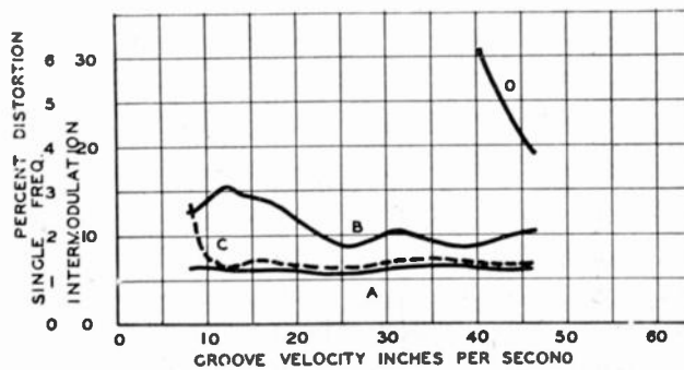
Fig. 6—Comparison of single-frequency and two-frequency (intermodulation) distortion tests. 1.2-mil playback tip radius. A—Single-frequency (400 cycles) distortion, unpolished master B—Single-frequency (400 cycles) distortion, polished master C—Two-frequency (400 and 4000 cycles) distortion, unpolished master D—Two-frequency (400 and 4000 cycles) distortion, polished master.
