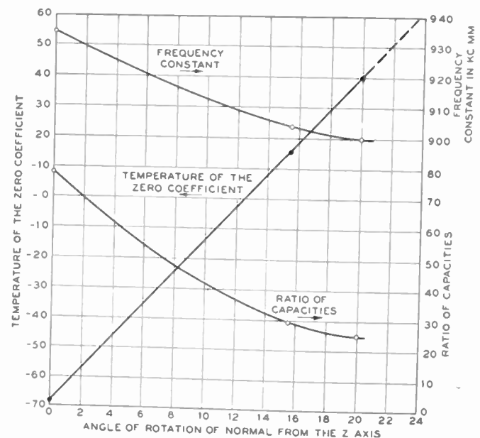
Fig. 19—Effect of angle of rotation on the frequency constant, ratio of capacitances, and temperature of zero coefficient for a thickness-vibrating EDT crystal.
