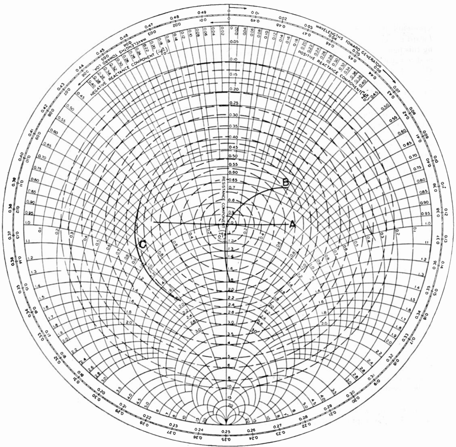
Fig. 4—Smith admittance chart.
