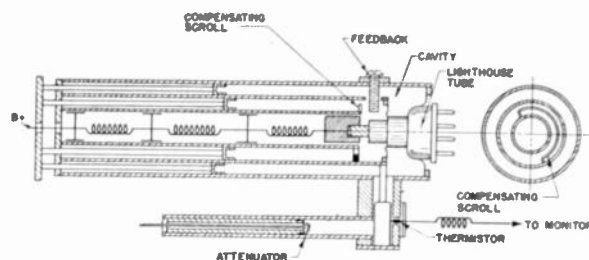
Fig. 4—A schematic drawing of the oscillator and attenuator assembly for the LAE model.
