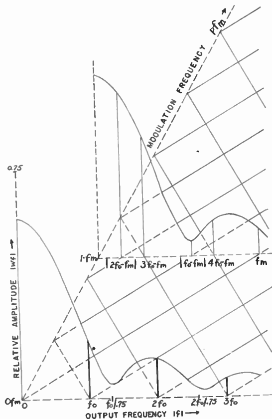
Fig. 5—Relative amplitudes of output terms. Attenuation constant \alpha=2f_0/3 , pulse width \beta/f_0=3/4f_0 .
