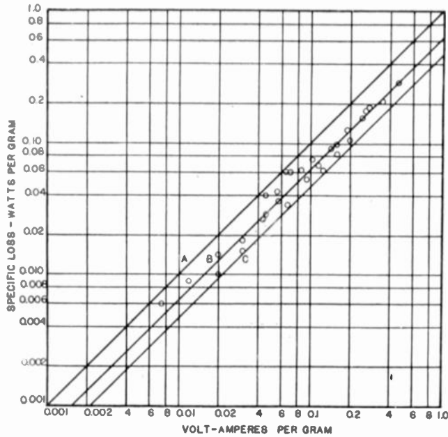
Fig. 13—Specific losses as function of specific volt-amperes for 0.002-inch hipersil. (A) Power factor = 1.000 (B) Power factor = 0.690 (C) Power factor = 0.465.
