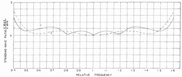
Fig. 6(a)—Standing-wave ratio in a 150-ohm balanced line connected by means of a balun to a 50-ohm single-ended line with two quarter-wave matching sections.
