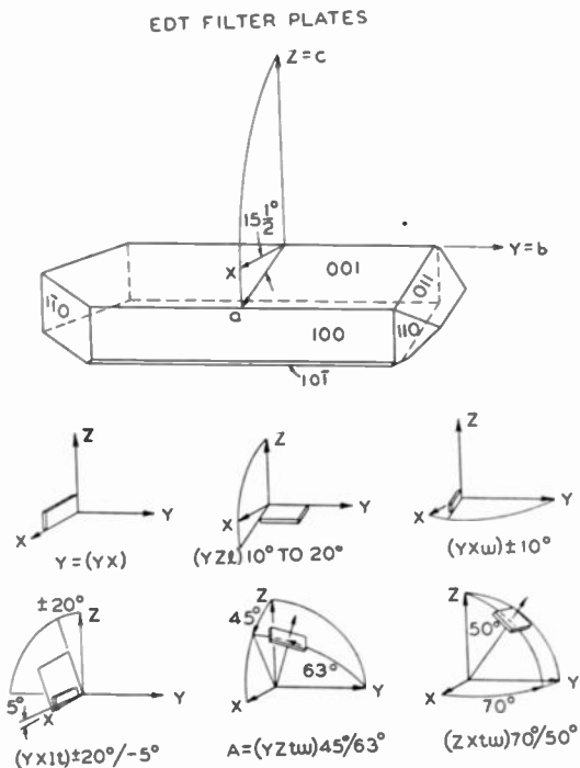
Fig. 15—Zero-temperature-coefficient cuts for EDT crystals.
