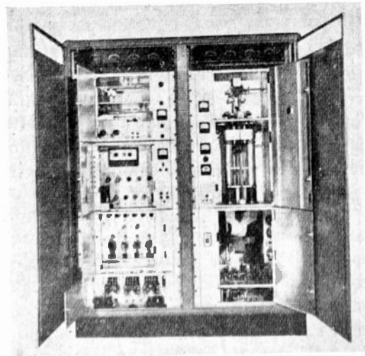
Fig. 9—Center-frequency-stabilized frequency-modulation unit, rear view.
