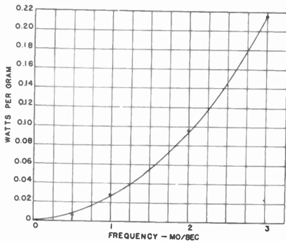
Fig. 14—Eddy-current loss for 0.002-inch hipersil with sine-wave excitation; B = 400 gauss.
