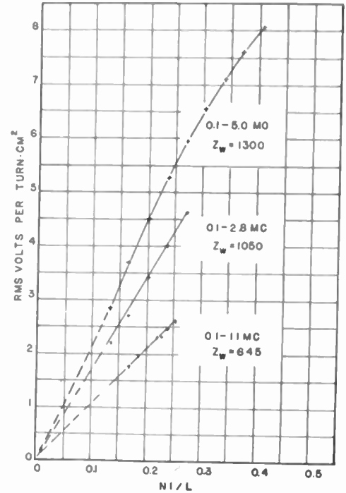
Fig. 9—Wide-band excitation characteristics for 0.002-inch hipersil. N =turns; l =root-mean-square exciting current; l =mean core length.
