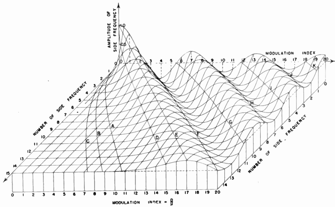
Fig. 4—Side-frequency amplitudes.
