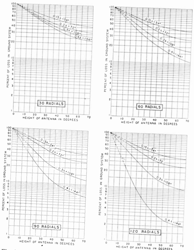
Fig. 3—Per cent power loss in the ground system for various lengths of buried-copper-wire radials, as identified on the curves, plotted as a function of antenna height for the indicated number of radials.
