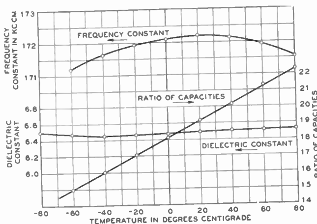
Fig. 17—Frequency constant, ratio of capacitances and dielectric constant for a 45^\circ Z-cut DKT crystal.
