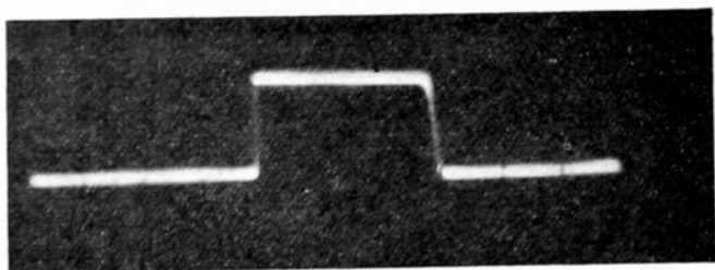
Fig. 11—The "unmodulated" radio-frequency pulse (rectified).
