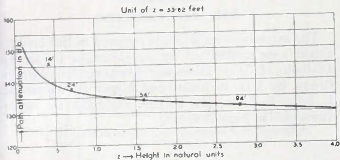
Fig. 9—Theoretical and observed vertical distribution of intensity of Antigua experiment at a range of 20 miles. Wavelength = 10 centimeters M + M_0 = 0.036h + 12.06 e^{-0.0714h} Y(Z) = Z + 10 e^{-2.4Z} Unit of Z = 33.62 feet — Theoretical x Average observed levels relative to level at 94 feet
