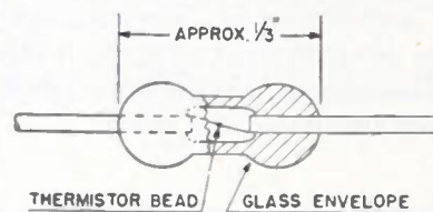
Fig. 3—Bead thermistor used in power measurement.
