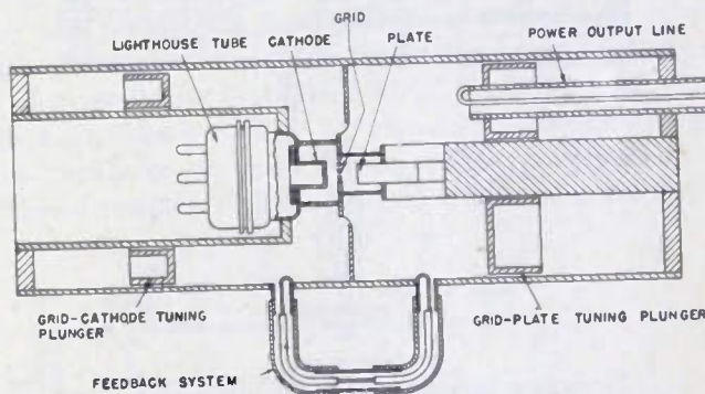
Fig. 3—A typical grid-separation circuit.
