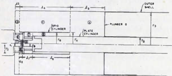
Fig. 20—Re-entrant oscillator.
