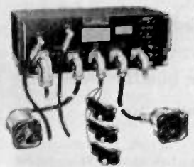
RCA air-borne radar altimeters for every commercial altitude
