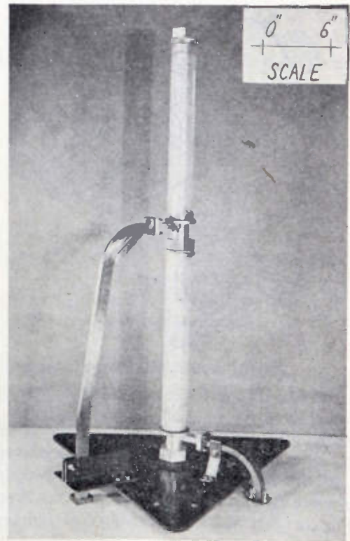
Fig. 8— E_0 wave-guide omnidirectional antenna.
