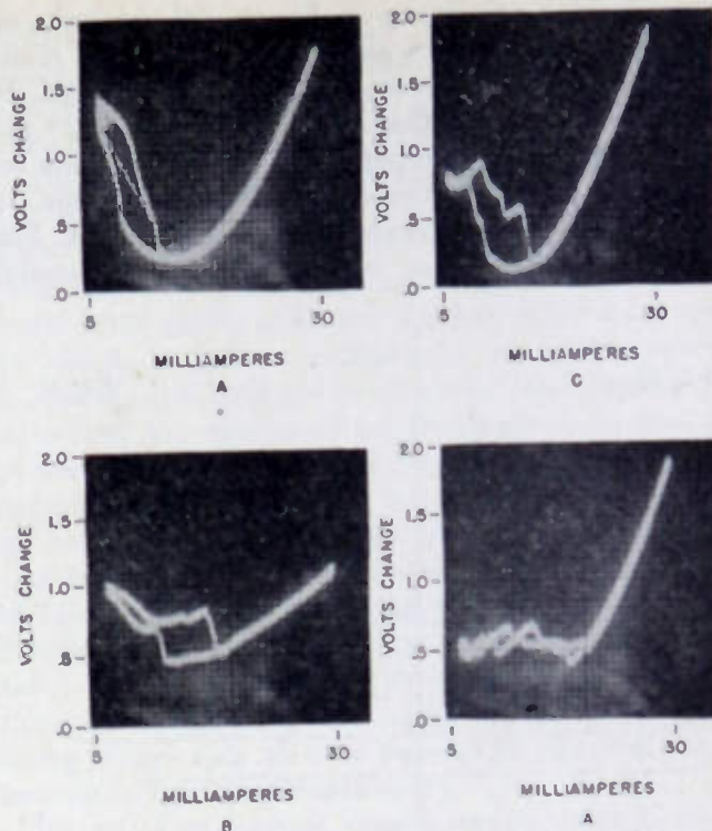
Fig. 6—Regulation characteristics of four VR150 tubes.
