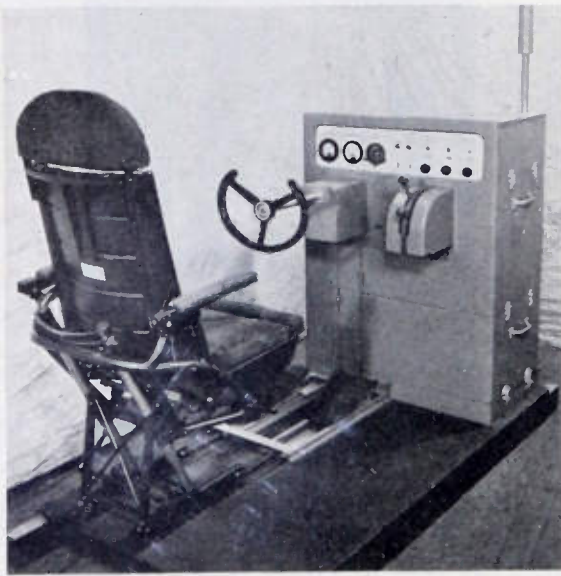
Fig. 6—Ground station.
