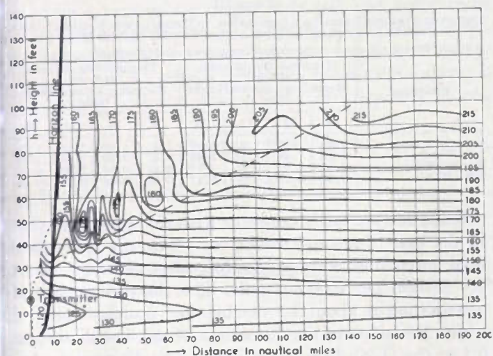
Fig. 5—Theoretical coverage diagram for a transmitter height of 16 feet.
