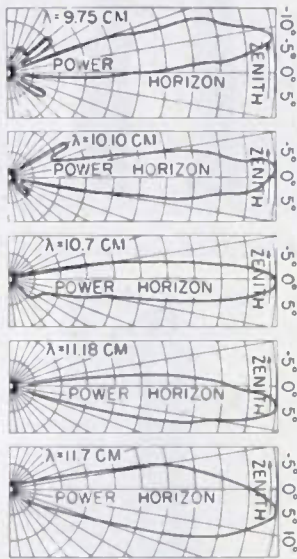
Fig. 6—Elevation patterns of a six-element antenna.
