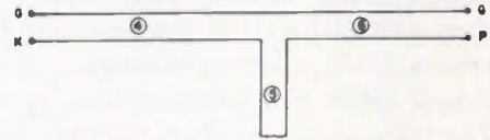
Fig. 21—Elementary equivalent circuit for a basic re-entrant oscillator.
