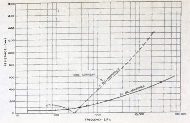
(b) Resistance of a VR105 tube.
