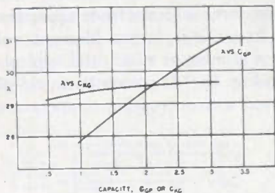
Fig. 27—Calculated curves of wavelength as a function of cathode-grid capacity and of grid-plate capacitance.
