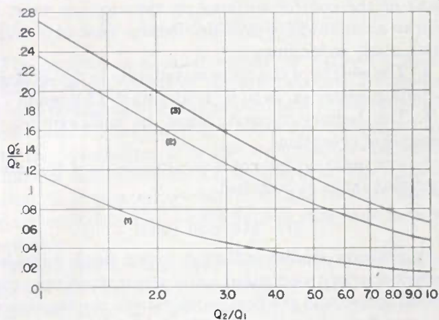
Fig. 12—Apparent Q of the secondary of the coupling transformer. (1) L 1 /L=0.75 Q 1 =10Q k=1.0 (2) L 1 /L=0.75 Q 1 =2Q k=1.0 (3) L 1 /L=0.75 Q 1 =Q k=1.0
