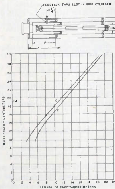
Fig. 10—A wide-range (9 to 30 centimeters) "folded-back" oscillator.
