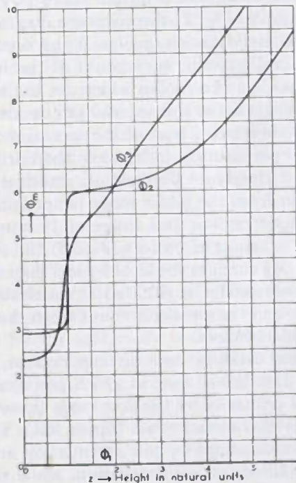
Fig. 8—Phases of the first three normal modes.
