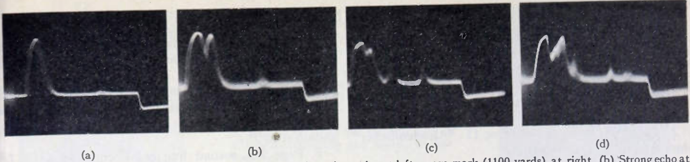
Fig. 1—(a) Taken under normal transmission conditions. Outgoing pulse at left, range mark (1100 yards) at right. (b) Strong echo at 150 yards. (c) Echoes at 100 yards, 325 yards, and 650 yards. (d) Multiple echoes.
