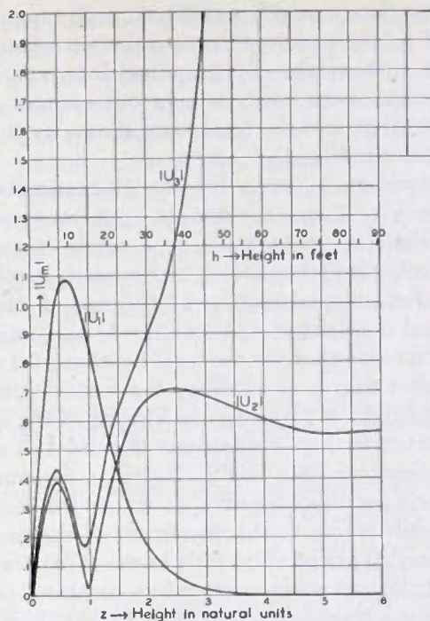
Fig. 7—Height-gain functions |U_m| for the first three normal modes.
