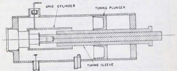
Fig. 13—Re-entrant oscillator with tuning device.
