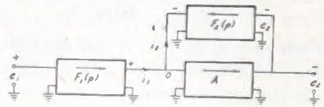
Fig. 5—Generalized circuit for operational computation.
