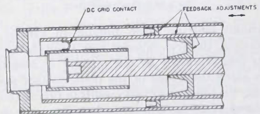
Fig. 14—A modified re-entrant oscillator.
