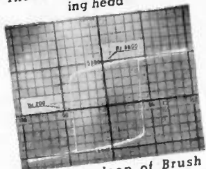
Hysteresis loop of Brush plated wire
