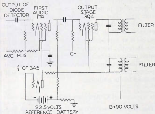
Fig. 8—Schematic diagram of compensating circuit.
