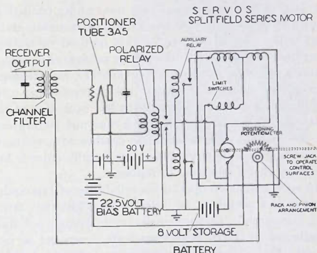
Fig. 10—Schematic diagram of positioning system.
