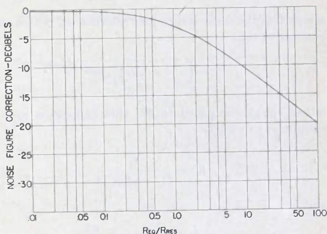
Fig. 9—Noise-figure correction variation with R_{eq}/R_{res} .
