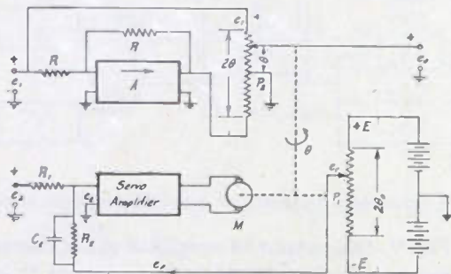
Fig. 10—Servomultiplier circuit.
