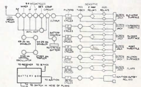
Fig. 1—Functional diagram of airplane installation.
