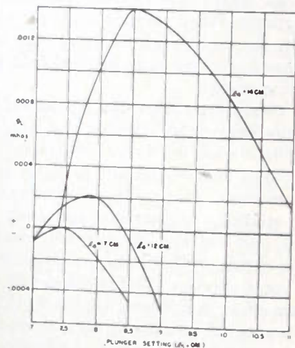
Fig. 26—Load conductance as a function of plunger setting with grid-cathode line l_4 as a parameter.
