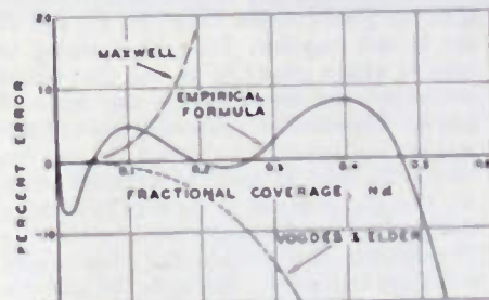
Fig. 1—Curve showing error of proposed empirical formula compared with the inexact theoretical formulas of Maxwell and Vogdes and Elder for amplification factor.
