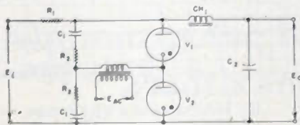
Fig. 2—Balanced circuit for use with two VR105 tubes.
