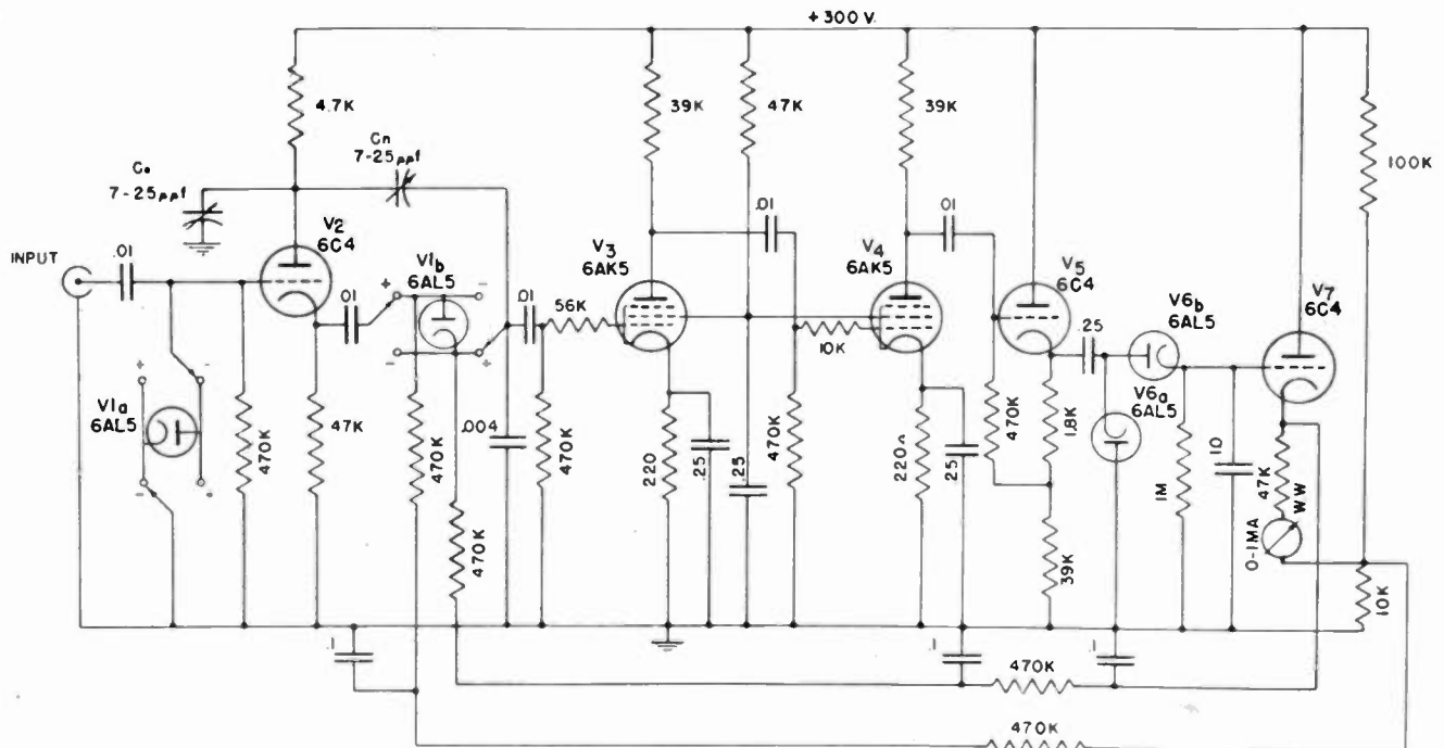
Fig. 4—A more refined circuit of a peak voltmeter for positive and negative pulses.
