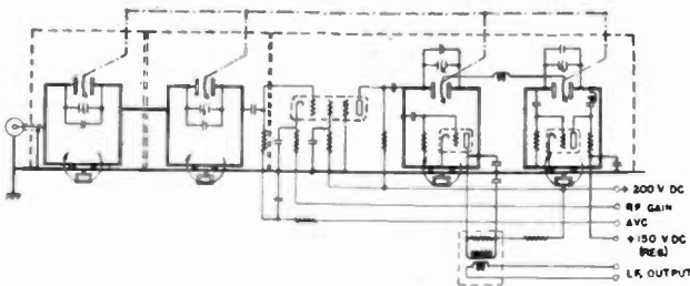
Fig. 10—200- to 400-megacycle preselector circuit diagram.
