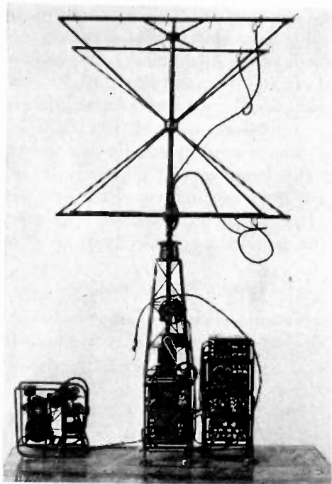
Fig. 11—Photograph of a model of the RAW or SCR-602 radar presented to Lt. Col. W. E. Phillips, president of Research Enterprises Limited.
