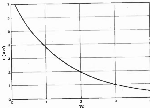
Fig. 10—Factor for obtaining the impedance parameter for helical propagation in terms of radius of the cylinder in radians (based on the axial phase velocity). The impedance parameter is given by (E_z^2/\beta^2 P)^{1/3} = (\beta/\beta_0)^{1/3} (\gamma/\beta)^{4/3} F(\gamma a) .
