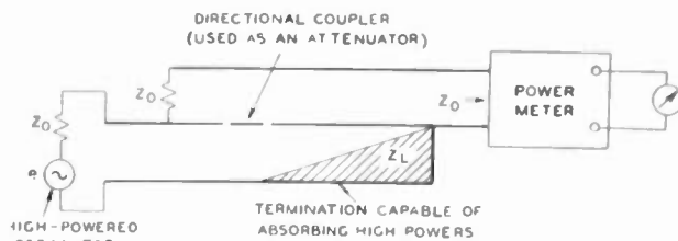
Fig. 9—Schematic diagram showing a power-measuring setup using the directional coupler as an attenuator.
