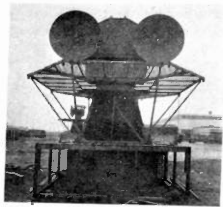
Fig. 7—The antenna and radio-frequency section of the CDX coast-defense radar set for control of coastal batteries.
