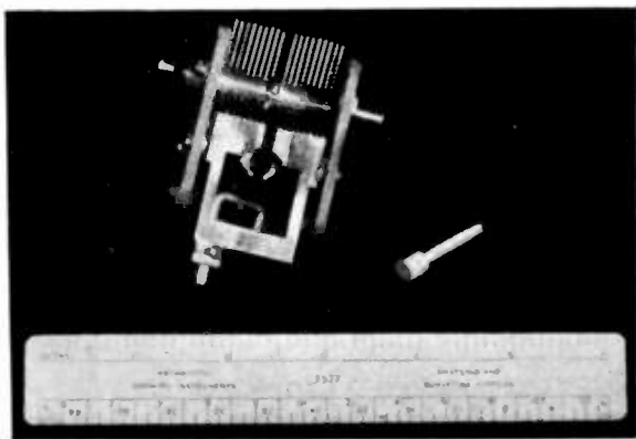
Fig. 6—Reverse view of 200- to 400-megacycle tuned-circuit assembly, with titanium-dioxide-compound coated plastic capacitance trimmer slug.
