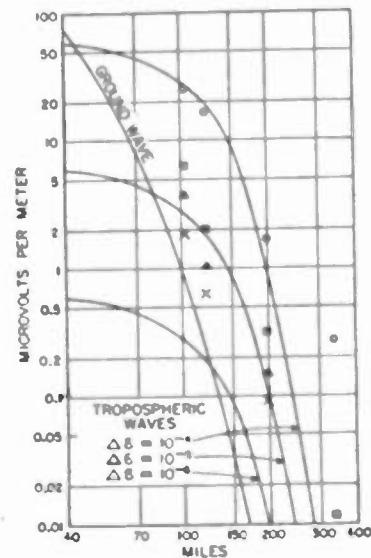
Fig. 3—Tropospheric-wave and ground-wave field intensity versus distance.
