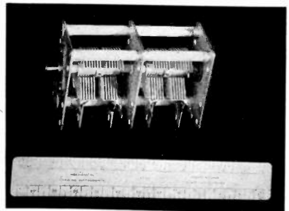
Fig. 11—Side view of experimental two-gang ultra-high-frequency tuning capacitors.
