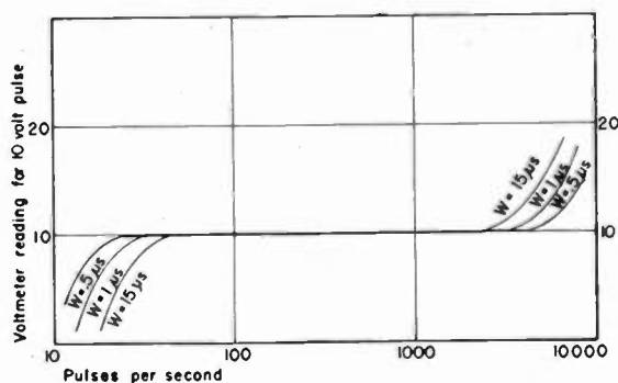
Fig. 5—Calibration curve for the circuit of Fig. 3.
