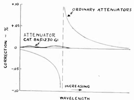
Fig. 3—Comparison of reaction on wavemeter.
