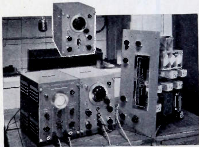
Visalgen Model 205 TS being used with 188 TS oscilloscope to align Harvey Hi-Fidelity FM Receiver.
