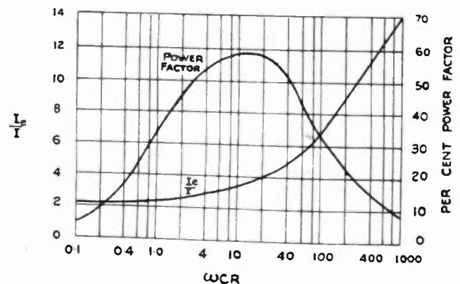
Fig. 2—The ratio of the effective input current to the average output current ( I_e/I ) and the input power factor.
