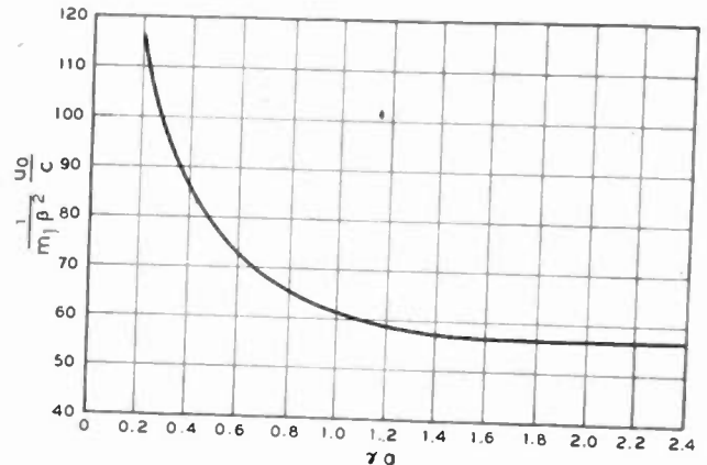
Fig. 8—Curve for use in evaluating approximately the circuit parameter Q used in connection with cutoff modes.
