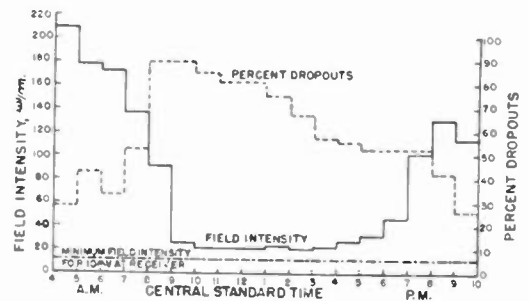
ONE OR MORE DROPOUTS RECORDED PER HOUR FOR 59% OF TOTAL HOURS. SIGNAL AT NOISE LEVEL FOR 12.2% OF TOTAL HOURS. SIGNAL BELOW MINIMUM FOR 5% OF ONE HOUR FOR 30.6% OF TOTAL HOURS.
