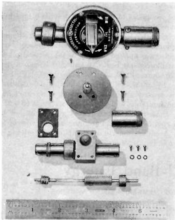
Fig. 1—Microwave attenuator.
