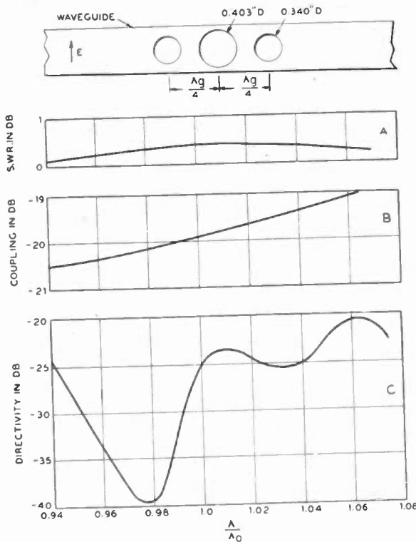
Fig. 7—Measured characteristics of a three-element directional coupler in \frac{1}{2} \times 1 -inch wave guide. \lambda_0 = 3.33 centimeters. (a) Input standing-wave ratio when primary is terminating in z_0 . (b) Coupling ( 10 \log_{10} P_{out}/P_{in} ). (c) Directivity versus wavelength.
