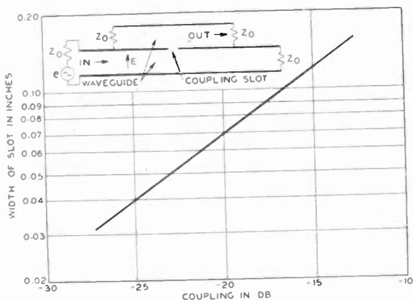
Fig. 6—Coupling ( 10 \log_{10} P_{out}/P_{in} ) versus slot width for narrow slots across the wide face of 1 \times 2 -inch rectangular wave guide. \lambda_0 = 7.4 centimeters. The wall thickness is 0.128 inch.
