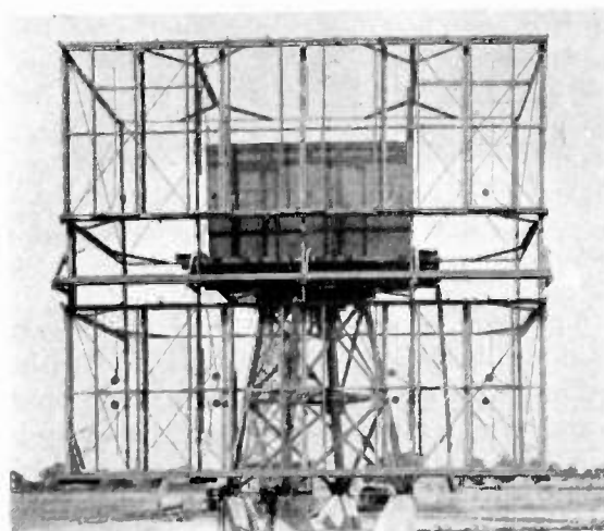
Fig. 10—Antennas of the RWG ground-control-interception radar set.
