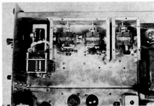
Fig. 8—Top view of experimental 200- to 400-megacycle preselector.
