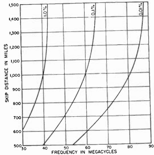
Fig. 6—Sporadic-E-layer interference: skip distance versus frequency for various percentages of the listening hours, six A.M. to midnight.
