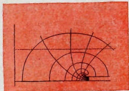
Type of equipotential and electrostatic flux lines established by probing electrolytic bath to determine shapes and disposition of electrodes. (POINT "A" IN PHOTOGRAPH)
