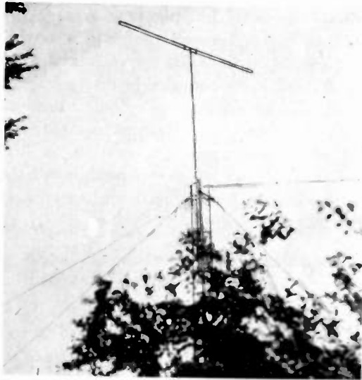
Fig. 3—Close-up view of the 45.5-megacycle half-wave folded dipole, used for monitoring.
