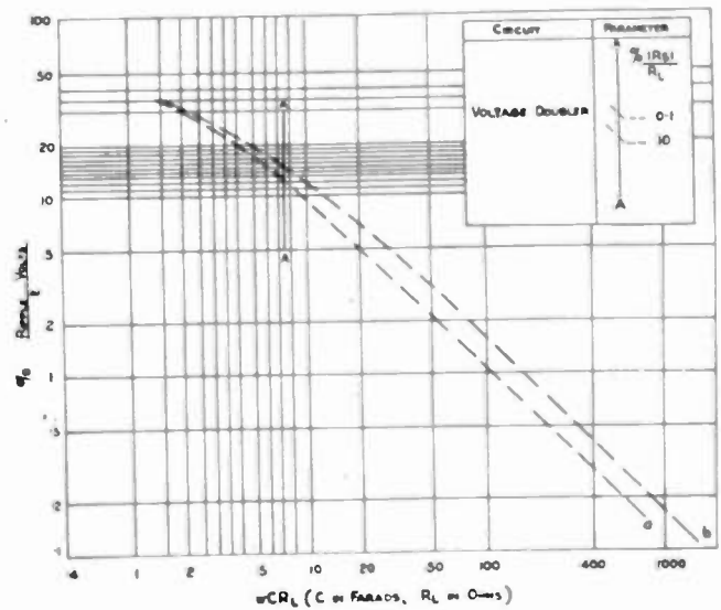
Fig. 4—Root-mean-square ripple voltage of voltage-doubling circuit.
