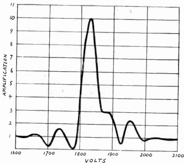
Fig. 3—Power amplification versus beam voltage.
