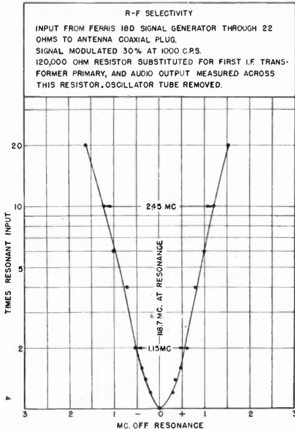
Fig. 3—Typical selectivity of three ganged preselector circuits at 118.7 megacycles.
