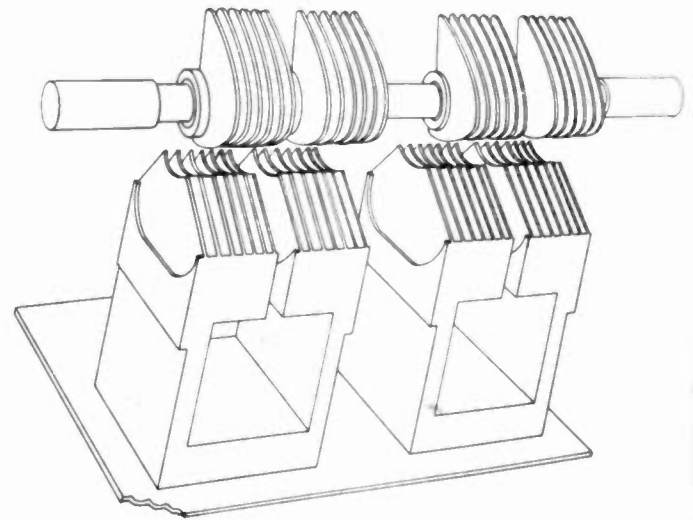
Fig. 4—Basic design of tuned-circuit elements for the 200- to 400-megacycle preselector.
