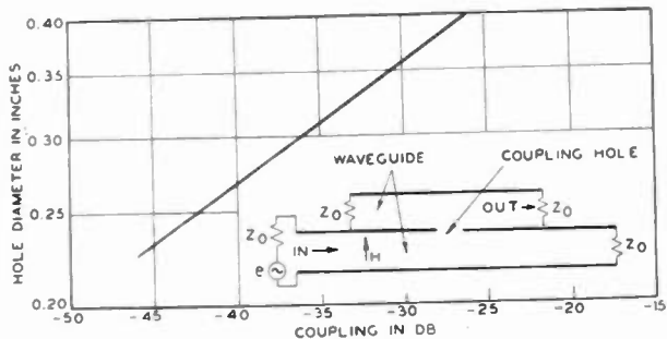
Fig. 5—Coupling ( 10 \log_{10} P_{out}/P_{in} ) versus hole diameter, for round holes in the narrow side of \frac{1}{2} \times 1 -inch rectangular wave guide. \lambda_0 = 3.33 centimeters. The wall thickness is 0.106 inch.
