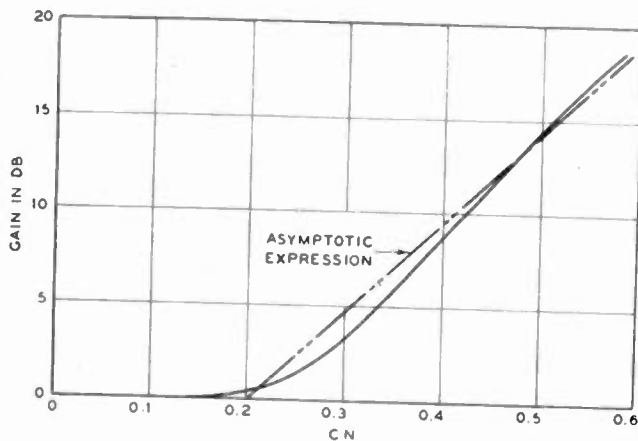
Fig. 1—Curve showing the gain of a traveling-wave tube in decibel versus the parameter C times the length of the circuit in wave lengths N . This curve is for zero circuit loss and for an electron speed equal to the wave speed in the absence of electrons.
