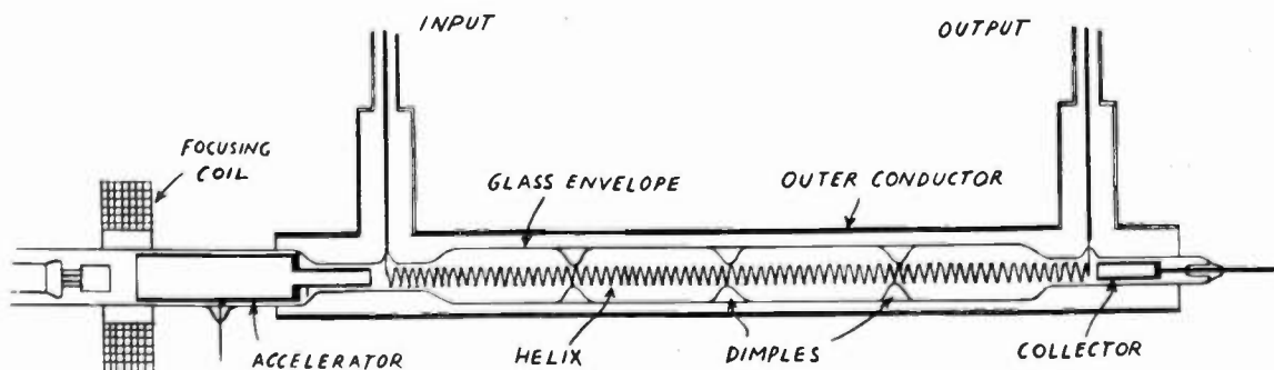
Fig. 2—Traveling-wave tube as amplifier. Helix: 66 centimeters long, No. 18 standard-wire-gauge copper wound on \frac{1}{4} -inch mandrel.
