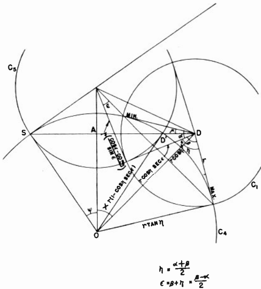
Fig. 6—Auxiliary drawing used in proof of (2) and (8).
