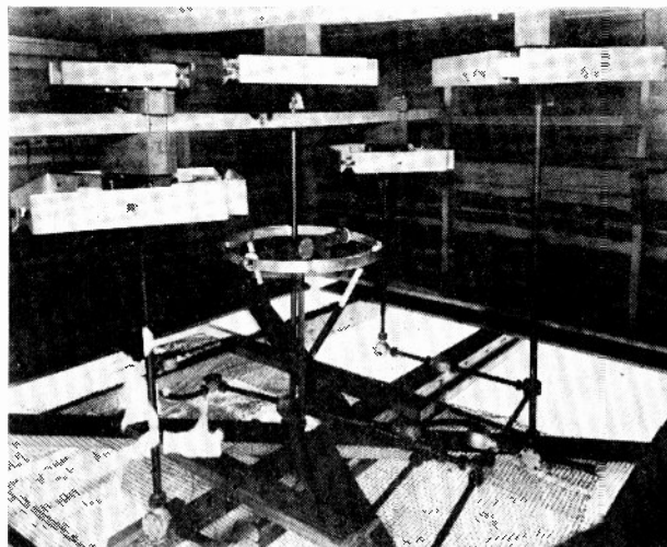
Fig. 18—Visual and aural loop antennas mounted above metal counterpoise.
