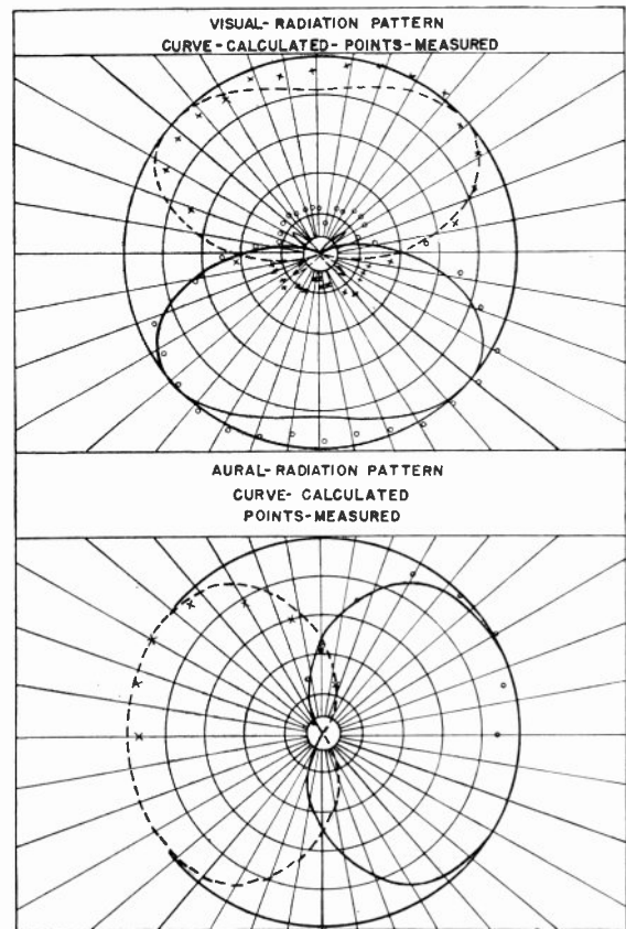
Fig. 6—Comparison of visual- and aural-radiation patterns.
