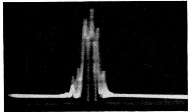
Fig. 9—Amplitude-modulation signal, 16-kilocycle, modulation 40 per cent; F=100 kilocycles; S=10 kilocycles; T=1/40 second.
