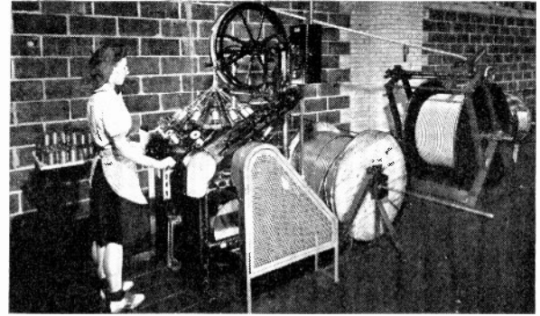
Fig. 3—Copper-wire braiding machine.
