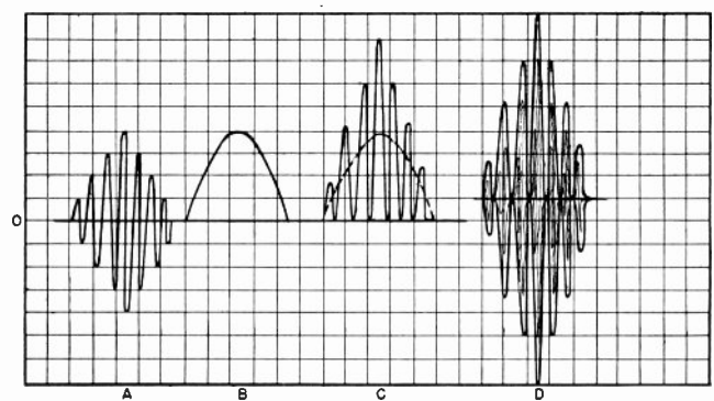
Fig. 10—Wave forms obtained in the operation of a controlled-carrier modulator.
