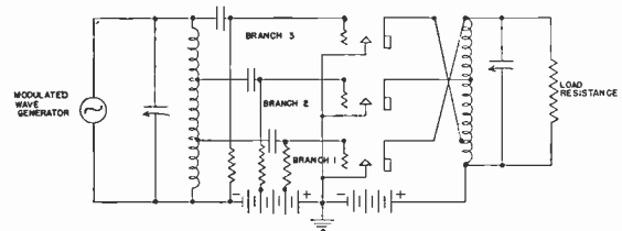
Fig. 4—Schematic circuit of a three-branch linear amplifier, with the grid drive and grid bias individually adjusted for each branch.
