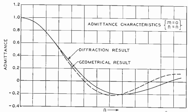
Fig. 18—Comparison of geometrical and diffraction admittance calculations. Solid curve calculated from curve of Fig. 17.
