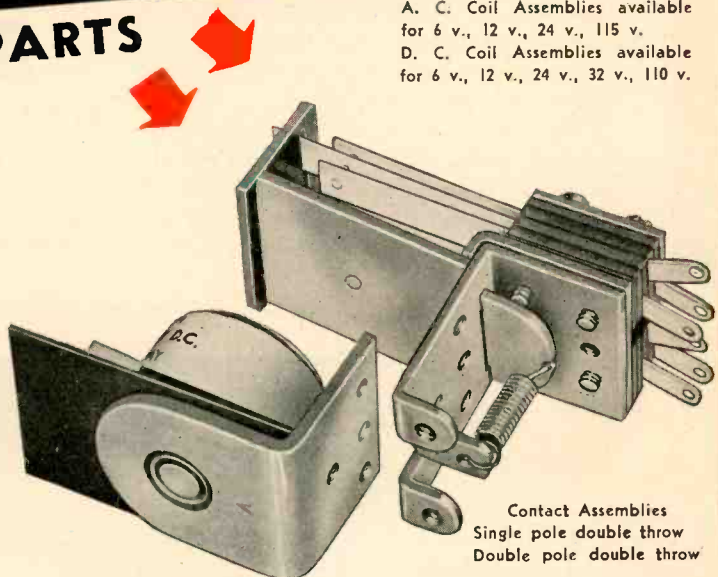
Series 200 Relay
