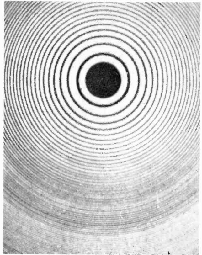
Fig. 12—Zone plate, without spurious structure.
