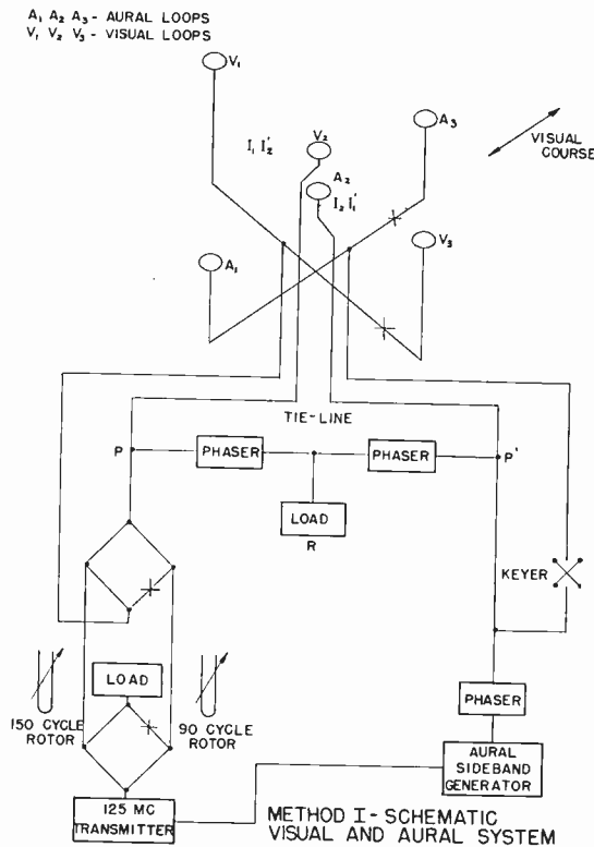
Fig. 11—Method I, schematic visual and aural system. A_1, A_2, A_3 = aural loops V_1, V_2, V_3 = visual loops
