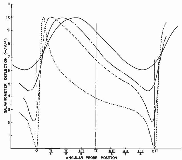
Fig. 11—Standing-wave patterns as a function of load. Curves experimental. Constant probe penetration 90 per cent.
