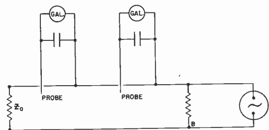
Fig. 18—Schematic diagram showing arrangement for direct measurement of probe admittance.
