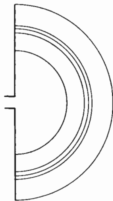
Fig. 2—Electric lines of force in principal waves.
