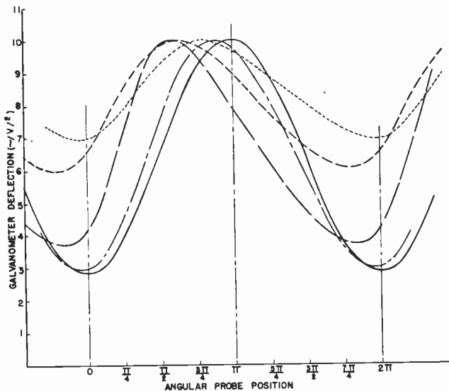
Fig. 13—Standing-wave patterns as a function of probe penetration. Curves experimental. Constant load reflection coefficient 0.31. ····· 25 per cent - · - 50 per cent - - - 75 per cent — 90 per cent - - - 97 per cent - - - 99 per cent
