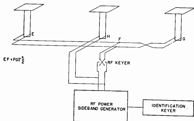
Fig. 7—Aural antenna network.
