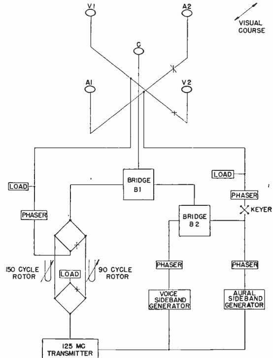
Fig. 13—Method II, schematic visual, voice, and aural system. A_1, A_2, C = aural loops V_1, V_2, C = visual loops C = voice loop
