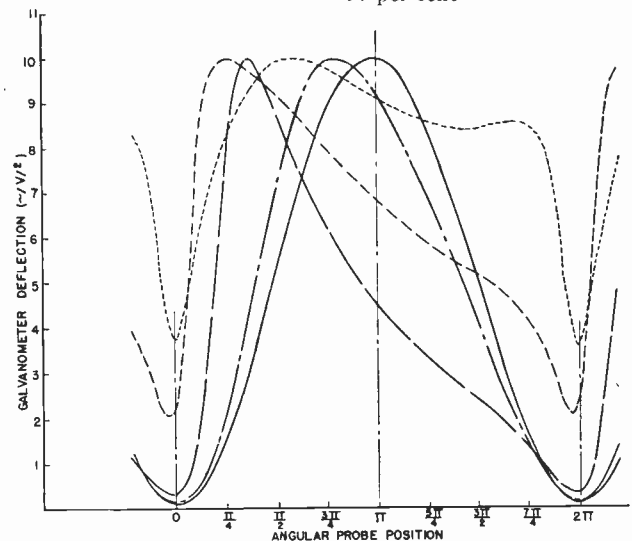
Fig. 15—Standing-wave patterns as a function of probe penetration. Curves experimental. Constant load reflection coefficient 0.82. ····· 25 per cent - · - 50 per cent - - - 75 per cent — 90 per cent - - - 97 per cent - - - 99 per cent
