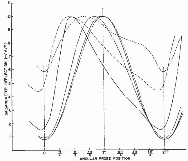
Fig. 14—Standing-wave patterns as a function of probe penetration. Curves experimental. Constant load reflection coefficient 0.56. ····· 10 per cent - · - 25 per cent - - - 50 per cent — 75 per cent - - - 90 per cent - - - 97 per cent
