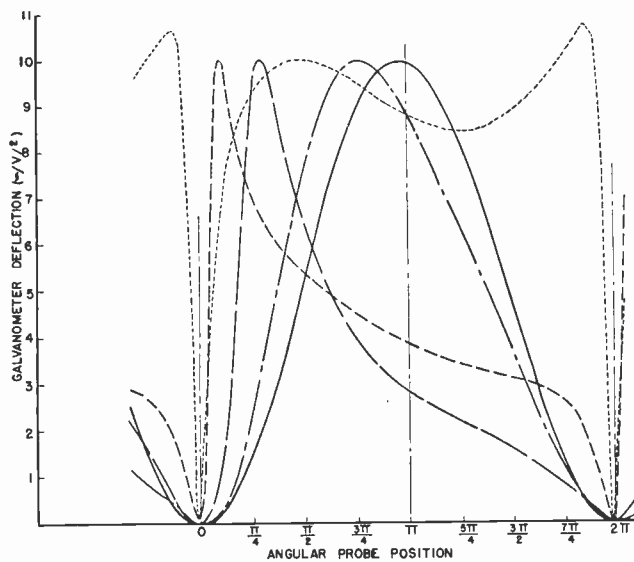
Fig. 16—Standing-wave patterns as a function of probe penetration. Curves experimental. Constant load reflection coefficient 1.00. —○—○—○—○— 25 per cent - - - - - × - - - - - × - - - - - × - - - - - × 50 per cent —□—□—□—□— 75 per cent - - - - - △ - - - - - △ - - - - - △ - - - - - △ 90 per cent ..... 97 per cent
