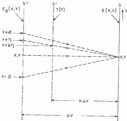
Fig. 5—Comparison of television and simulation systems.
