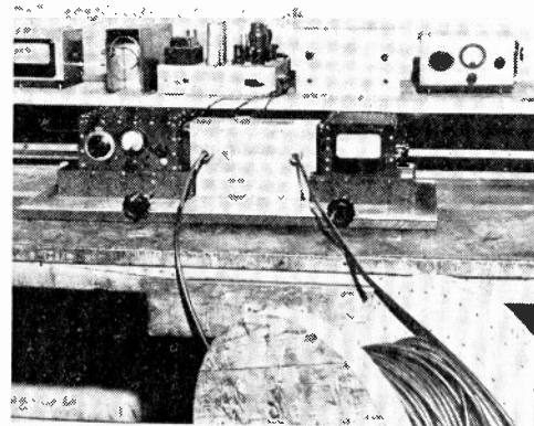
Fig. 6—Equipment for measuring the total attenuation of a transmission line.
