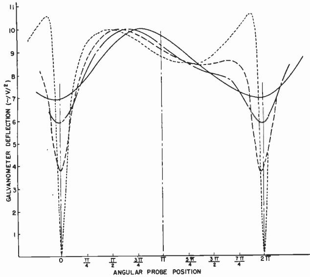
Fig. 12—Standing-wave pattern as a function of load. Curves experimental. Constant probe penetration 97 per cent. — 0.31 - - - 0.56 Reflection coefficient - · - 0.82 ····· 1.00
