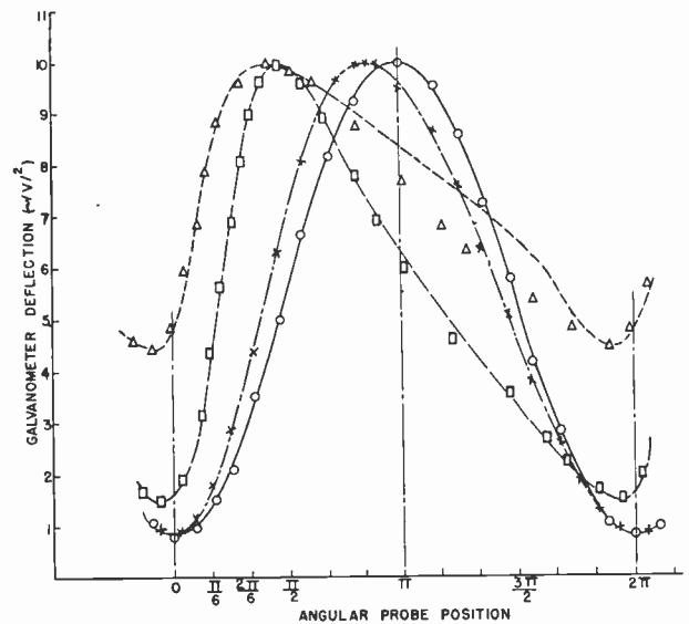
Fig. 17—Comparison of experimental and calculated patterns. Points experimental, curves calculated. Constant load reflection coefficient 0.56.
