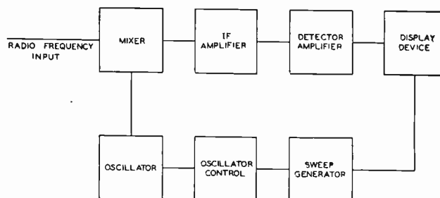
Fig. 1—Continuous-tuning spectrum analyzer.
