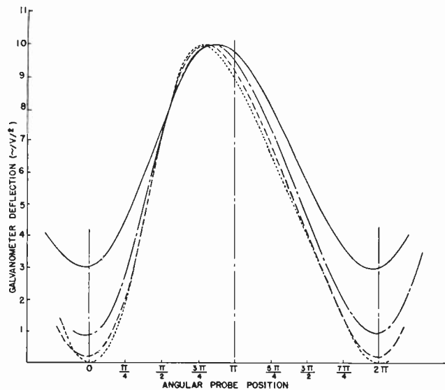
Fig. 9—Standing-wave patterns as a function of load. Curves experimental. Constant probe penetration 50 per cent.
