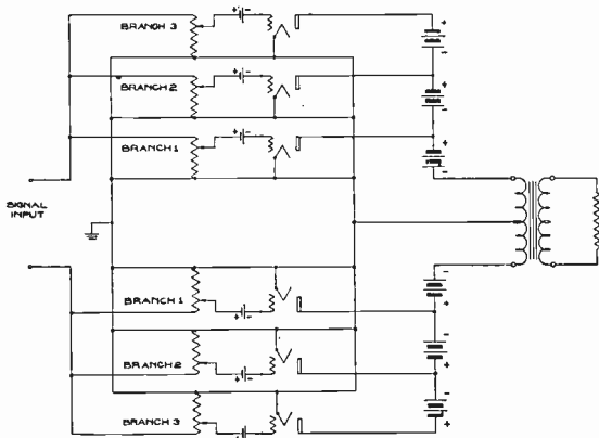
Fig. 11—Schematic circuit for switching supply voltage.
