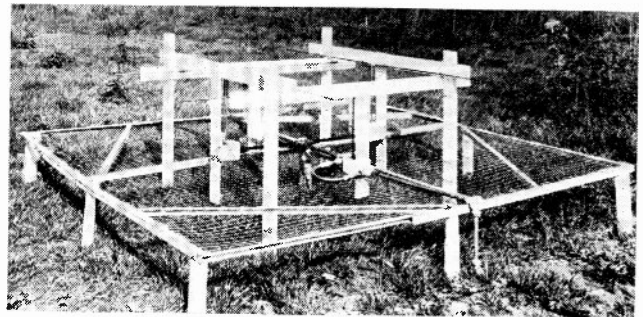
Fig. 15—125.020-megacycle marker antenna array.
