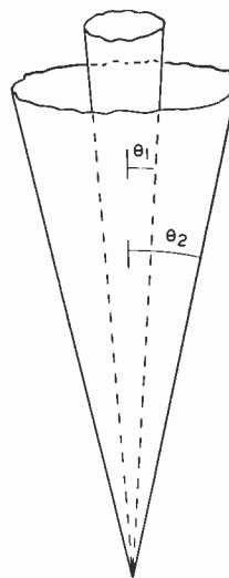
Fig. 4—Coaxial cones with a common apex.
