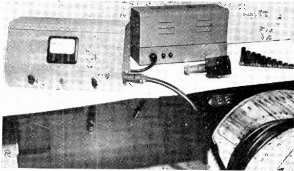
Fig. 7—Electrical-length meter.
