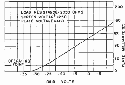
Fig. 3—Grid-voltage—plate-current characteristic of the tube of Fig. 2.
