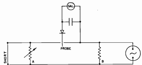
Fig. 7—Schematic arrangement showing wave detector and variable load.
