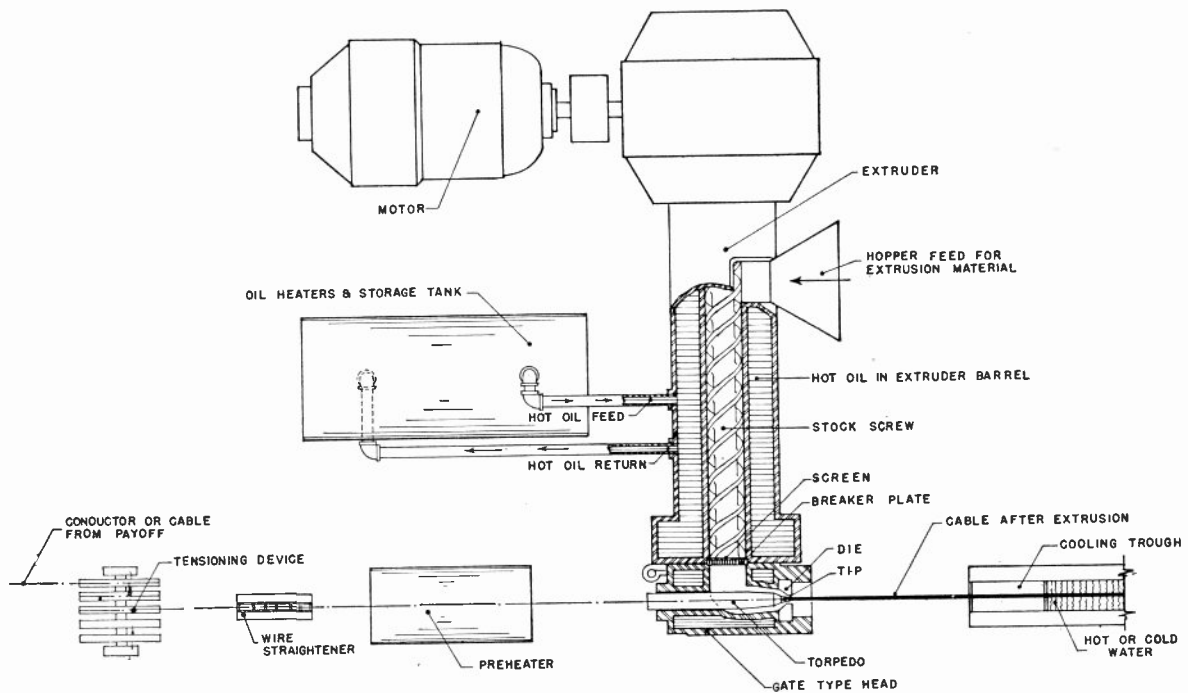
Fig. 2—Schematic cross section of extruder.
