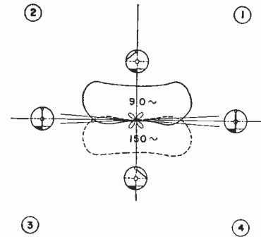
Fig. 2—Two-course localizer.
