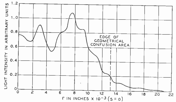
Fig. 17—Diffraction calculation. Light distribution in the out-of-focus plane t = -2 produced by an axial point source in the film plane.
