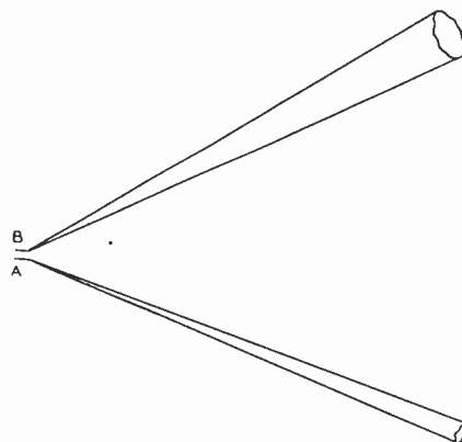
Fig. 5—Cones with a common apex.
