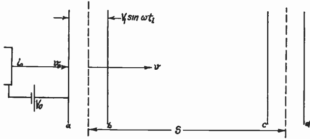
Fig. 1—Basic quantities in a klystron.
