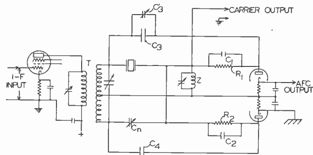
Fig. 4—Alternative carrier filter and automatic-frequency-control discriminator circuit.
