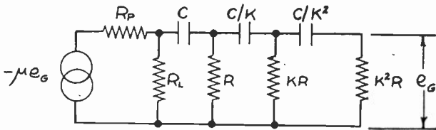
Fig. 3—Equivalent circuit of Fig. 2.
