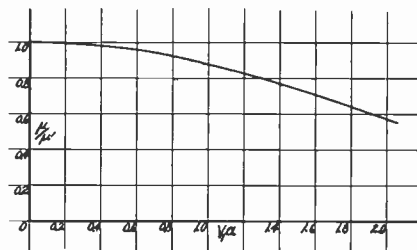
Fig. 2—Variation of klystron amplification with a change in input voltage.
