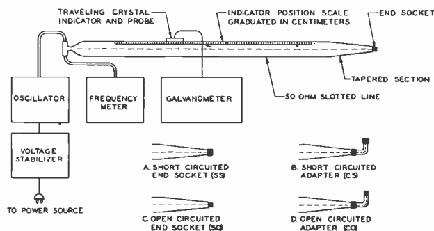
Fig. 3—Arrangement of apparatus for measurement of characteristic impedance of fittings for coaxial connectors by the slotted-line null-shift method.
