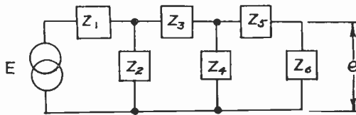
Fig. 5—General phase-shifting network.
