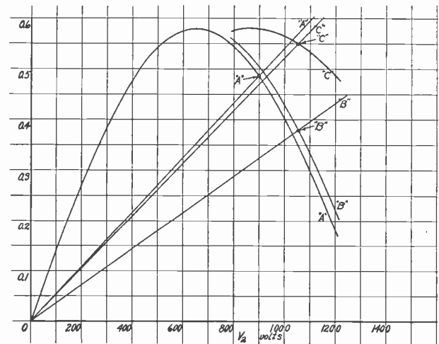
Fig. 6—Characteristic curves for an oscillator with arbitrary parameters.
