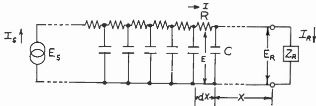
Fig. 7—Equivalent circuit for the resistance-capacitance transmission line.
