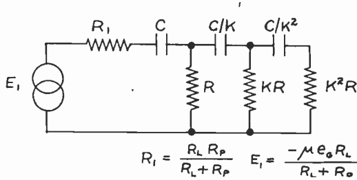
Fig. 4—Equivalent circuit of Fig. 3.
