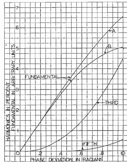
Fig. 7—Fundamental and harmonic output for phase-modulation detection. Curve A=fundamental output for exalted-carrier diode detection with or without carrier limiting, or for multigrad detection with carrier limiting. Curve B=fundamental output for multigrad detection without carrier limiting.
