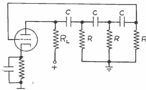
Fig. 1—Conventional phase-shift oscillator.
