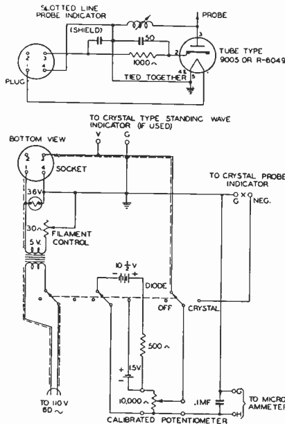
Fig. 4—Suggested circuit for precision slideback voltmeter for general slotted-line use.
