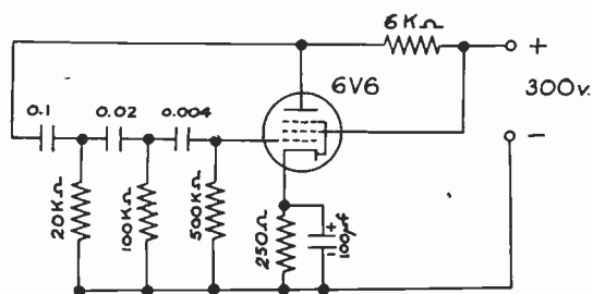
Fig. 12—40-cycle phase-shift oscillator with K = 5 .
