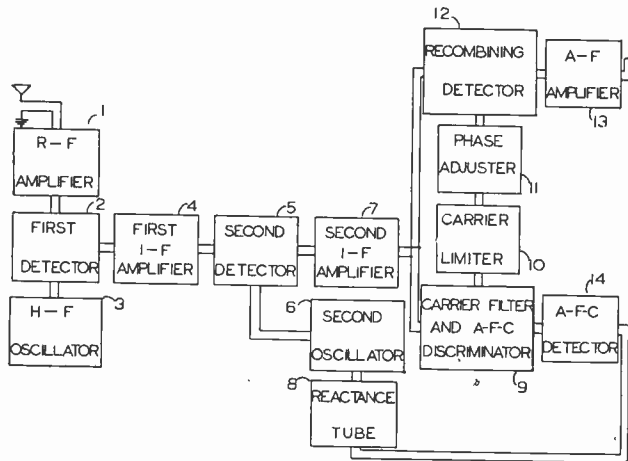
Fig. 1—Block diagram of an exalted-carrier receiving system.
