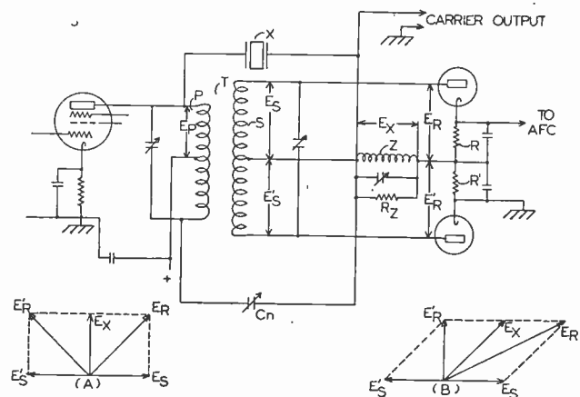
Fig. 2—Carrier filter and automatic-frequency-control discriminator circuit.
