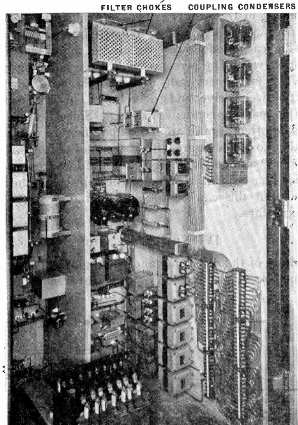
Fig. 11—Rear of exciter cubicle, 50 kilowatt transmitter.
