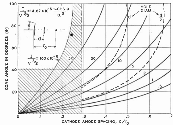
Fig. 9—Beam perveance for spherical caps.
