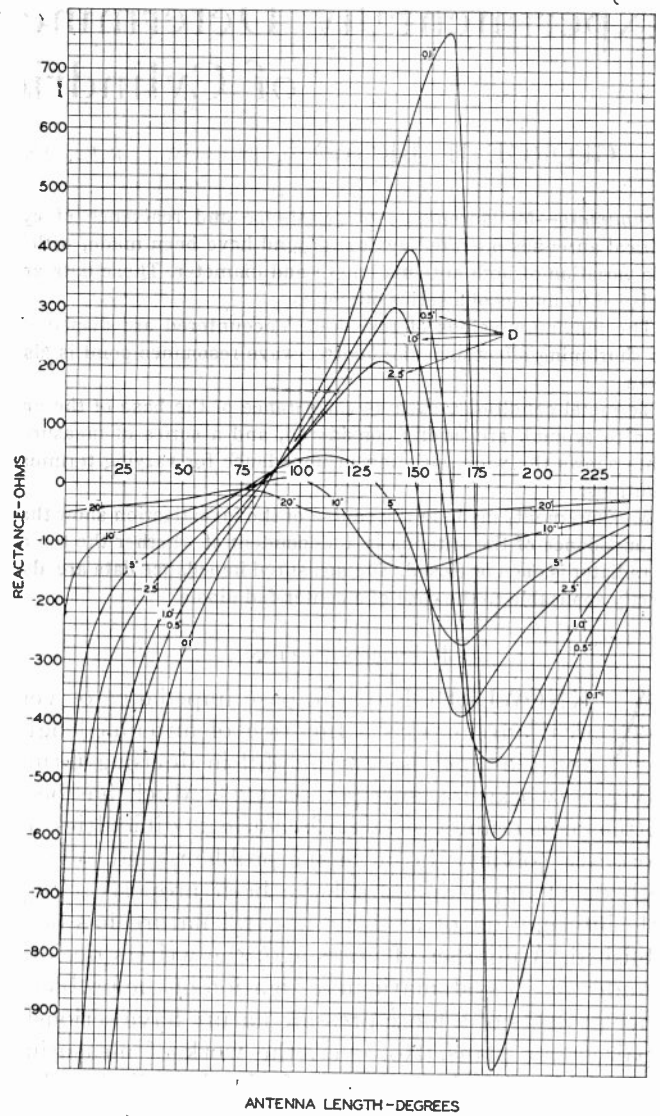
Fig. 3—Measured reactance curves versus antenna length in degrees. Again the frequency is held constant and the physical length of the antenna is changed.
