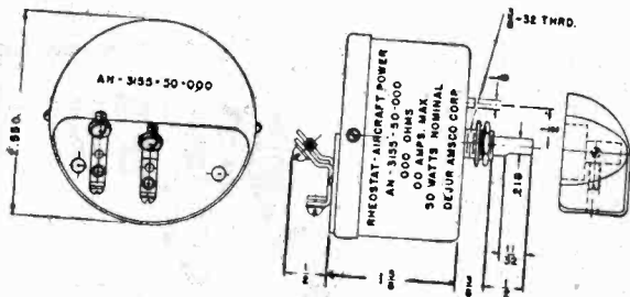
MODEL 231—50 WATTS, Ranges from \frac{1}{4} to 10,000 OHMS
