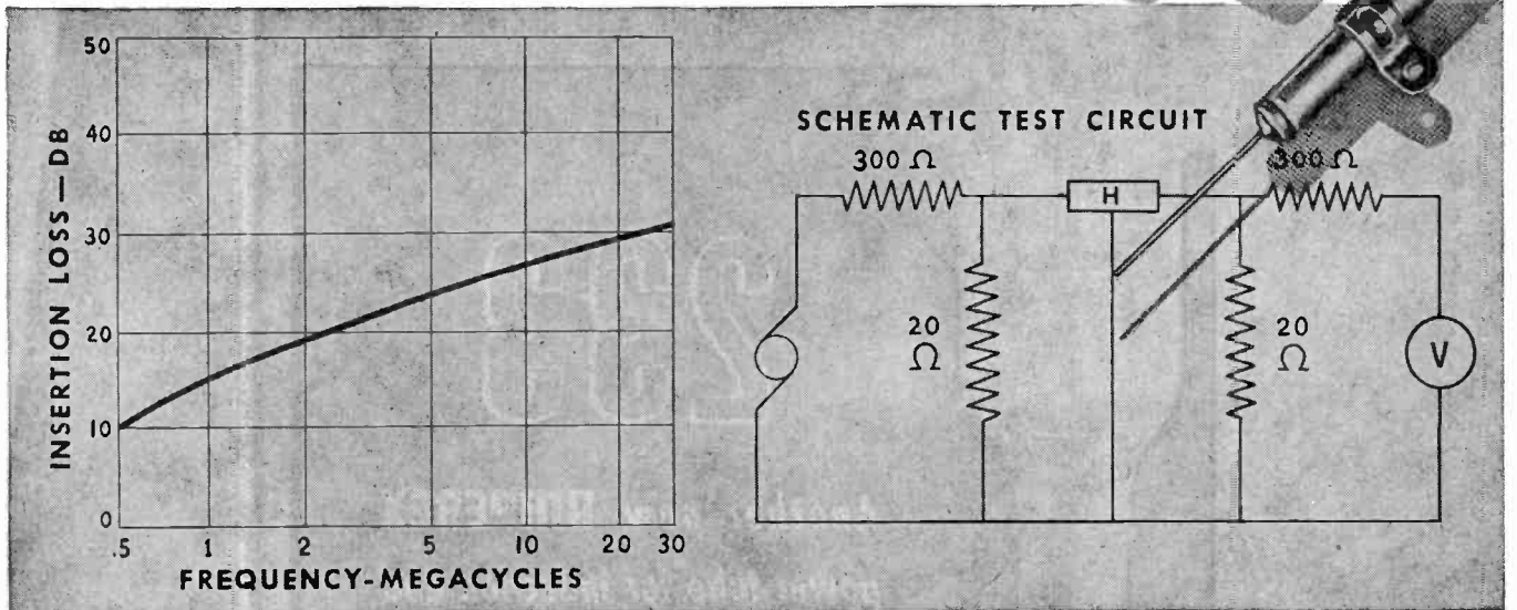
Curve showing insertion loss of a Sprague HYPASS Capacitor.
