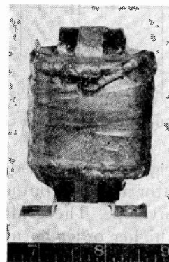
Fig. 16—Pulse transformer.
