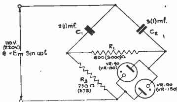
Fig. 6—Circuit of the resistance-capacitance bridge regulator.
