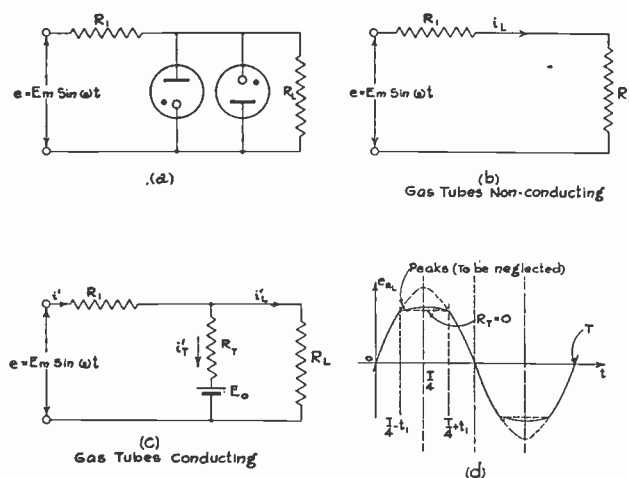
Fig. 2—Equivalent circuits of conventional-type regulator and resultant wave form.
