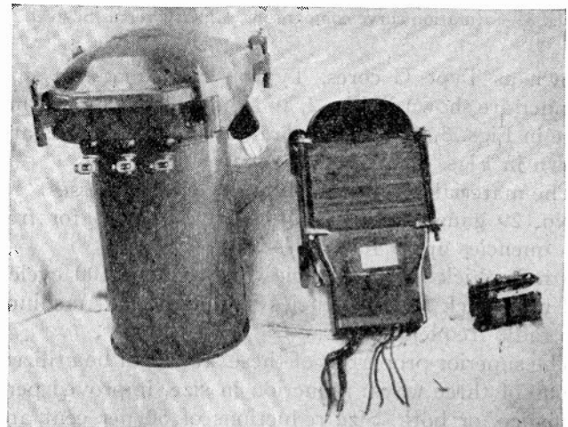
Fig. 9—Comparison picture of oil and dry distribution transformers with dry aircraft transformer.
