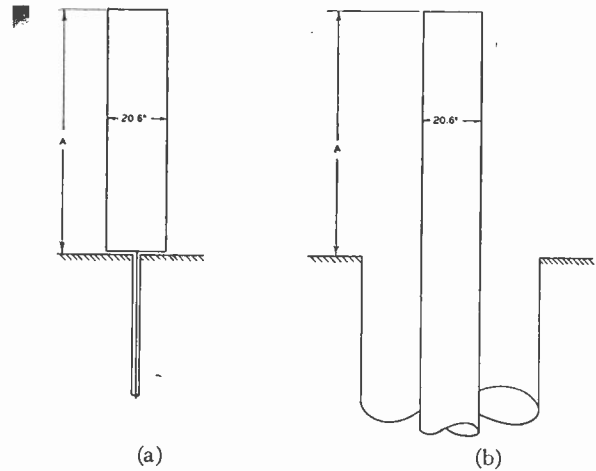
Fig. 12—Experimental arrangement for obtaining curves in Figs. 13 and 14. (a) For curve A . (b) For curves B , C , and D .
