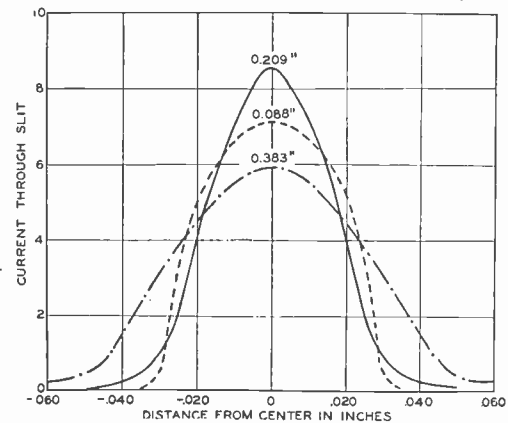
Fig. 17—Probe data at different distances from gun.
