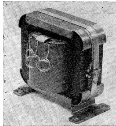
Fig. 8—Radio-transformer coil and core assembly.
