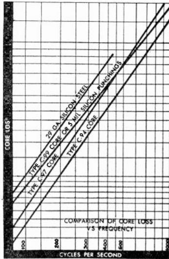
Fig. 6—Comparison of core loss versus frequency.
