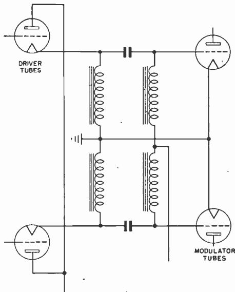
Fig. 10—Cathode-follower circuit.
