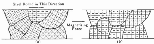
Fig. 1—Grain orientation.
