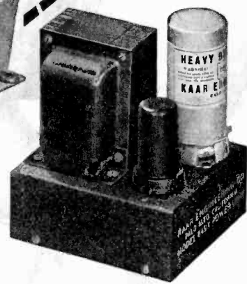
TYPE 649—Provides 240 volts at 50 ma. Available at other standard ratings, and for operation from 6 or 12 volt batteries. Type 647, not illustrated, provides 240 volts at 75 ma.
