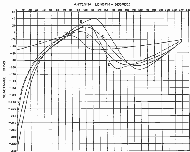
Fig. 14—Reactance curves corresponding to the resistance curves of Fig. 13.
