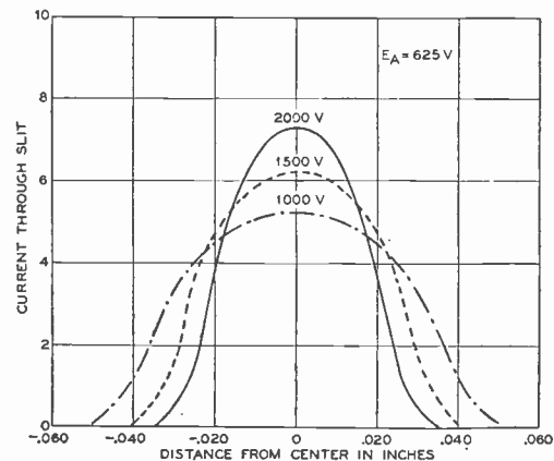
Fig. 18—Effects of accelerating field on beam diameter.
