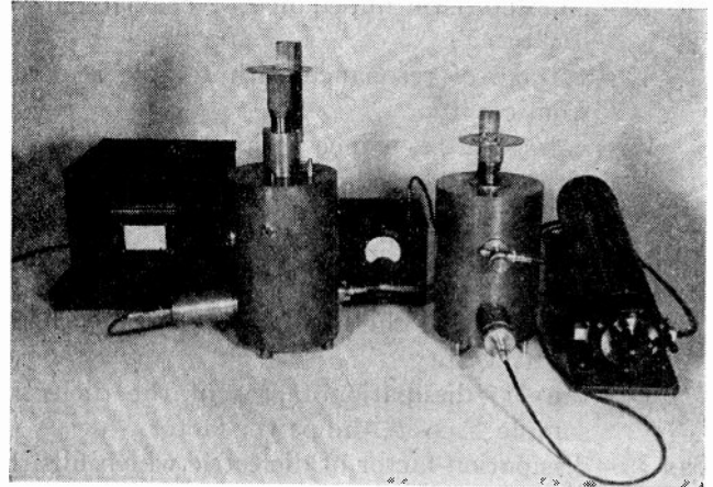
Fig. 3—Measuring apparatus for use at 200 megacycles. Left to right: galvanometer, measuring cavity, microammeter, cavity wave-meter, oscillator.
