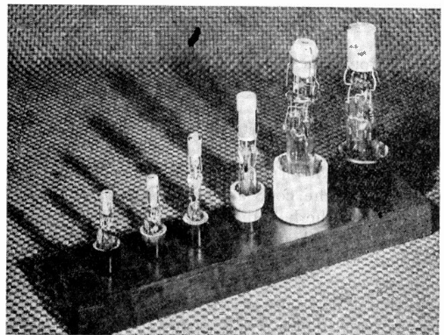
Fig. 14—A series of point-focused guns.
