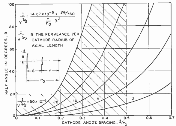
Fig. 10—Beam perveance for cylindrical segments.
