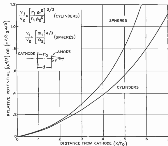
Fig. 8—Potential distribution between coaxial cylinders and concentric spheres with complete space charge. (Authors note. The second expression in the ordinate should read (r^2/3\beta^4/3/r_0^2/3) .)
