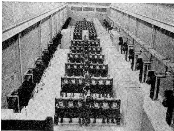
Fig. 9—A large power-rectifier installation, output 60,000 amperes, 600 volts.
