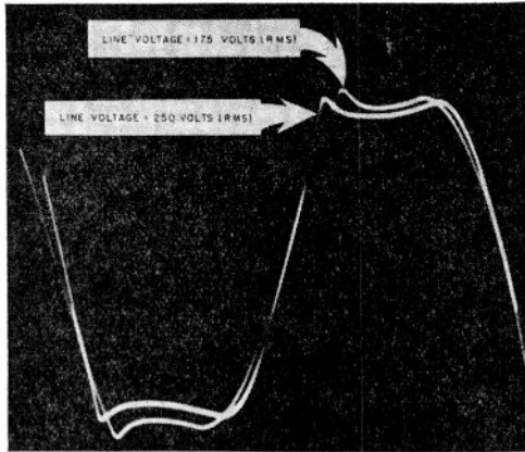
Fig. 5—Wave form of output current of bridge-circuit regulator.
