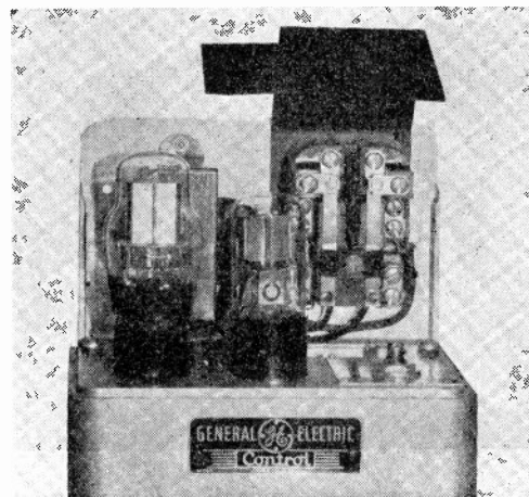
Fig. 8—The chassis of a simple photoelectric relay.
