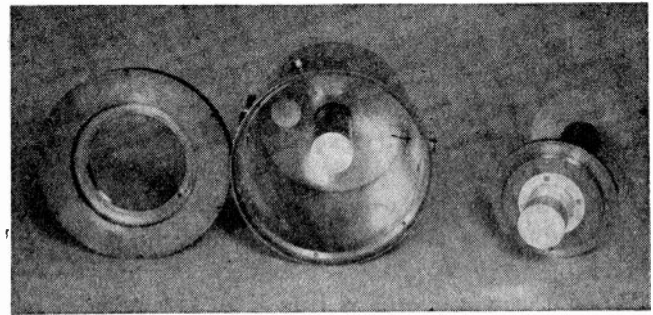
Fig. 5—Interior view of the measuring cavity for use at 200 megacycles. This cavity is 10 inches long and 6 inches in diameter.
