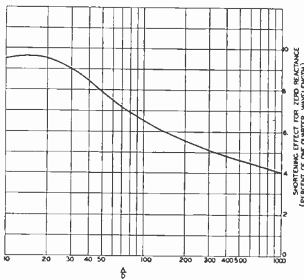
Fig. 11—Shortening effect near the quarter-wave point.
