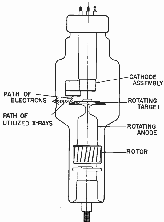
Fig. 1—Rotating anode X-ray tube for radiography requiring high X-ray output.
