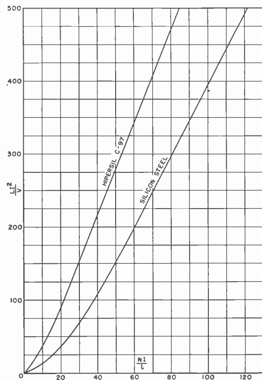
Fig. 5—Choke sizes in HiperSil and Si steel.
