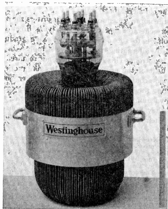
Fig. 6—WL-895-R modern 100-kilowatt maximum rating tube for radio and industrial applications.
