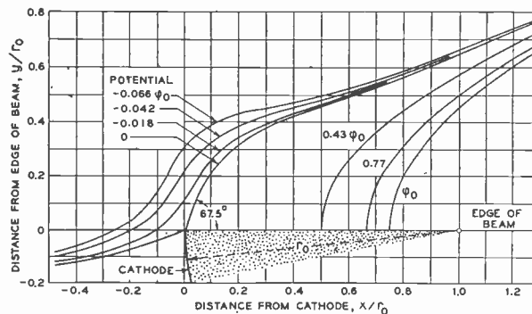
Fig. 5—Equipotential surfaces for radial rectilinear electron flow between segments of cylinders.
