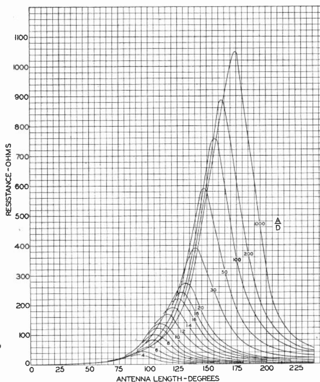
Fig. 6—Antenna resistance versus antenna length A , when a constant ratio of length to diameter A/D is maintained. Here the length and diameter are held constant while the frequency is changed.
