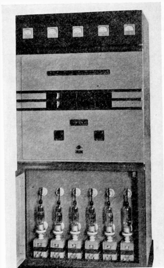
Fig. 4—Front view of modulator.
