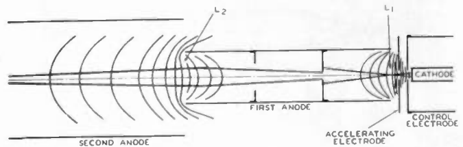
Fig. 1—Schematic representation of a conventional electron gun.
