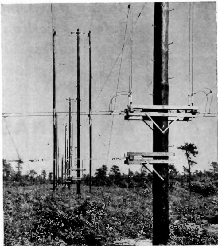
(Above) 13 DIRECTIONAL ANTENNAS are provided at the new stations, and several of them are of the four-section type shown here. Isolantite* strain insulators are extensively used in the construction of these antennas. These insulators find wide application in the radio and communications fields, because of their high mechanical strength and electrical efficiency.
