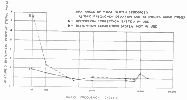
Fig. 9—Distortion characteristics—Maximum angle of phase shift = 32 degrees.
