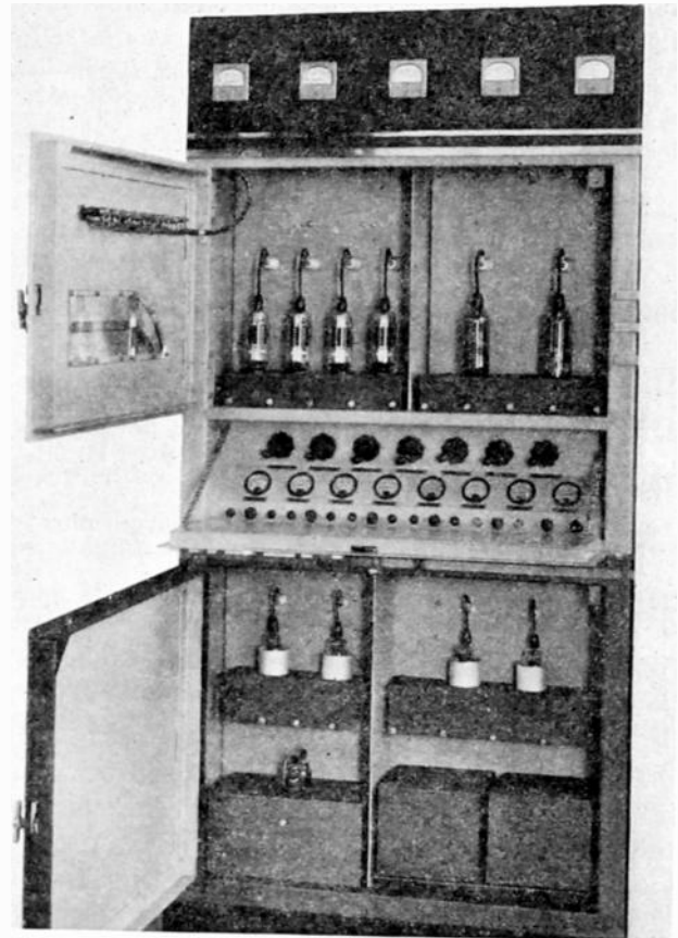
Fig. 2—Front view of exciter.
