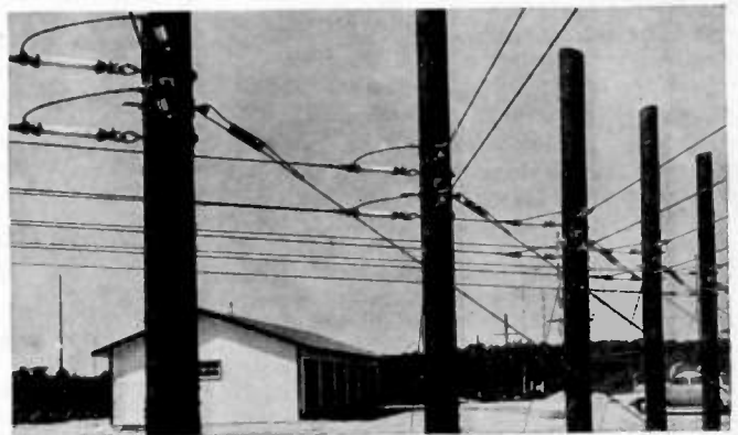
(Below) SPECIAL FITTINGS used on Isolantite strain and other types of Isolantite insulators at the new stations were designed and tested by engineers of Mackay Radio and Telegraph Company and the Columbia Broadcasting System. These fittings were manufactured by Burndy Engineering Company.
