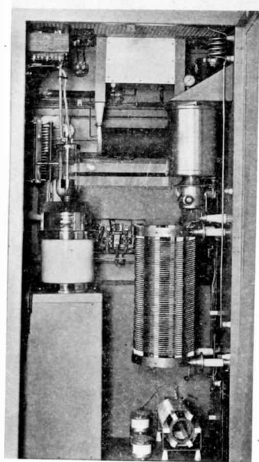
Fig. 9—Rear of power amplifier.
