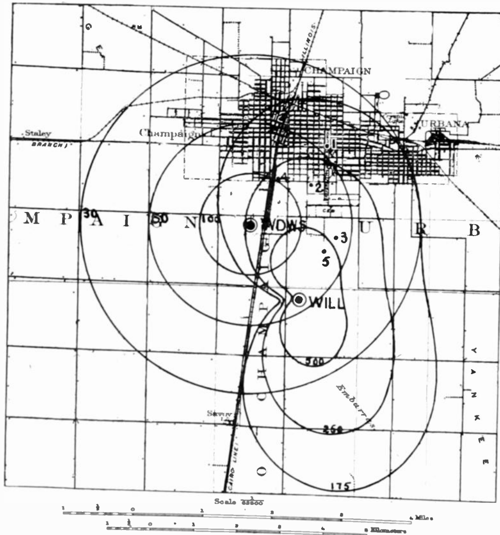
Fig. 1—WILL contours measured. WDWS contours calculated from measured efficiency. Figures on contours are field strength in microvolts per meter.
