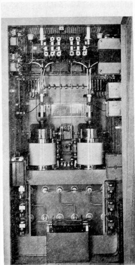
Fig. 10—Rear of modulator.
