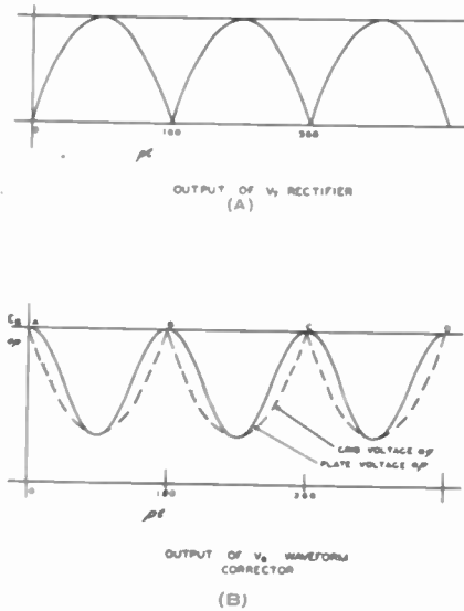
Fig. 7—Input and output voltages of carrier modulator.
