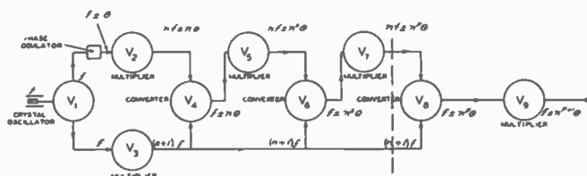
Fig. 2—Stabilized frequency-modulation system using several converters.
