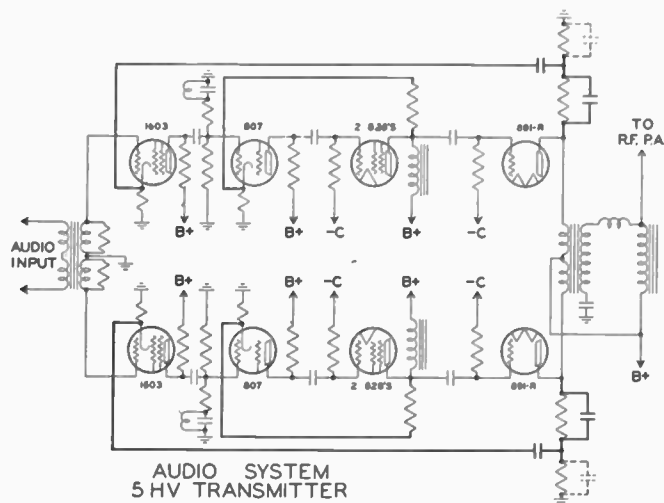
Fig. 6—Fundamental schematic of audio circuits.
