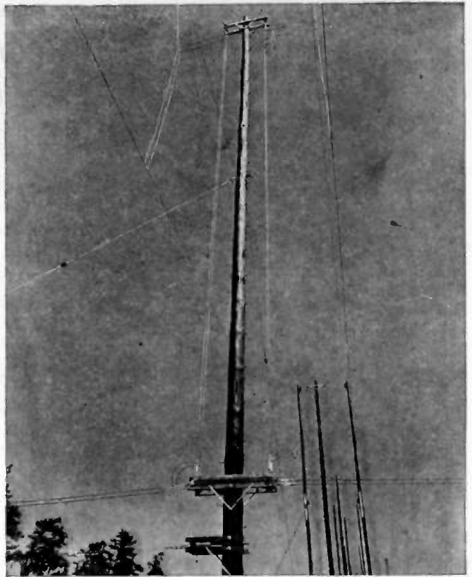
(Above) CONSTRUCTION DETAILS of the antennas are shown here. Horizontal wires at left near base of pole provide means for tuning the antennas through the medium of variable line shunts.
