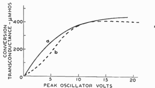
Fig. 14—Conversion transconductance of a typical mixer designed for outer-grid injection of oscillator. Signal-grid bias, E_{c1} = -3 volts. Curve a corresponds to fixed No. 3 grid bias, E_{c3} = -8 volts. Curve b corresponds to bias obtained through a 50,000-ohm grid leak.
