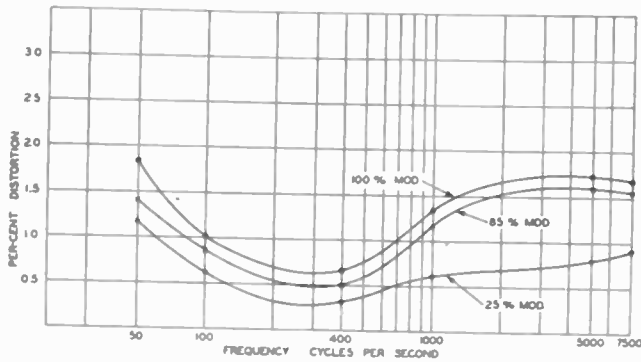
Fig. 7—Distortion curves.
