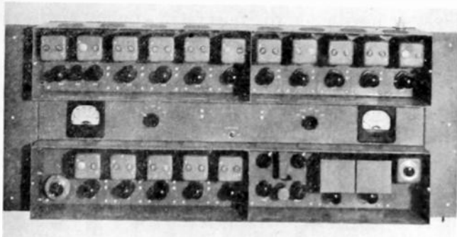
Fig. 3—Experimental unit.
