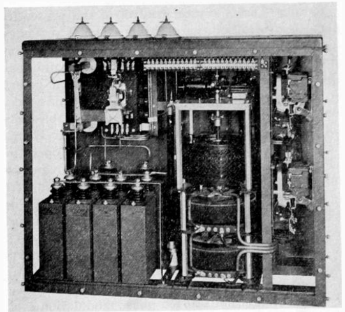
Fig. 11—Power and filter frame.
