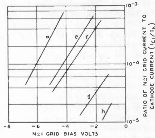
Fig. 21—Signal-grid (grid No. 1) current of the outer-grid injection mixers shown in Fig. 20. Curve a corresponds to the original design (a) of Fig. 18 and is shown for comparison. Data taken with a 20-megacycle oscillator voltage of 12 volts peak amplitude applied to the oscillator-grid. E_{c3} = -10 volts, E_{c2 \text{ and } 4} = 100 volts, E_b = 250 volts.
