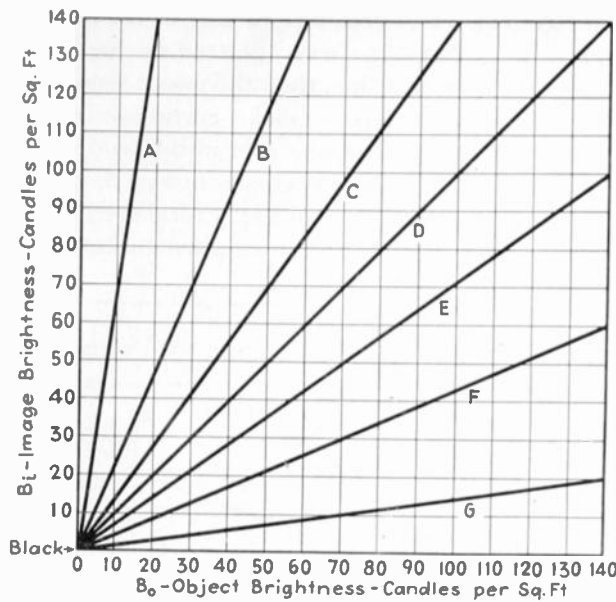
Fig. 4—Distortionless characteristics illustrating the effect of changing the over-all gain of the system.
