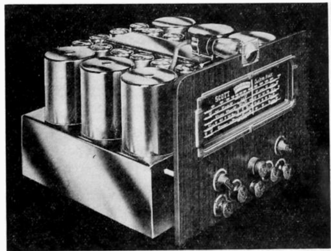
Fig. 1—Tuning chassis of Scott Phantom Deluxe (standard) receiver.
