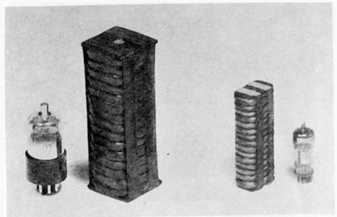
Fig. 14—Typical assemblies of the wrapped-cell type of B-battery construction.
