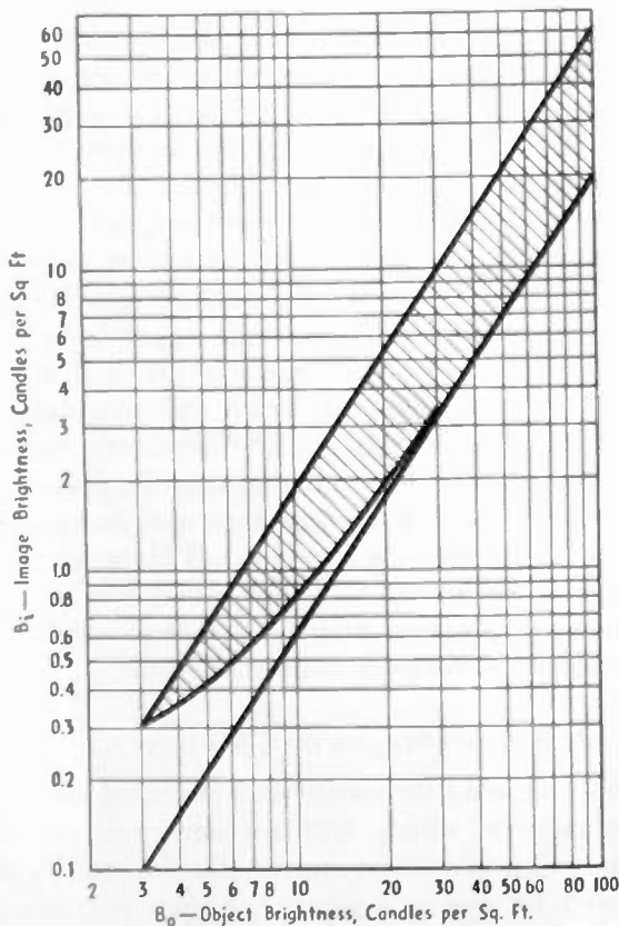
Fig. 14—Compensation of ambient illumination.
