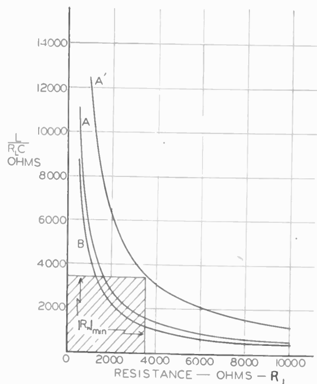
Fig. 10—Method of determining continuity of oscillations in the resistance-tuned oscillator of Fig. 4. Curve A' : C=0.00510 microfarad, L=0.064 henry Curve A : C=0.00510 microfarad, L=0.0285 henry Curve B : C=0.00650 microfarad, L=0.0285 henry
