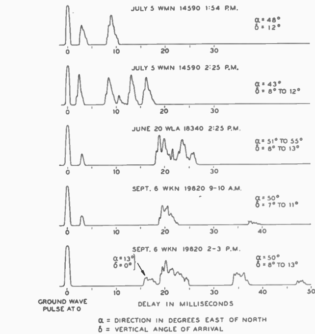
Fig. 6—Echoes observed on 16 and 20 meters in the second series of tests.
