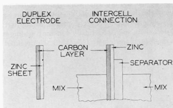
Fig. 6—Elements of flat-cell type of B battery.
