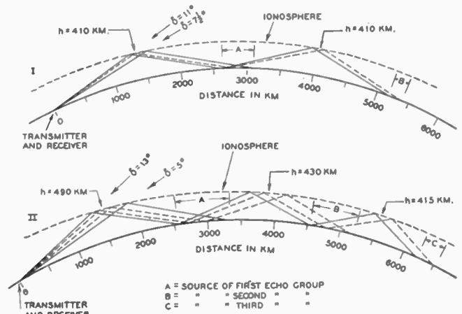
Fig. 8—Paths of multiple echoes on September 6, 1939.
