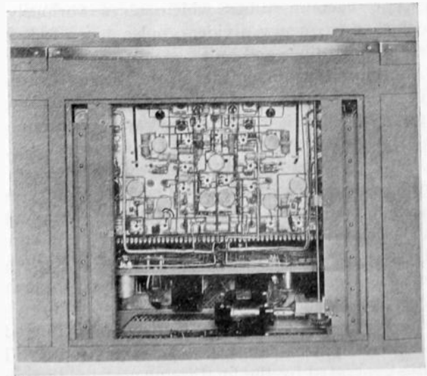
Fig. 6—Rear view of console showing elevator arrangement.
