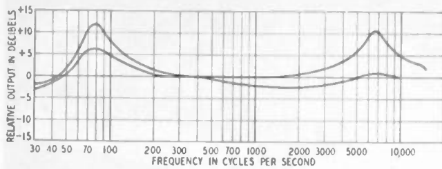
Fig. 8—Electrical fidelity data. Audio amplifier of 20-tube receiver.
