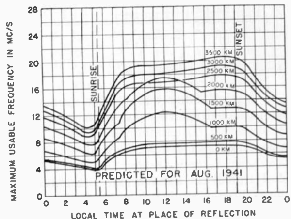
Fig. 2—Predicted maximum usable frequencies for dependable radio transmission via the regular layers, average for undisturbed days, for August, 1941. The values shown will be considerably exceeded during irregular periods by reflections from clouds of sporadic E layer. For information on use in practical radio transmission problems, see Letter Circulars on radio transmission obtainable from the National Bureau of Standards, Washington, D. C., on request.
