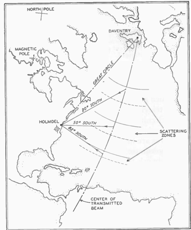
Fig. 10—Routes of southerly deviated waves caused by scattering.
