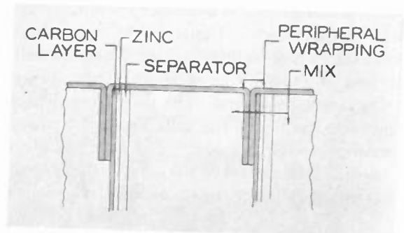
Fig. 10—Cell wrappings in new type of B-battery construction.
