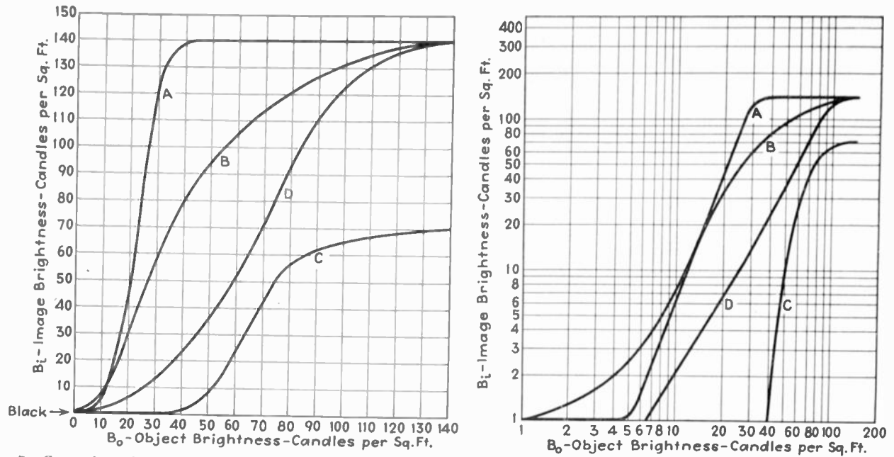
Fig. 7—General nonlinear saturation curves, showing brightness and contrast distortions typical of practical television systems.
