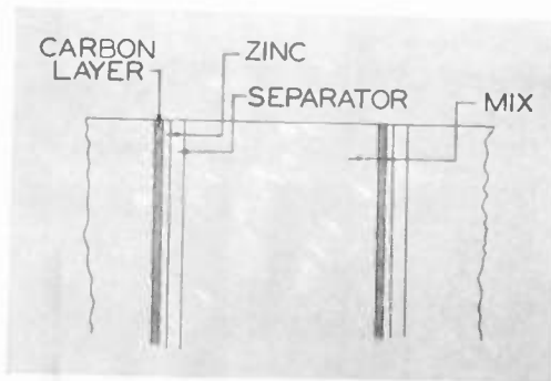
Fig. 9—Elements of flat-cell type of B battery.
