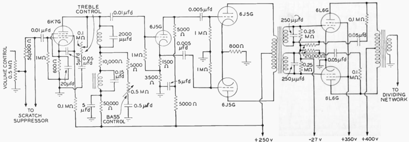
Fig. 7—Audio amplifier circuit.
