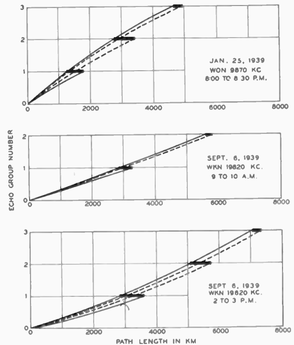
Fig. 9—Relation between path length and echo group number for multiple echoes.
