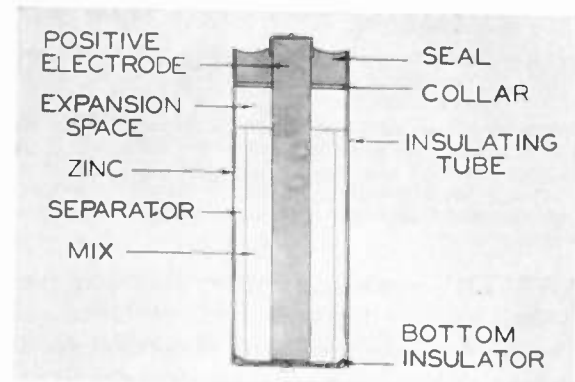
Fig. 4—Structure of cylindrical-type B-battery cell.
