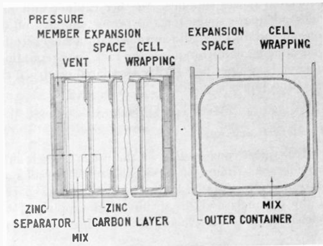
Fig. 13—Structure of wrapped-cell type of B battery.
