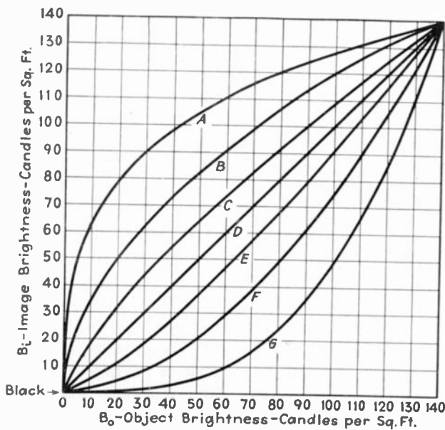
Fig. 5—Power functions displaying brightness distortion, but free of any corresponding contrast distortion.
