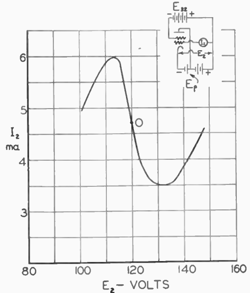
Fig. 5—Current-voltage characteristic of transistron oscillator showing quiescent point O . Type '57 Tube
