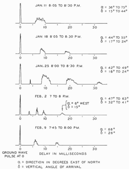
Fig. 4—Echoes observed in the first series of tests. WON, 9870 kilocycles.
