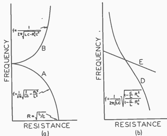
Fig. 3—Frequency of resistance-tuned oscillator. Curve A : R_c = 0 , R_L varied from 0 to \sqrt{L/C} . Curve B : R_L = 0 , R_c varied from 0 to \sqrt{L/C} . Curve D : R_L + R_c = k < \sqrt{L/C} , R_L varied from 0 to k . Curve E : R_L + R_c = k/2 , R_L varied from 0 to k/2 .
