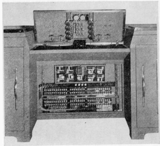
Fig. 5—Terminal wiring, relay panel, and control details of console.
