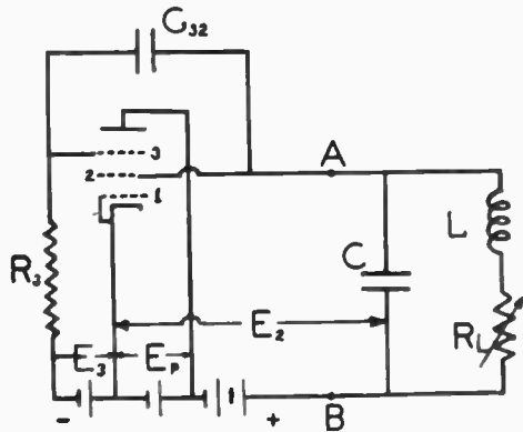
Fig. 4—Transistron oscillator. Type '57 Tube
