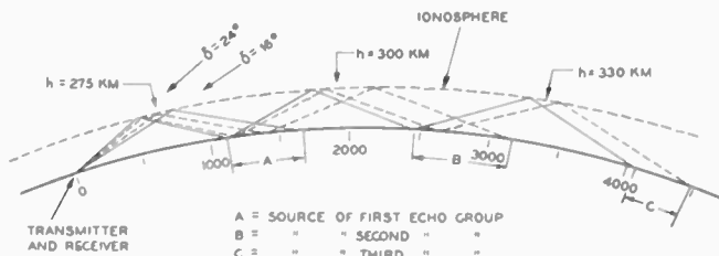
Fig. 7—Paths of multiple echoes on January 25, 1939.
