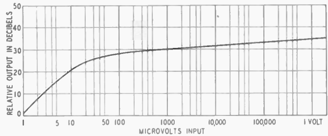
Fig. 12—Automatic-volume-control characteristics of 20-tube receiver measured at 1000 kilocycles with 30 per cent modulation.
