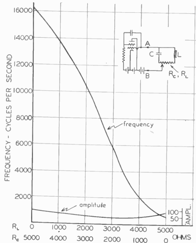
Fig. 14—Extended-range tuning varying both R_L and R_c simultaneously.
