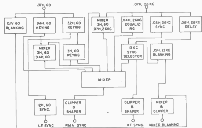
Fig. 9—Functional diagram of synchronizing and blanking-pulse generator.
