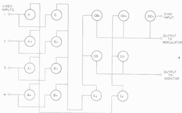
Fig. 10—Functional diagram of mixing and line amplifier.
