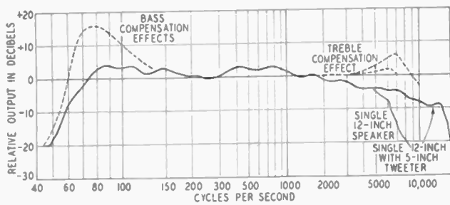
Fig. 5—Sound-pressure data and the effect of audio compensation in the receiver. Measurements were made in an open-back cabinet. This curve is not shown to present the limits of fidelity of a Scott receiver, but rather to present the fidelity for a given set of conditions. They are of the mean-energy type.
