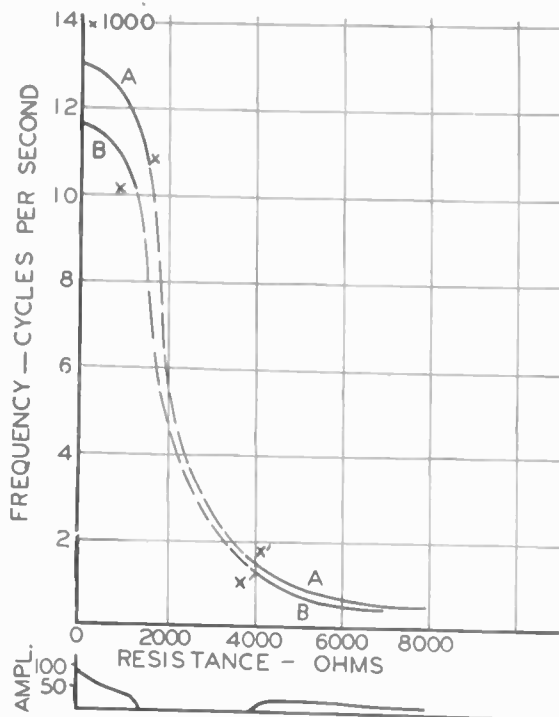
Fig. 9—Extinction of oscillations with too low L/C ratio. Curve A: C=0.00510 microfarad, L=0.0285 henry Curve B: C=0.00650 microfarad, L=0.0285 henry Lower curve: Amplitude of oscillations for curve A For all curves E_2 = 120 volts, E_3 = -10.4 volts, E_p = 11.0 volts |R_n|_{min} = 3500 ohms when R = 0
