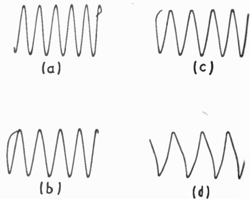
Fig. 7—Wave forms of resistance-tuned oscillator. (Using circuit of Fig. 4.) (Cathode-ray oscillograms, retouched.) (a) R = 0 frequency = 8760 cycles per second (b) R = 1000 " = 8300 " " " (c) R = 3000 " = 3800 " " " (d) R = 5000 " = 590 " " "
