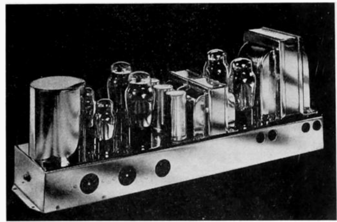
Fig. 6—Power amplifier for new custom-built Scott Phantom Deluxe receiver.
