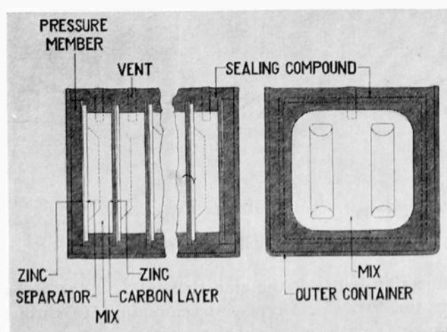
Fig. 7—Structure of flat-cell type of B battery.
