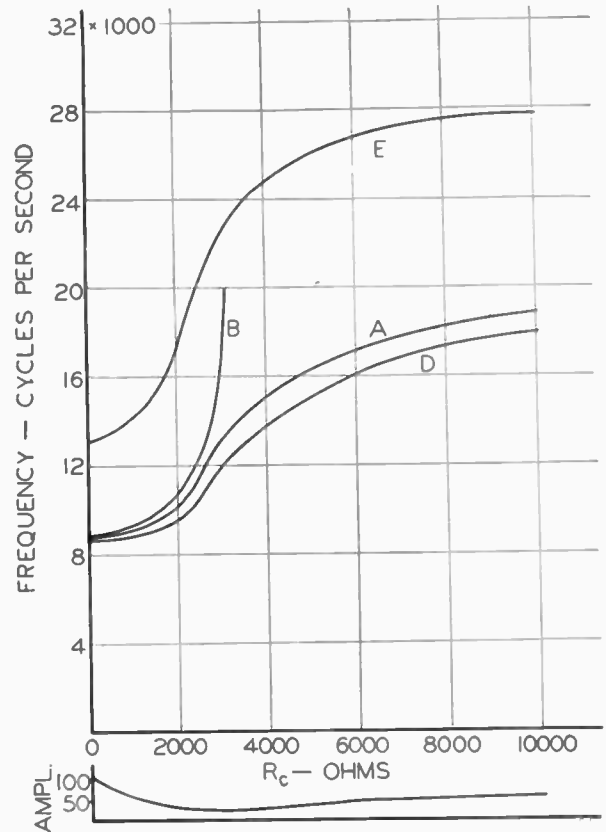
Fig. 12—Variation of frequency with R_c . Curve A: C=0.0051 microfarad, L=0.064 henry, C_{32}=0.0012 microfarad Curve B: Theoretical curve from equation (4''') Curve D: C=0.0051 microfarad, L=0.064 henry, C_{32}=0.1080 microfarad Curve E: C=0.0051 microfarad, L=0.0285 henry, C_{32}=0.0012 microfarad Lower curve: Amplitude of oscillations for curve A For all curves E_2=120 volts, E_3=-10.4 volts, E_p=11 volts.
