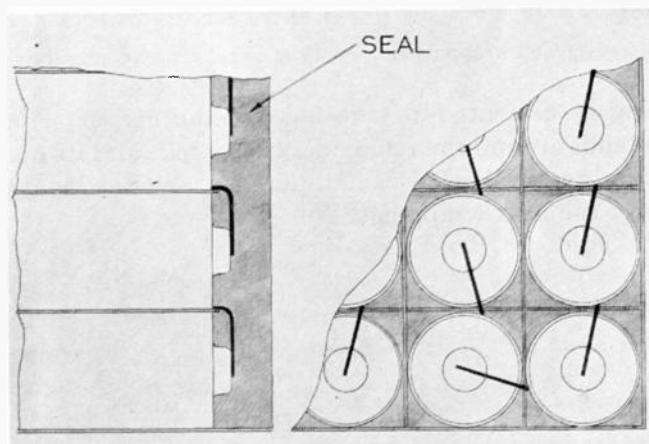
Fig. 5—Space occupied by sealing material and cylindrical cells in old type of B battery.
