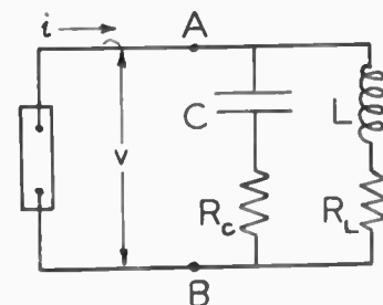
Fig. 1—Simplified oscillator circuit.
