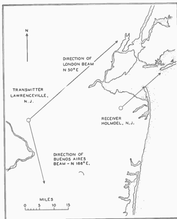
Fig. 3—Transmitter and receiver locations.
