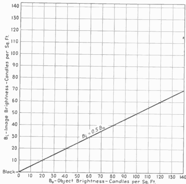
Fig. 1—Typical distortionless brightness transfer characteristic.
