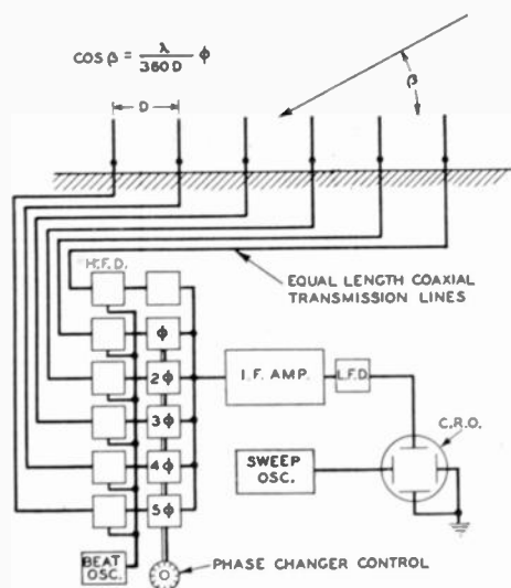
Fig. 1—Musa-type direction-finder-array schematic.
