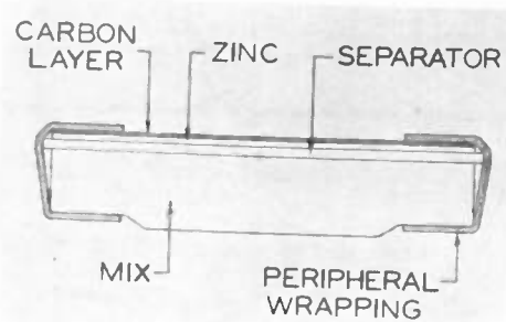
Fig. 11—Individual cell of new wrapped type.
