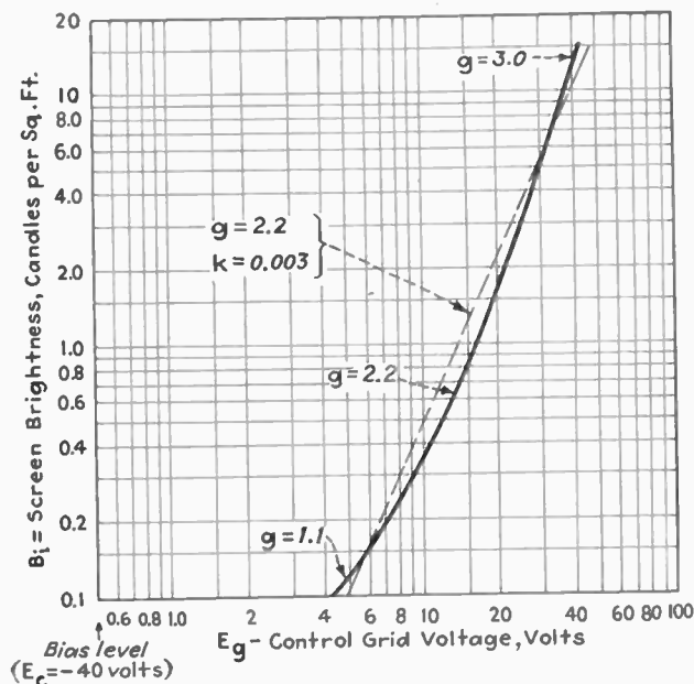
Fig. 11—Transfer characteristic of a typical picture tube (Type 12AP4).
