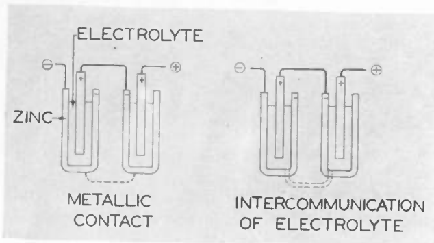
Fig. 8—Short-circuiting of B-battery cells by electrolyte intercommunication.
