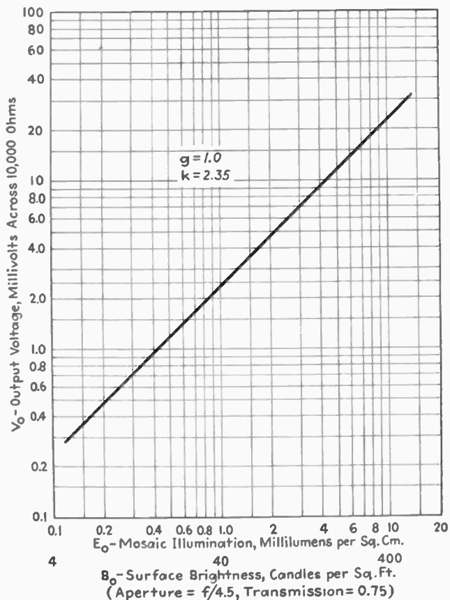
Fig. 10—Transfer characteristic of a typical orthiconoscope.
