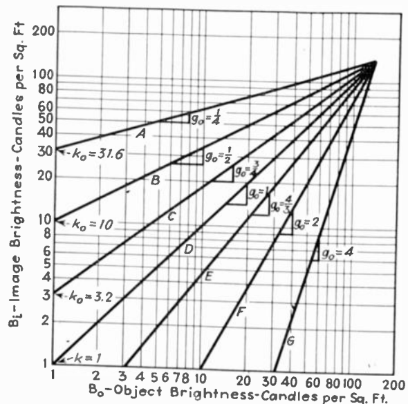
Fig. 5—Power functions displaying brightness distortion, but free of any corresponding contrast distortion.
