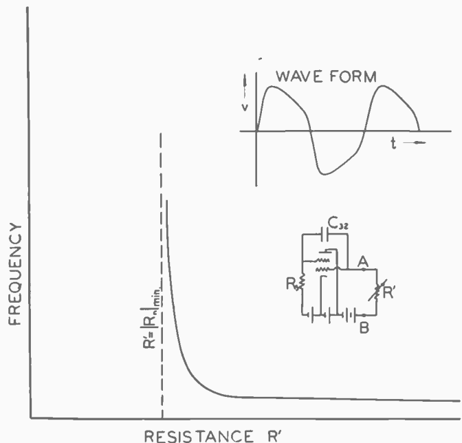
Fig. 8—Relaxation oscillations. (Circuit to left of terminals A-B same as in Fig. 4).
