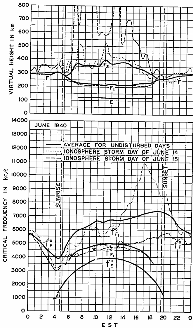
Fig. 1—Virtual heights and critical frequencies of the ionospheric layers, June, 1940.
