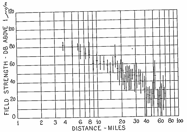
Fig. 6—Summary of field-strength record taken between New York City and Port Jervis, N. Y.
