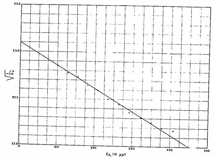
Fig. 11—Plot for determination of residual inductance L'' in lead from circuit to susceptance condenser C_B . Slope = 2440 \times 10^6 Intercept = 23.10 L'' = 2.97 \times 10^{-9} henry
