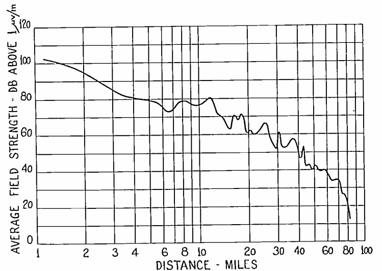
Fig. 7—Average field strength, New York City to Camden, N. J. Corrected to receiving-antenna height of 30 feet.
