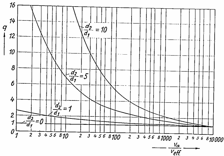
Fig. 4—The factor q which represents the influence of the grid-anode space on the input resistance.
