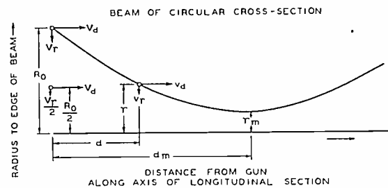
Fig. 1—Diagram of a half-longitudinal section of a beam of circular cross section beyond an electron lens.
