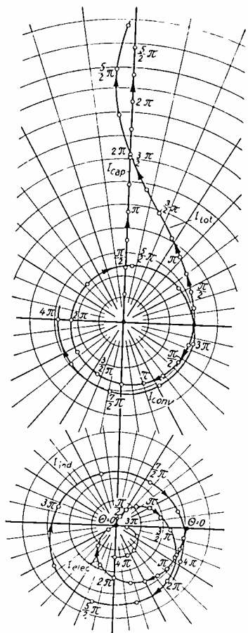
Fig. 1—Vector-diagram of the alternating-currents in a space-charge-limited diode.
