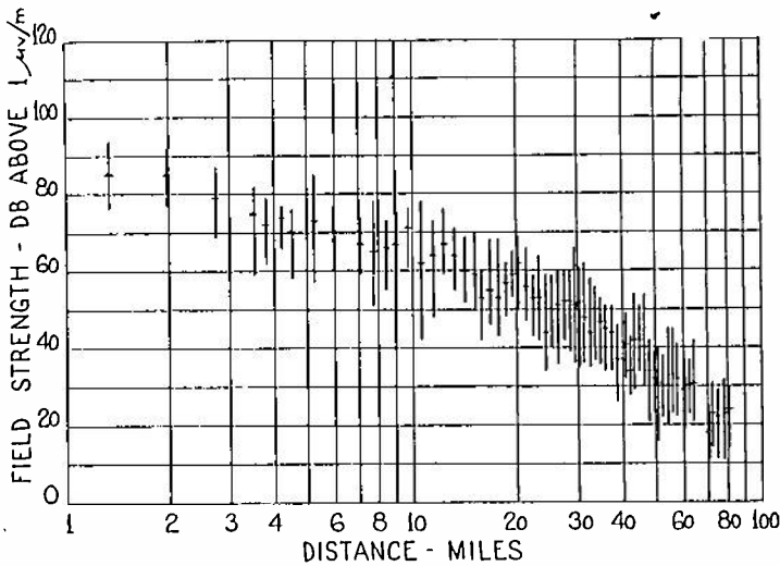
Fig. 5—Summary of field-strength record taken between New York City and Middletown, Conn.
