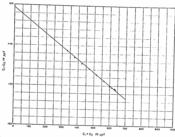
Fig. 9—Plot for determination of common internal inductance L_c of susceptance condenser C_B . Slope = 0.0323 Intercept = 149.4 micromicrofarads L_c = 6.08 \times 10^{-9} henry
