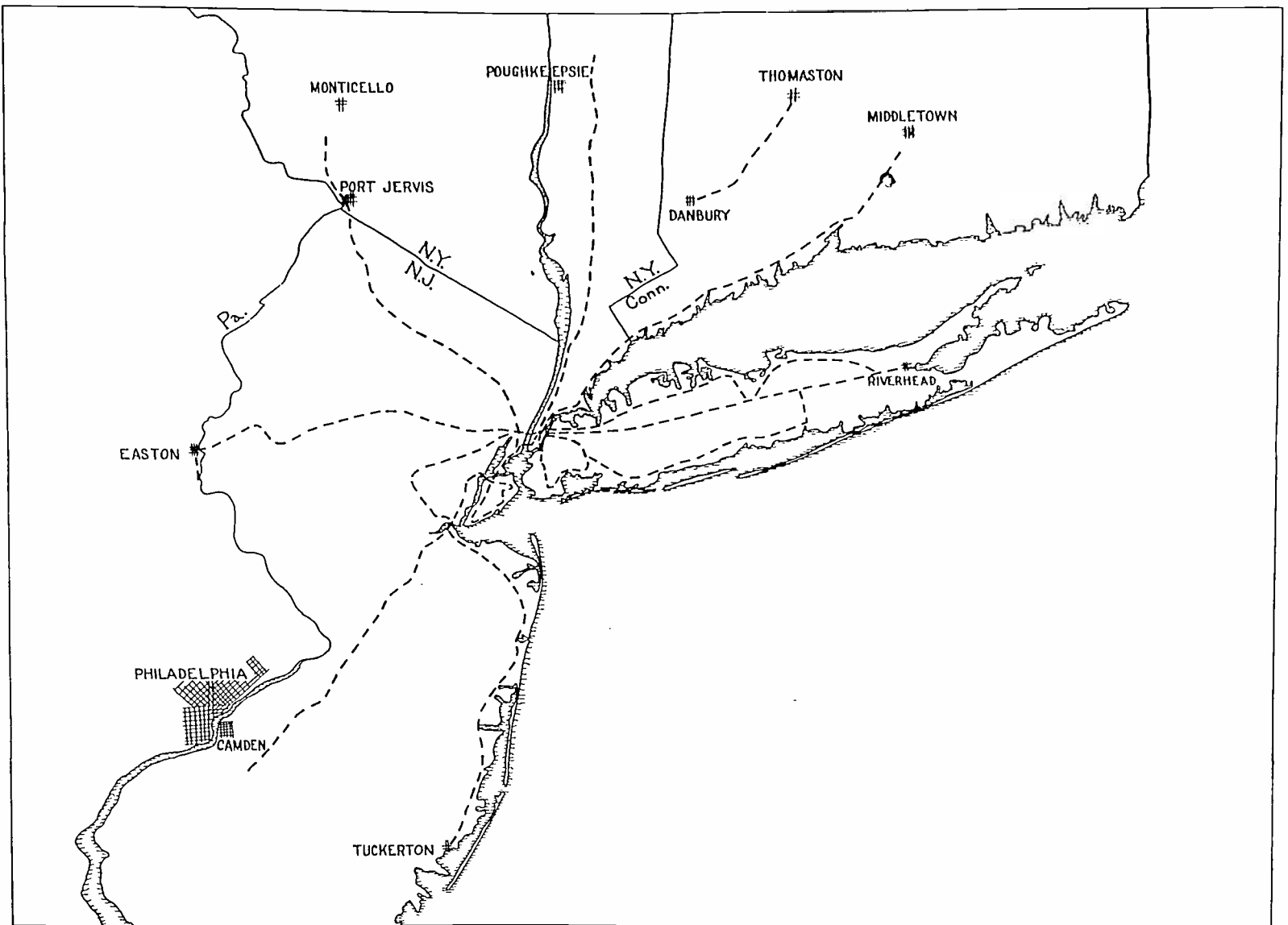
Fig. 2—Routes covered by mobile field-strength survey. 52.75 megacycles, 3.6 kilowatts. May and June, 1937.
