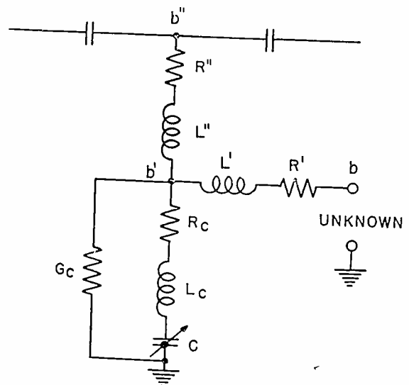
Fig. 8—Approximate equivalent circuit of susceptance condenser C B including residual resistances caused by losses in metal structure and dielectric supports.
