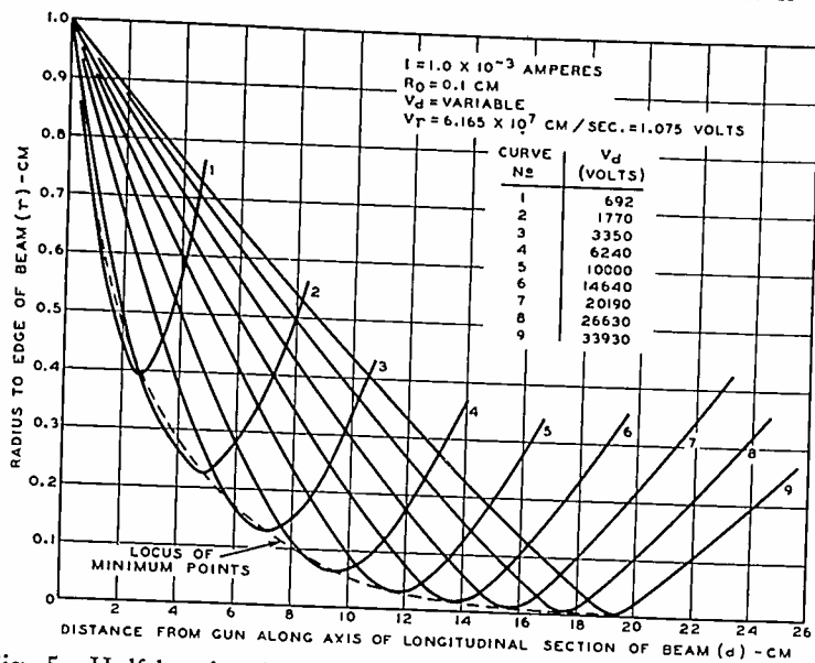
Fig. 5—Half-longitudinal sections of an electron beam of circular cross section with the beam voltage as a parameter. The other variables, i.e., initial radial component of electron velocity, beam current, and initial beam radius are held constant.
