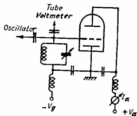
Fig. 5—Schematic diagram of the test circuit for investigating the grid input impedance.
