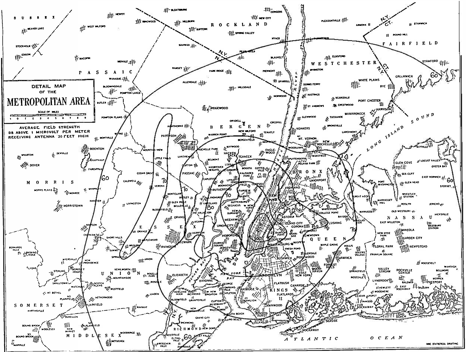
Fig. 9—Field strength near New York City.
