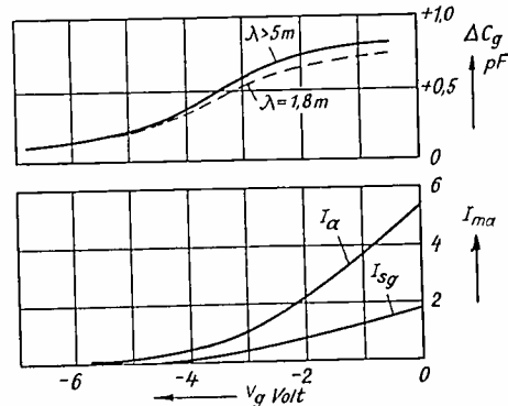
Fig. 9— R_g and \Delta C_g of the acorn-type pentode SF1A for different wavelengths ( V_a = 150 volts, V_{sg} = 75 volts).
