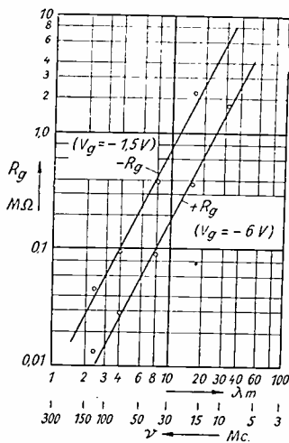
Fig. 12—Positive ( V_g = -6 Volts) and negative ( V_g = -1.5 Volts) input resistance of the same tube as in fig. 14 as a function of frequency.
