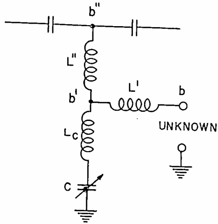
Fig. 7—Approximate equivalent circuit of susceptance condenser C B showing residual inductances of leads to internal circuit and to panel terminal and common residual inductance in stack structure.
