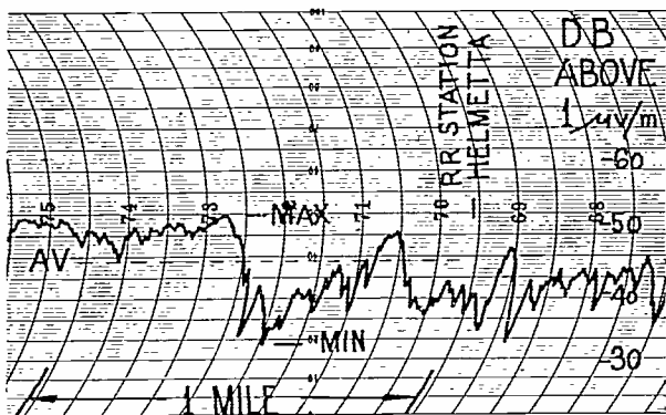
Fig. 3—Sample of mobile recording.
