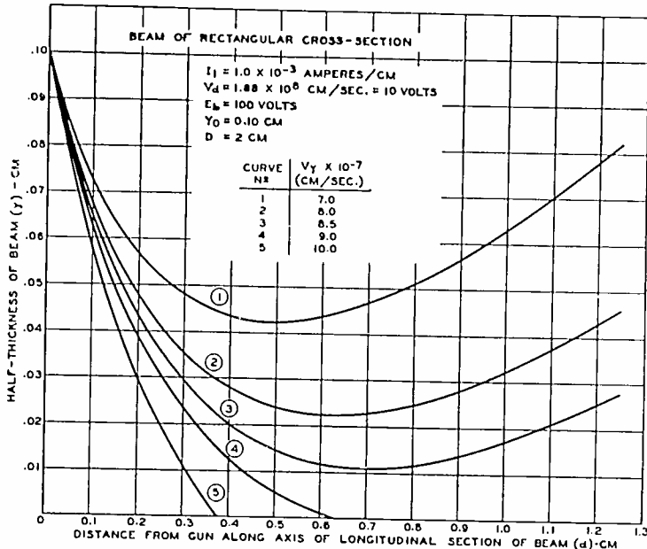
Fig. 9—Half-longitudinal section of an electron beam of rectangular cross section with the initial perpendicular component of electron velocity as a parameter. The variables, i.e., beam current per unit length, beam voltage, initial beam thickness, anode voltage, and distance from anode to cathode are held constant.
