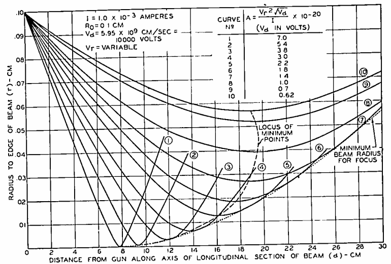
Fig. 3—Half-longitudinal sections of an electron beam of circular cross section with the initial radial component of electron velocity as a parameter. The other variables, i.e., beam current, initial radius, and voltage are held constant.
