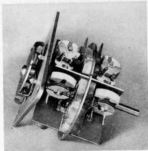
Fig. 5—Range switch used to change the scale of the conductance condenser. Different small condensers carried on this switch are connected in parallel with the C' and C'' condensers shown in Fig. 4 for operation at frequencies of 1, 3, and 10 megacycles.
