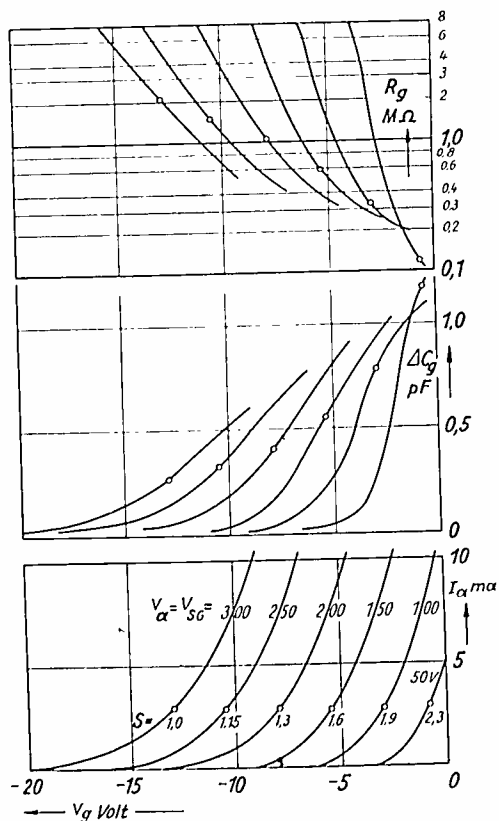
Fig. 8— R_g and \Delta C_g of a pentode for a wavelength of 24 meters.
