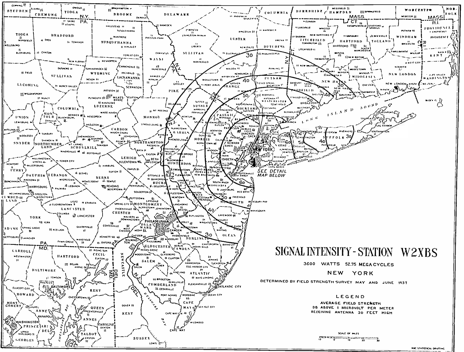
Fig. 8—Field strength beyond the Metropolitan area.
