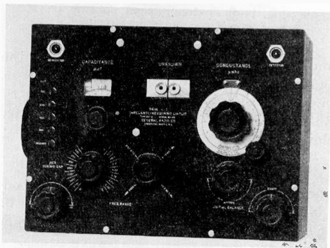
Fig. 2—Panel view of experimental model of twin-T impedance-measuring circuit. At the left of the panel are the susceptance condenser (CAPACITANCE \mu\mu\text{f} ) and the auxiliary tuning condenser (AUX. TUNING CAP.). At the right are the conductance condenser (CONDUCTANCE \mu\text{mho} ), and the parallel trimmer condensers (INITIAL BALANCE). The remaining controls (FREQ. RANGE) are the coil switch, at the left, and the conductance range switch, at the right.
