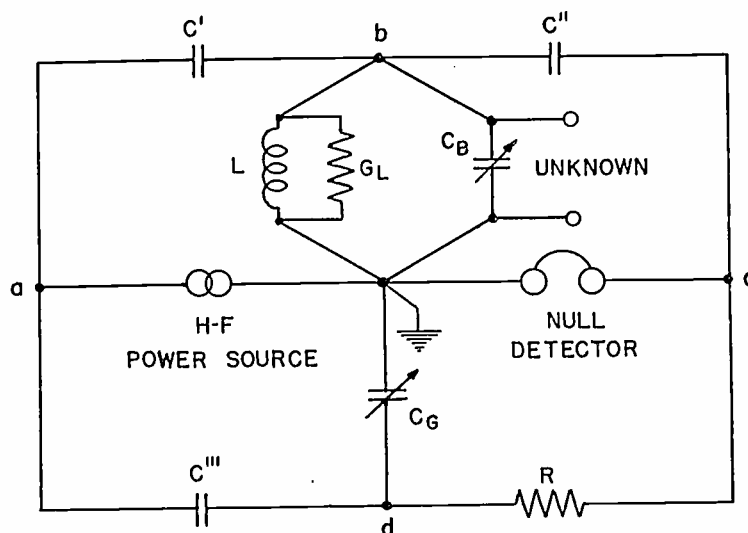
Fig. 1—Basic circuit diagram of twin-T impedance-measuring circuit.
